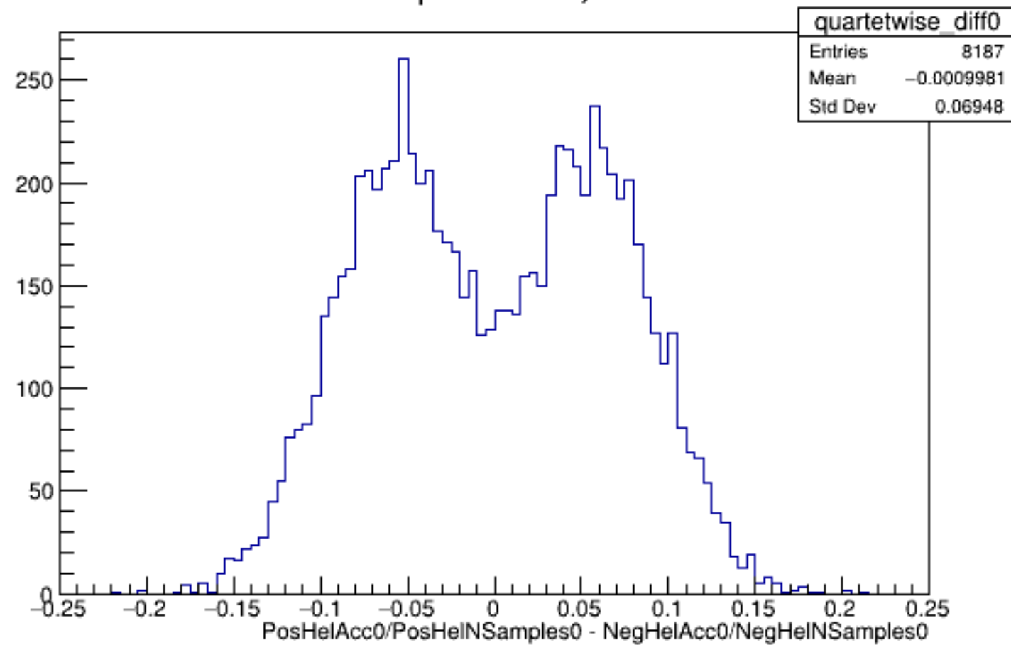
Run 5860 quartetwise, Diffs0: All
