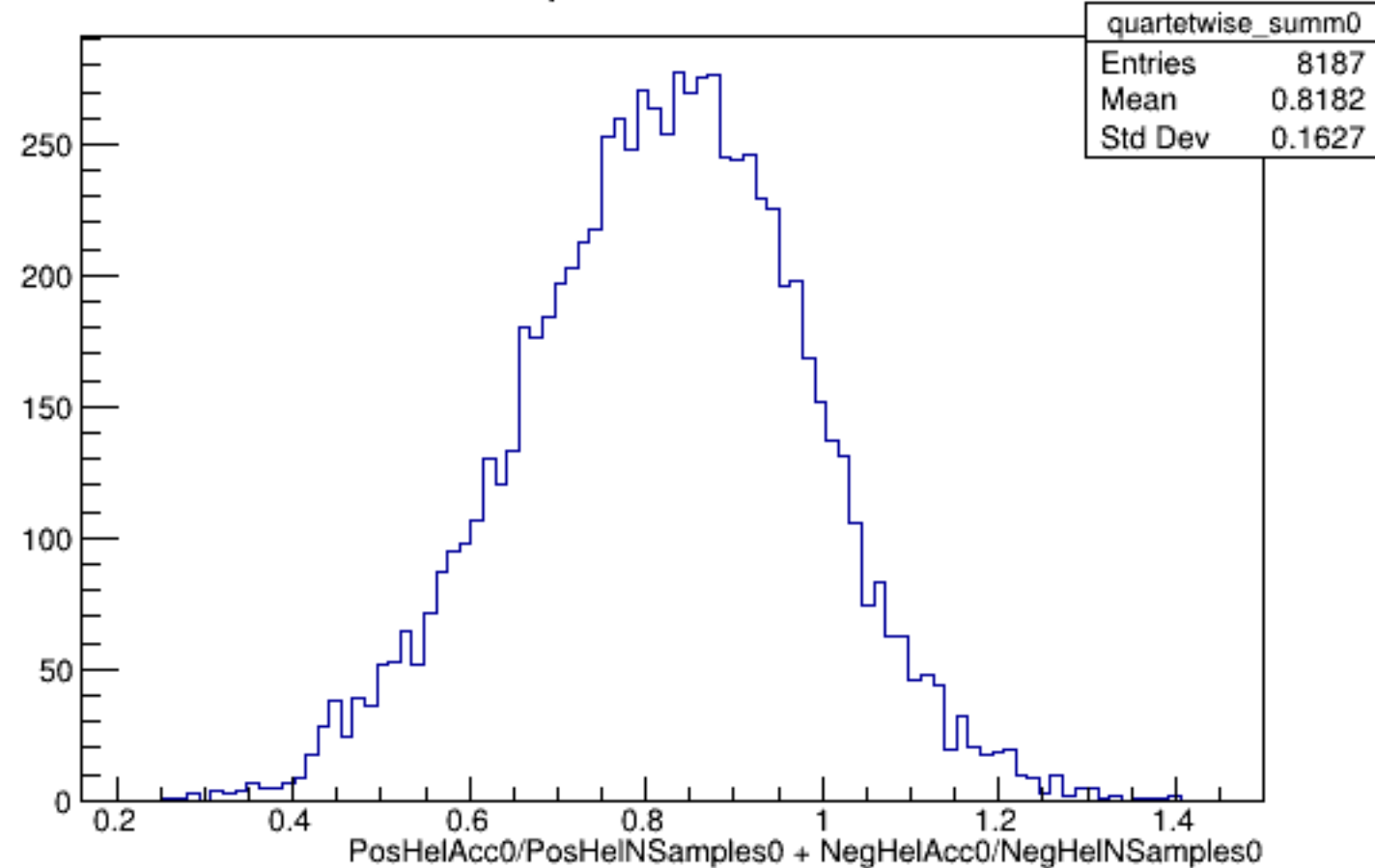
Run 5860 quartetwise, Sums0: All
