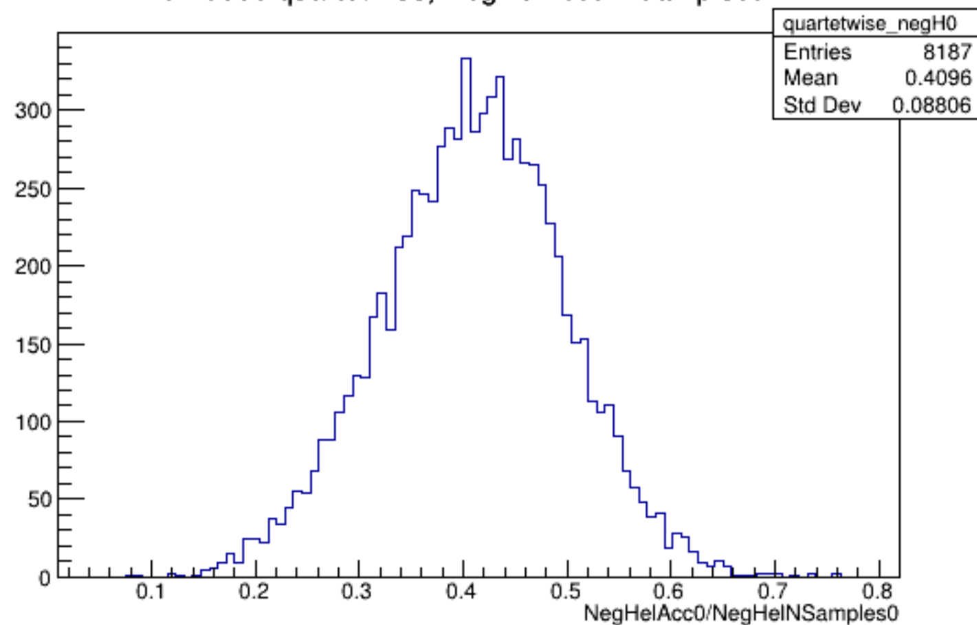
Run 5860 quartetwise, NegHelAcc0/NSamples0: All
