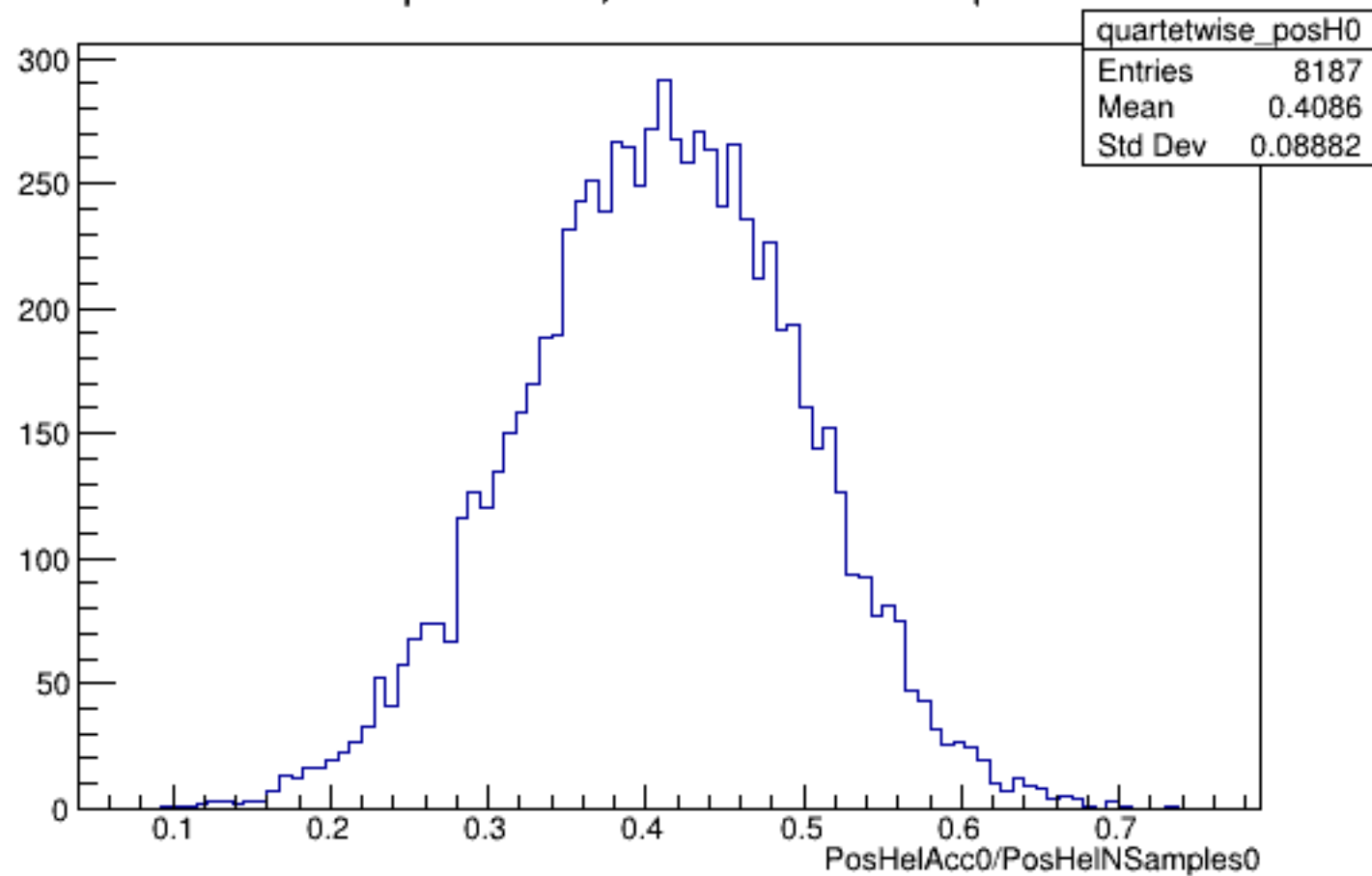
Run 5860 quartetwise, PosHelAcc0/NSamples0: All
