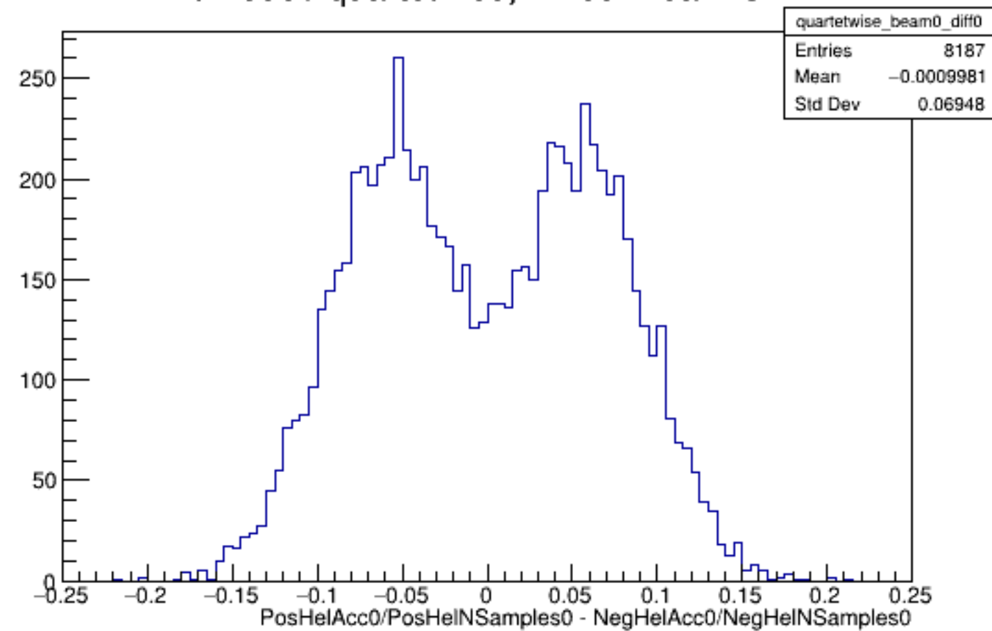
Run 5860 quartetwise, Diffs0: Beam OFF
