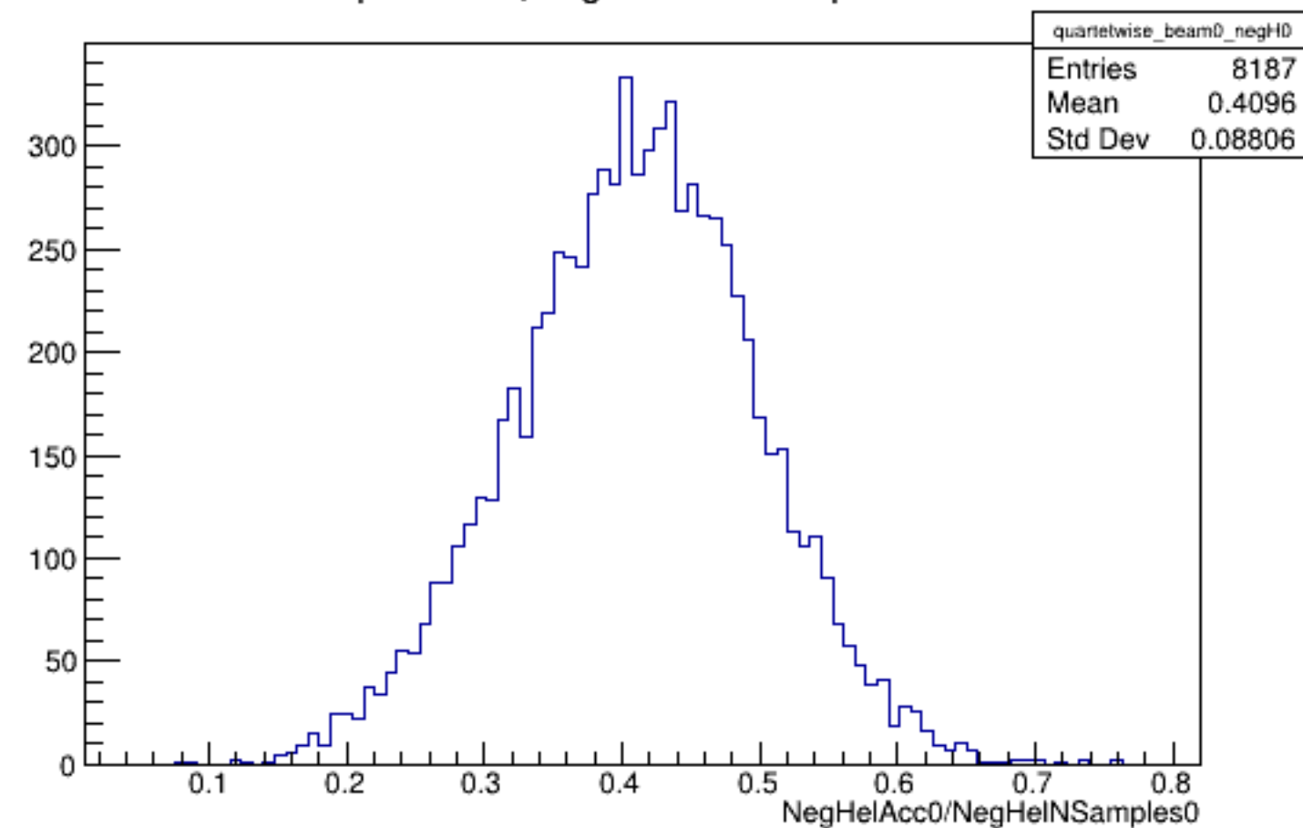
Run 5860 quartetwise, NegHelAcc0/NSamples0: Beam OFF
