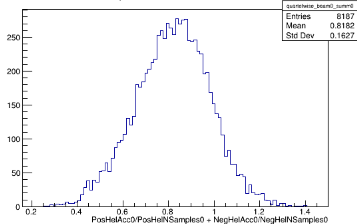
Run 5860 quartetwise, Sums0: Beam OFF
