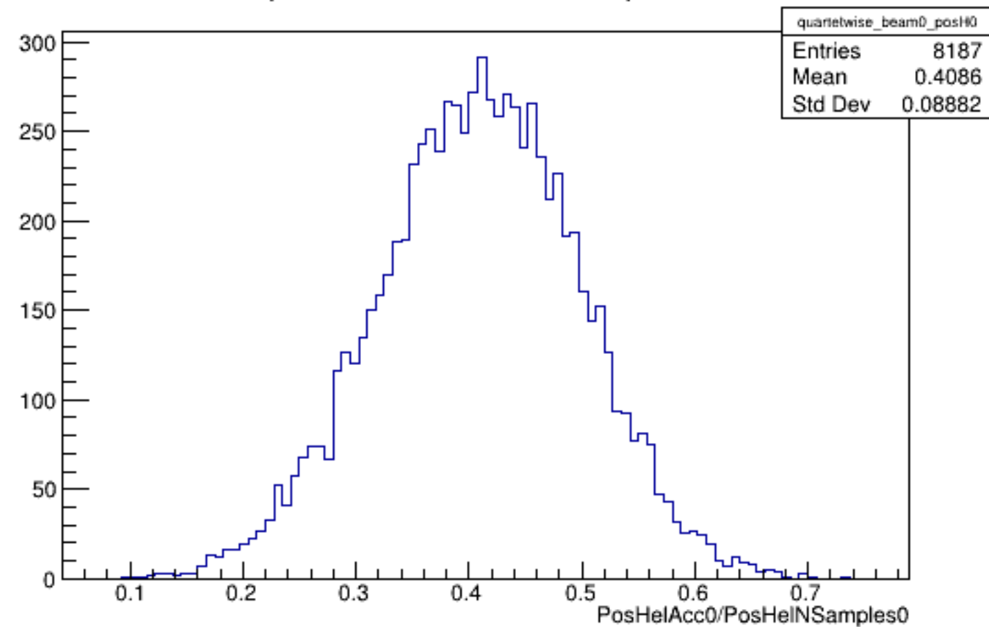
Run 5860 quartetwise, PosHelAcc0/NSamples0: Beam OFF
