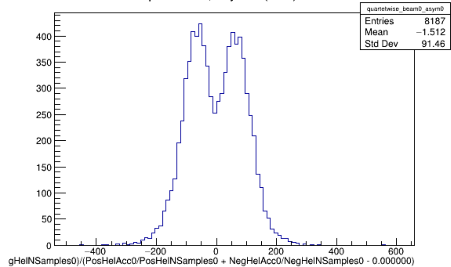
Run 5860 quartetwise, Asyms0 (Raw): Beam OFF
