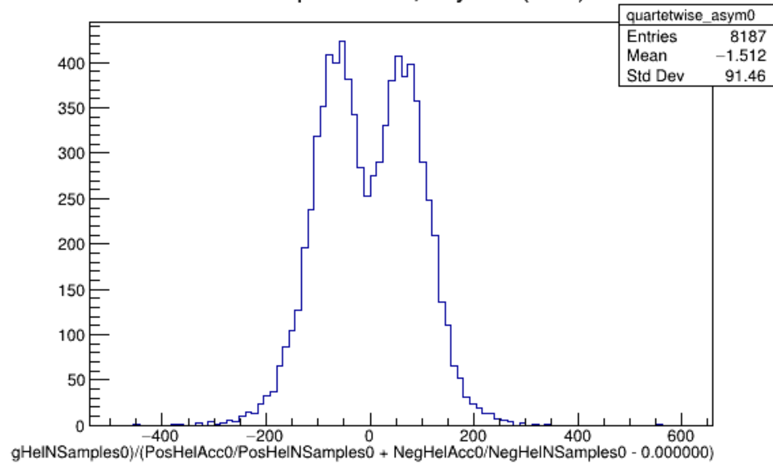
Run 5860 quartetwise, Asyms0 (Raw): All
