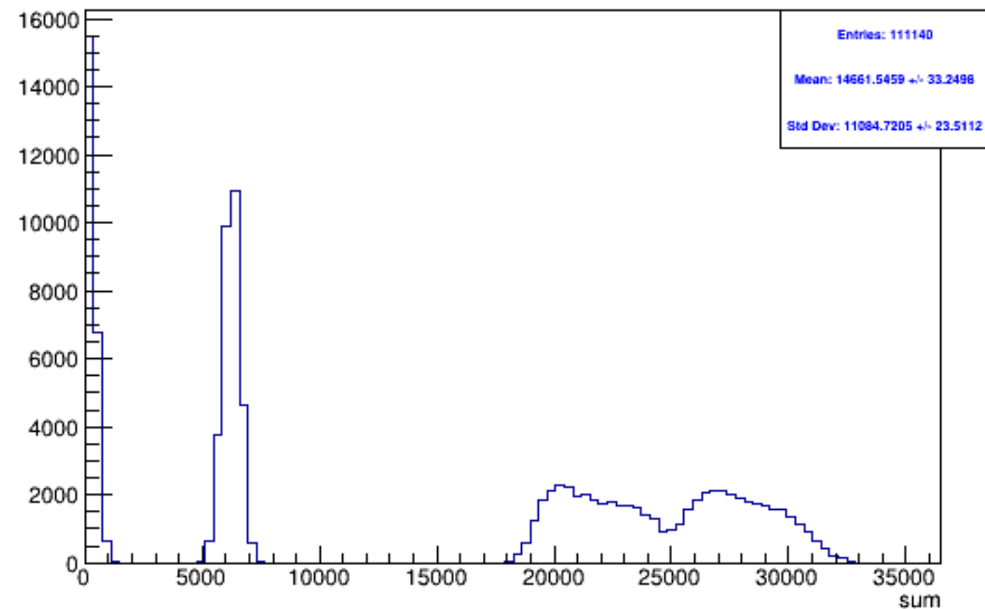
Run 5862 triggerwise, sums: Beam OFF
