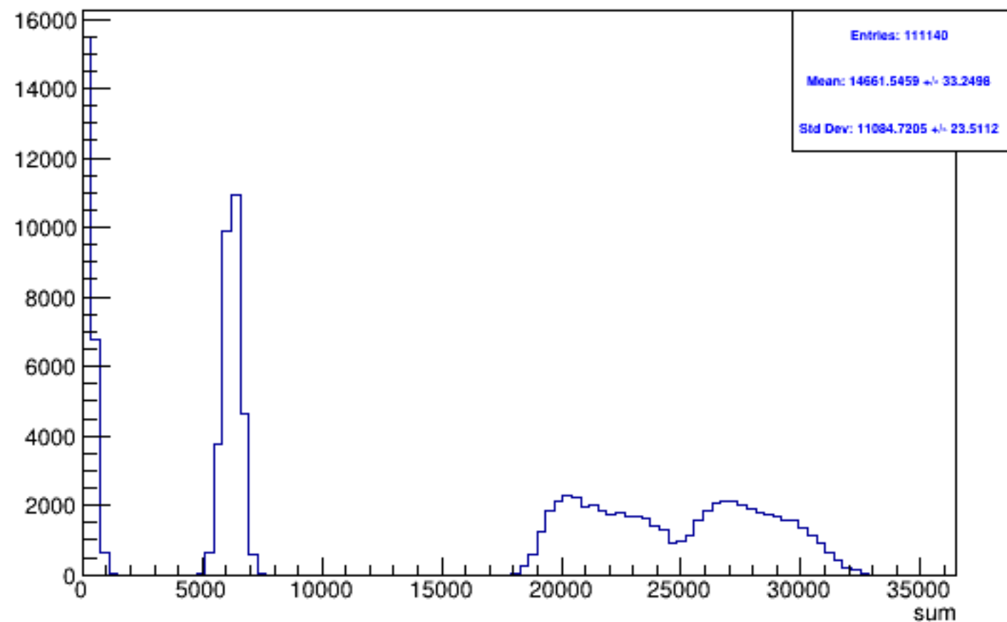
Run 5862 triggerwise, sums: All
