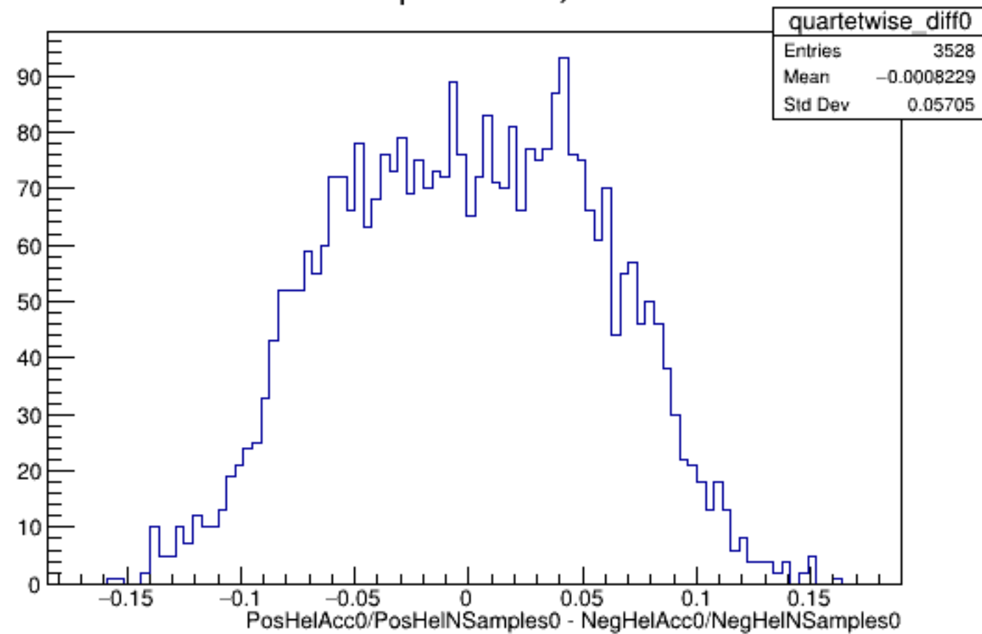
Run 5867 quartetwise, Diffs0: All
