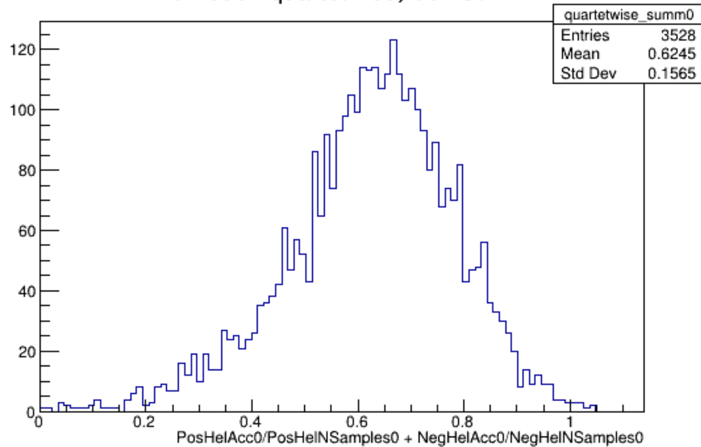
Run 5867 quartetwise, Sums0: All
