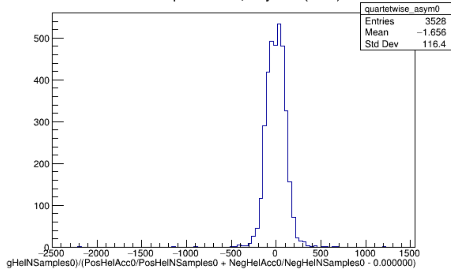
Run 5867 quartetwise, Asyms0 (Raw): All
