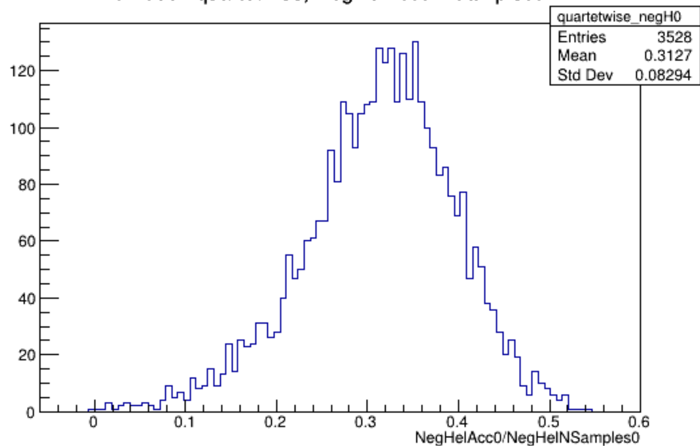
Run 5867 quartetwise, NegHelAcc0/NSamples0: All
