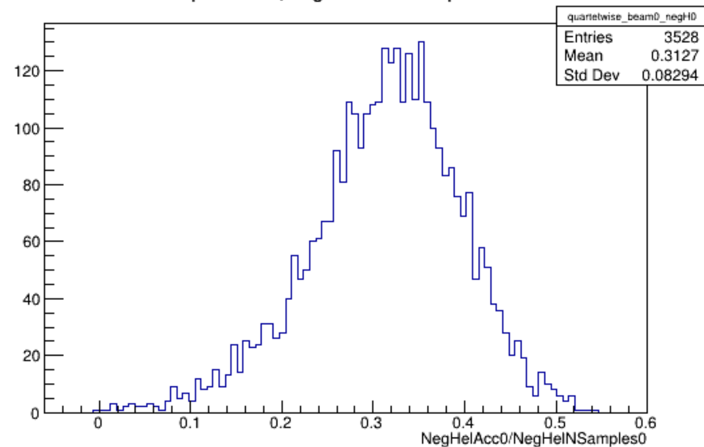
Run 5867 quartetwise, NegHelAcc0/NSamples0: Beam OFF
