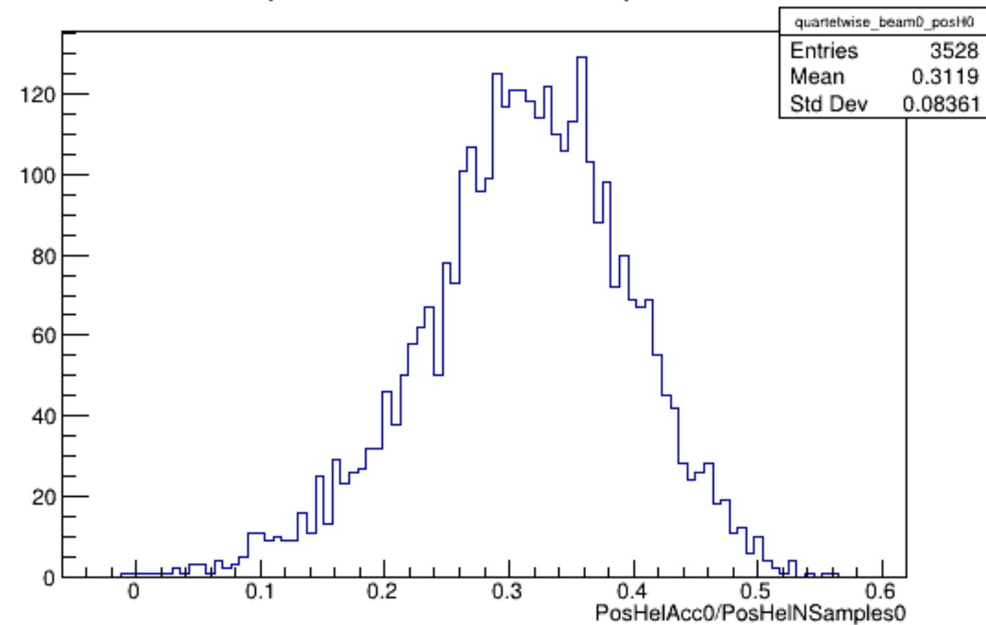
Run 5867 quartetwise, PosHelAcc0/NSamples0: Beam OFF
