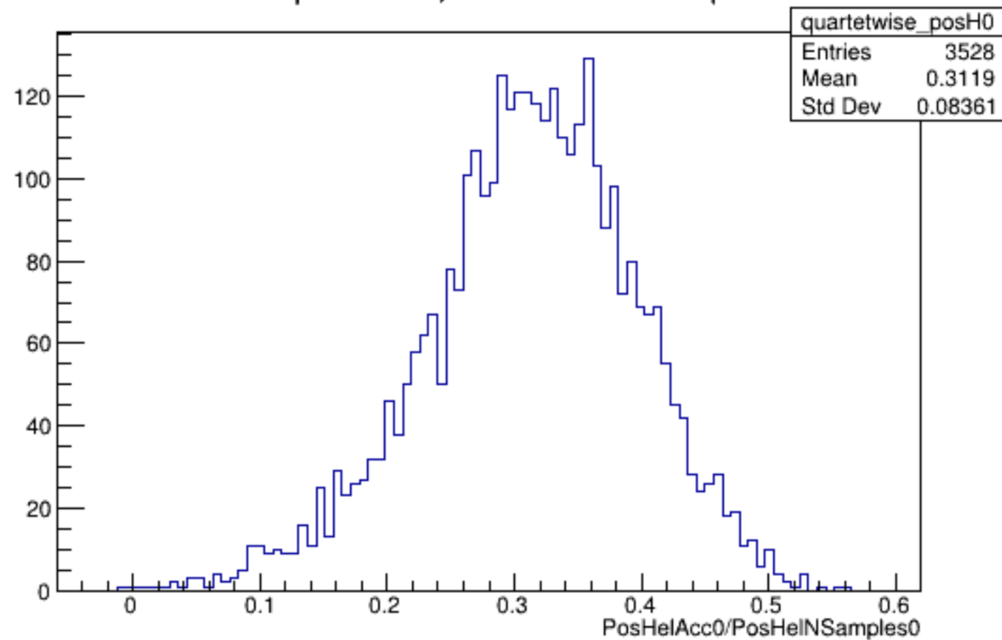
Run 5867 quartetwise, PosHelAcc0/NSamples0: All
