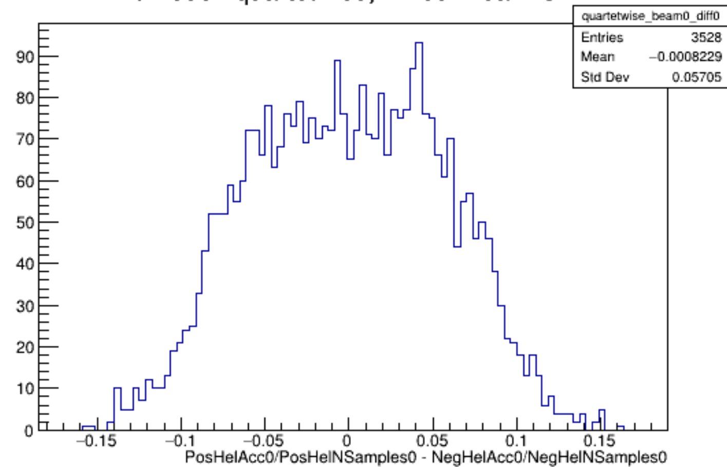
Run 5867 quartetwise, Diffs0: Beam OFF
