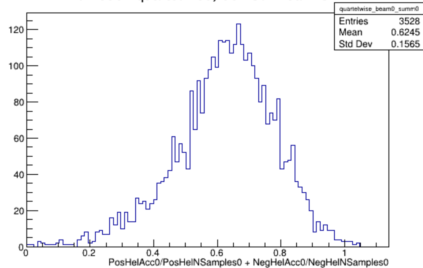
Run 5867 quartetwise, Sums0: Beam OFF
