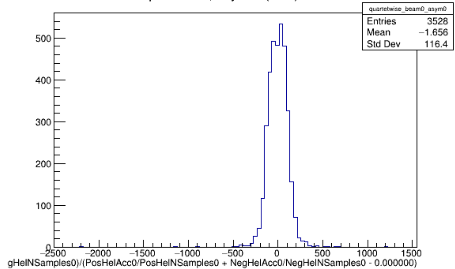
Run 5867 quartetwise, Asyms0 (Raw): Beam OFF
