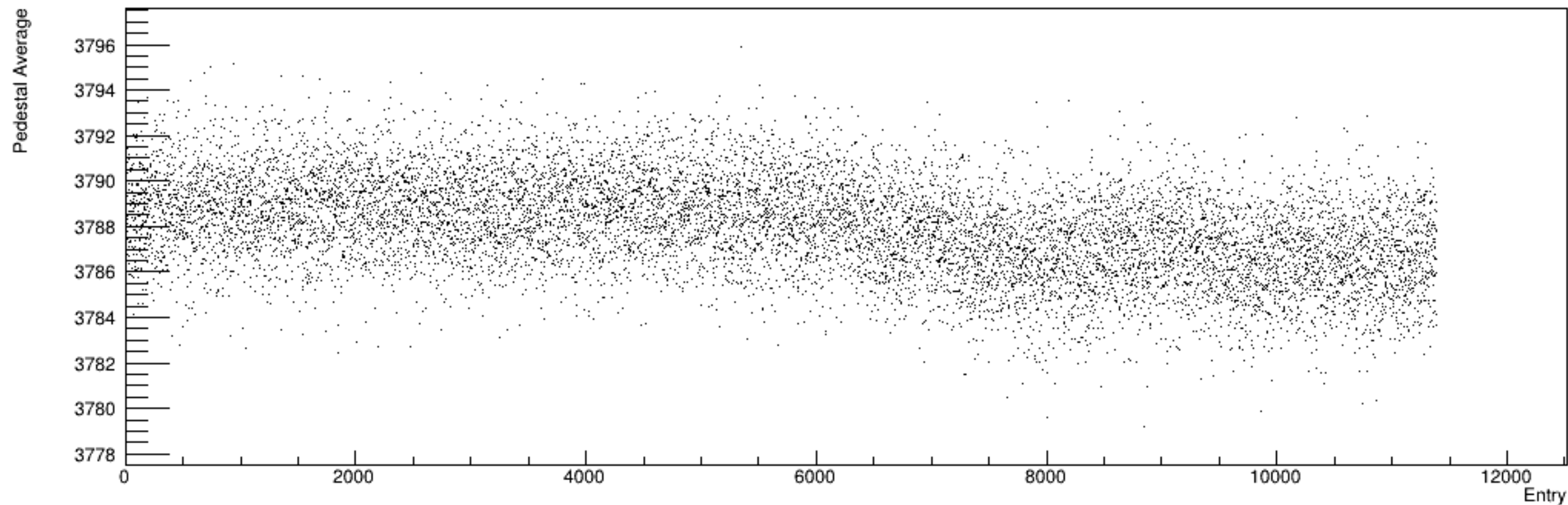
Run 5867, snapshots: Pedestal vs. Time
