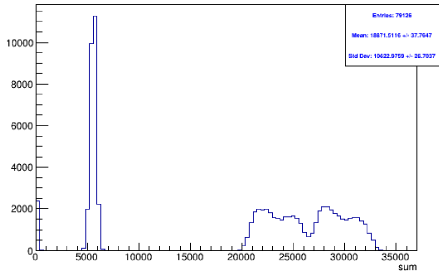
Run 5871 triggerwise, sums: All
