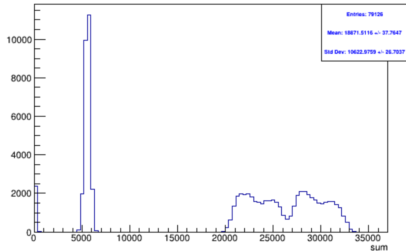
Run 5871 triggerwise, sums: Beam OFF
