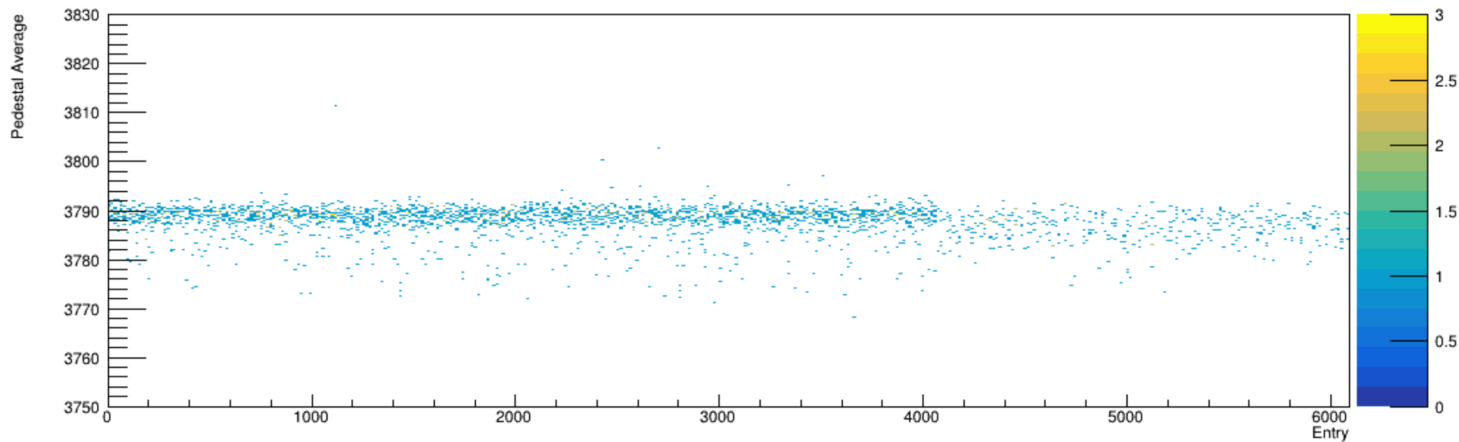
Run 5878, snapshots: Pedestal vs. Time
