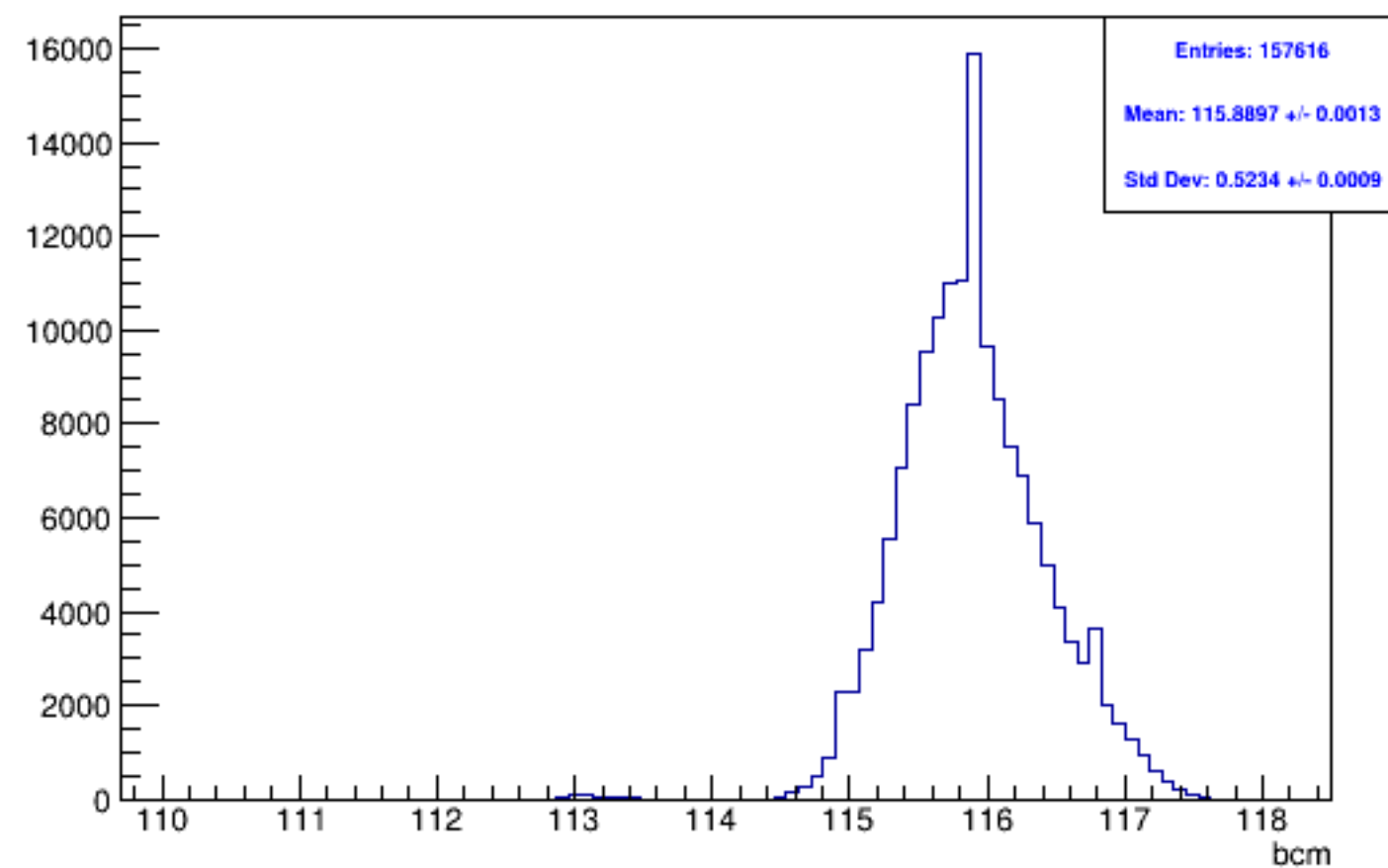
Run 5880, mpwise, BCM: Beam ON, Laser OFF
