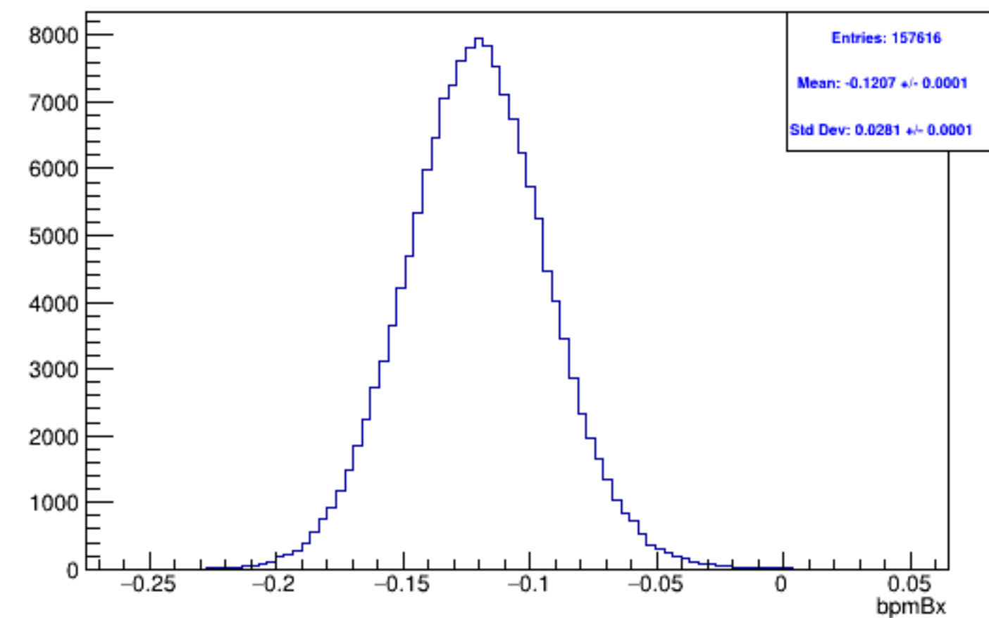
Run 5880, mpswise, bpmBx: Beam ON, Laser OFF
