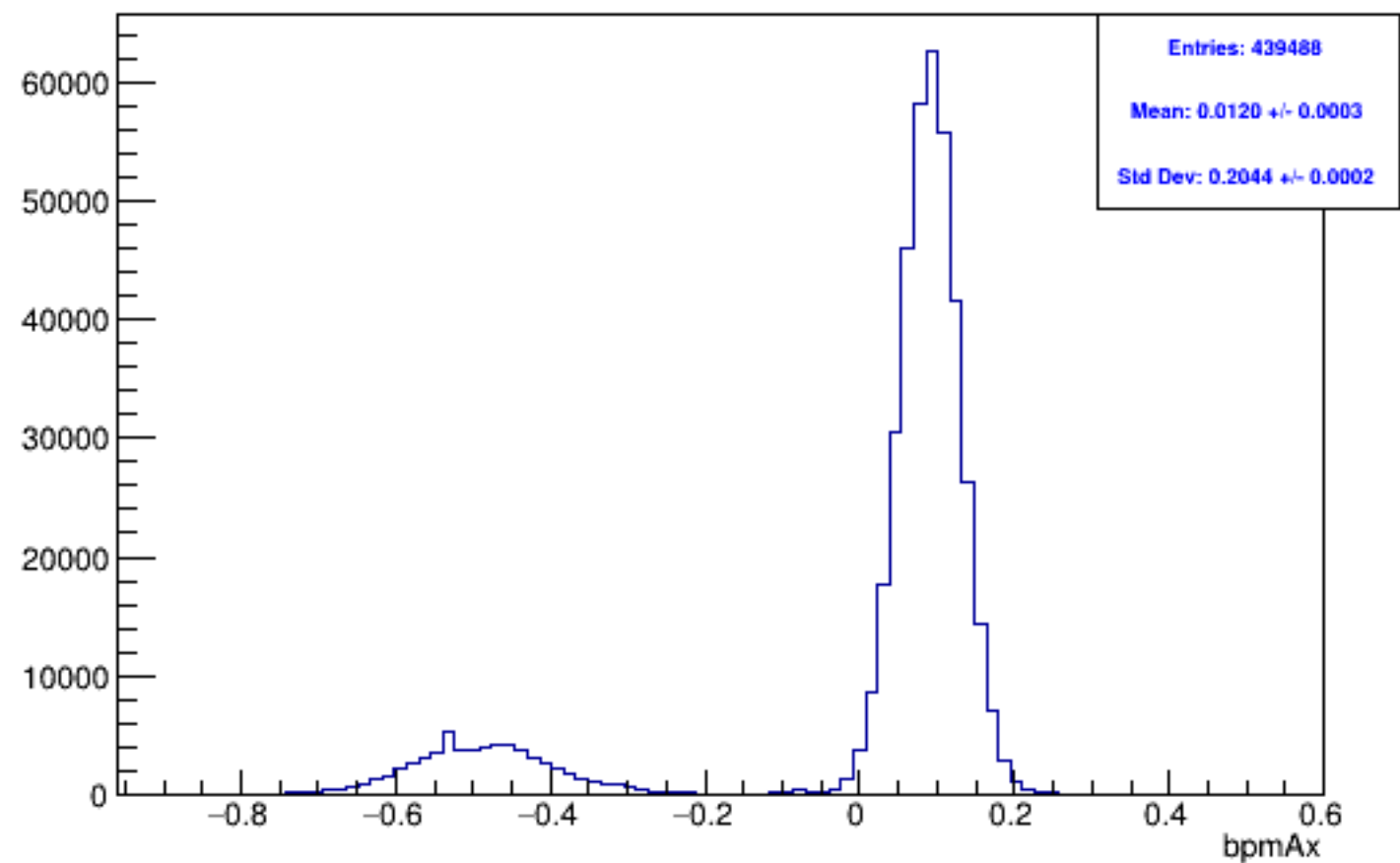
Run 5880 mpwise, bpmAx: All
