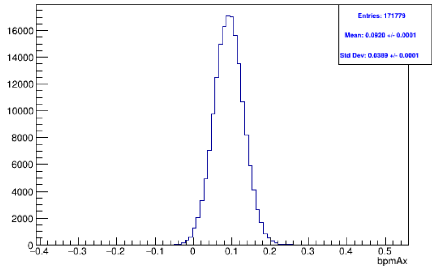
Run 5880, mpwise, bpmAx: Beam ON, Laser ON
