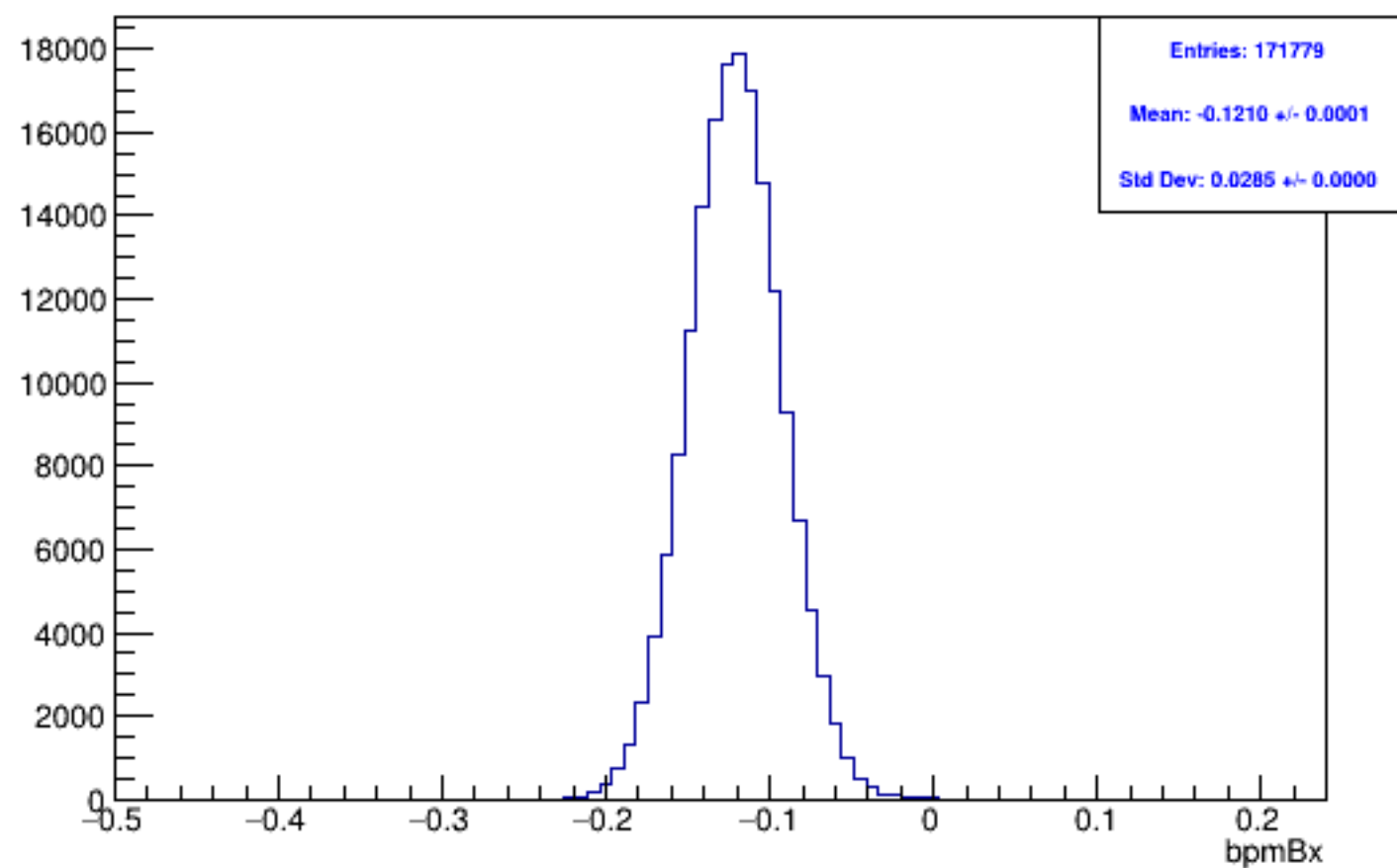
Run 5880, mpswise, bpmBx: Beam ON, Laser ON
