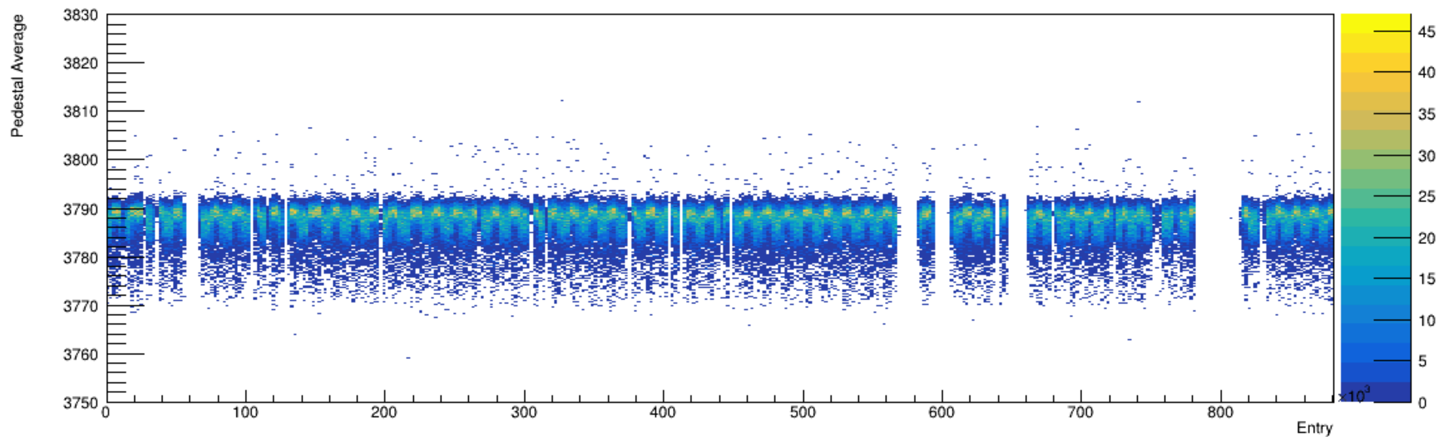
Run 5881, snapshots: Pedestal vs. Time
