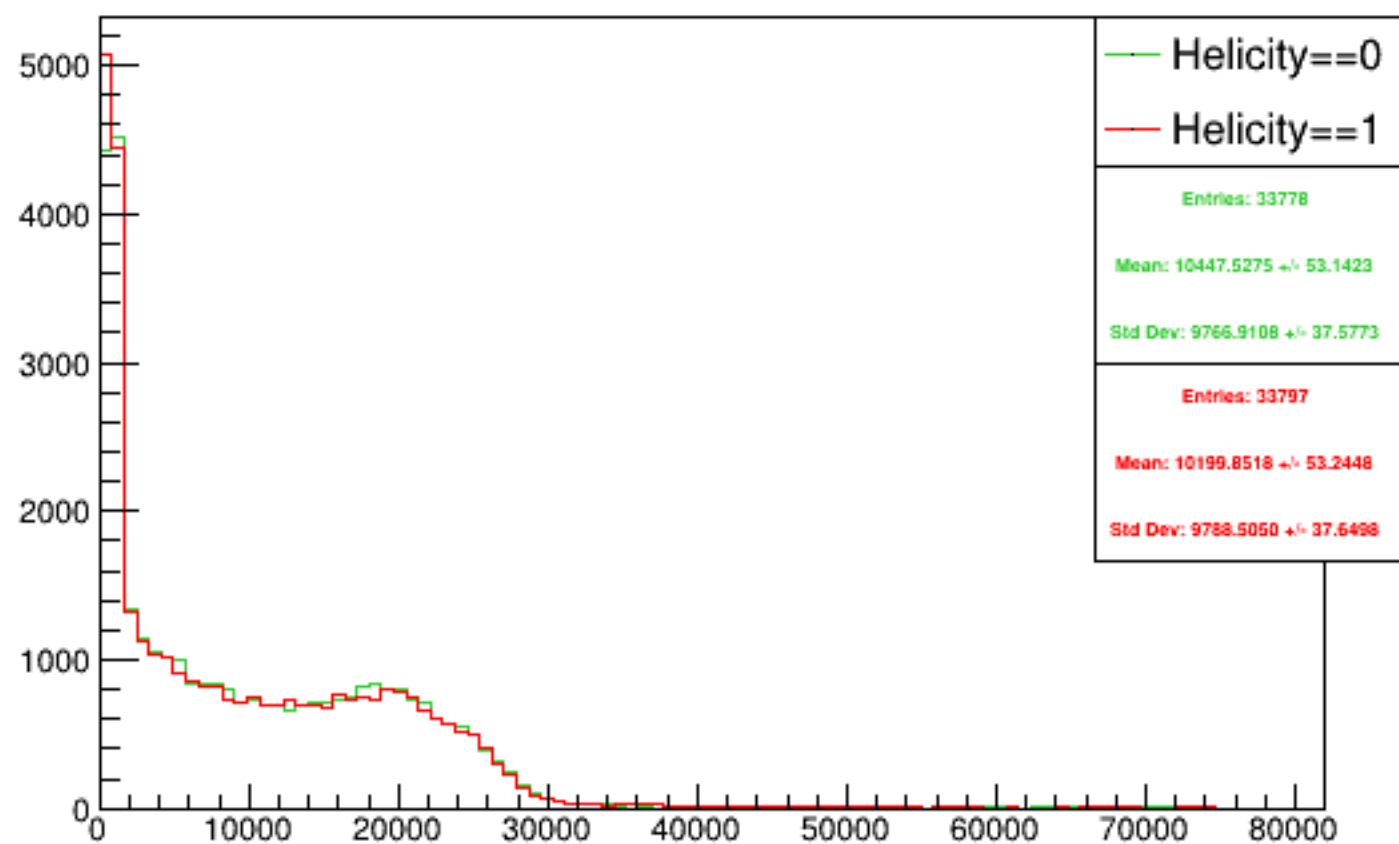
Run 5884 triggerwise, sums: Beam ON, Laser ON
