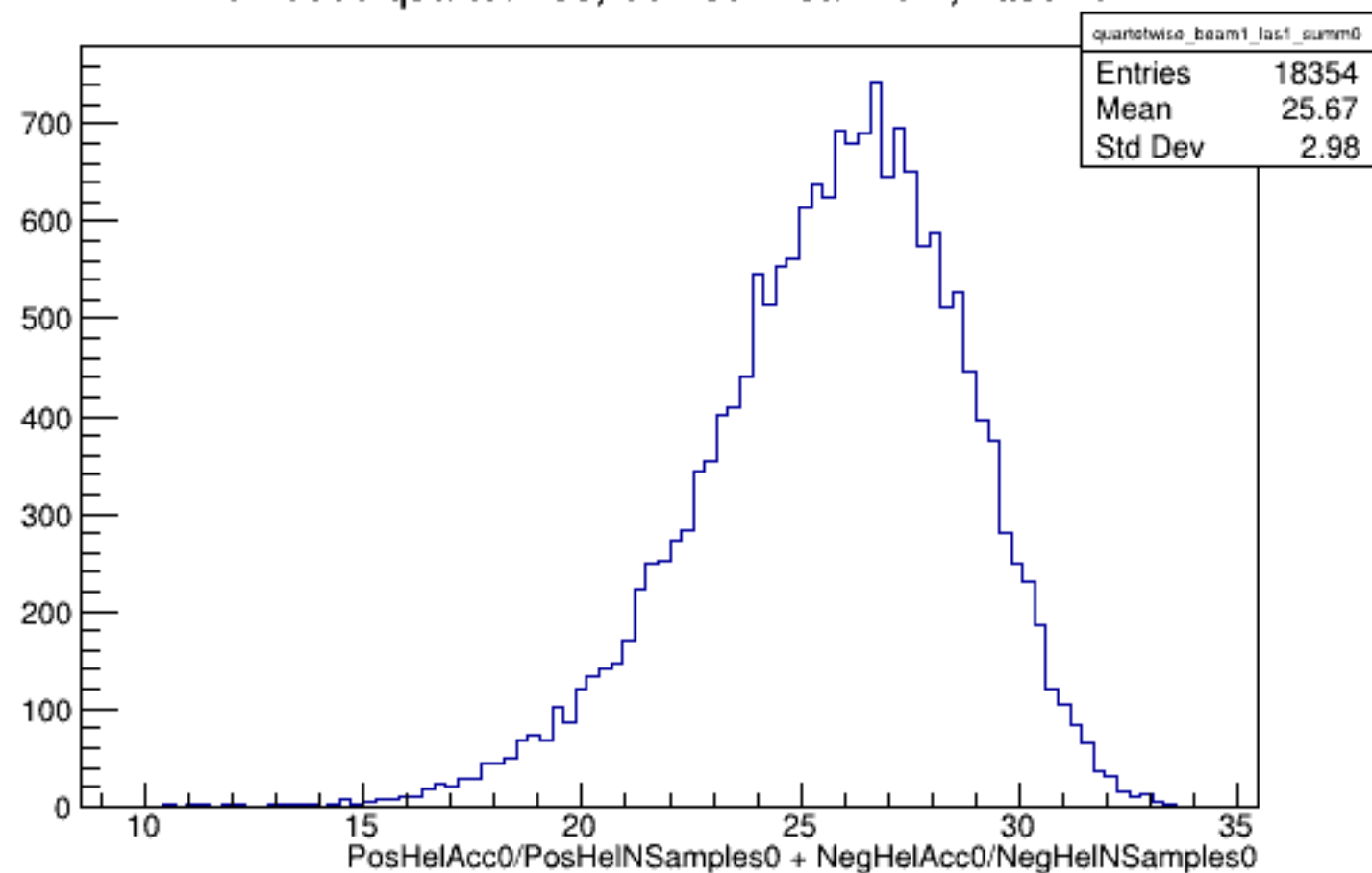
Run 5885 quartetwise, Sums0: Beam ON, Laser ON
