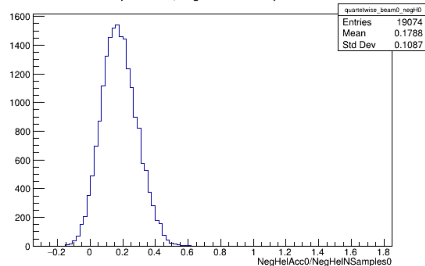
Run 5885 quartetwise, NegHelAcc0/NSamples0: Beam OFF
