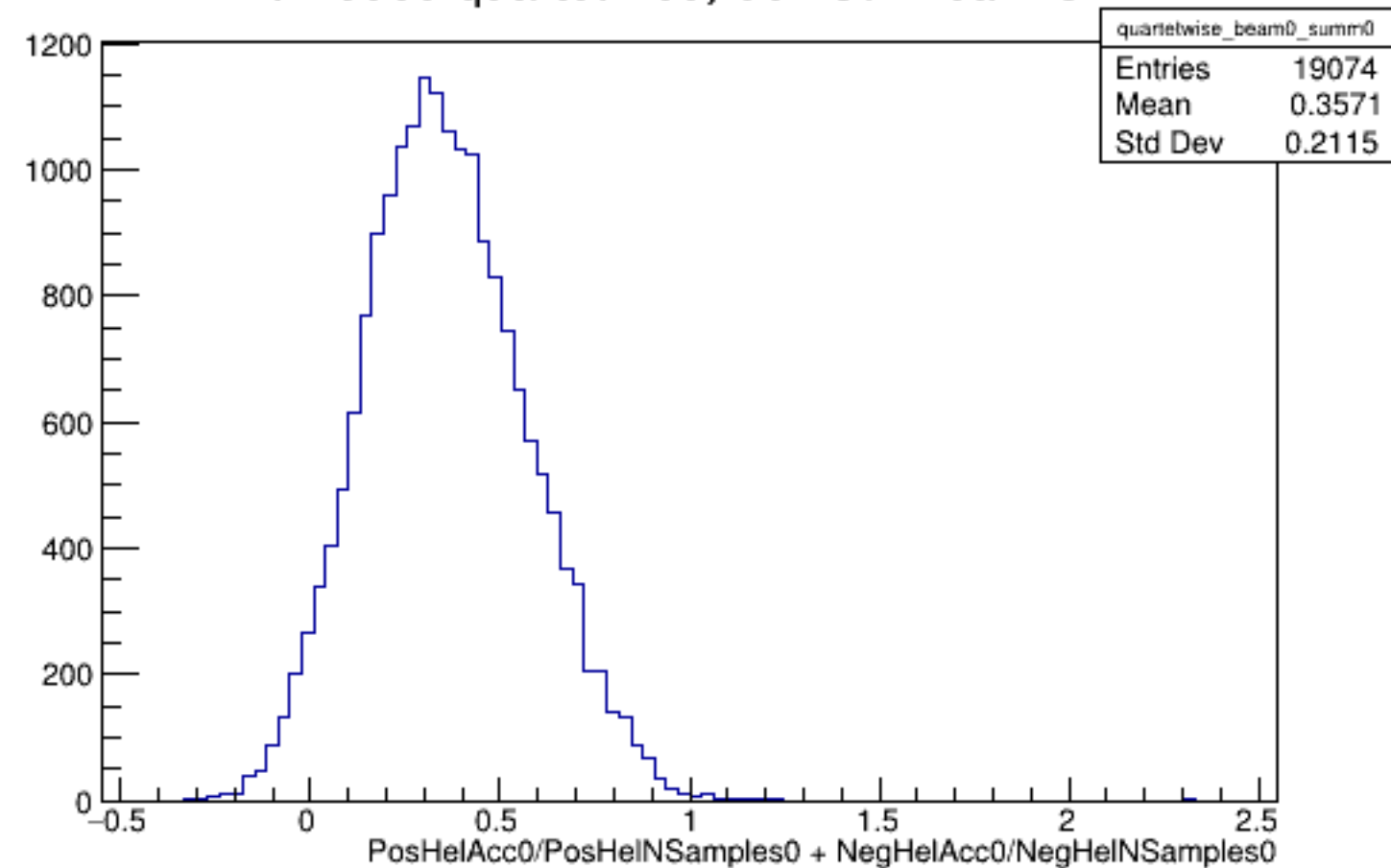
Run 5885 quartetwise, Sums0: Beam OFF
