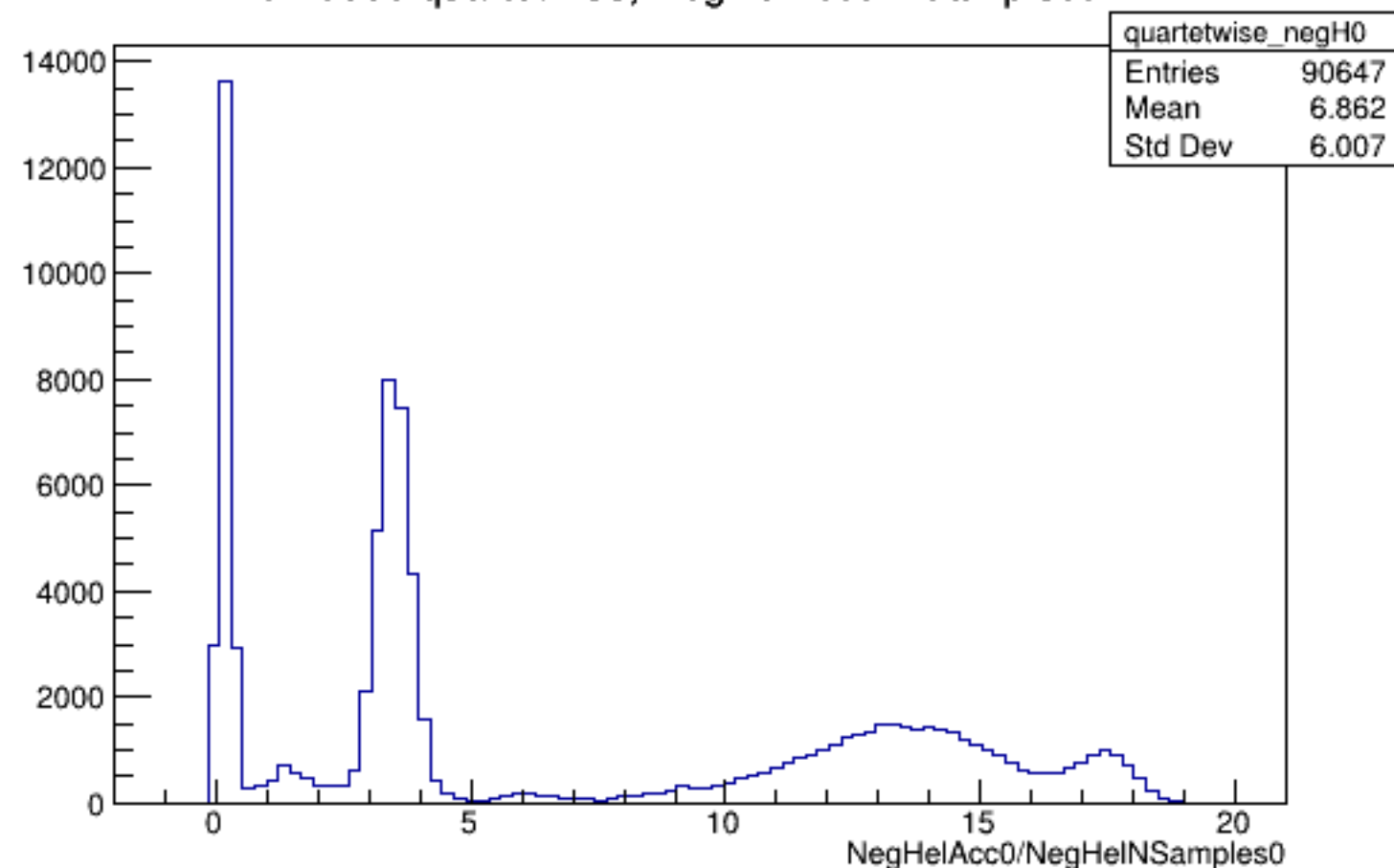
Run 5885 quartetwise, NegHelAcc0/NSamples0: All
