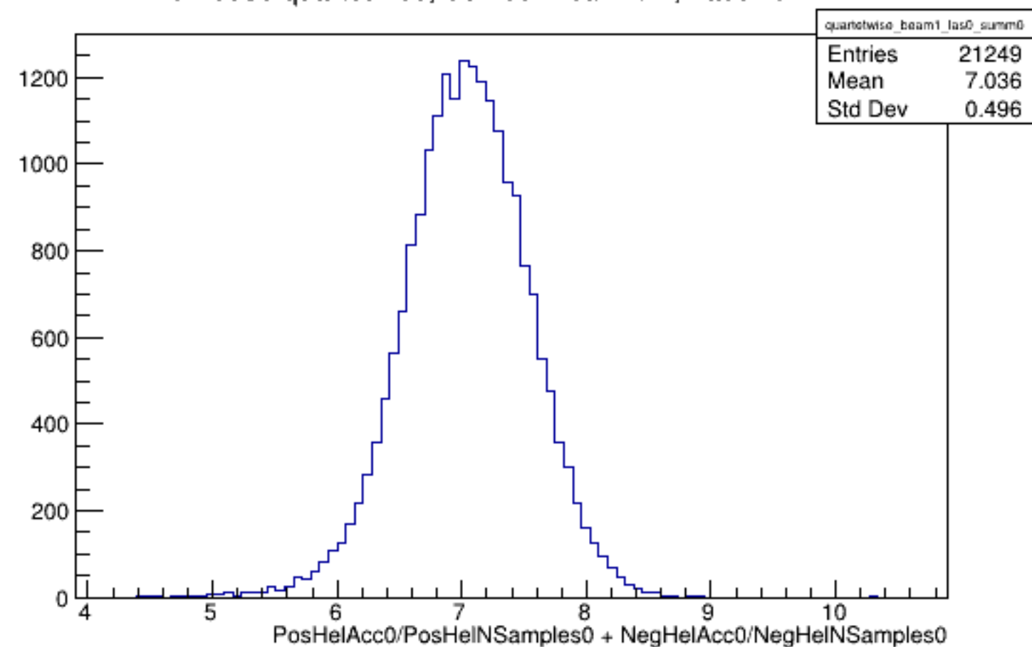
Run 5885 quartetwise, Sums0: Beam ON, Laser OFF
