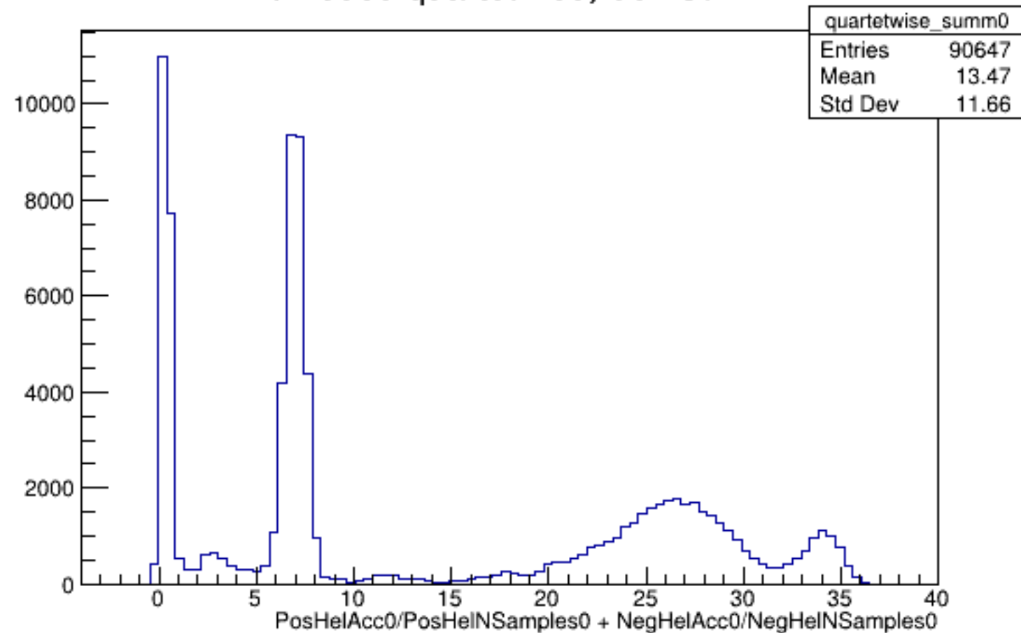
Run 5885 quartetwise, Sums0: All
