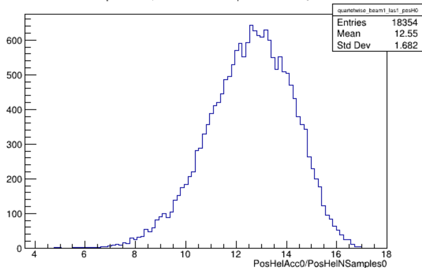
Run 5885 quartetwise, PosHelAcc0/NSamples0: Beam ON, Laser ON
