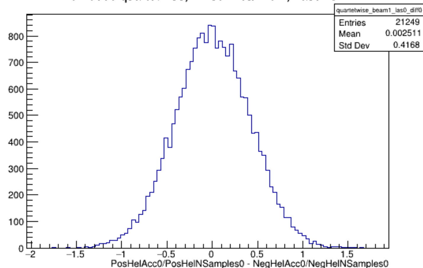
Run 5885 quartetwise, Diffs0: Beam ON, Laser OFF
