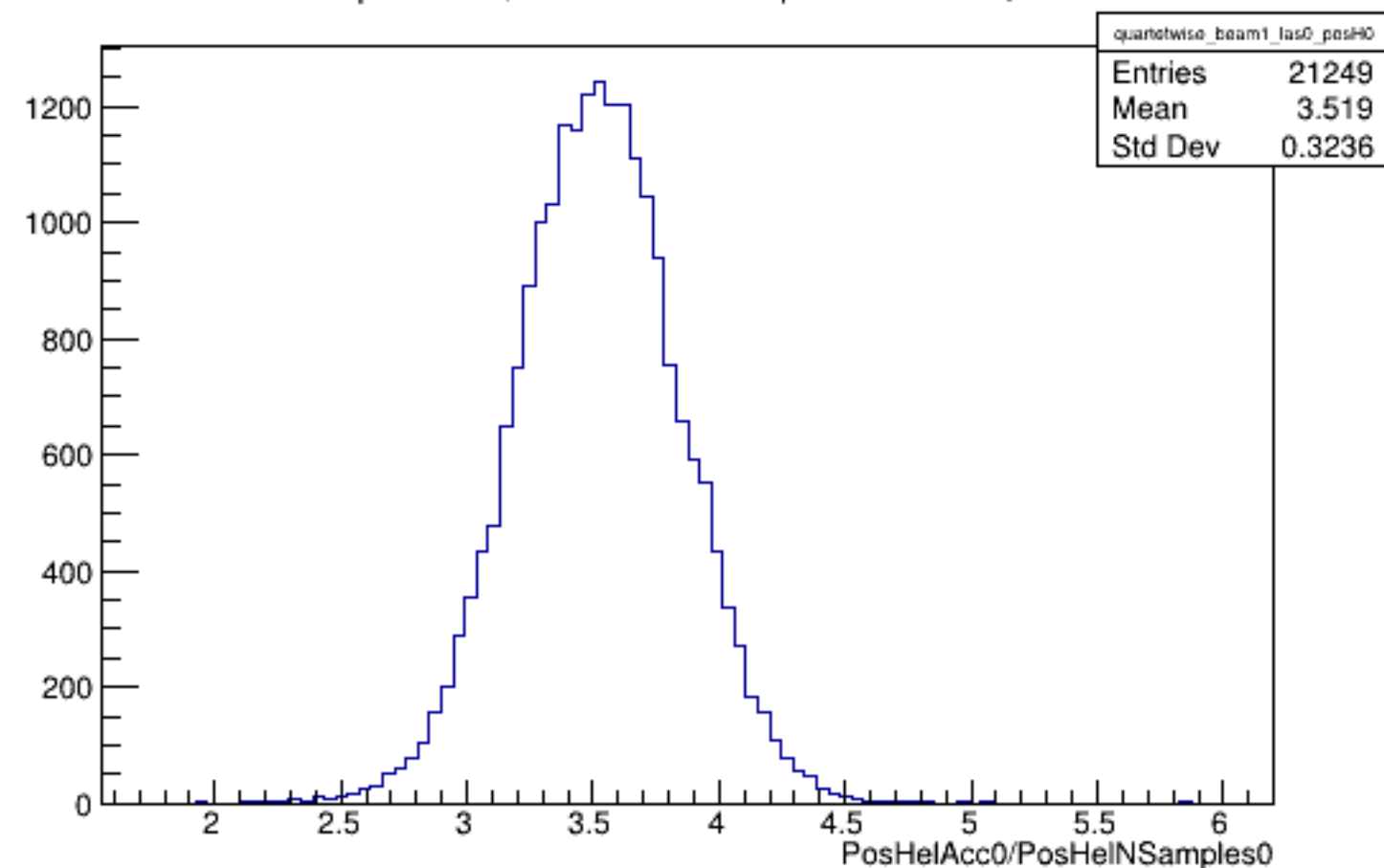
Run 5885 quartetwise, PosHelAcc0/NSamples0: Beam ON, Laser OFF
