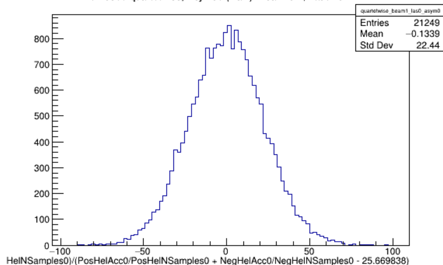
Run 5885 quartetwise, Asyms0 (Raw): Beam ON, Laser OFF
