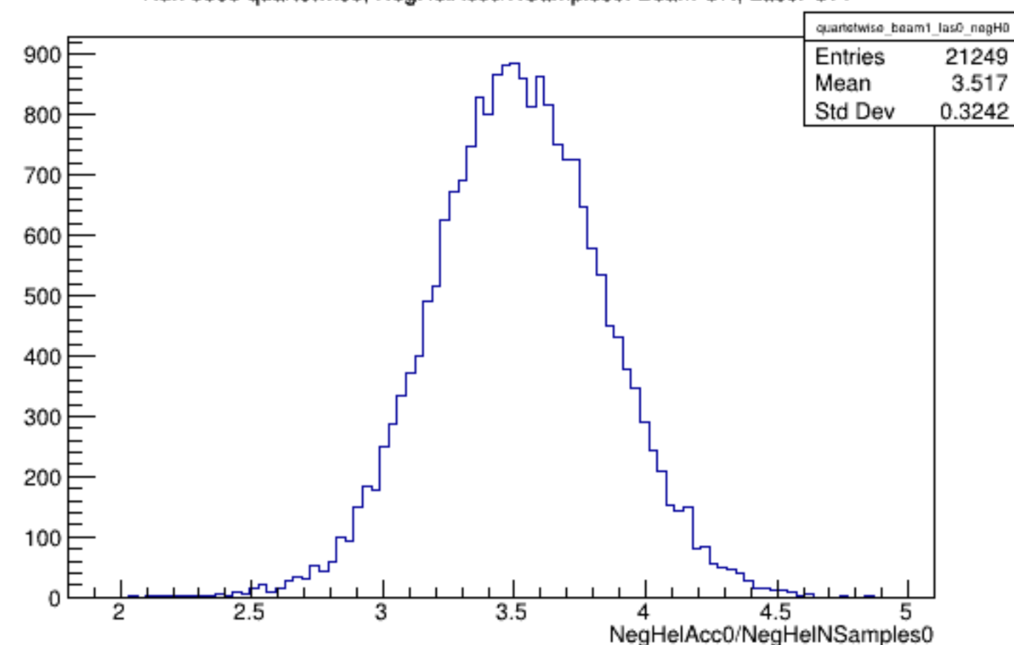
Run 5885 quartetwise, NegHelAcc0/NSamples0: Beam ON, Laser OFF
