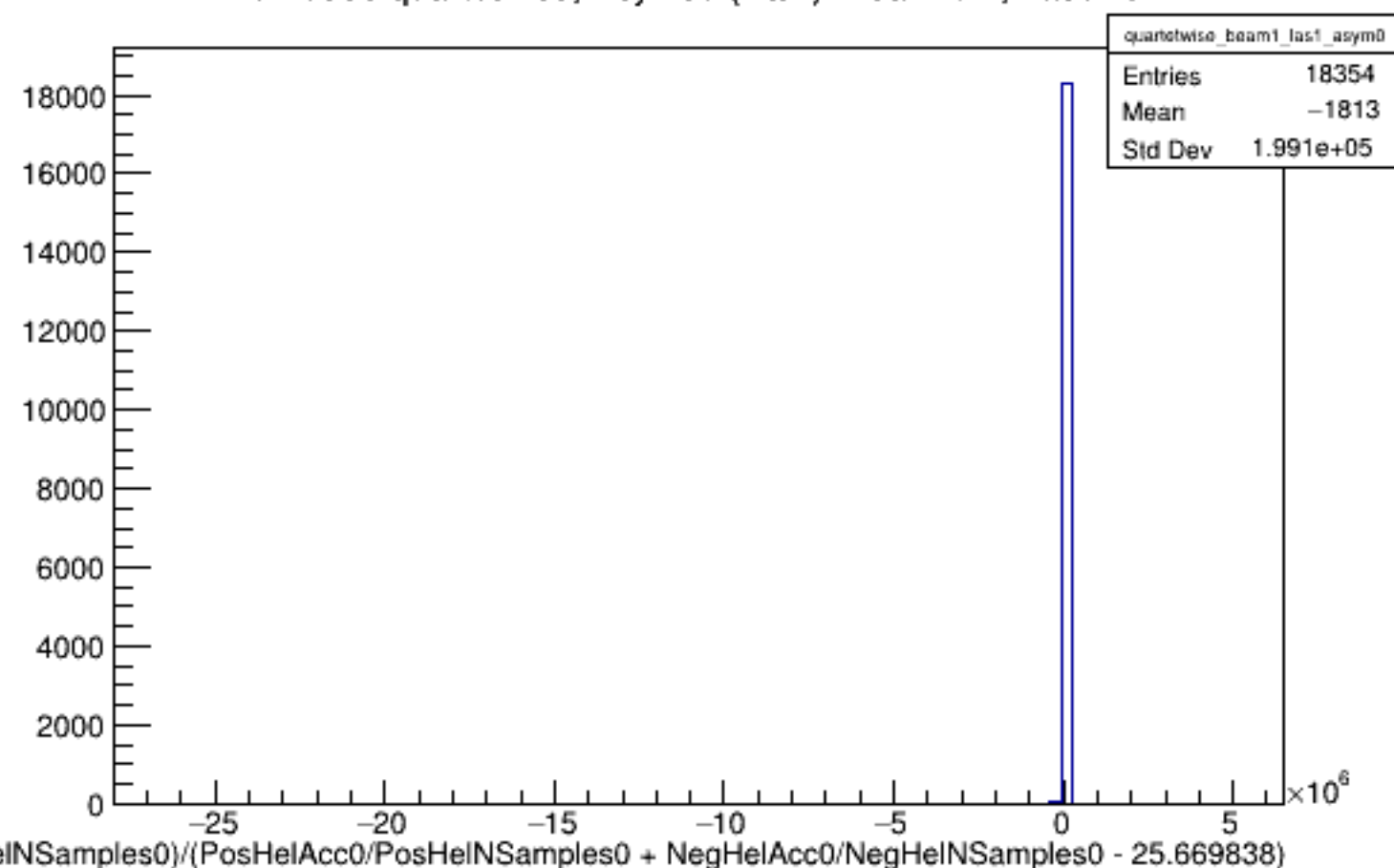
Run 5885 quartetwise, Asyms0 (Raw): Beam ON, Laser ON
