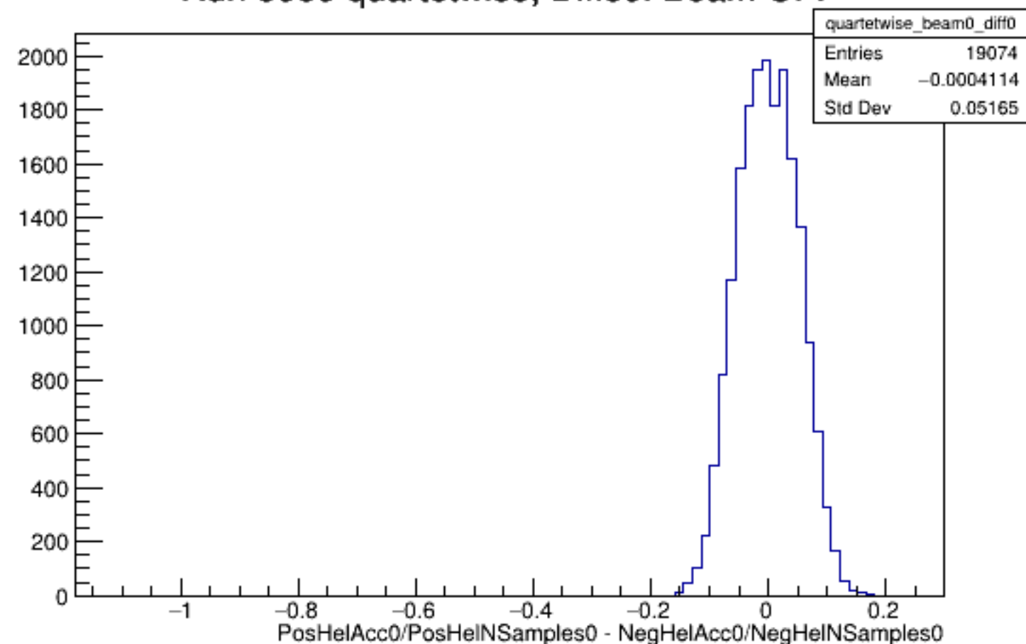
Run 5885 quartetwise, Diffs0: Beam OFF
