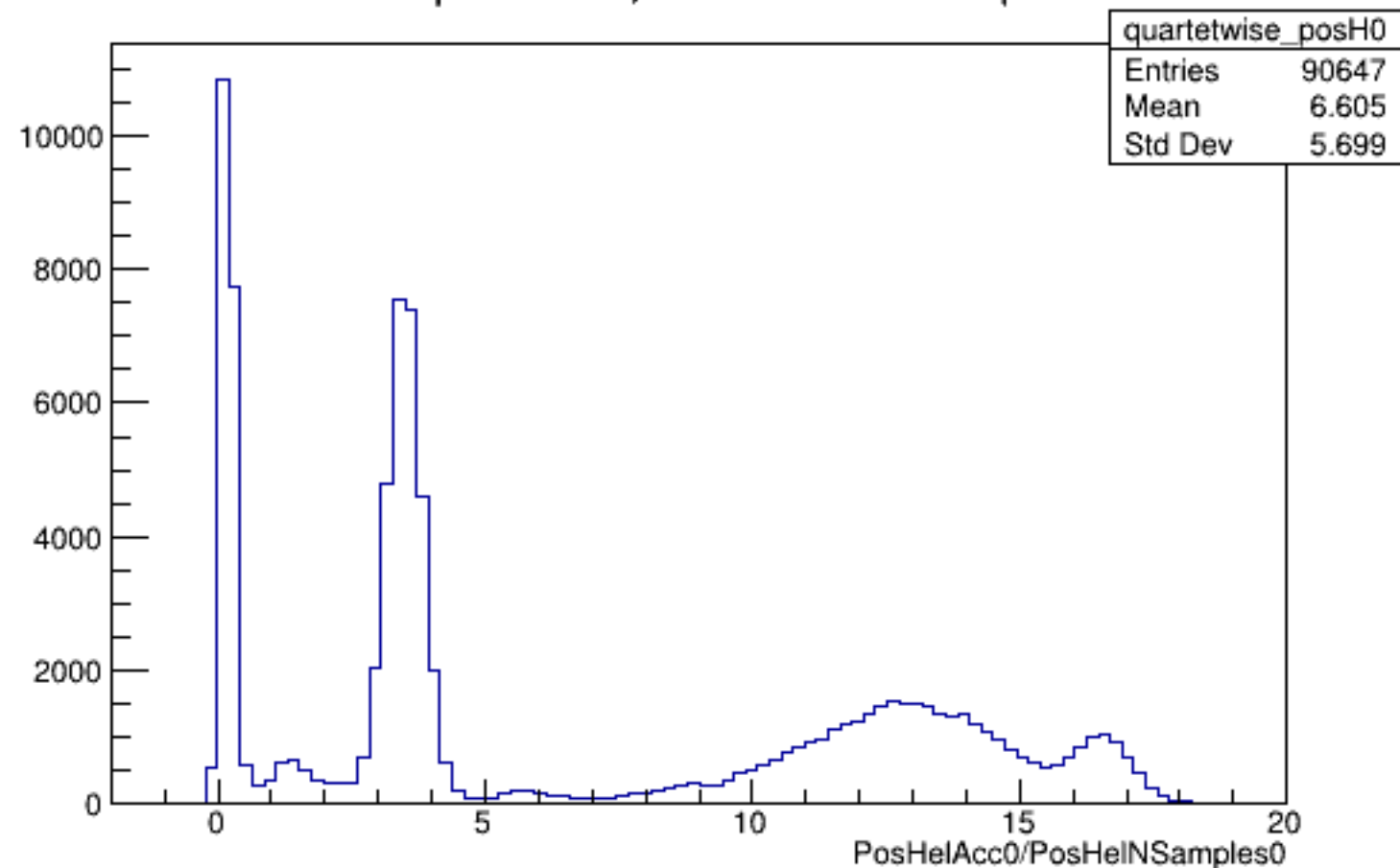
Run 5885 quartetwise, PosHelAcc0/NSamples0: All
