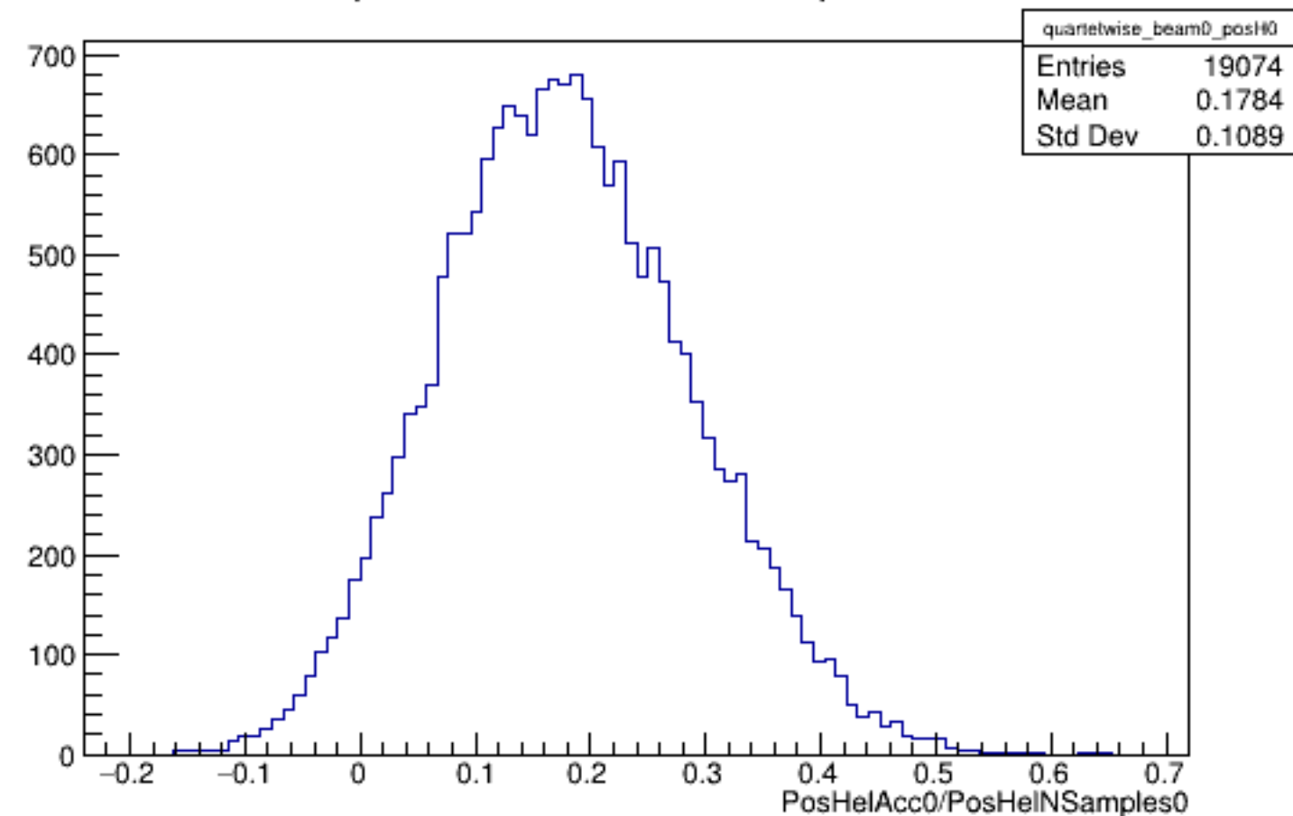
Run 5885 quartetwise, PosHelAcc0/NSamples0: Beam OFF
