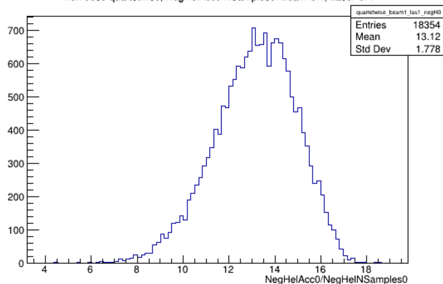
Run 5885 quartetwise, NegHelAcc0/NSamples0: Beam ON, Laser ON
