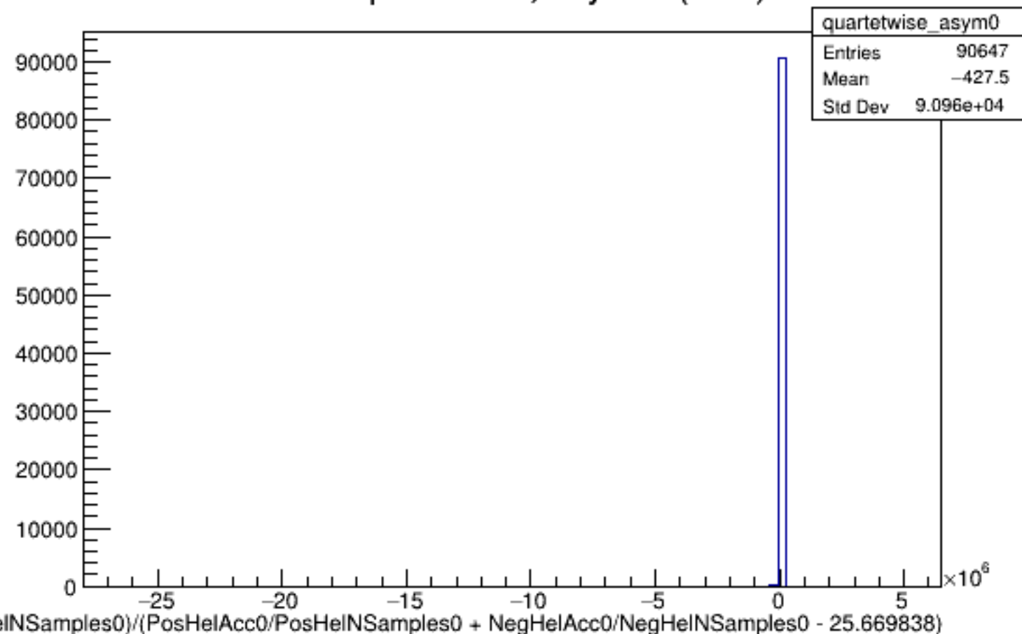
Run 5885 quartetwise, Asyms0 (Raw): All
