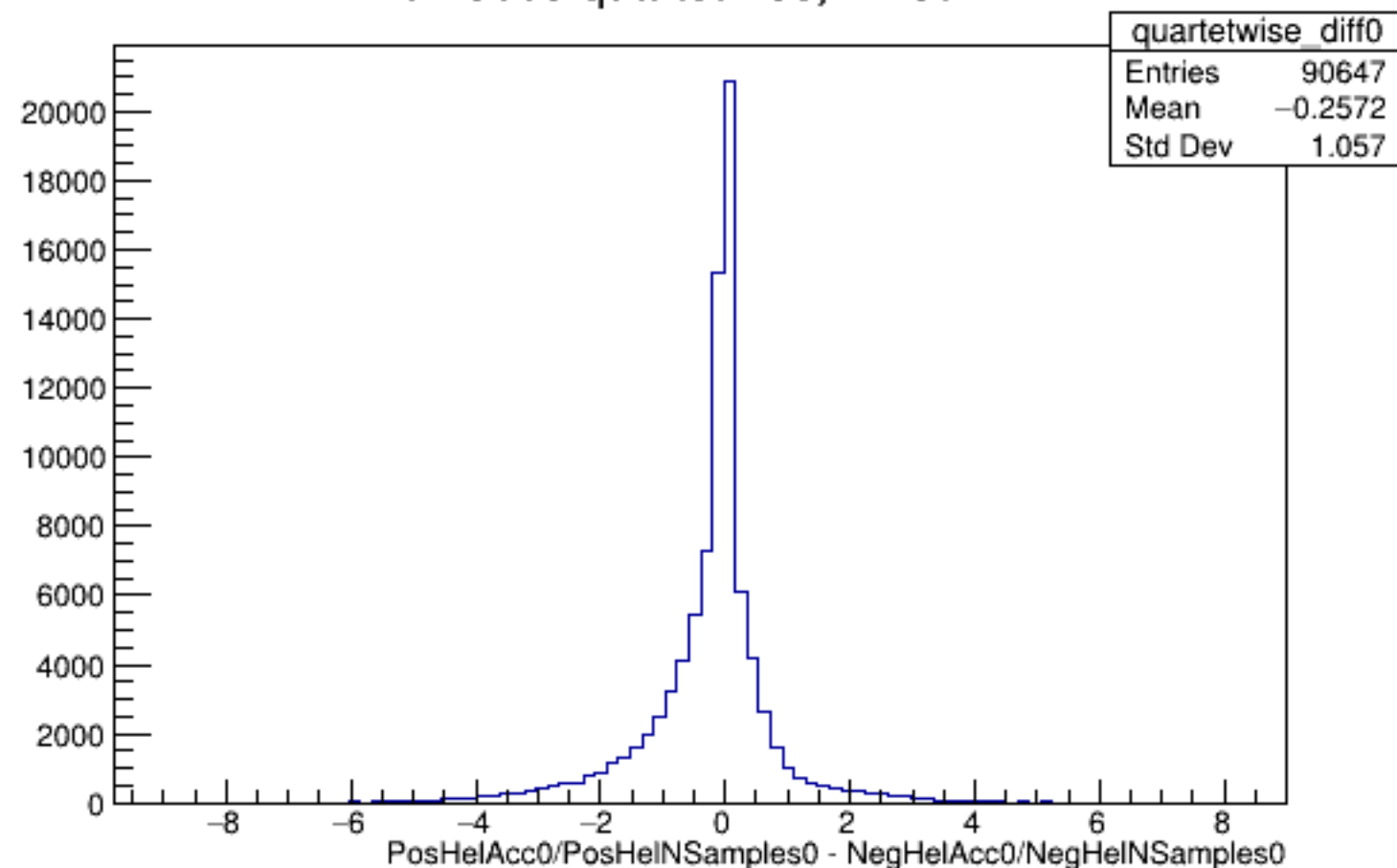
Run 5885 quartetwise, Diffs0: All
