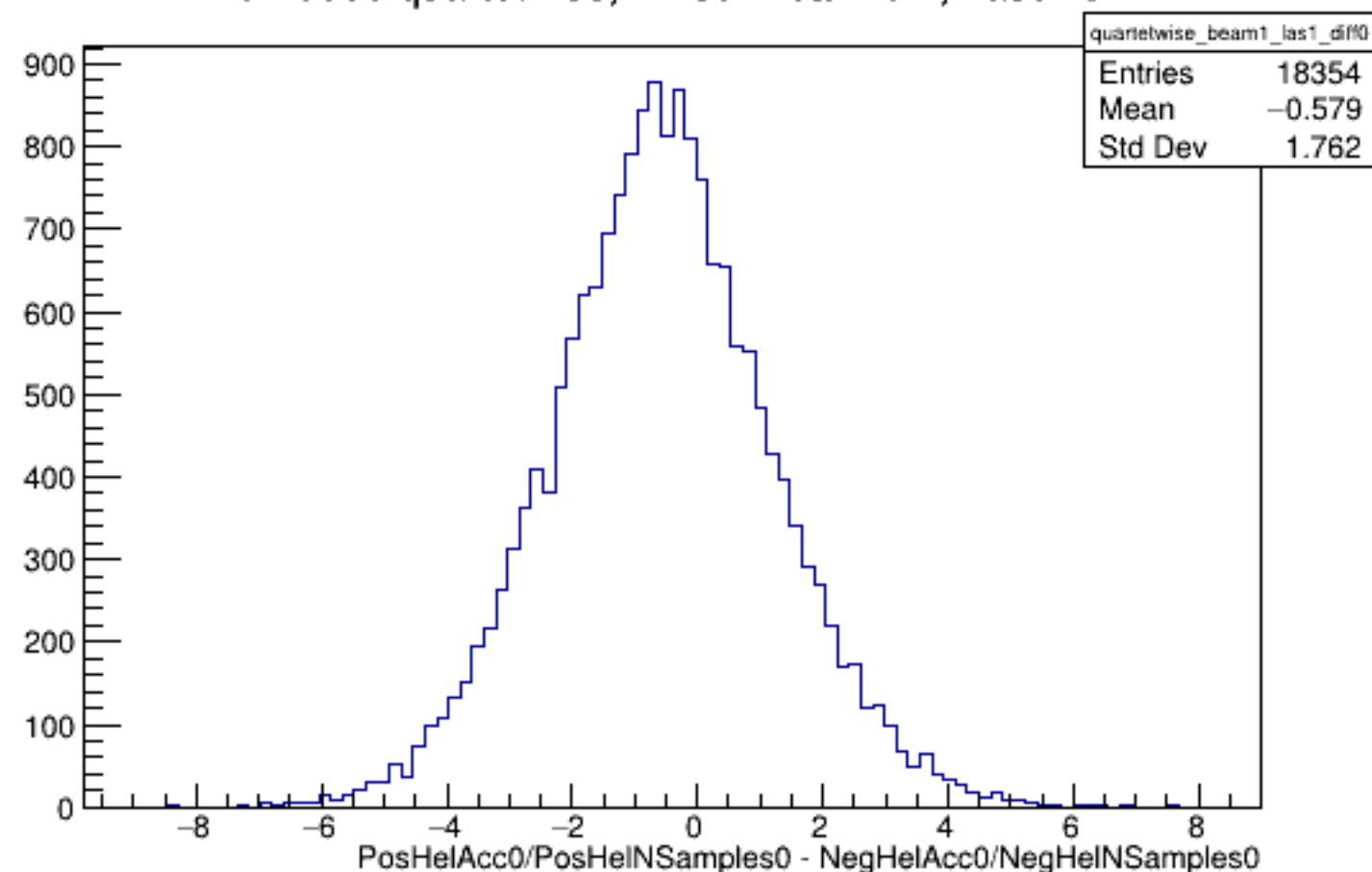
Run 5885 quartetwise, Diffs0: Beam ON, Laser ON
