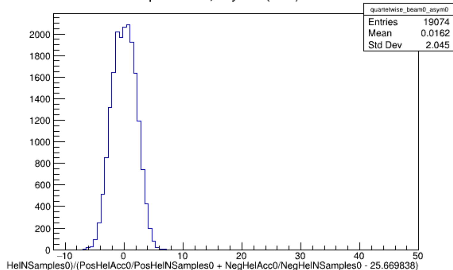
Run 5885 quartetwise, Asyms0 (Raw): Beam OFF
