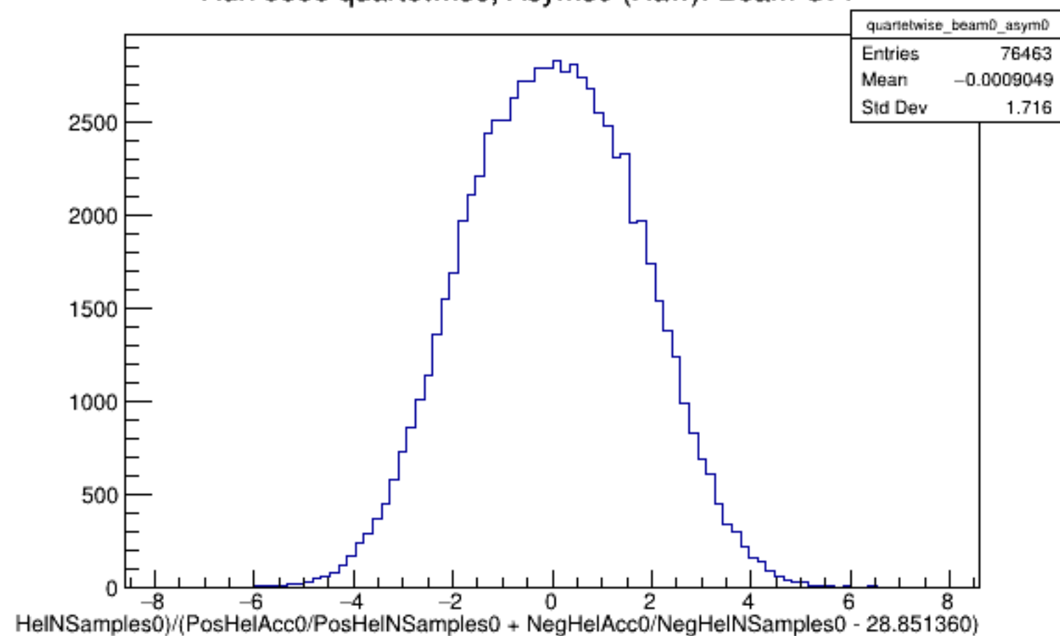
Run 5888 quartetwise, Asyms0 (Raw): Beam OFF
