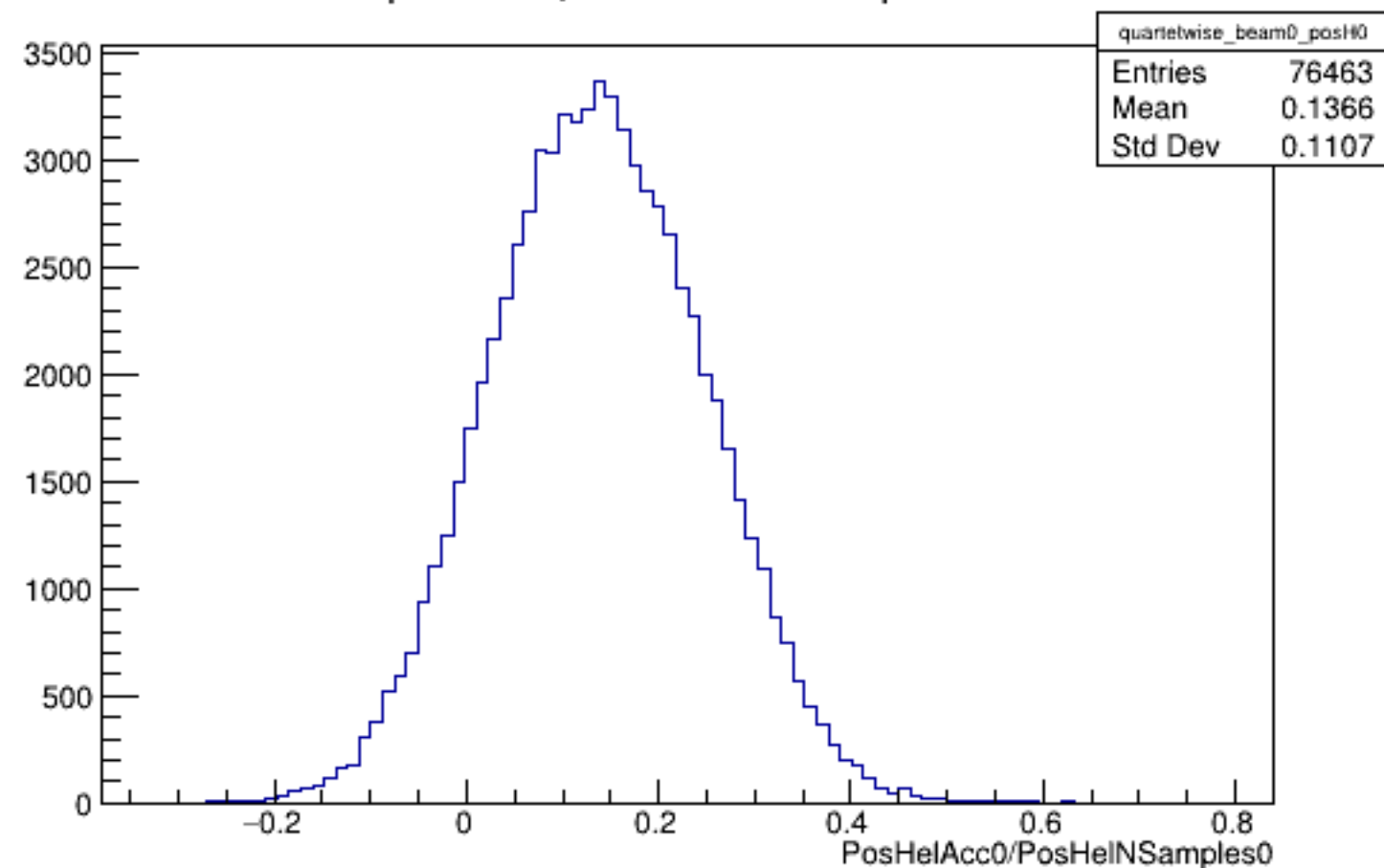
Run 5888 quartetwise, PosHelAcc0/NSamples0: Beam OFF
