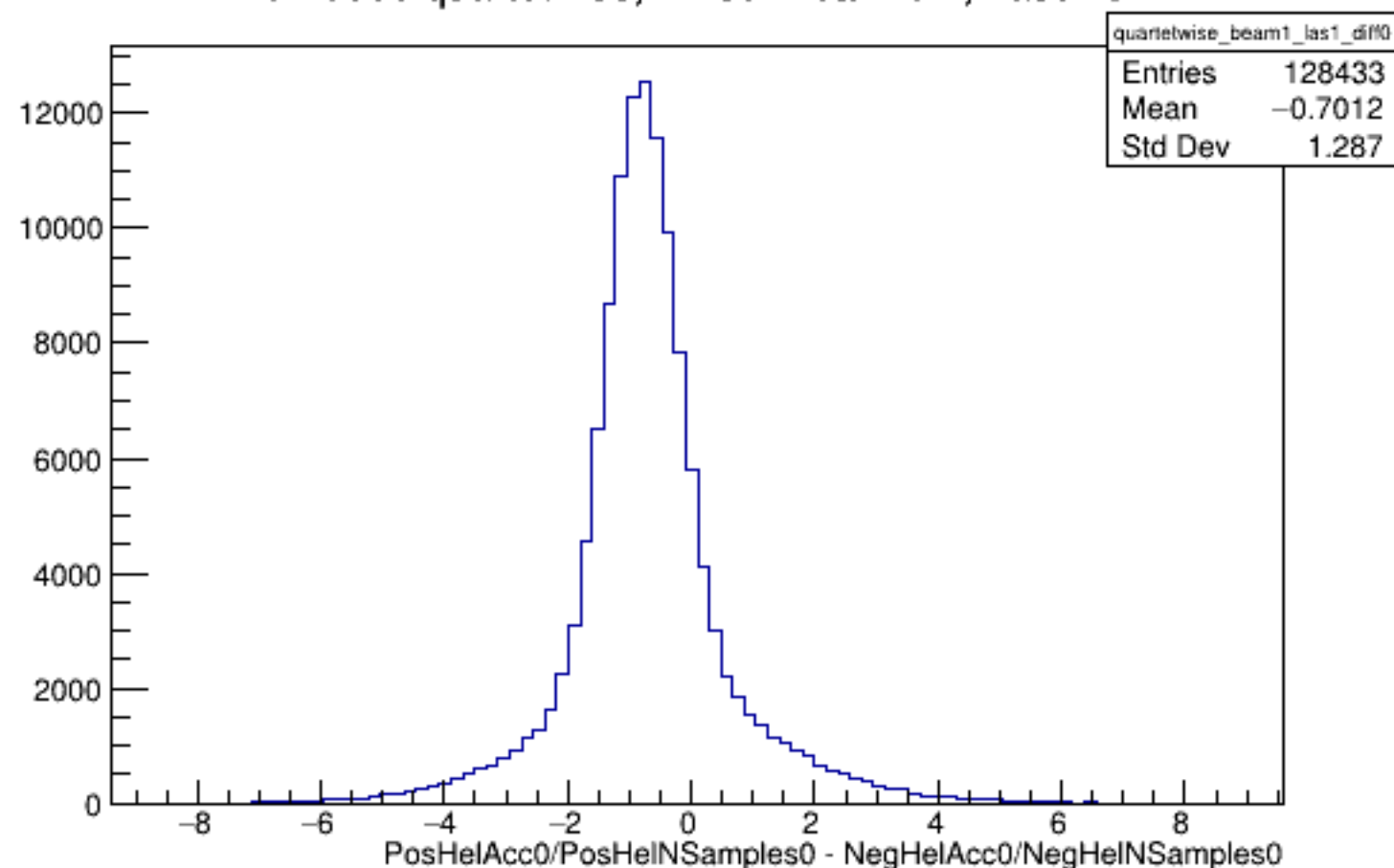
Run 5888 quartetwise, Diffs0: Beam ON, Laser ON
