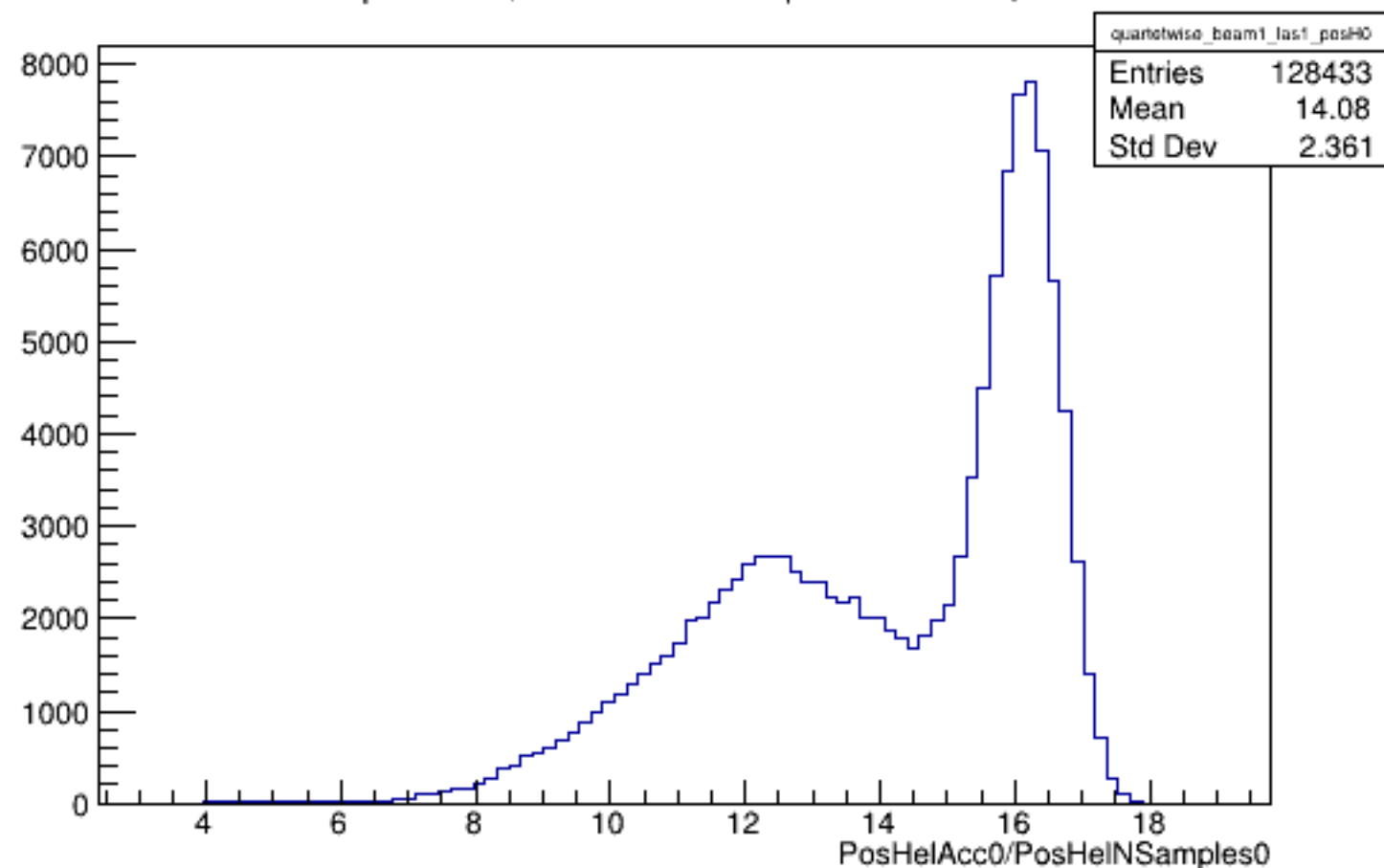
Run 5888 quartetwise, PosHelAcc0/NSamples0: Beam ON, Laser ON
