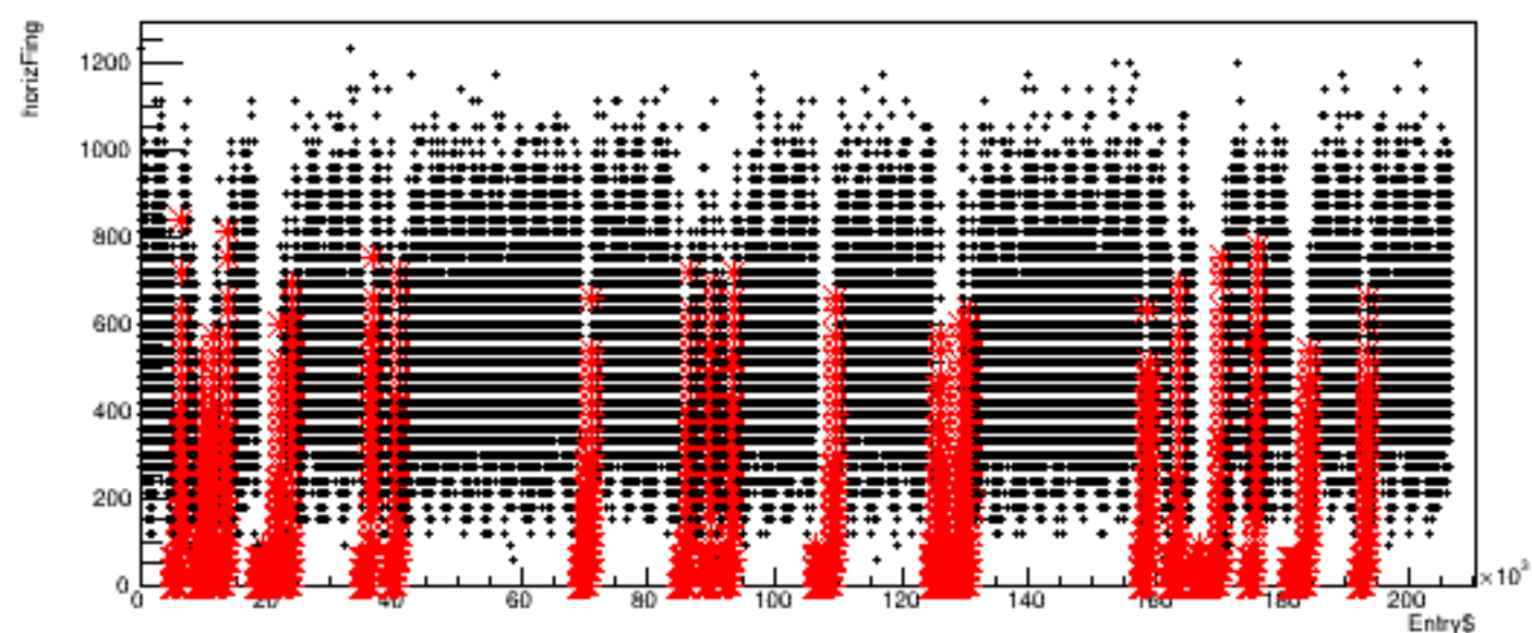
Run 5889, quartetwise: horizFing vs time
