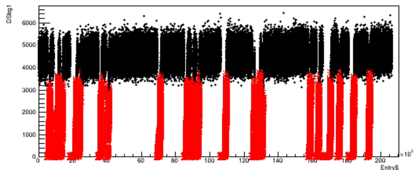
Run 5889, quartetwise: DSbg1 vs time
