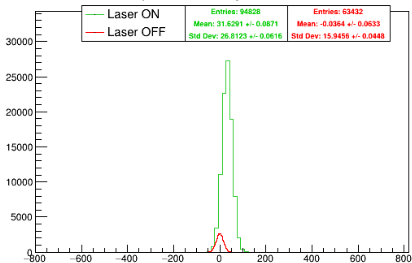
Run 5891 quartetwise, asym0sub: Beam ON
