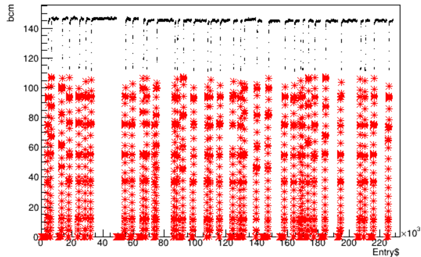
Run 5891 quartetwise, bcm vs time
