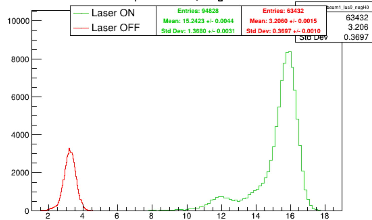
Run 5891 quartetwise, negH0: Beam ON
