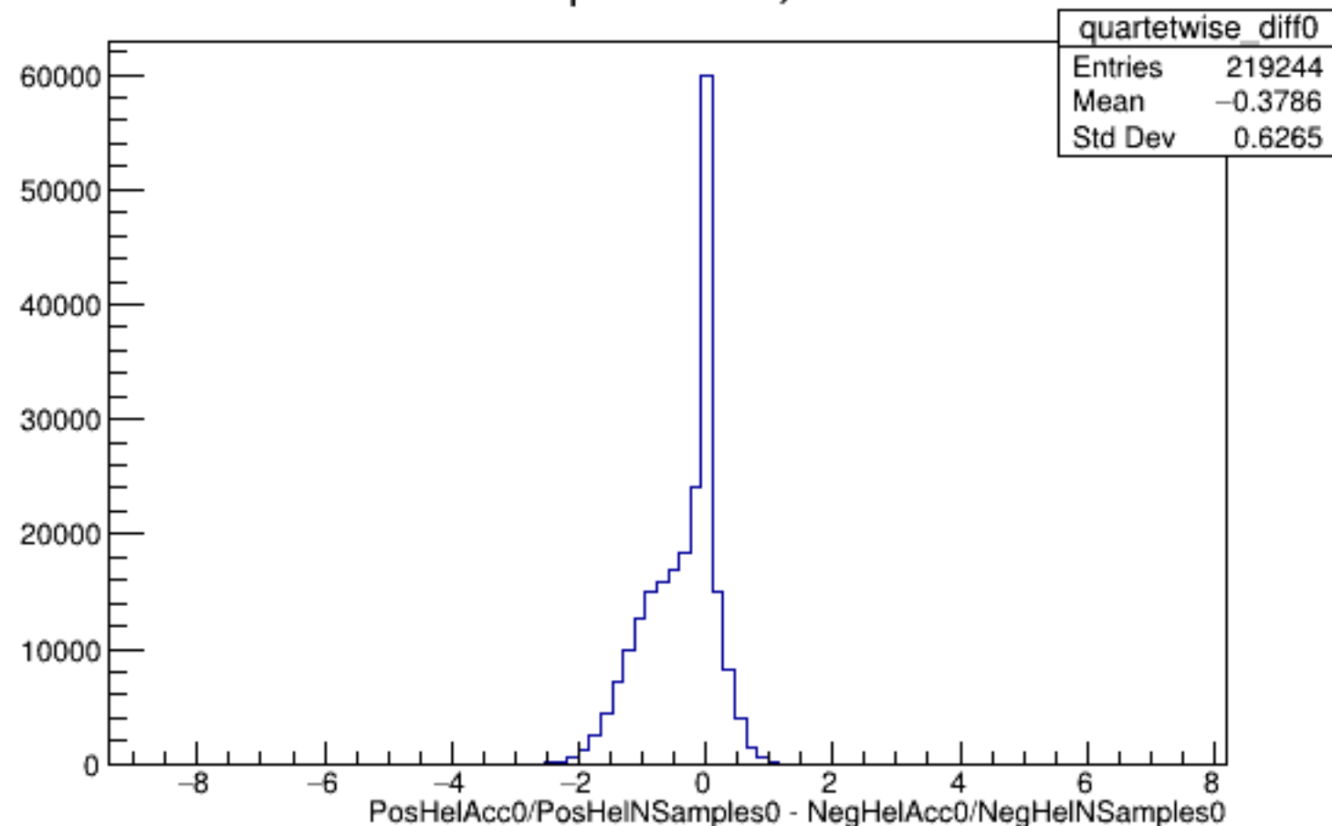
Run 5898 quartetwise, Diffs0: All
