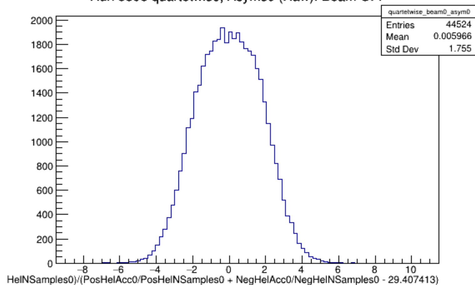
Run 5898 quartetwise, Asyms0 (Raw): Beam OFF
