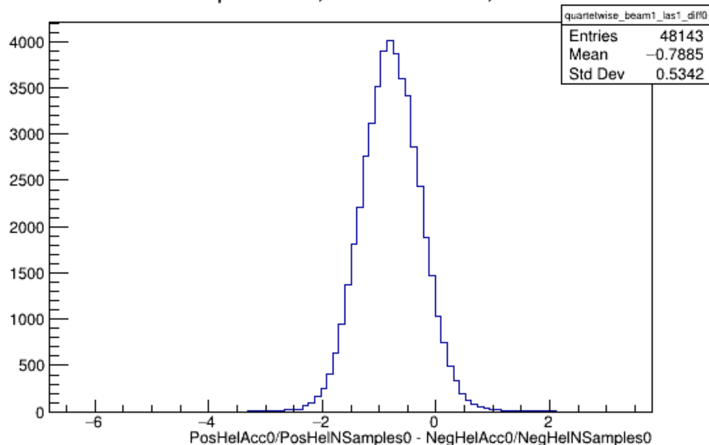
Run 5898 quartetwise, Diffs0: Beam ON, Laser ON
