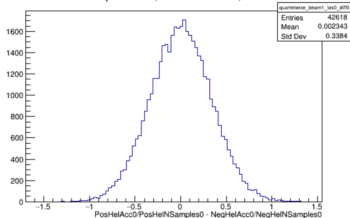
Run 5898 quartetwise, Diffs0: Beam ON, Laser OFF
