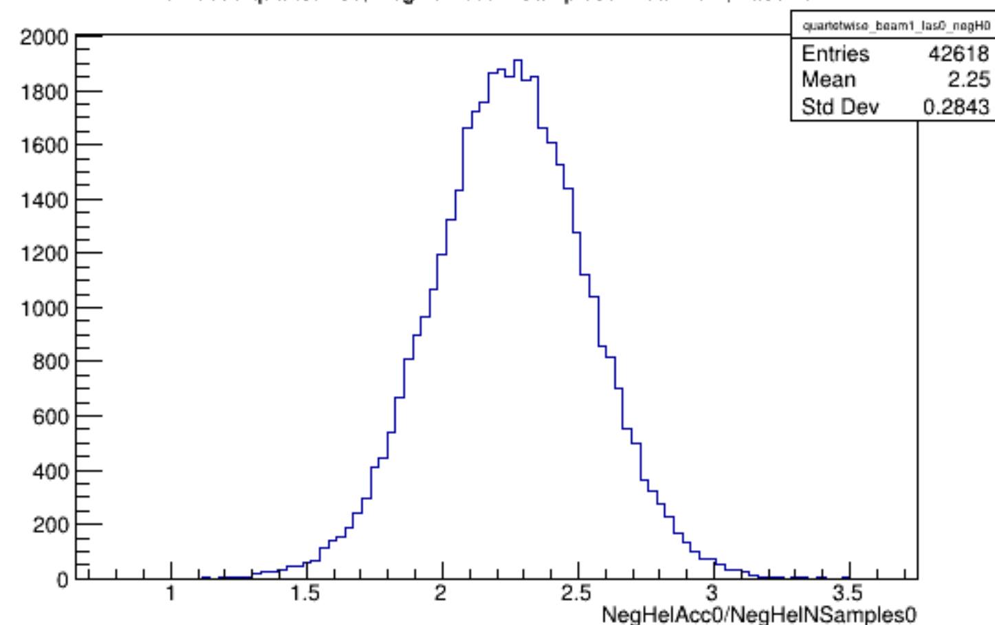
Run 5898 quartetwise, NegHelAcc0/NSamples0: Beam ON, Laser OFF
