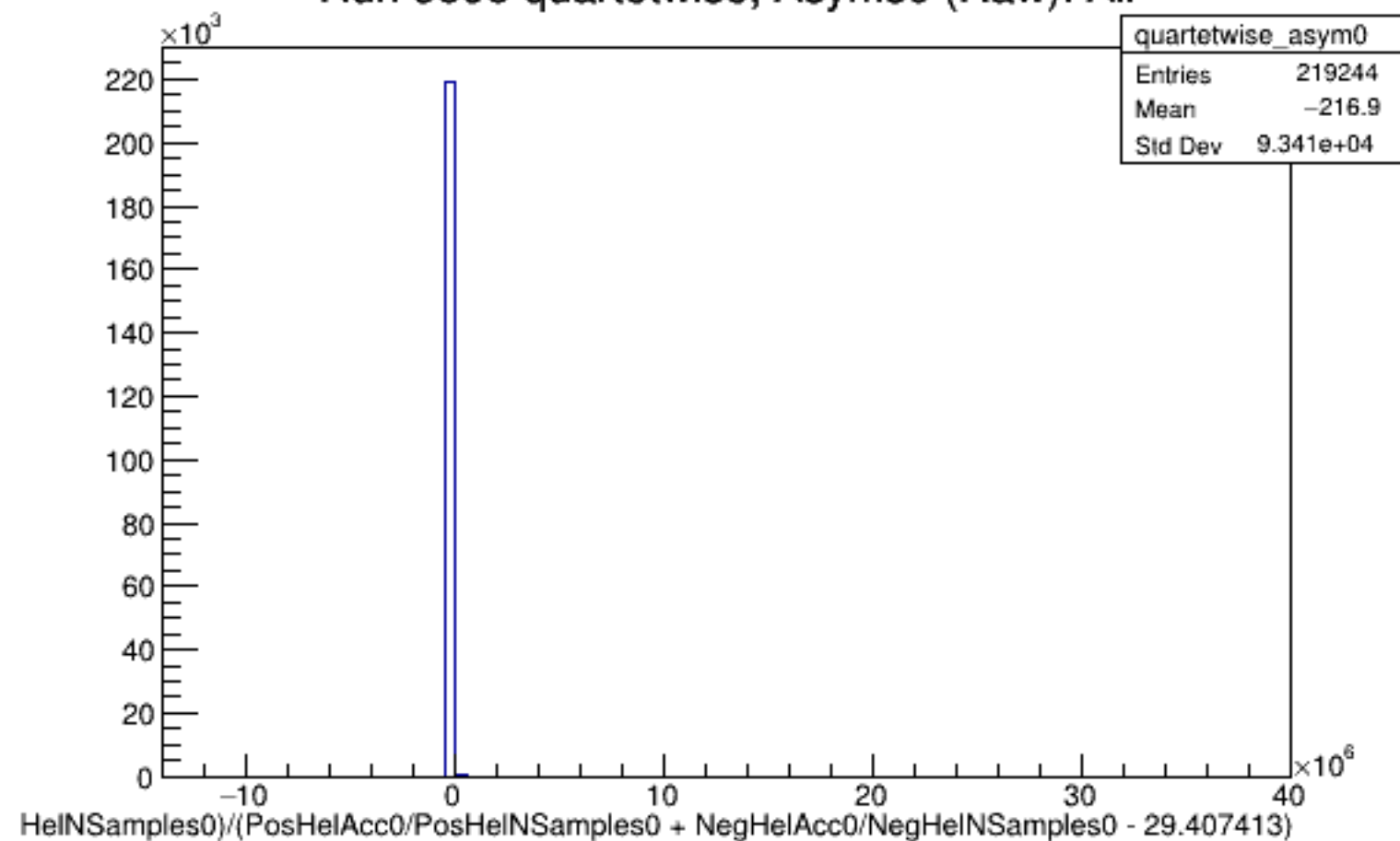
Run 5898 quartetwise, Asyms0 (Raw): All
