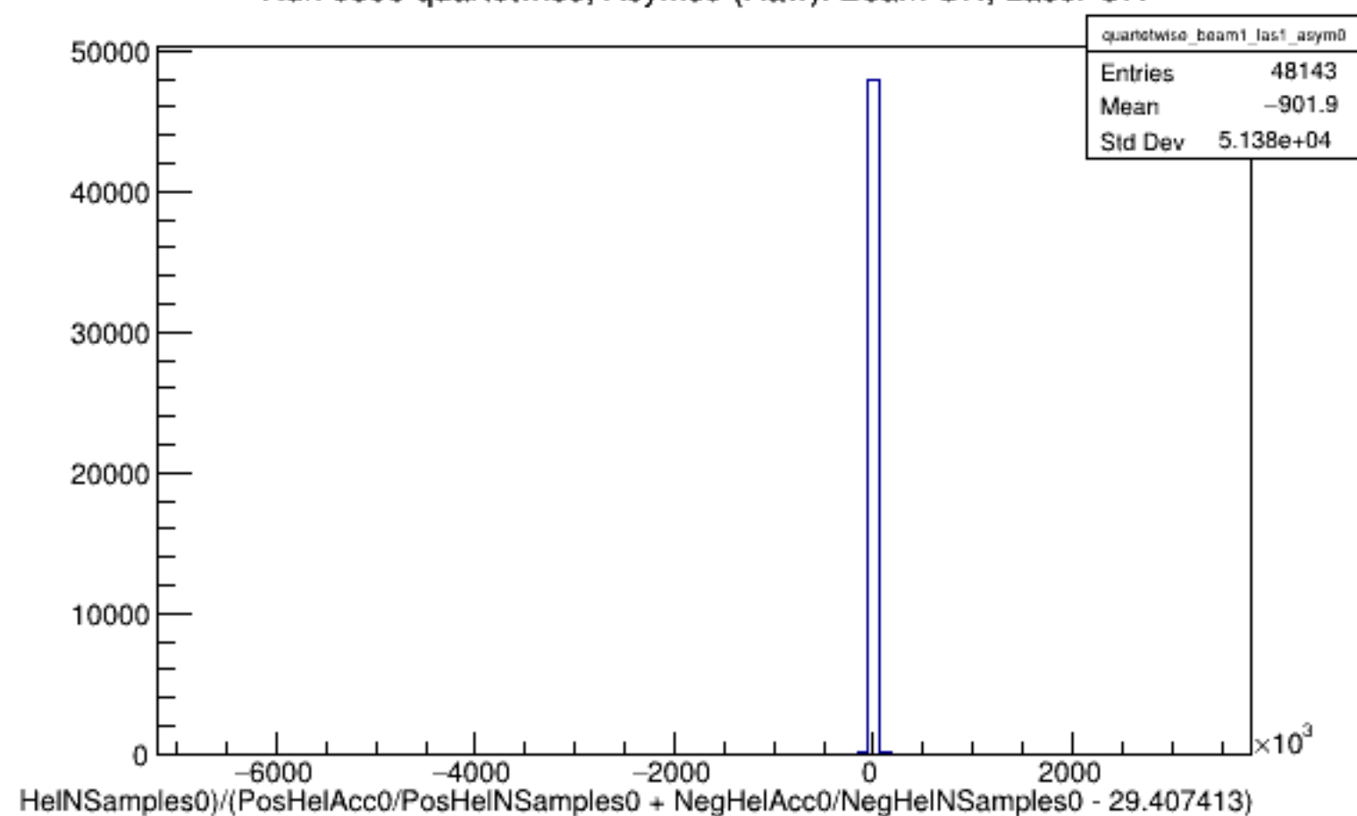
Run 5898 quartetwise, Asyms0 (Raw): Beam ON, Laser ON
