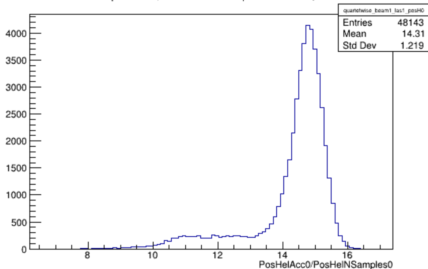
Run 5898 quartetwise, PosHelAcc0/NSamples0: Beam ON, Laser ON
