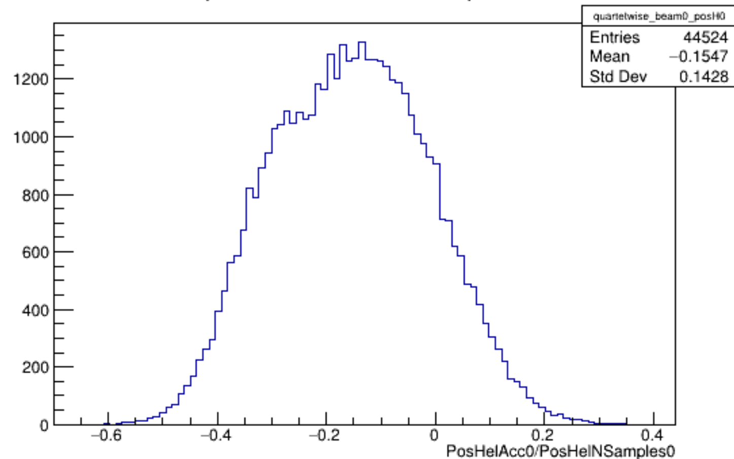
Run 5898 quartetwise, PosHelAcc0/NSamples0: Beam OFF
