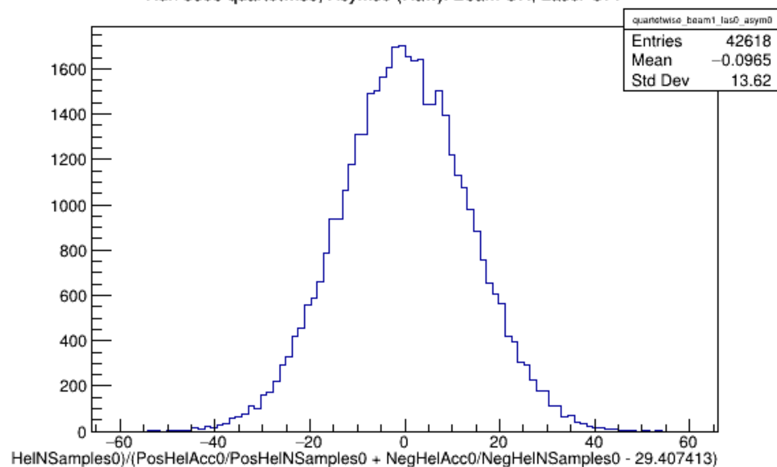
Run 5898 quartetwise, Asyms0 (Raw): Beam ON, Laser OFF
