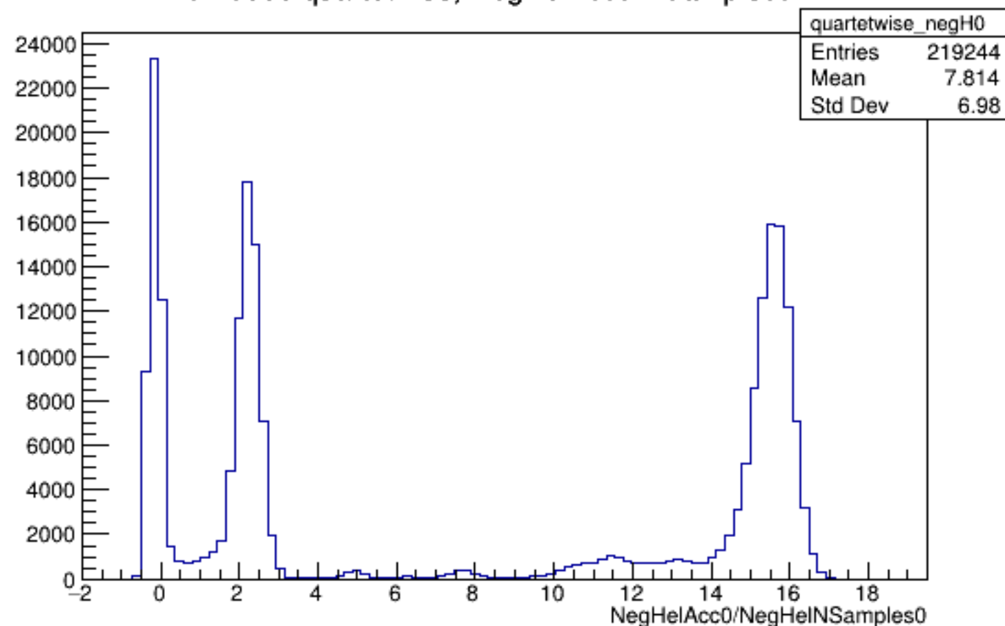
Run 5898 quartetwise, NegHelAcc0/NSamples0: All
