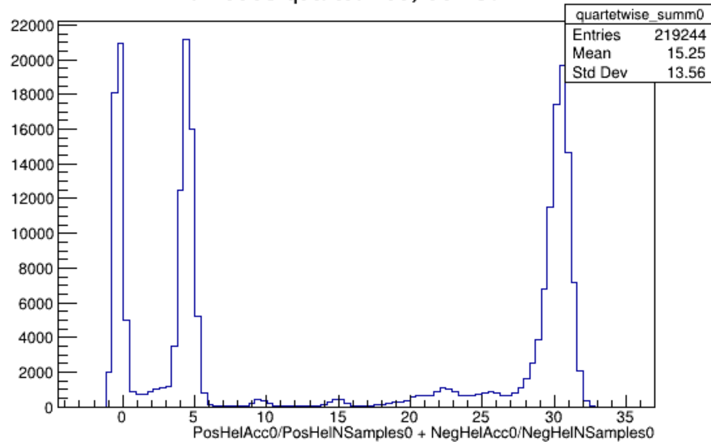
Run 5898 quartetwise, Sums0: All
