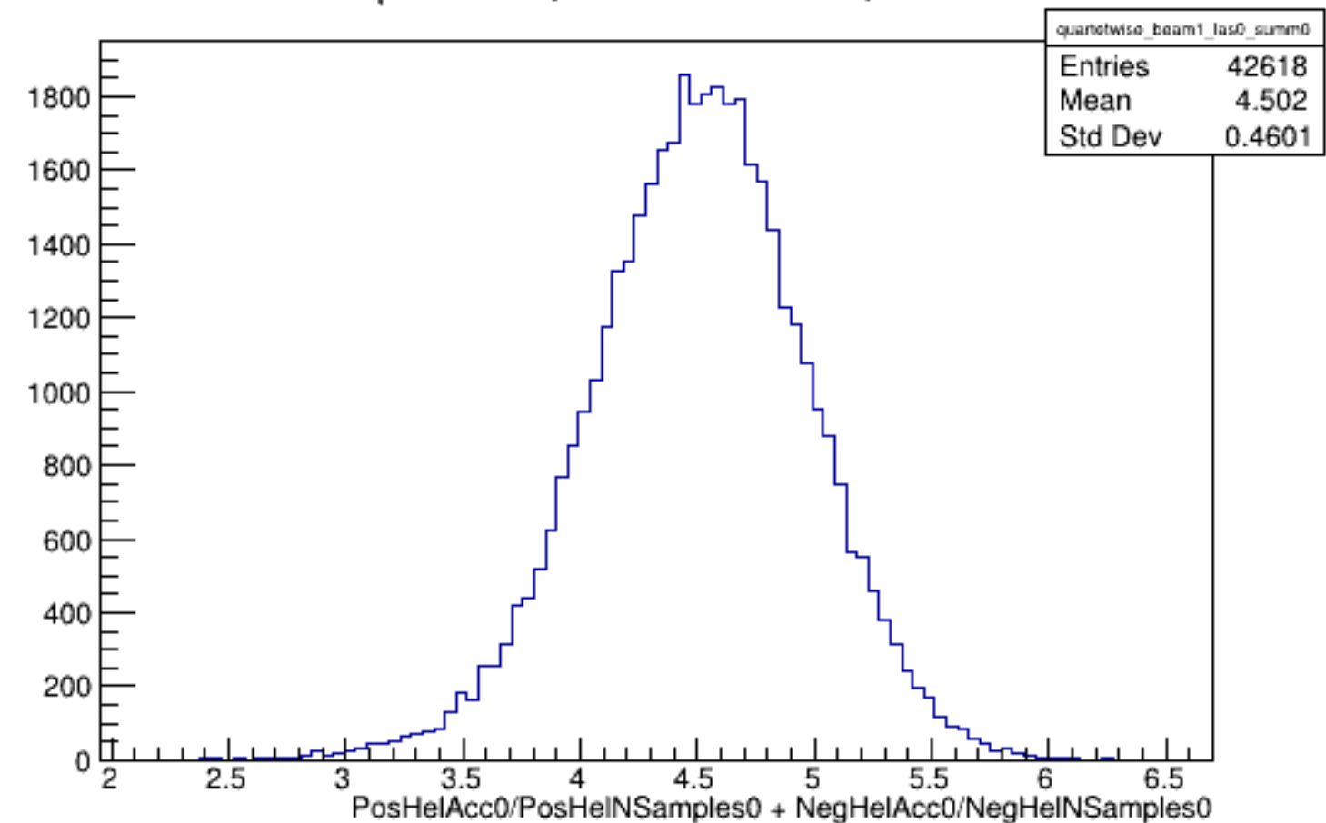
Run 5898 quartetwise, Sums0: Beam ON, Laser OFF
