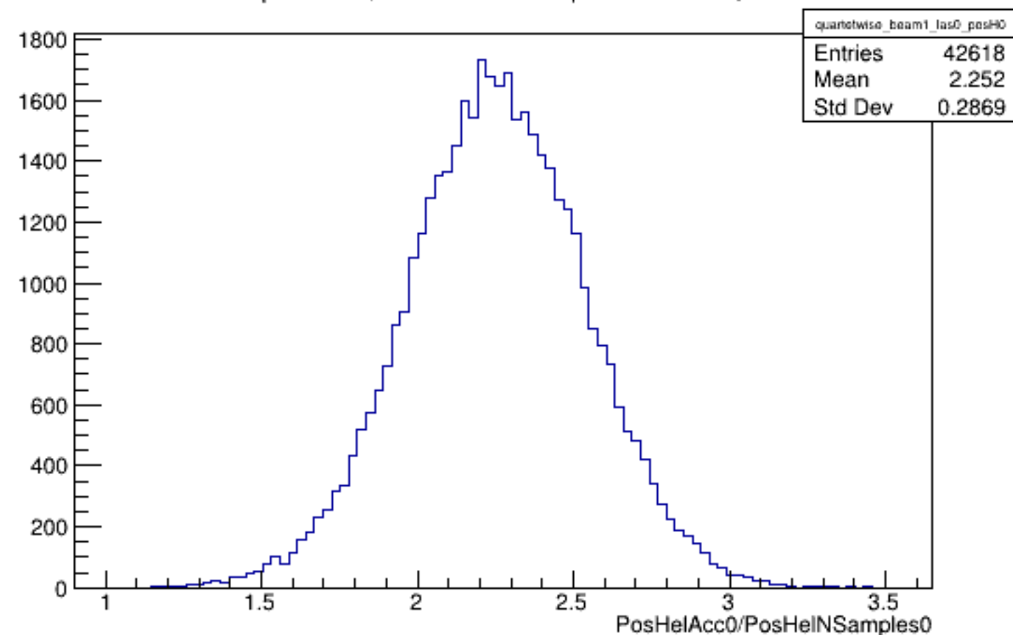
Run 5898 quartetwise, PosHelAcc0/NSamples0: Beam ON, Laser OFF
