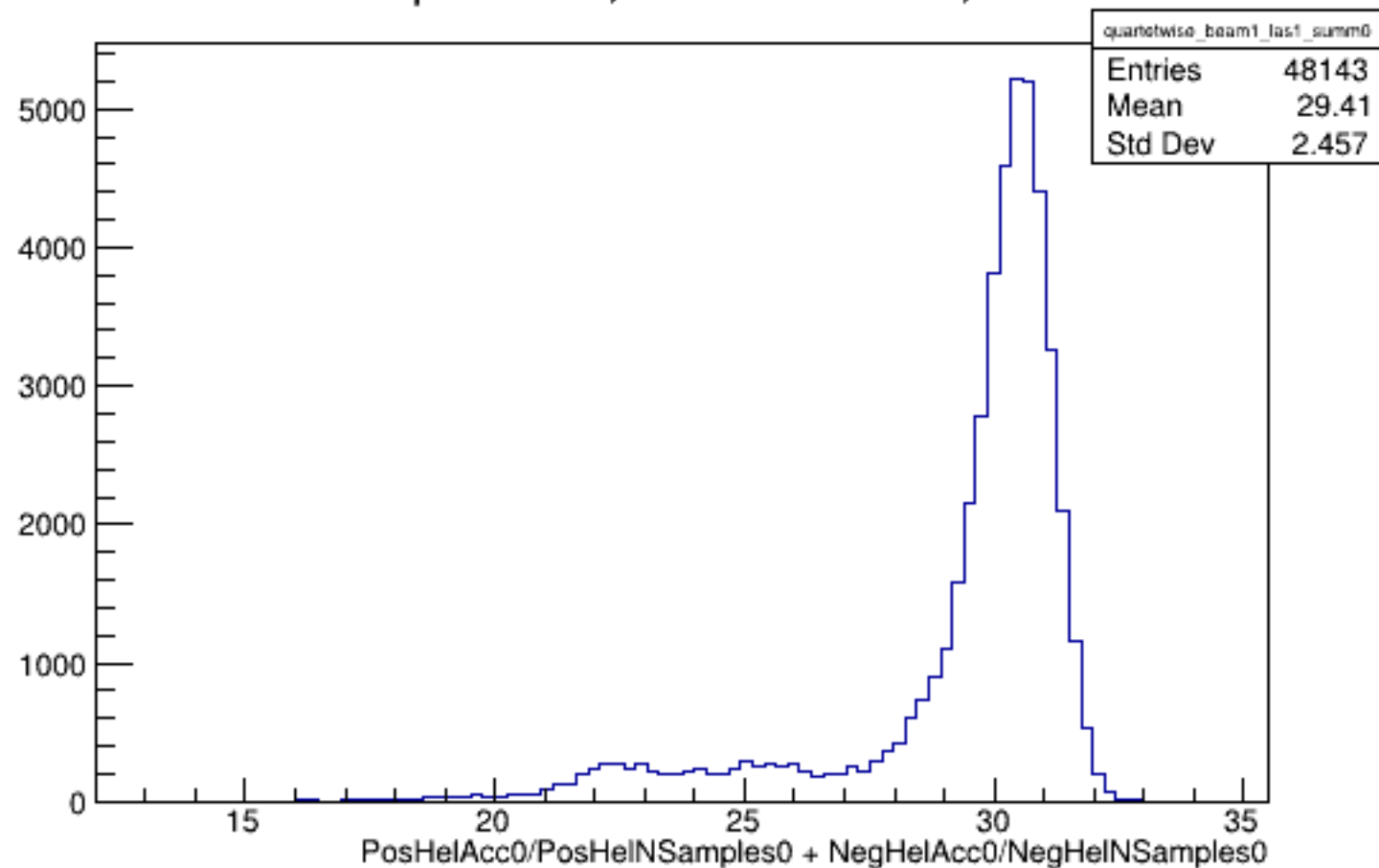
Run 5898 quartetwise, Sums0: Beam ON, Laser ON
