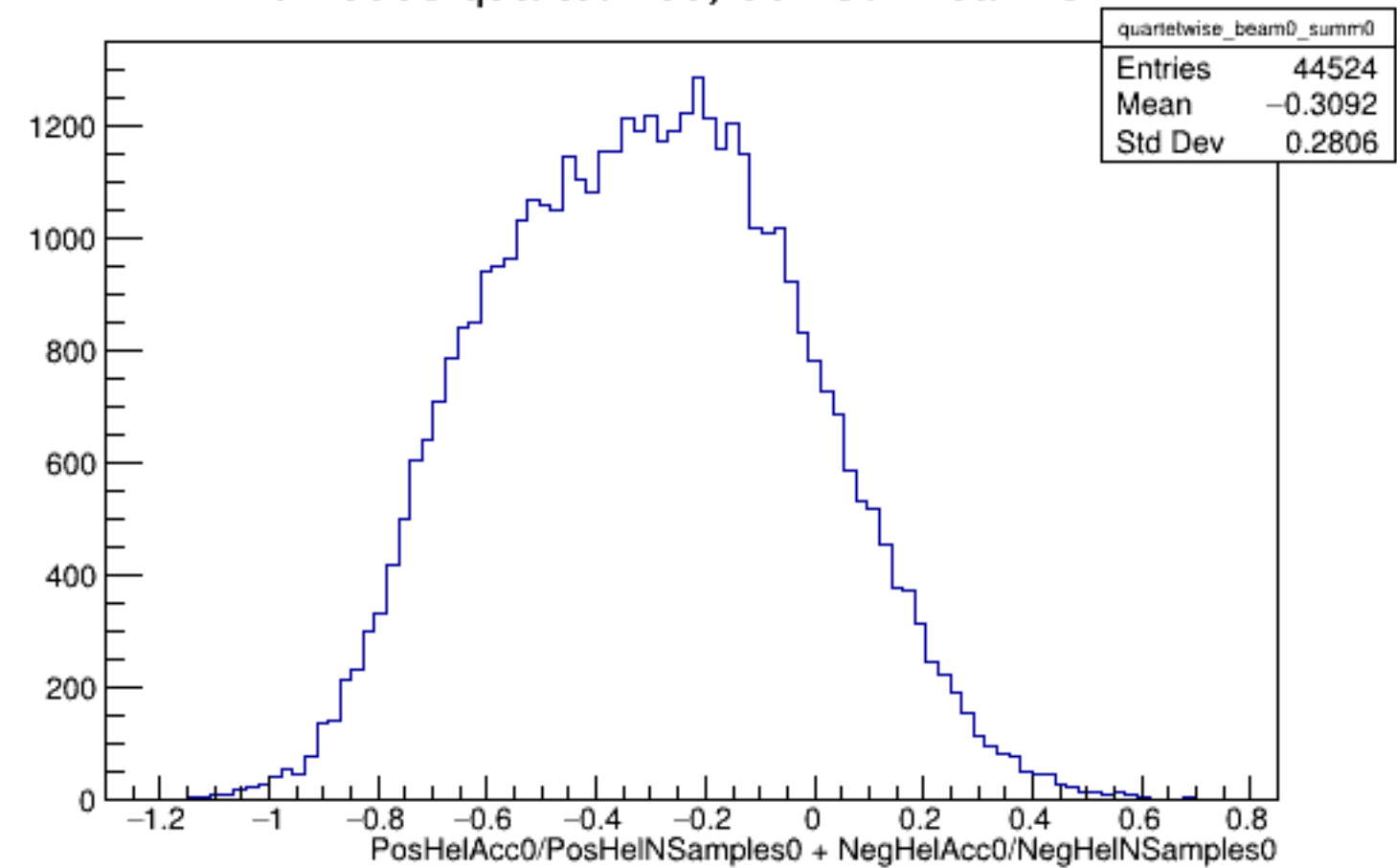
Run 5898 quartetwise, Sums0: Beam OFF
