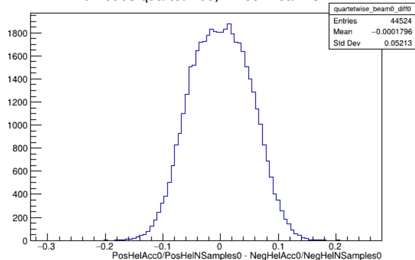
Run 5898 quartetwise, Diffs0: Beam OFF
