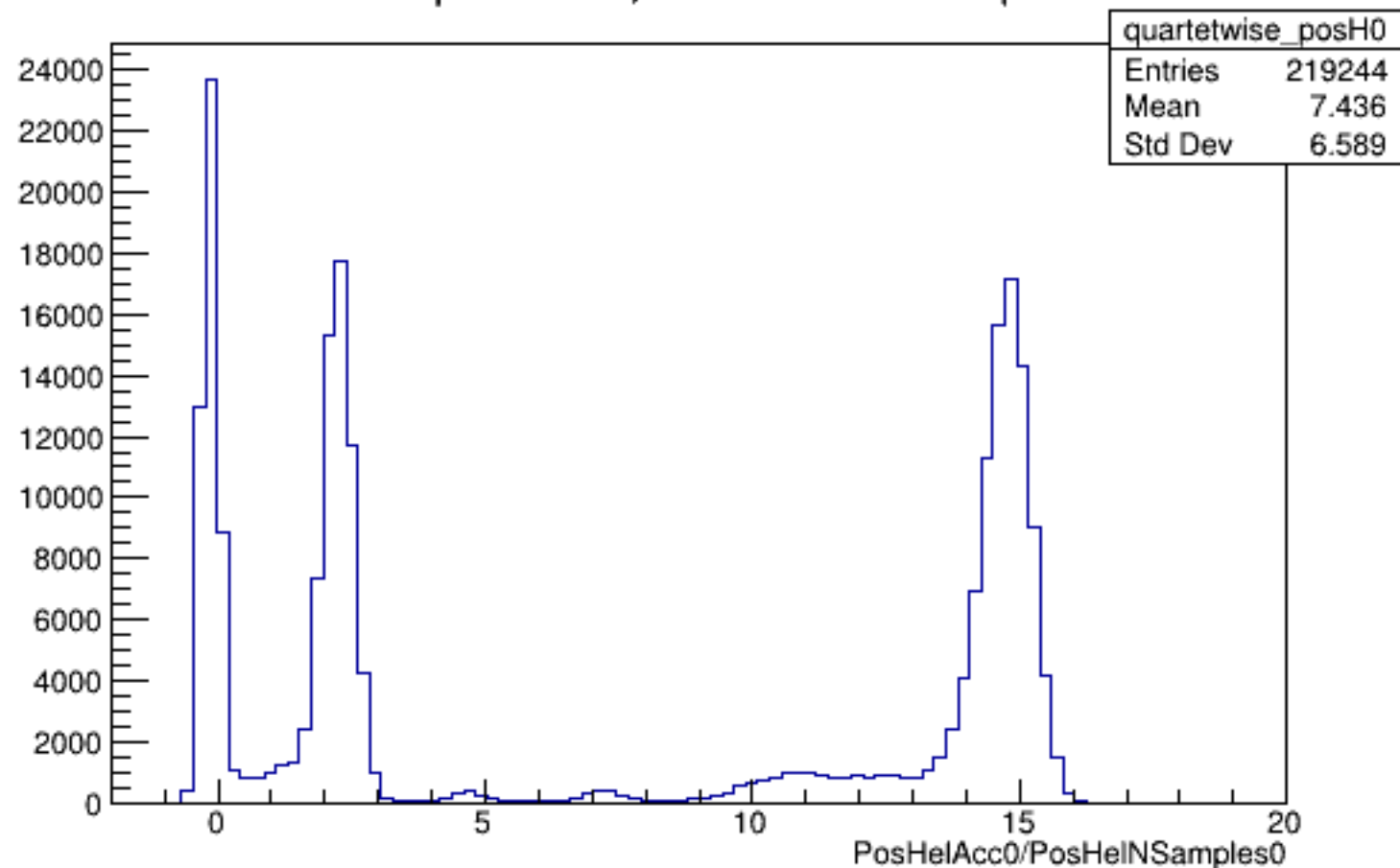
Run 5898 quartetwise, PosHelAcc0/NSamples0: All
