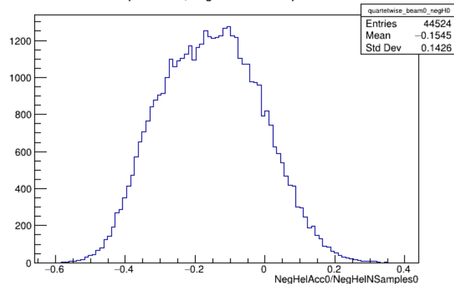
Run 5898 quartetwise, NegHelAcc0/NSamples0: Beam OFF
