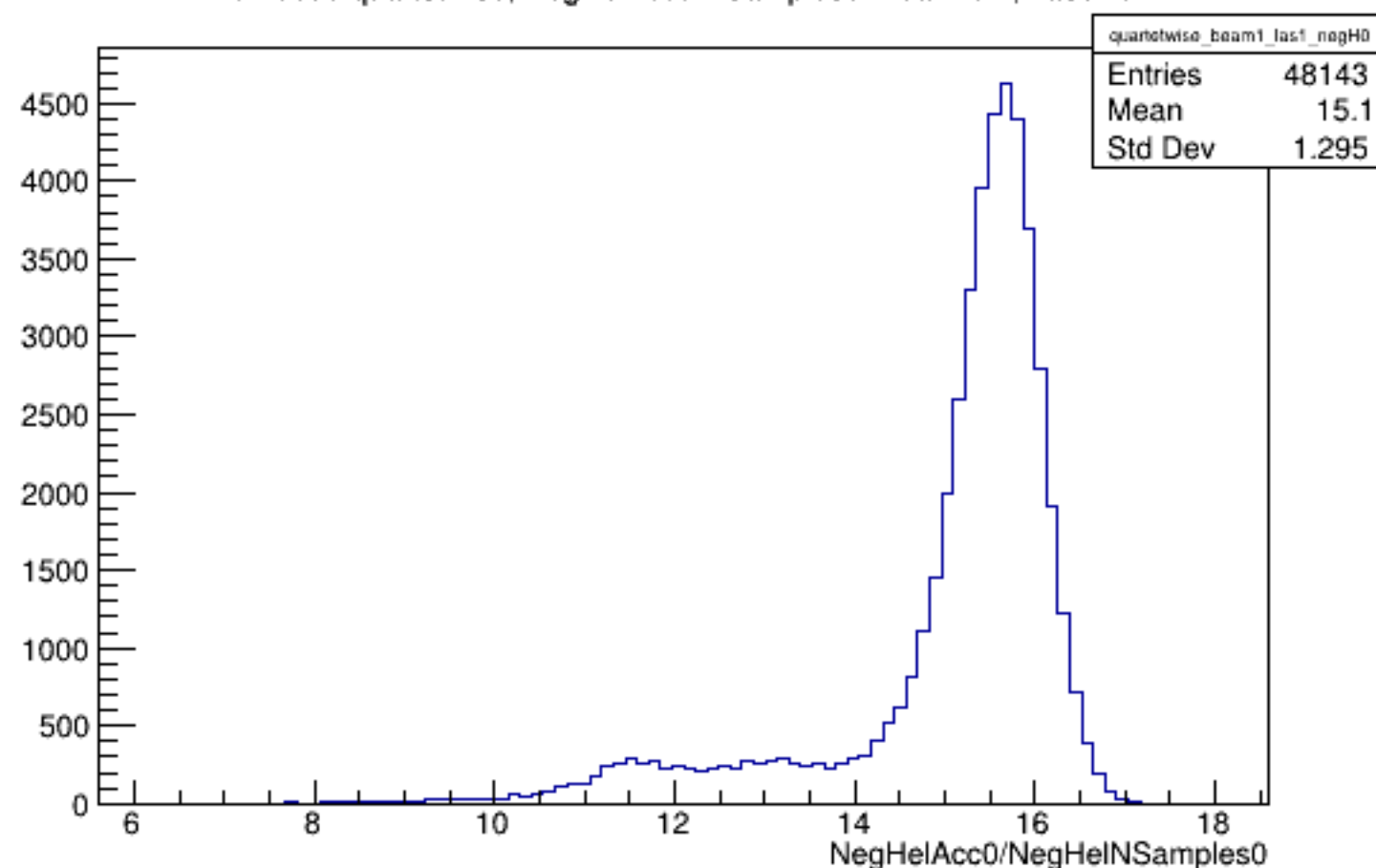
Run 5898 quartetwise, NegHelAcc0/NSamples0: Beam ON, Laser ON
