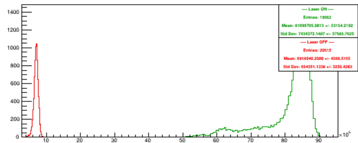
Run 5900 quartetwise, Sums4
