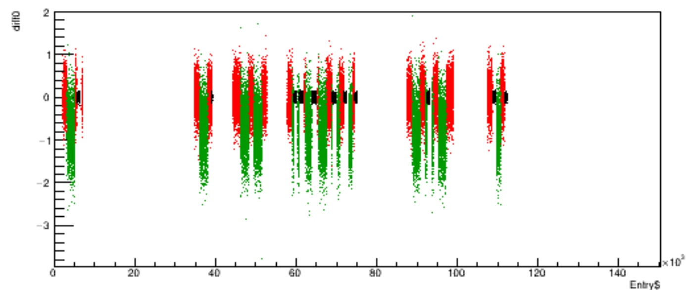
Run 5900 quartetwise, diff0 vs time
