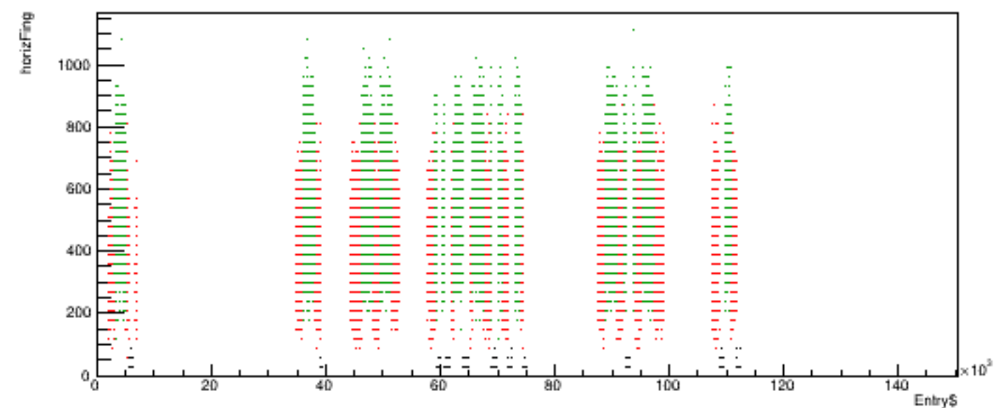
Run 5900 quartetwise, horizFing vs time
