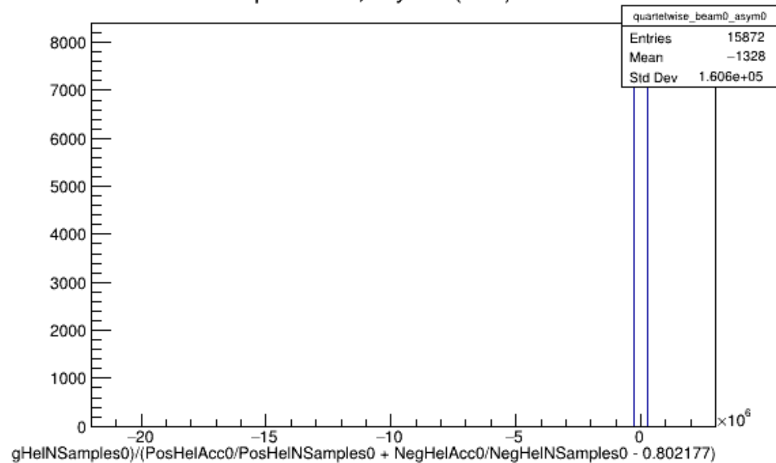
Run 5902 quartetwise, Asyms0 (Raw): Beam OFF
