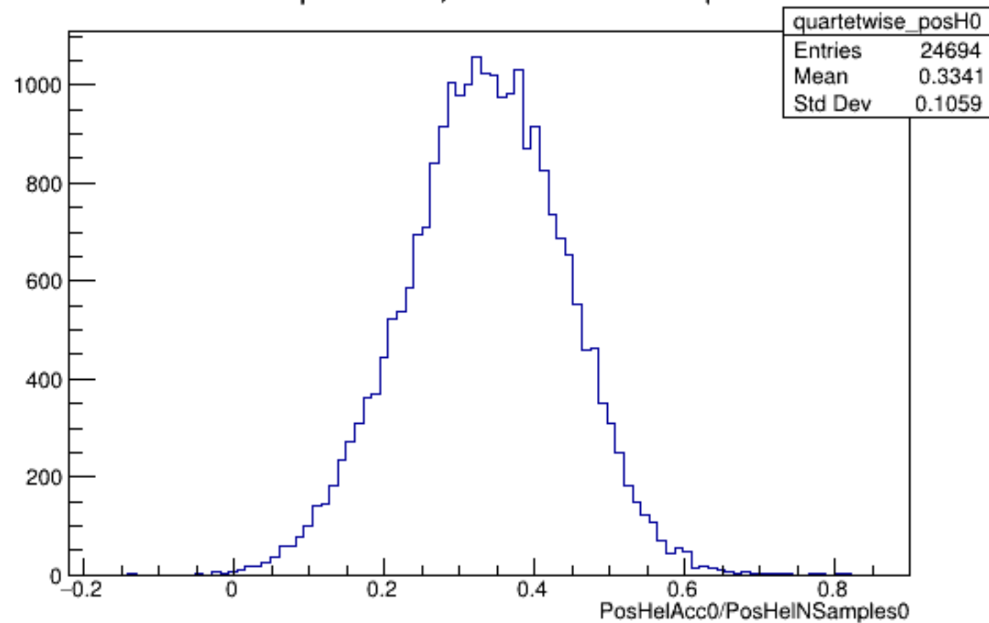
Run 5902 quartetwise, PosHelAcc0/NSamples0: All
