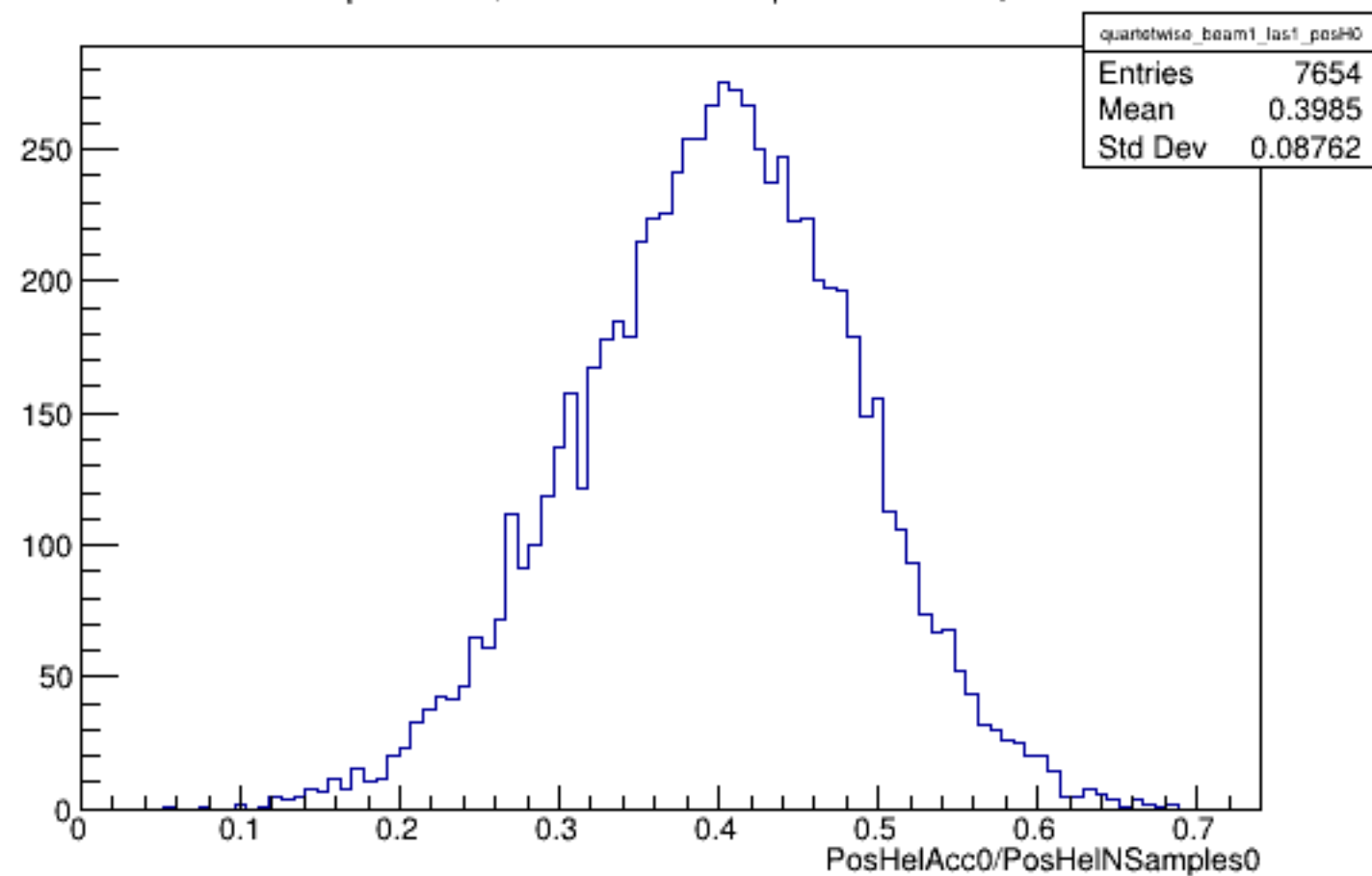
Run 5902 quartetwise, PosHelAcc0/NSamples0: Beam ON, Laser ON
