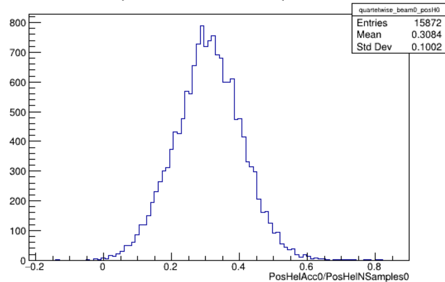
Run 5902 quartetwise, PosHelAcc0/NSamples0: Beam OFF
