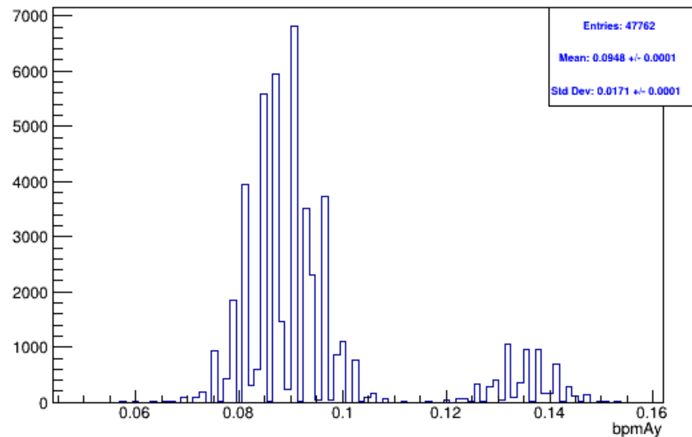
Run 5903, mpwise, bpmAy: Beam ON, Laser OFF
