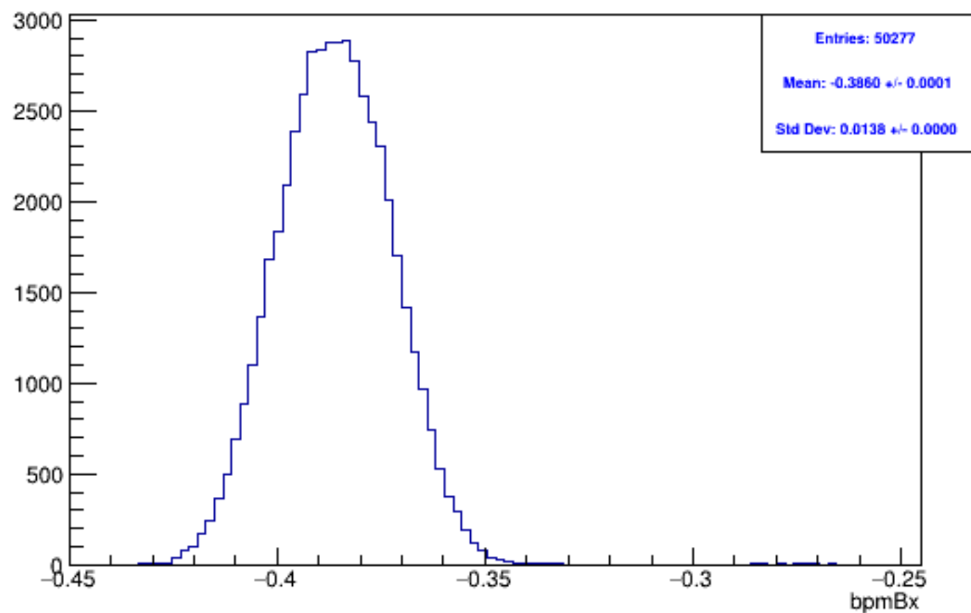
Run 5903, mpwise, bpmBx: Beam ON, Laser ON
