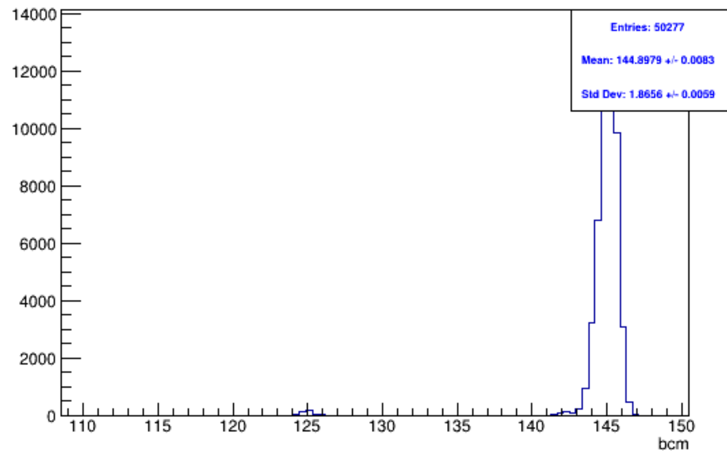
Run 5903, mpwise, BCM: Beam ON, Laser ON
