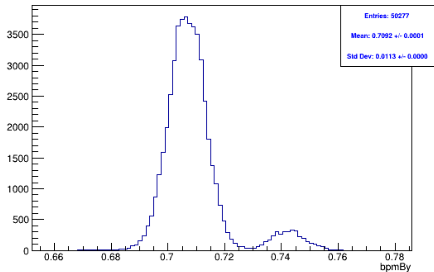
Run 5903, mpswise, bpmBy: Beam ON, Laser ON
