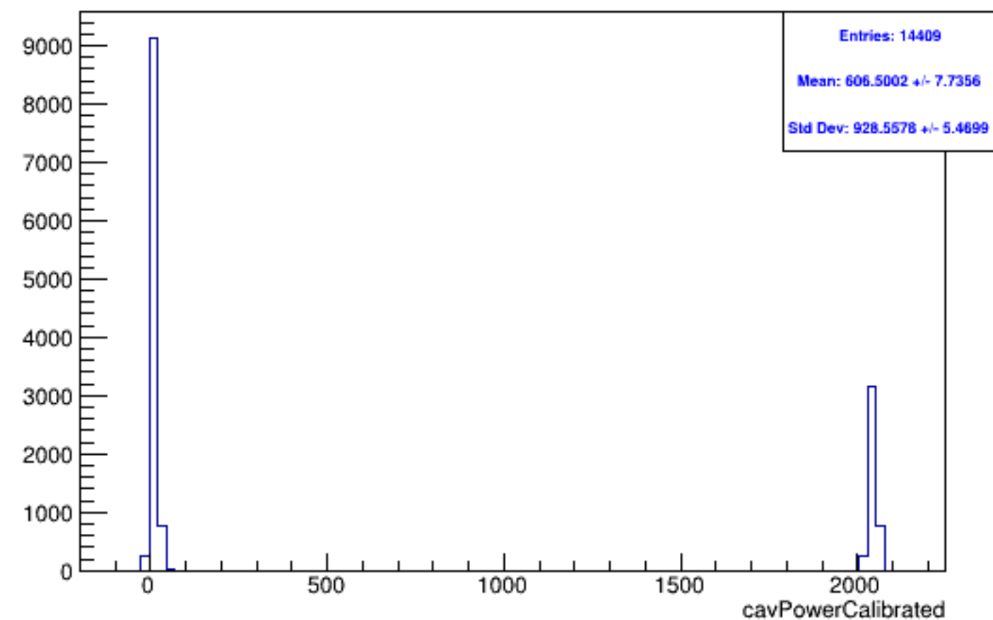
Run 5903 mpswise, lasPow: Beam OFF
