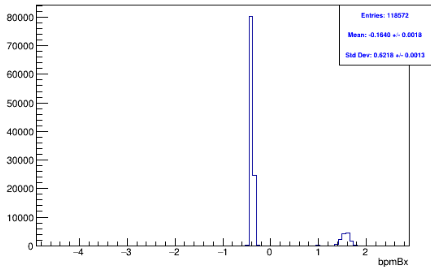
Run 5903 mpwise, bpmBx: All
