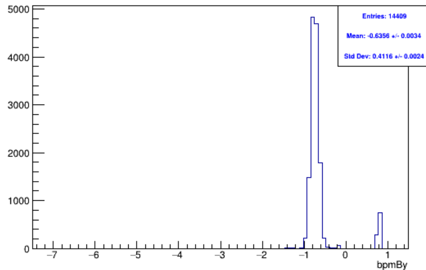
Run 5903 mpswise, bpmBy: Beam OFF
