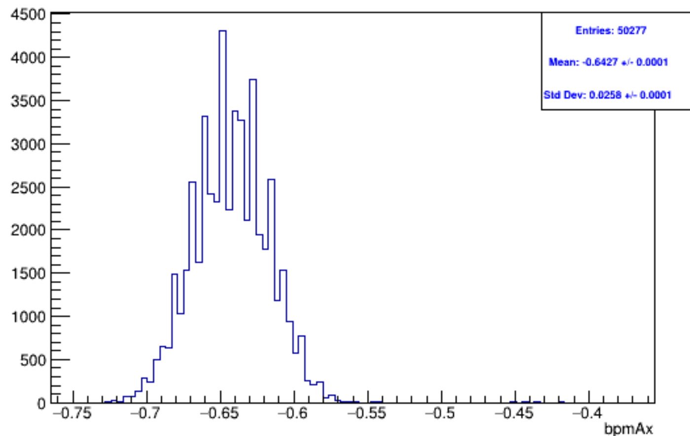
Run 5903, mpwise, bpmAx: Beam ON, Laser ON
