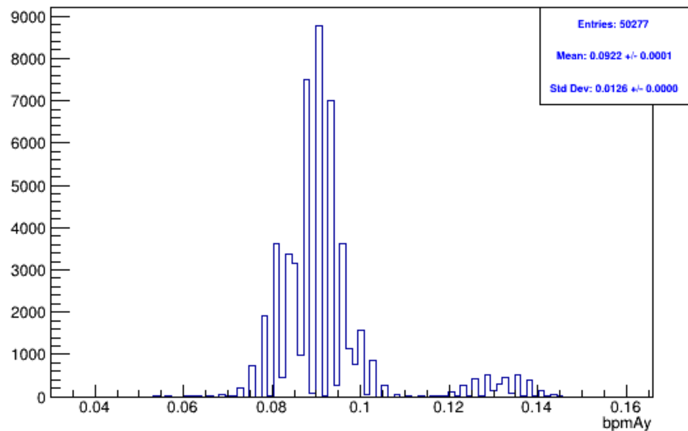
Run 5903, mpwise, bpmAy: Beam ON, Laser ON
