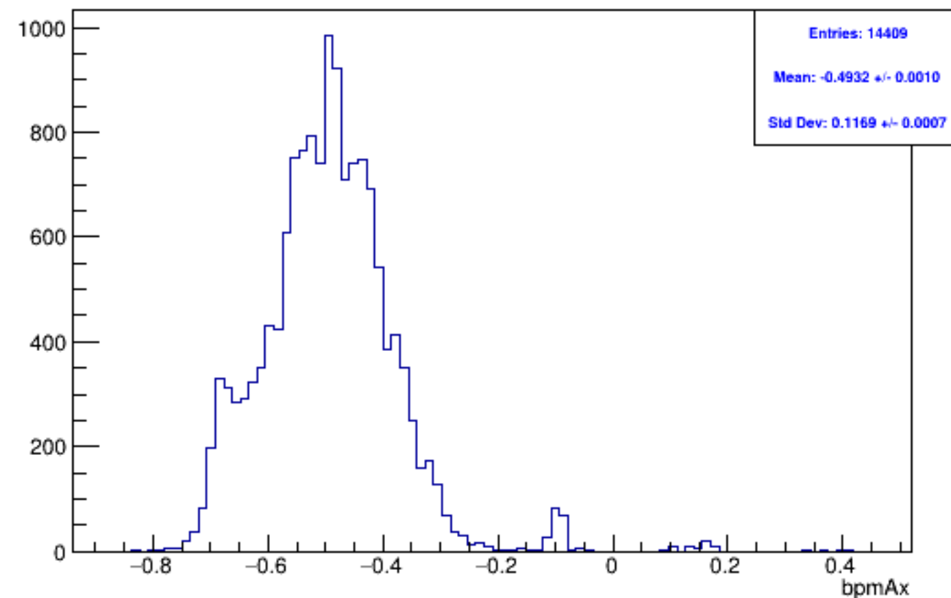
Run 5903 mpwise, bpmAx: Beam OFF
