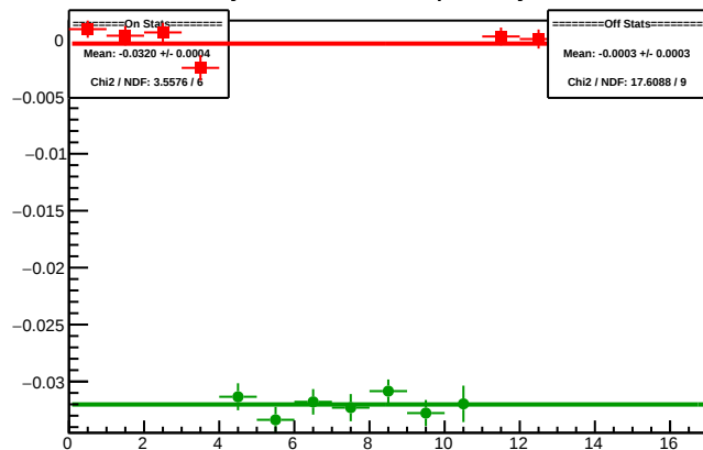
Cycle 5904.1: Multiplet Asyms
