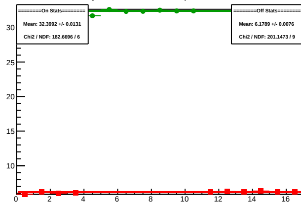
Cycle 5904.1: Multiplet Sums
