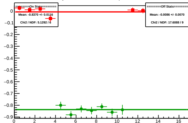
Cycle 5904.1: Multiplet Diffs
