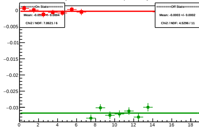
Cycle 5904.9: Multiplet Asyms
