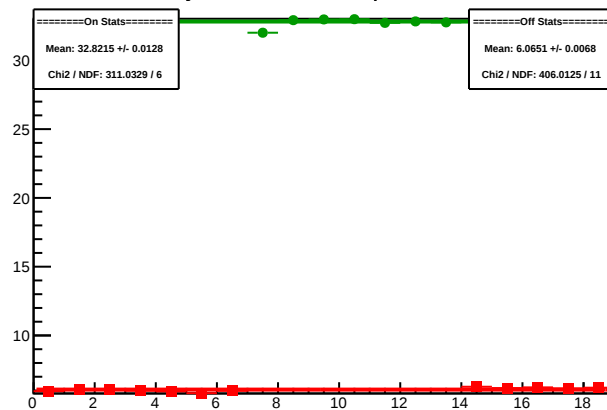
Cycle 5904.9: Multiplet Sums
