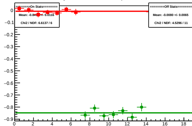
Cycle 5904.9: Multiplet Diffs
