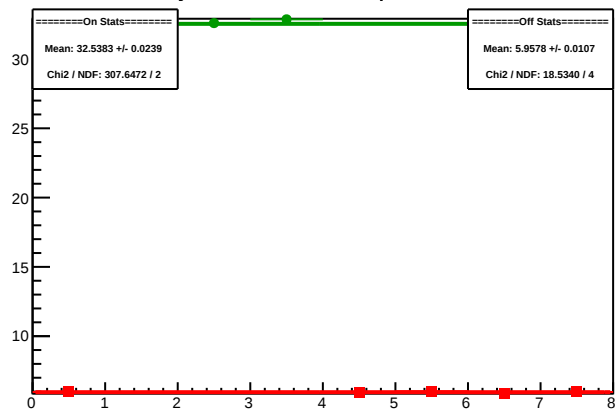
Cycle 5904.13: Multiplet Sums
