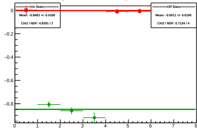
Cycle 5904.13: Multiplet Diffs
