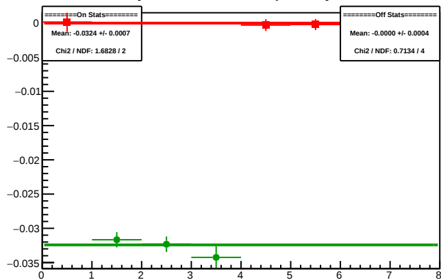
Cycle 5904.13: Multiplet Asyms
