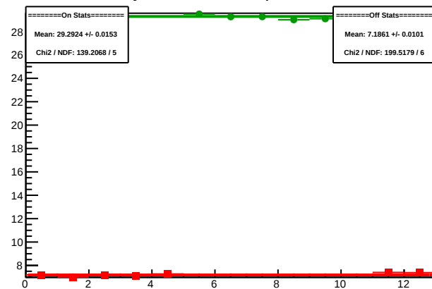
Cycle 5909.4: Multiplet Sums
