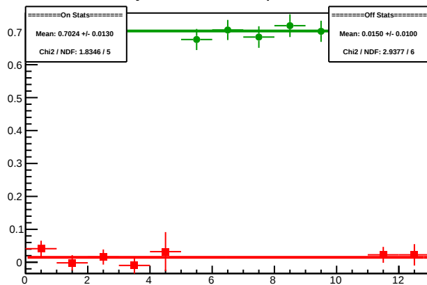
Cycle 5909.4: Multiplet Diffs
