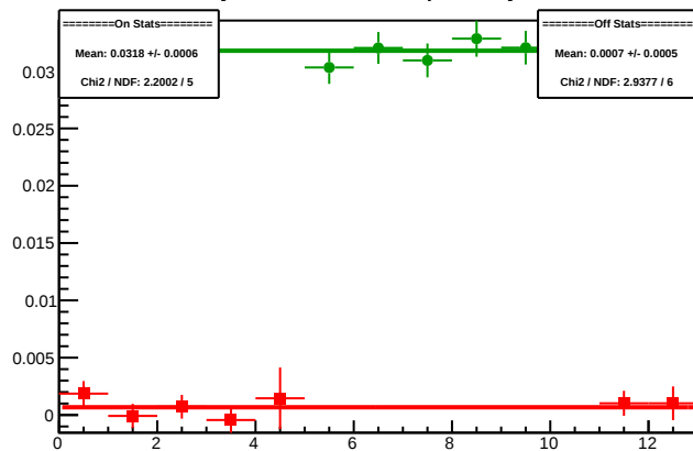
Cycle 5909.4: Multiplet Asyms
