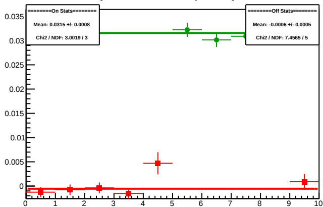
Cycle 5909.6: Multiplet Asyms
