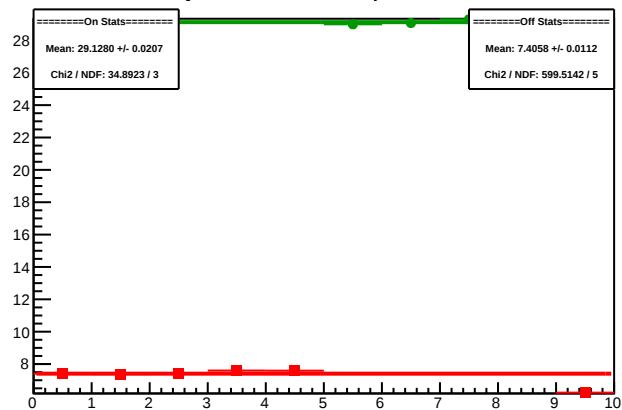
Cycle 5909.6: Multiplet Sums
