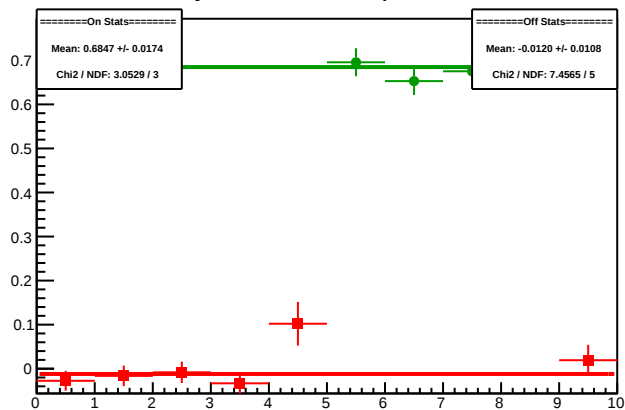
Cycle 5909.6: Multiplet Diffs
