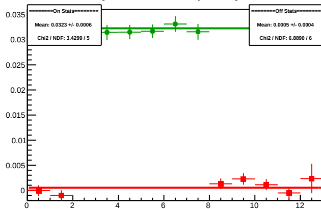
Cycle 5909.8: Multiplet Asyms
