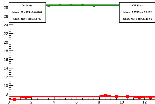
Cycle 5909.8: Multiplet Sums
