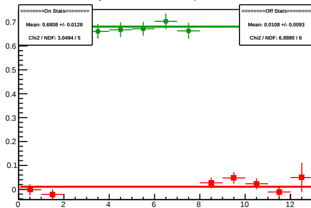
Cycle 5909.8: Multiplet Diffs
