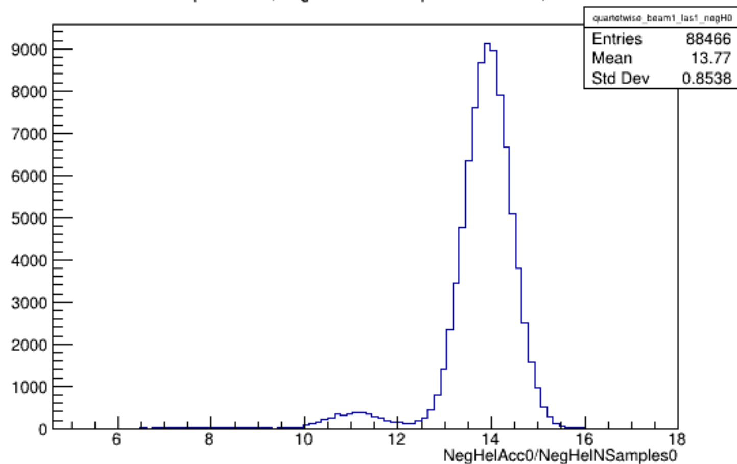
Run 5909 quartetwise, NegHelAcc0/NSamples0: Beam ON, Laser ON
