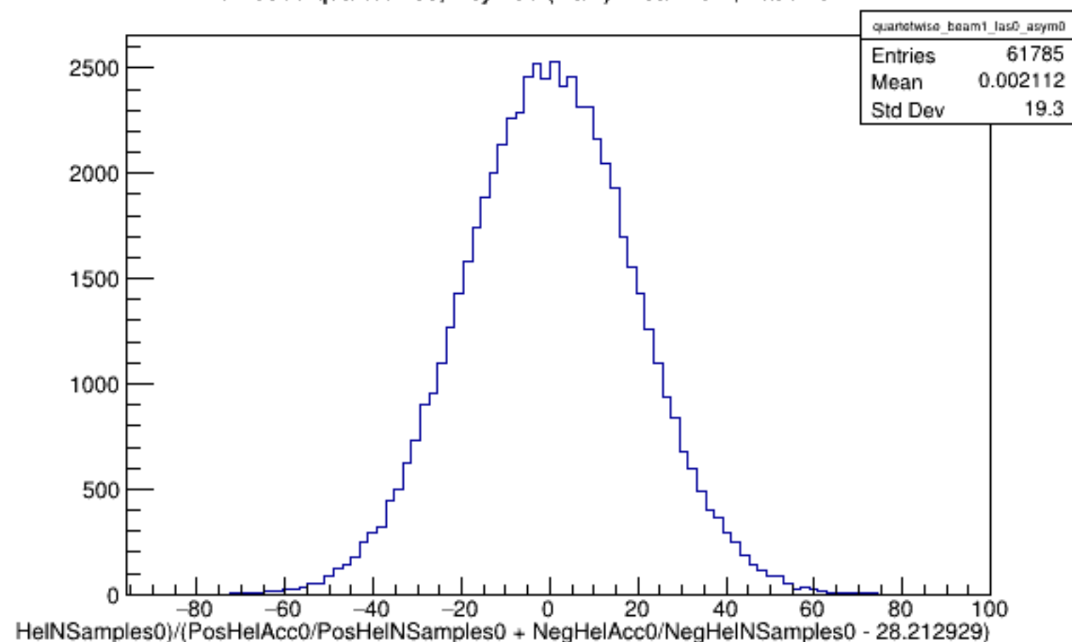
Run 5909 quartetwise, Asyms0 (Raw): Beam ON, Laser OFF
