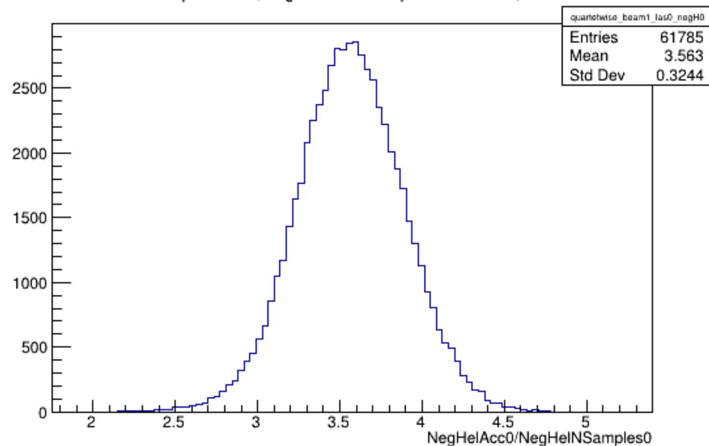
Run 5909 quartetwise, NegHelAcc0/NSamples0: Beam ON, Laser OFF
