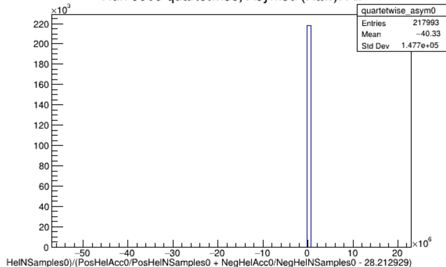
Run 5909 quartetwise, Asyms0 (Raw): All
