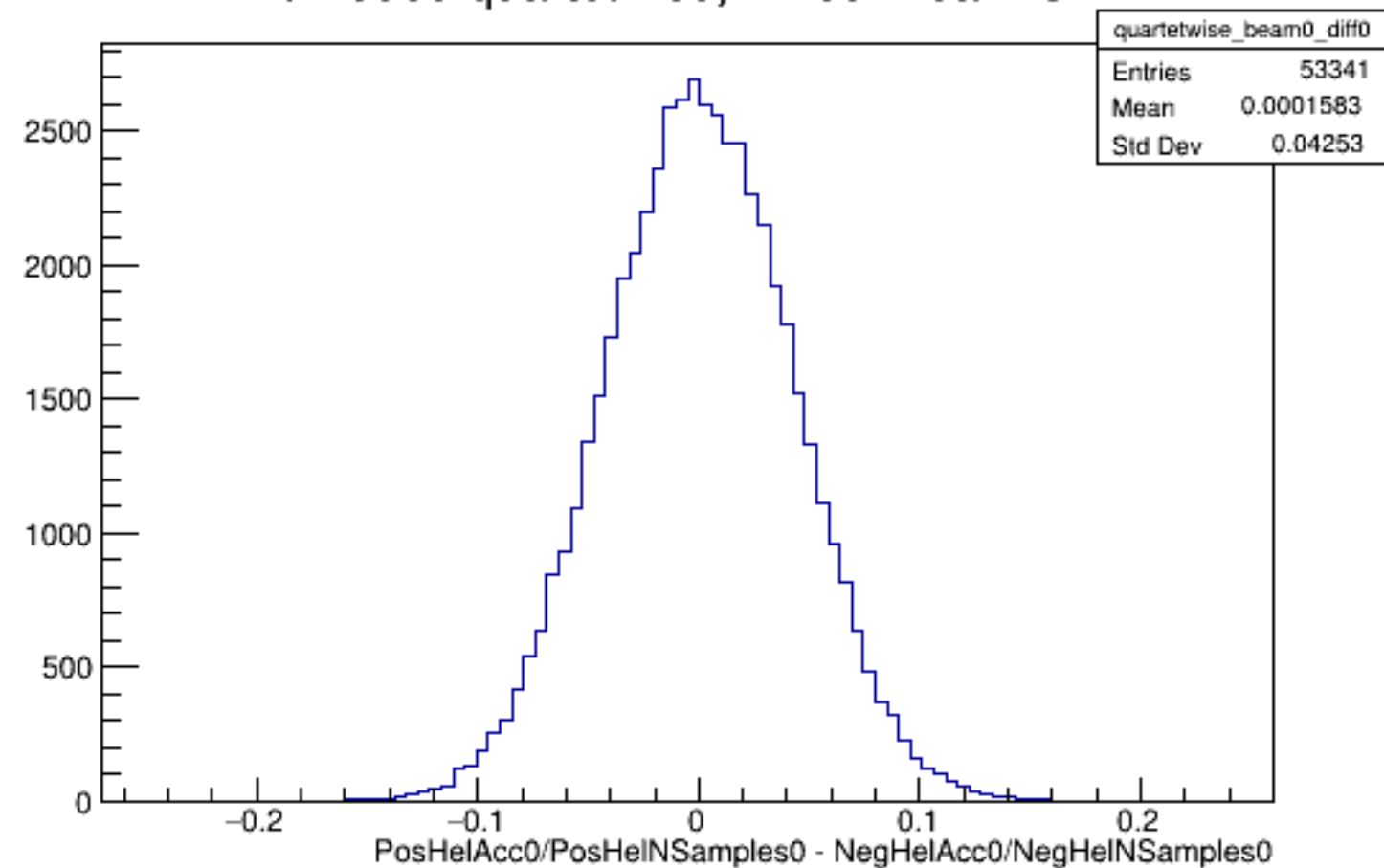
Run 5909 quartetwise, Diffs0: Beam OFF
