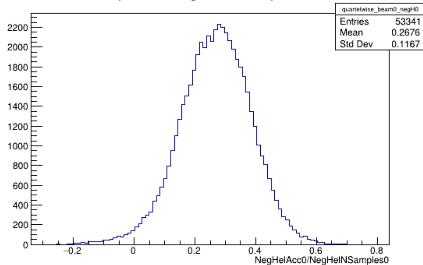
Run 5909 quartetwise, NegHelAcc0/NSamples0: Beam OFF
