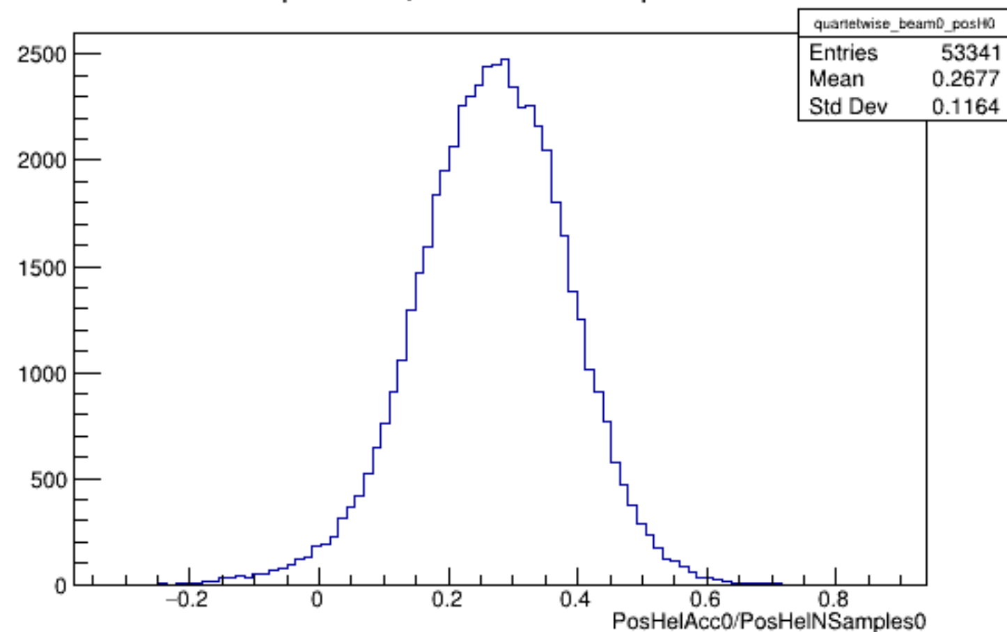
Run 5909 quartetwise, PosHelAcc0/NSamples0: Beam OFF
