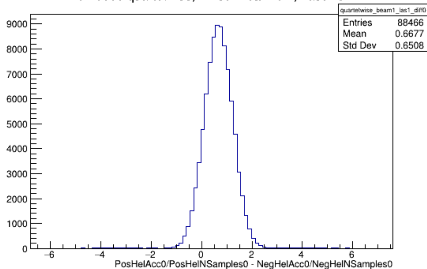
Run 5909 quartetwise, Diffs0: Beam ON, Laser ON
