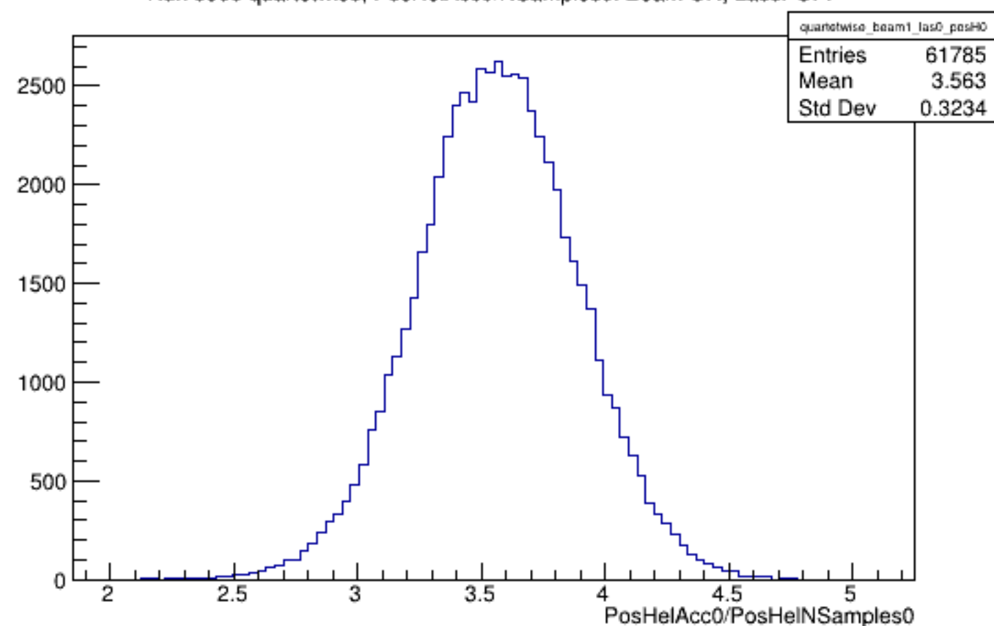
Run 5909 quartetwise, PosHelAcc0/NSamples0: Beam ON, Laser OFF
