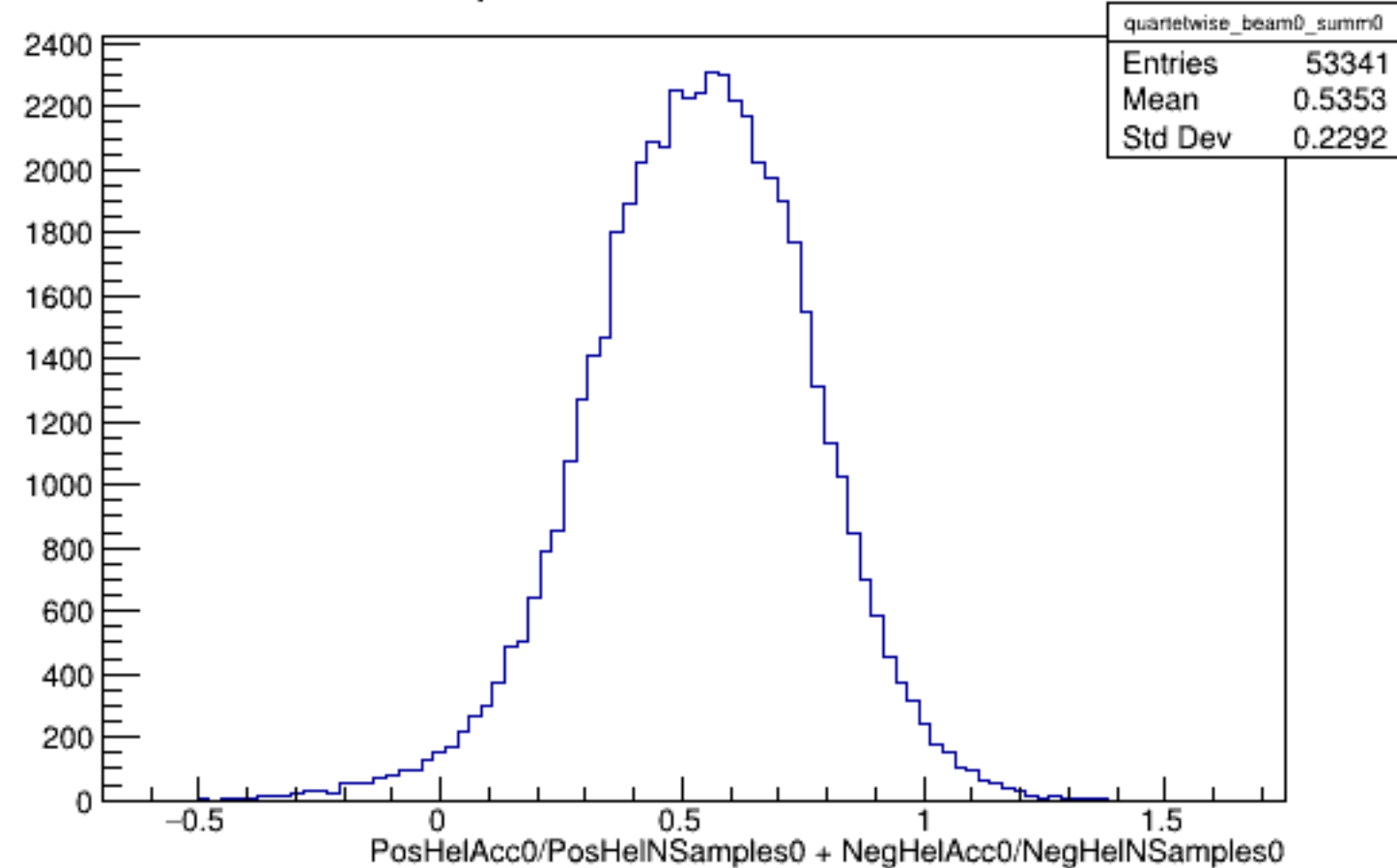
Run 5909 quartetwise, Sums0: Beam OFF
