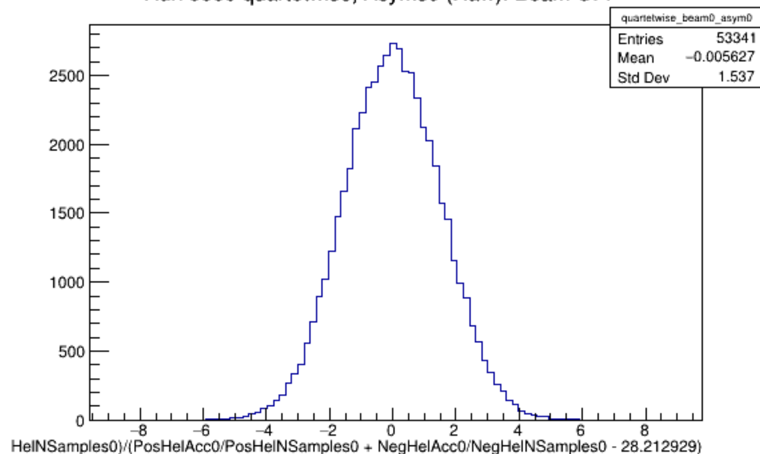
Run 5909 quartetwise, Asyms0 (Raw): Beam OFF
