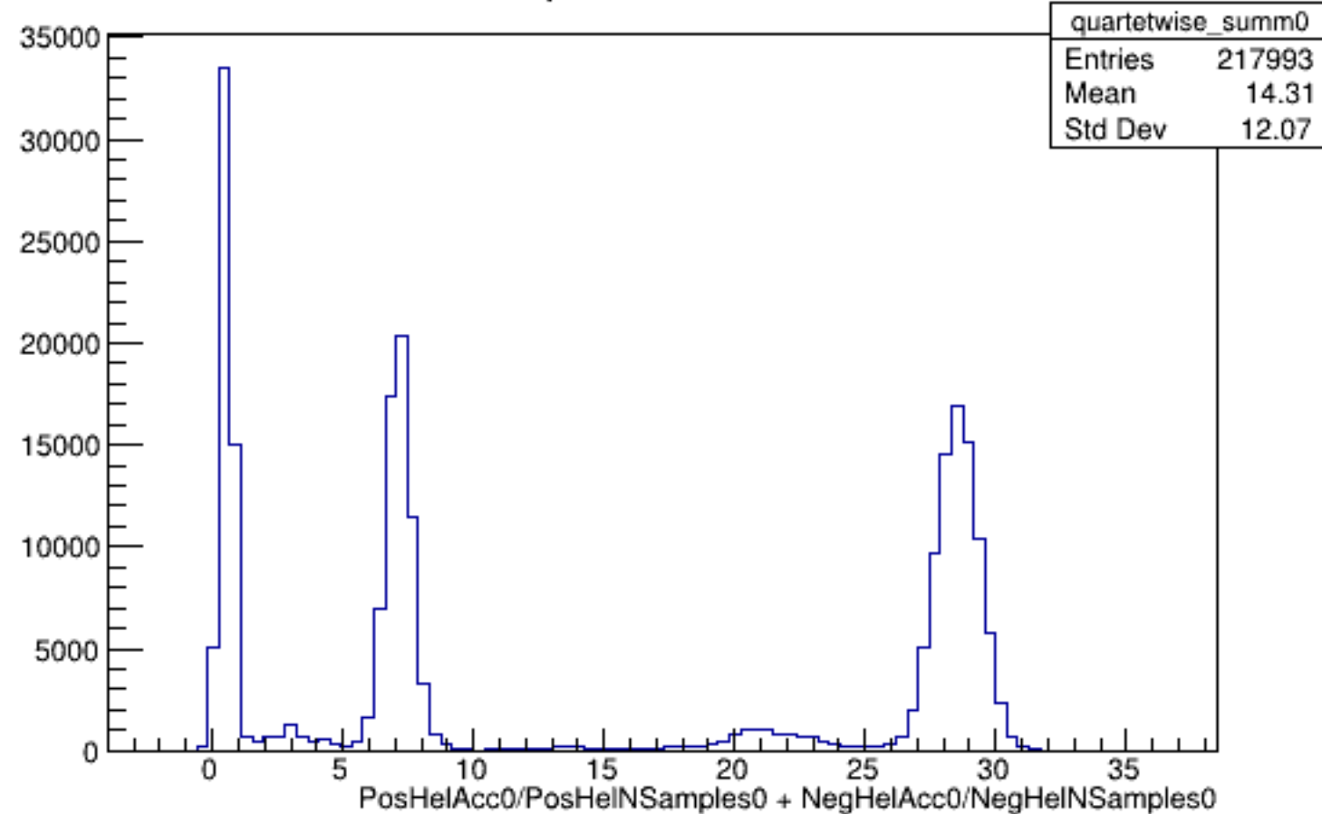
Run 5909 quartetwise, Sums0: All
