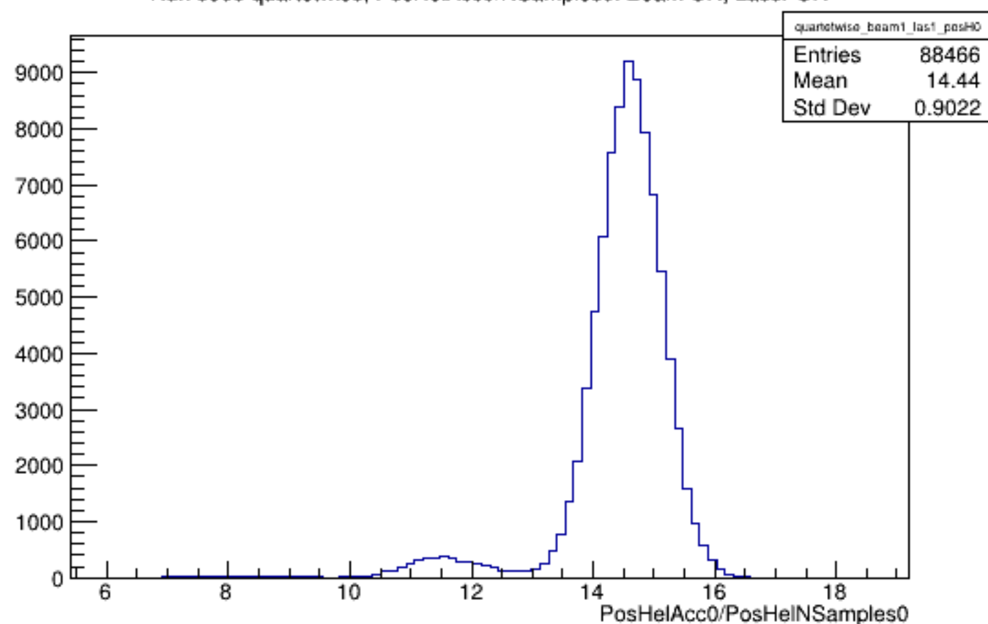
Run 5909 quartetwise, PosHelAcc0/NSamples0: Beam ON, Laser ON
