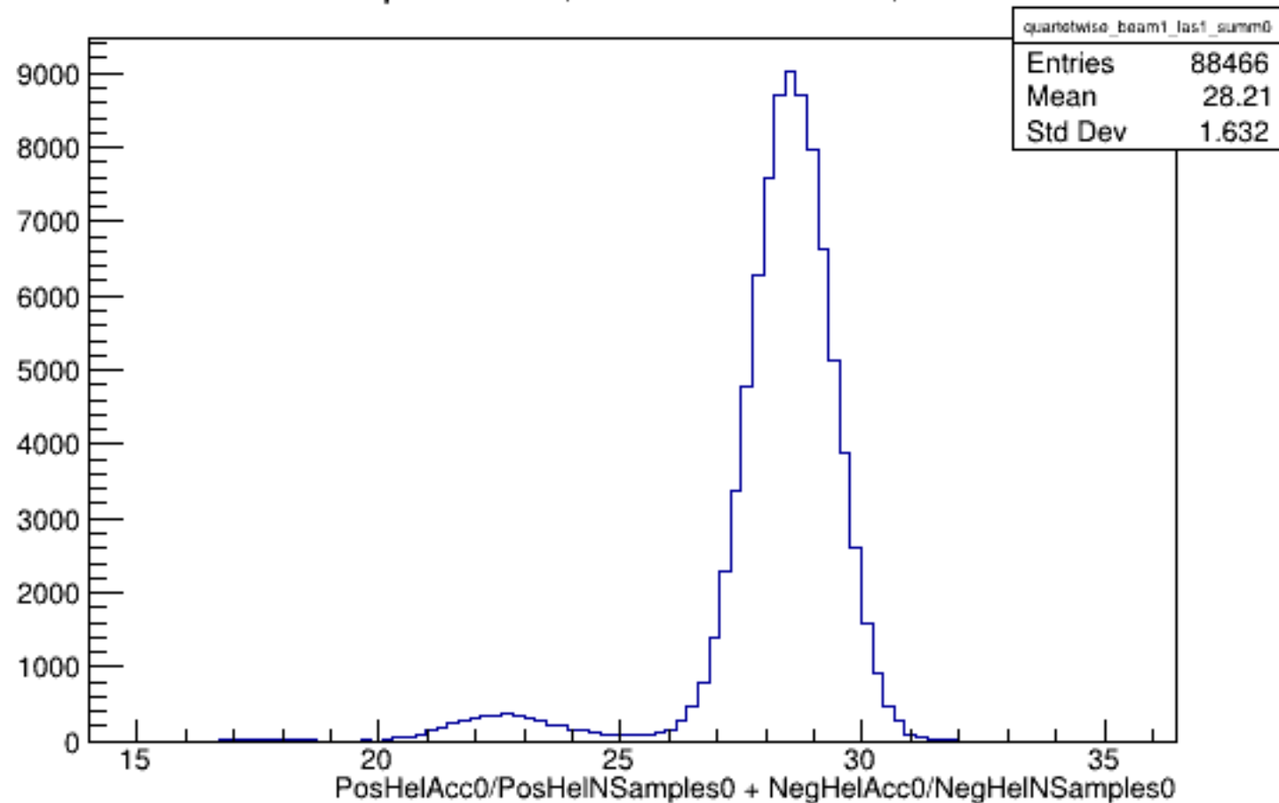
Run 5909 quartetwise, Sums0: Beam ON, Laser ON
