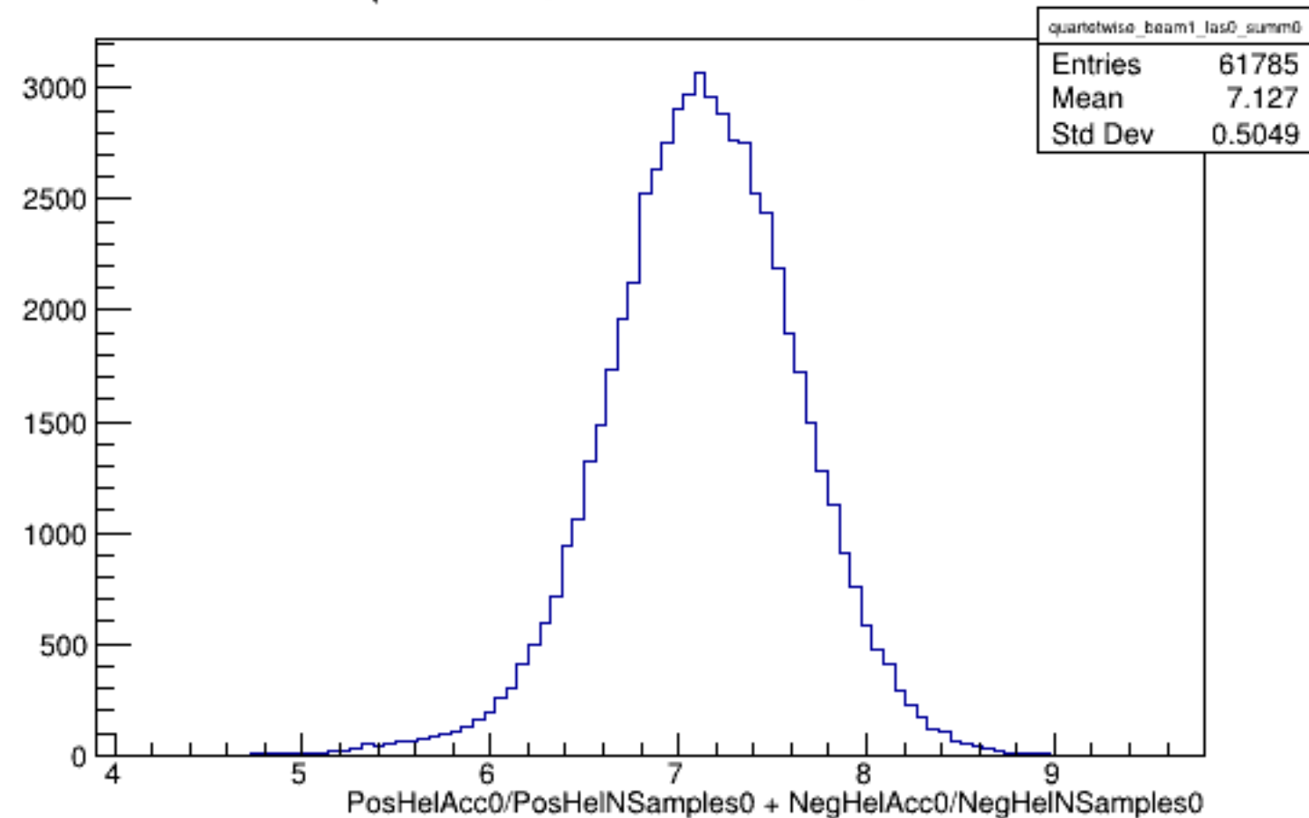
Run 5909 quartetwise, Sums0: Beam ON, Laser OFF
