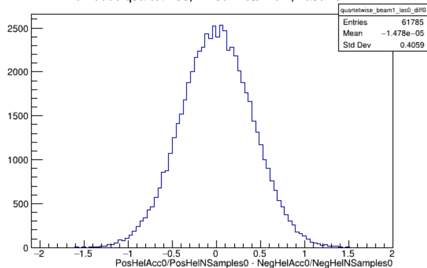
Run 5909 quartetwise, Diffs0: Beam ON, Laser OFF
