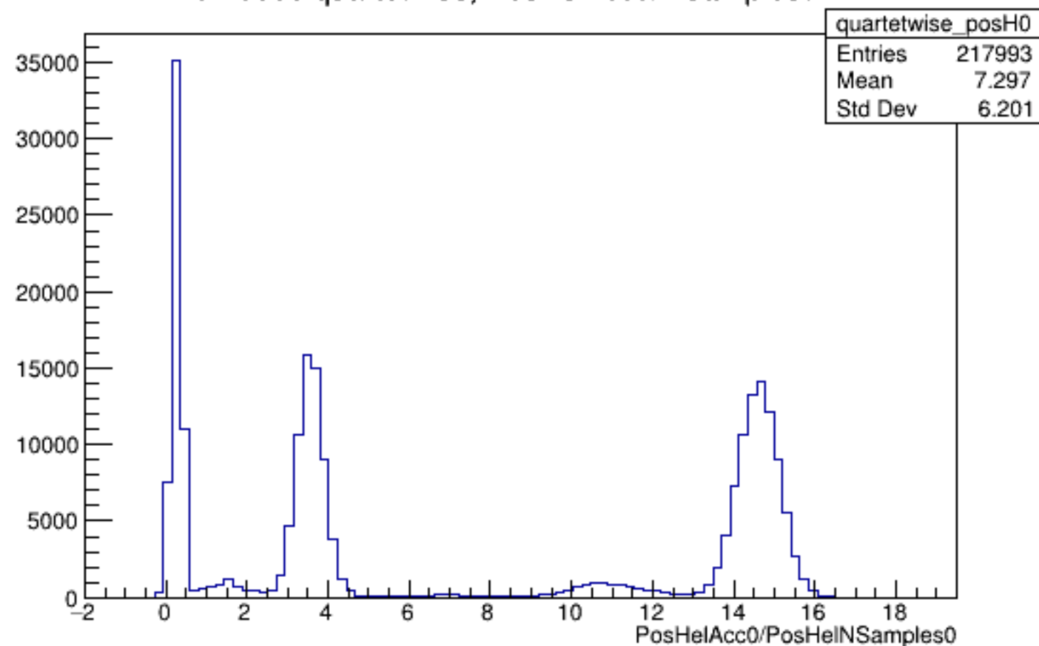
Run 5909 quartetwise, PosHelAcc0/NSamples0: All
