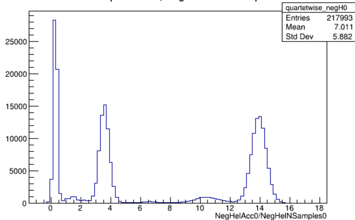
Run 5909 quartetwise, NegHelAcc0/NSamples0: All
