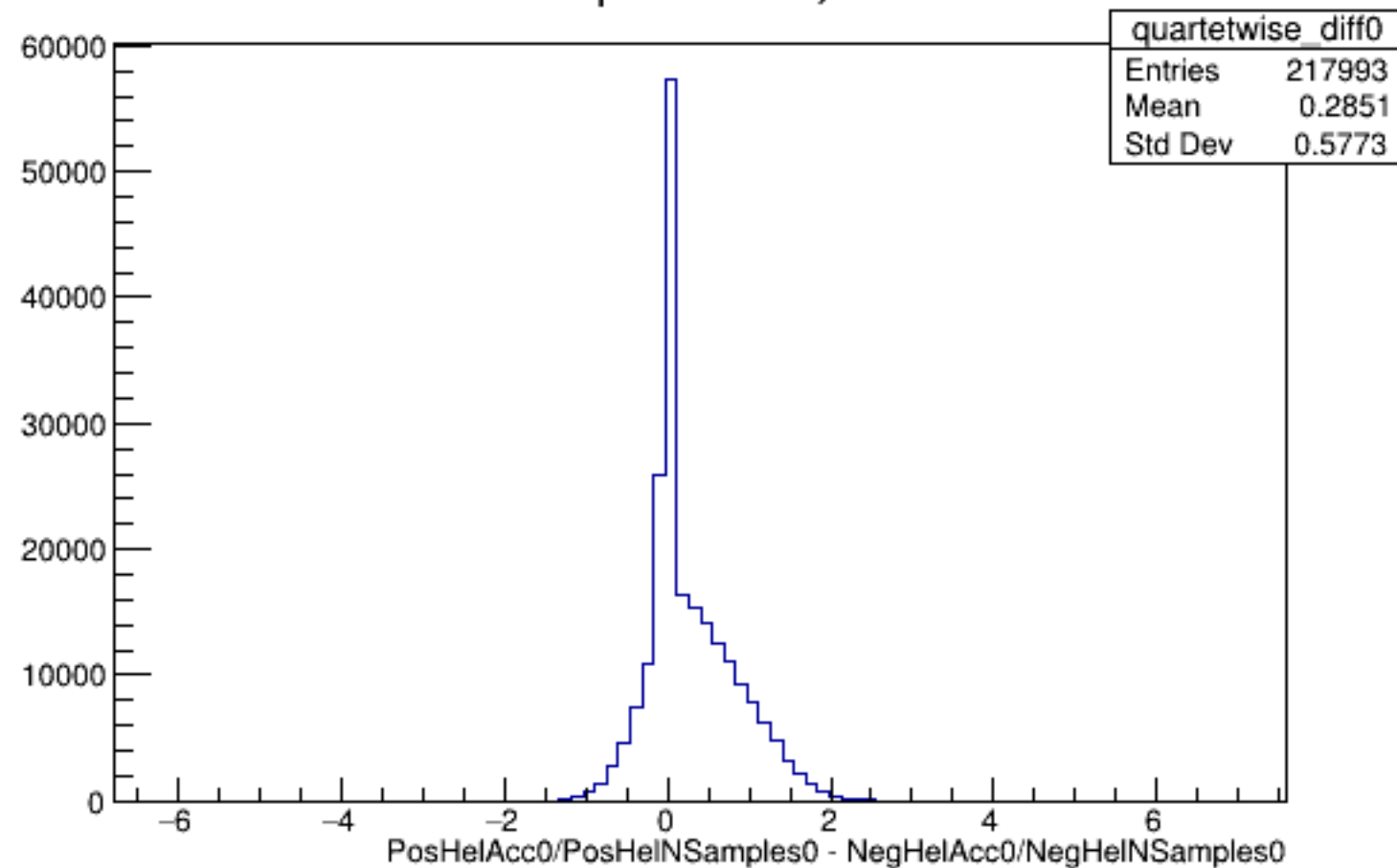
Run 5909 quartetwise, Diffs0: All
