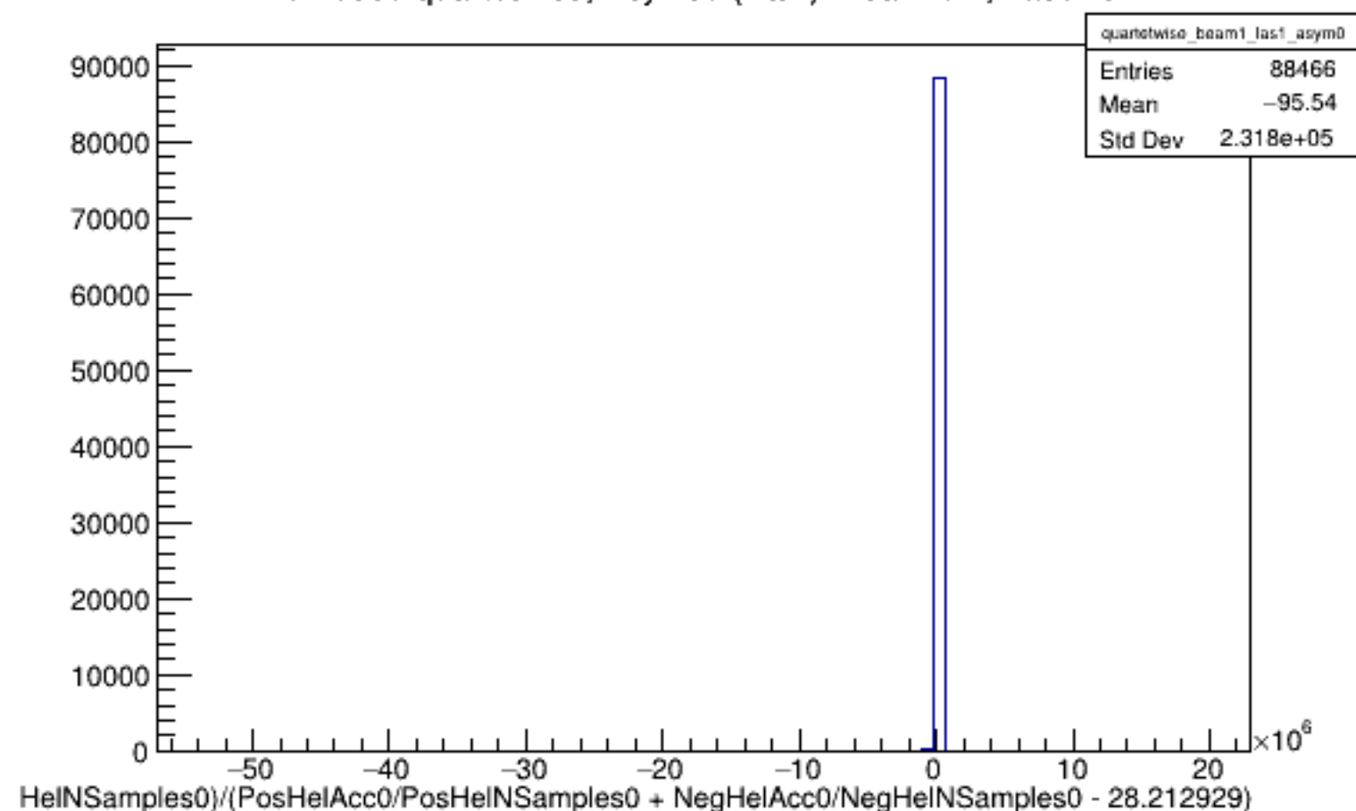
Run 5909 quartetwise, Asyms0 (Raw): Beam ON, Laser ON
