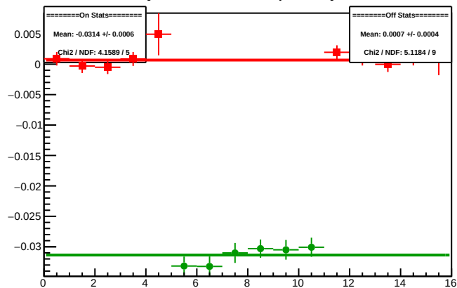
Cycle 5911.5: Multiplet Asyms
