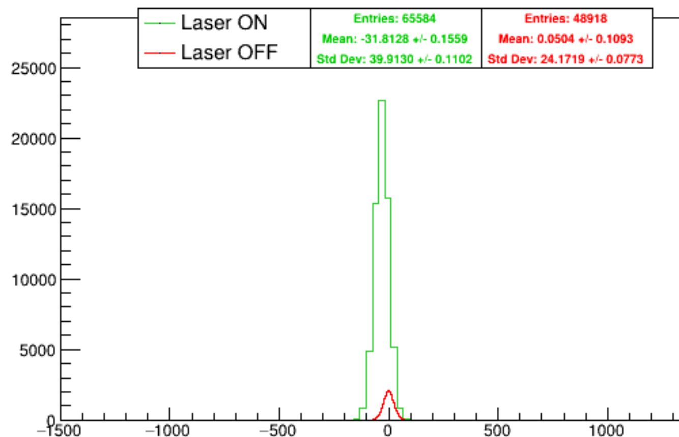
Run 5915 quartetwise, asym0sub: Beam ON
