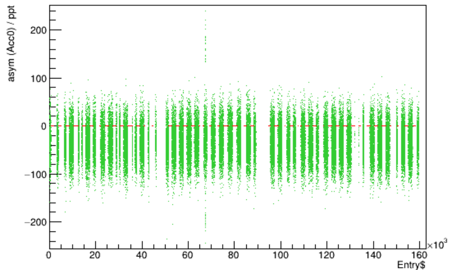
Run 5915 quartetwise, asym0sub vs time
