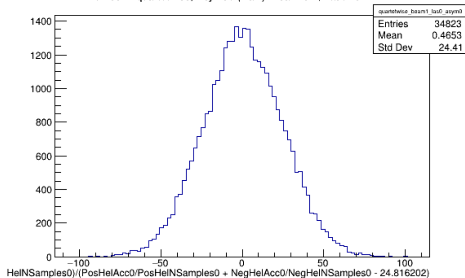
Run 5917 quartetwise, Asyms0 (Raw): Beam ON, Laser OFF
