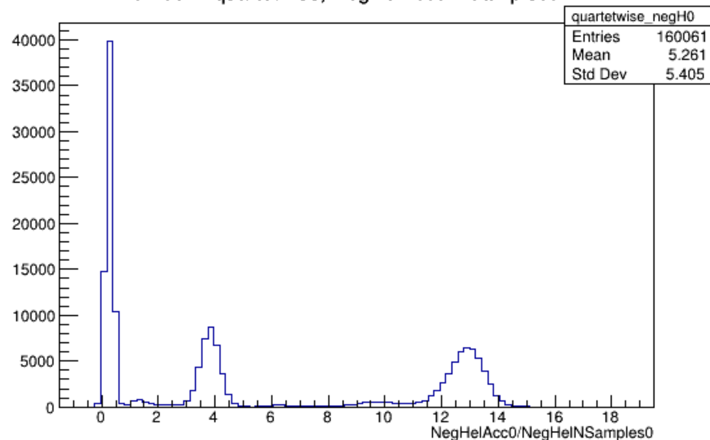
Run 5917 quartetwise, NegHelAcc0/NSamples0: All
