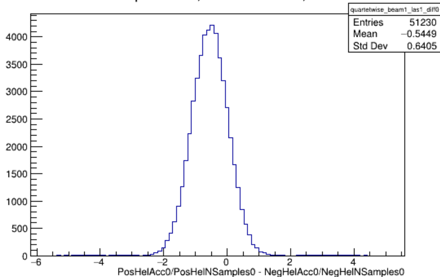
Run 5917 quartetwise, Diffs0: Beam ON, Laser ON
