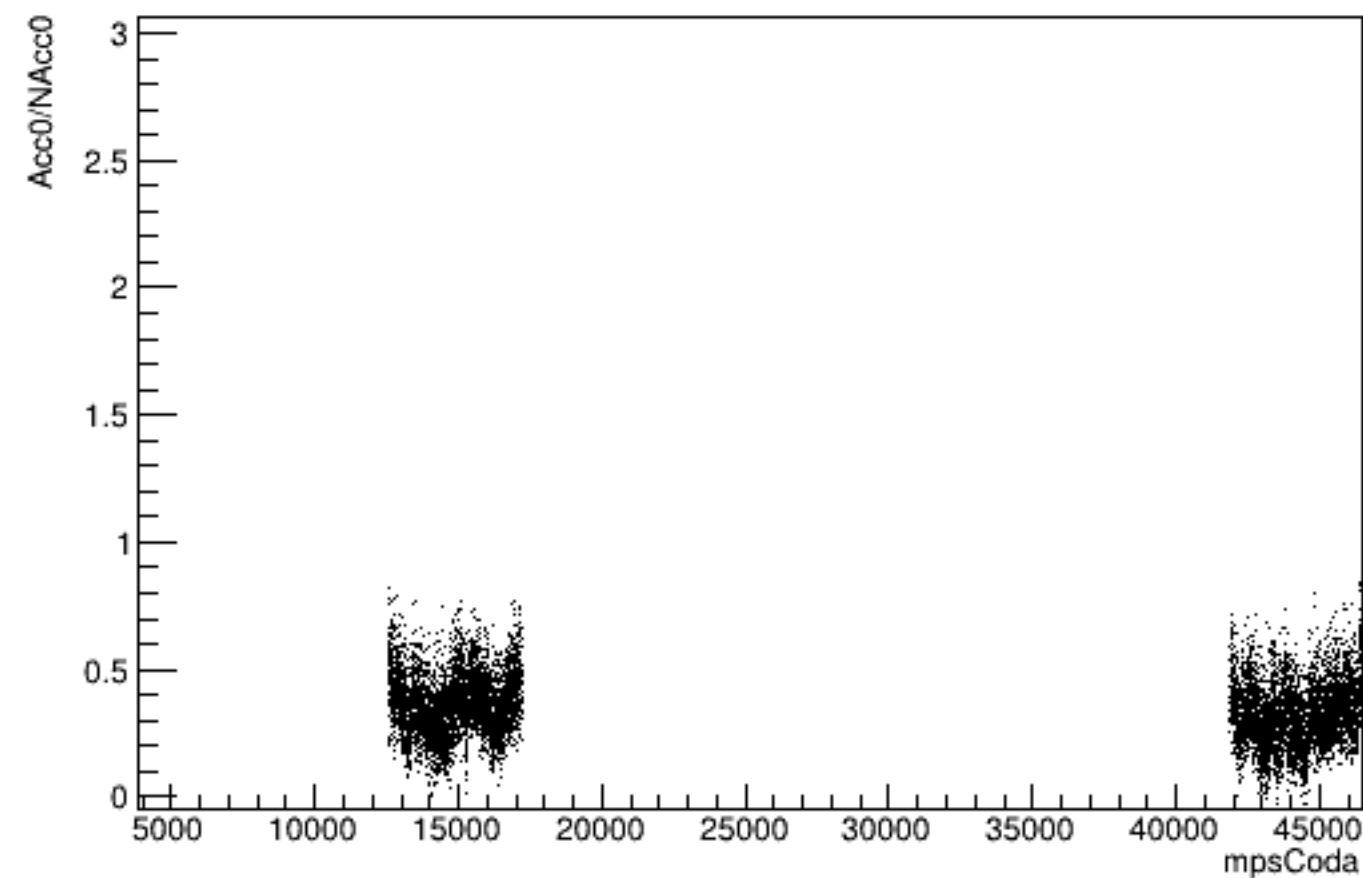
Run 5927 mpwise, Acc0 vs Time: Beam ON, Laser OFF
