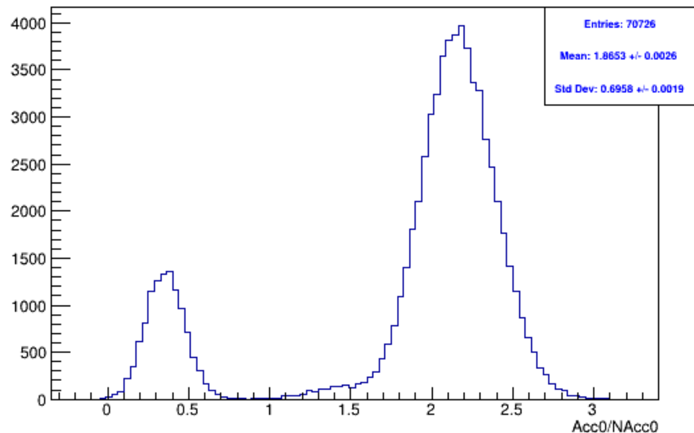
Run 5927 mpwise, acc0: All
