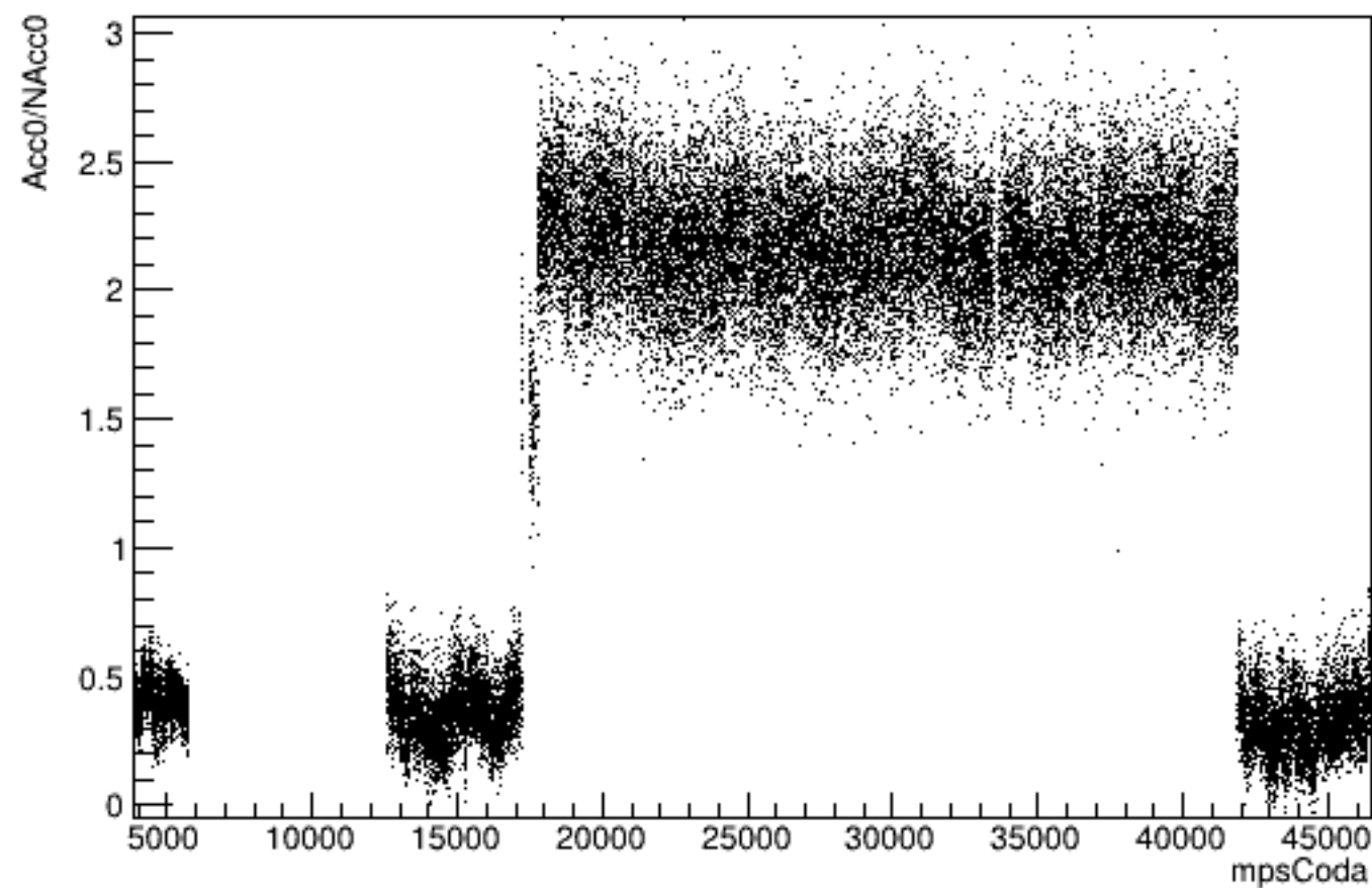
Run 5927 mpwise, Acc0 vs Time: All
