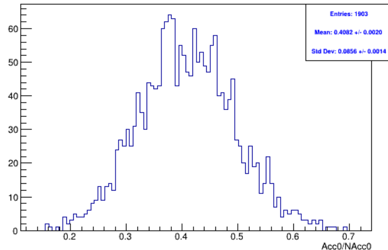
Run 5927 mpwise, acc0: Beam OFF
