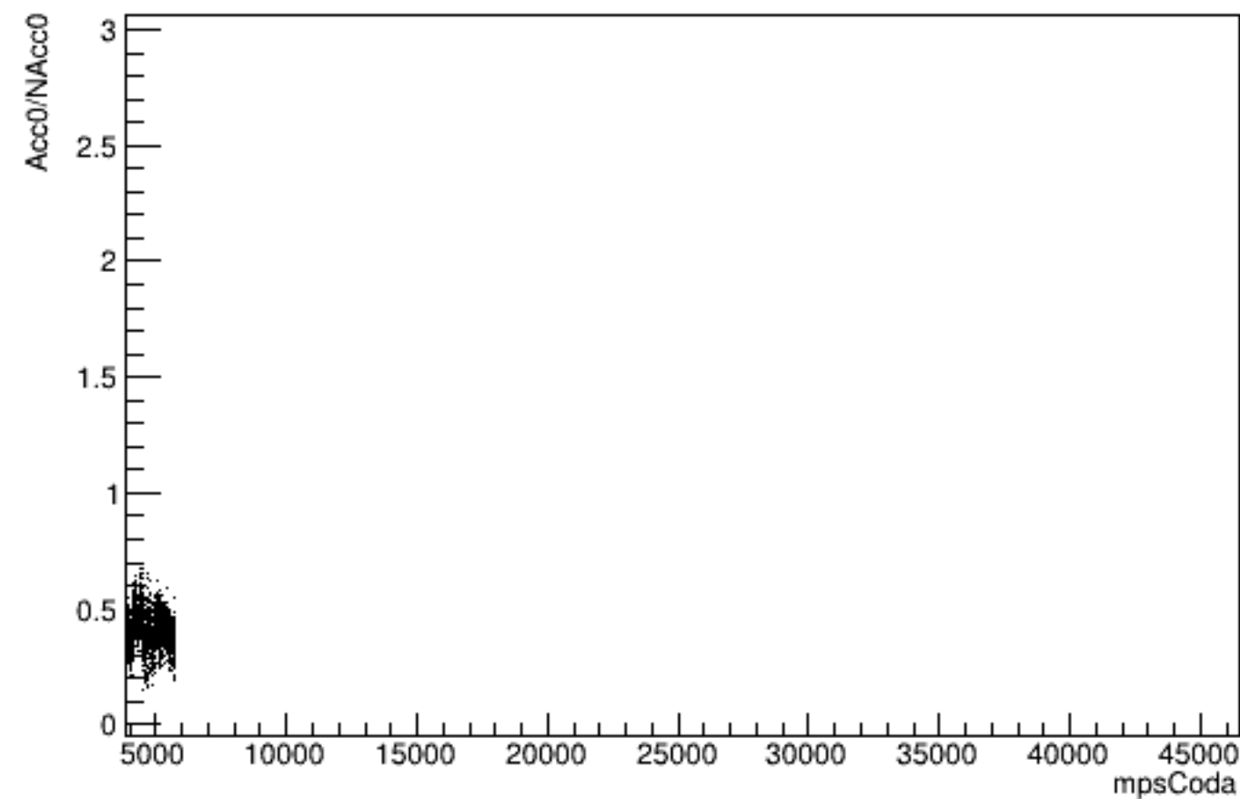
Run 5927 mpwise, Acc0 vs Time: Beam OFF
