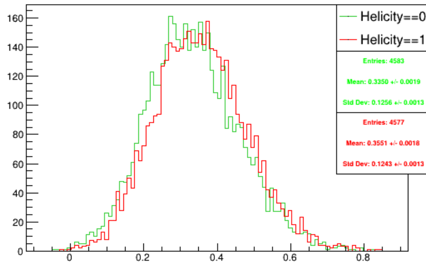
Run 5927 mpwise, acc0: Beam ON, Laser OFF
