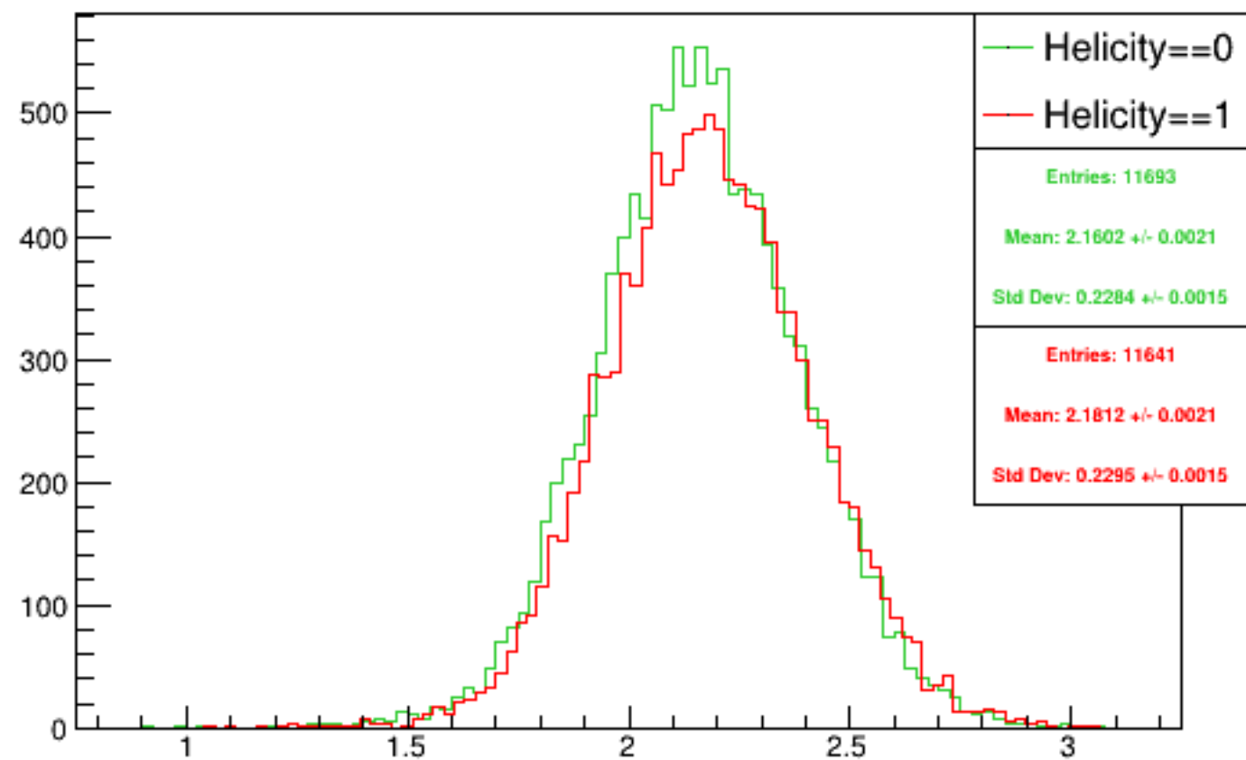
Run 5927 mpwise, acc0: Beam ON, Laser ON
