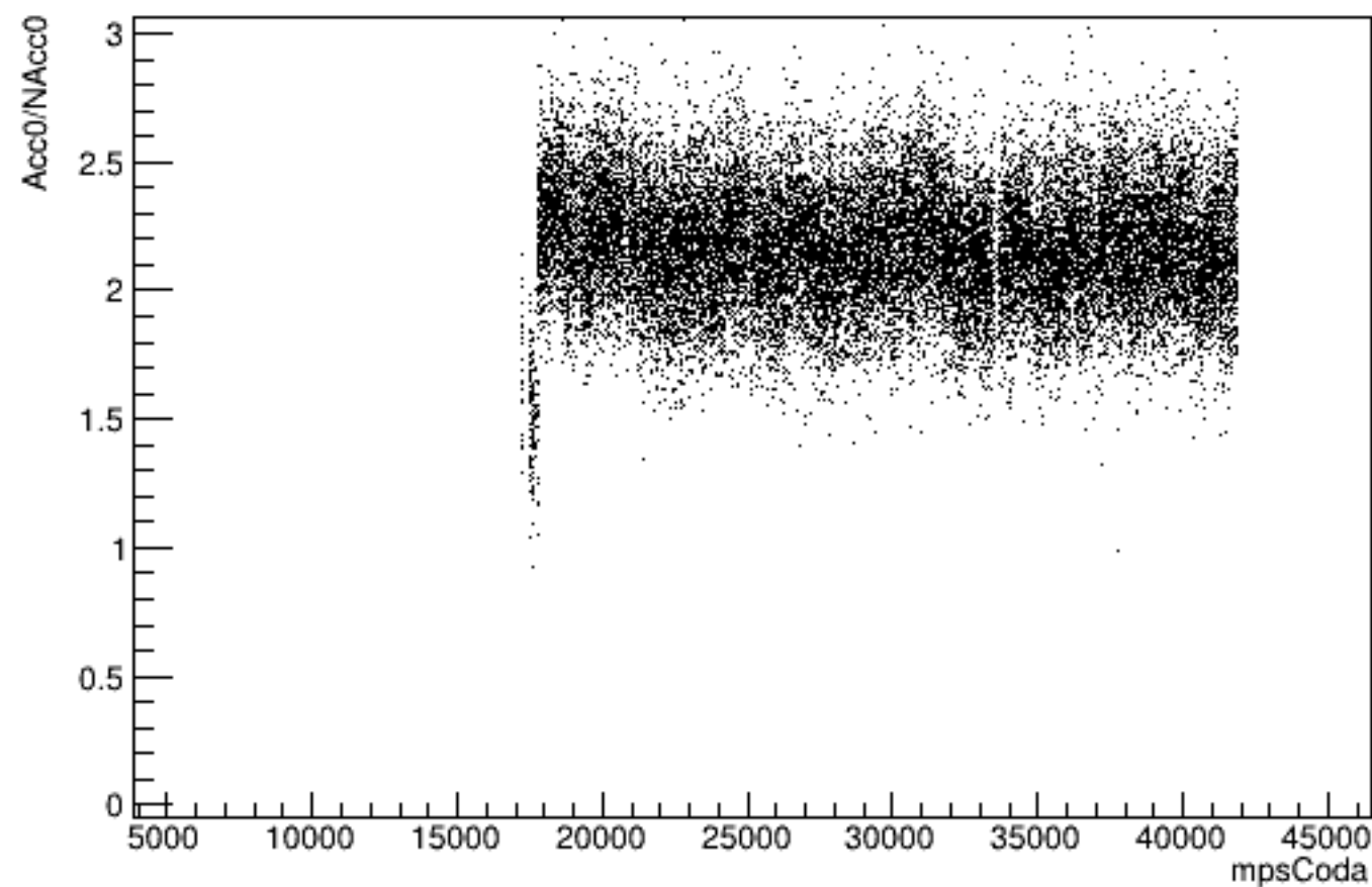
Run 5927 mpwise, Acc0 vs Time: Beam ON, Laser ON
