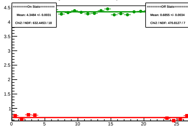
Cycle 5927.1: Multiplet Sums
