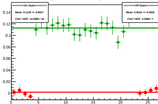
Cycle 5927.1: Multiplet Diffs
