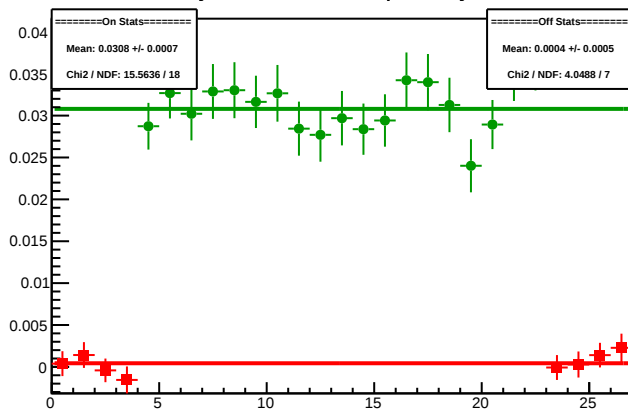
Cycle 5927.1: Multiplet Asyms
