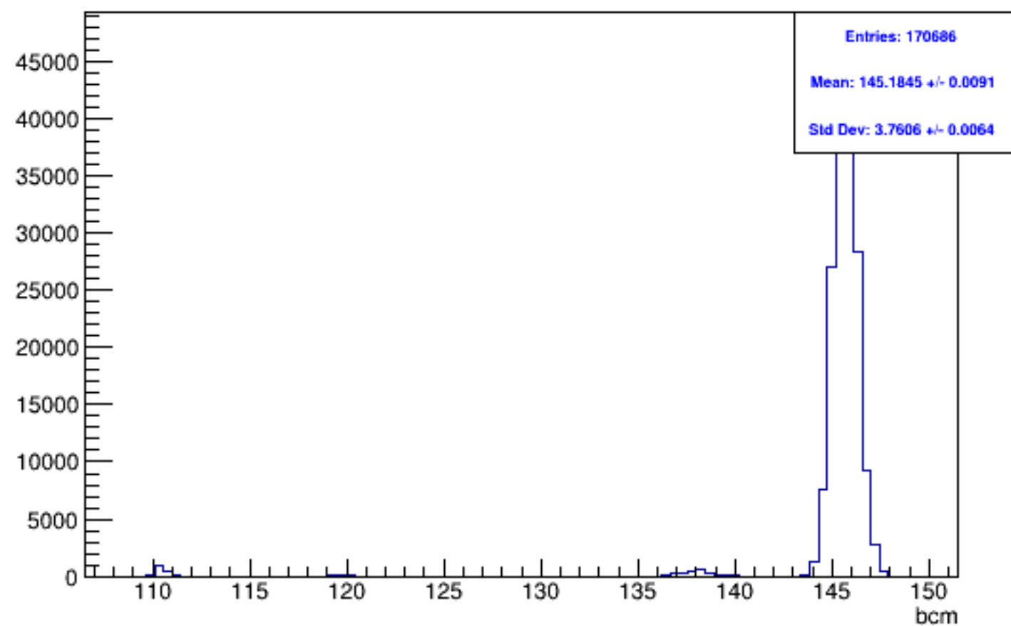
Run 5936, mpwise, BCM: Beam ON, Laser ON
