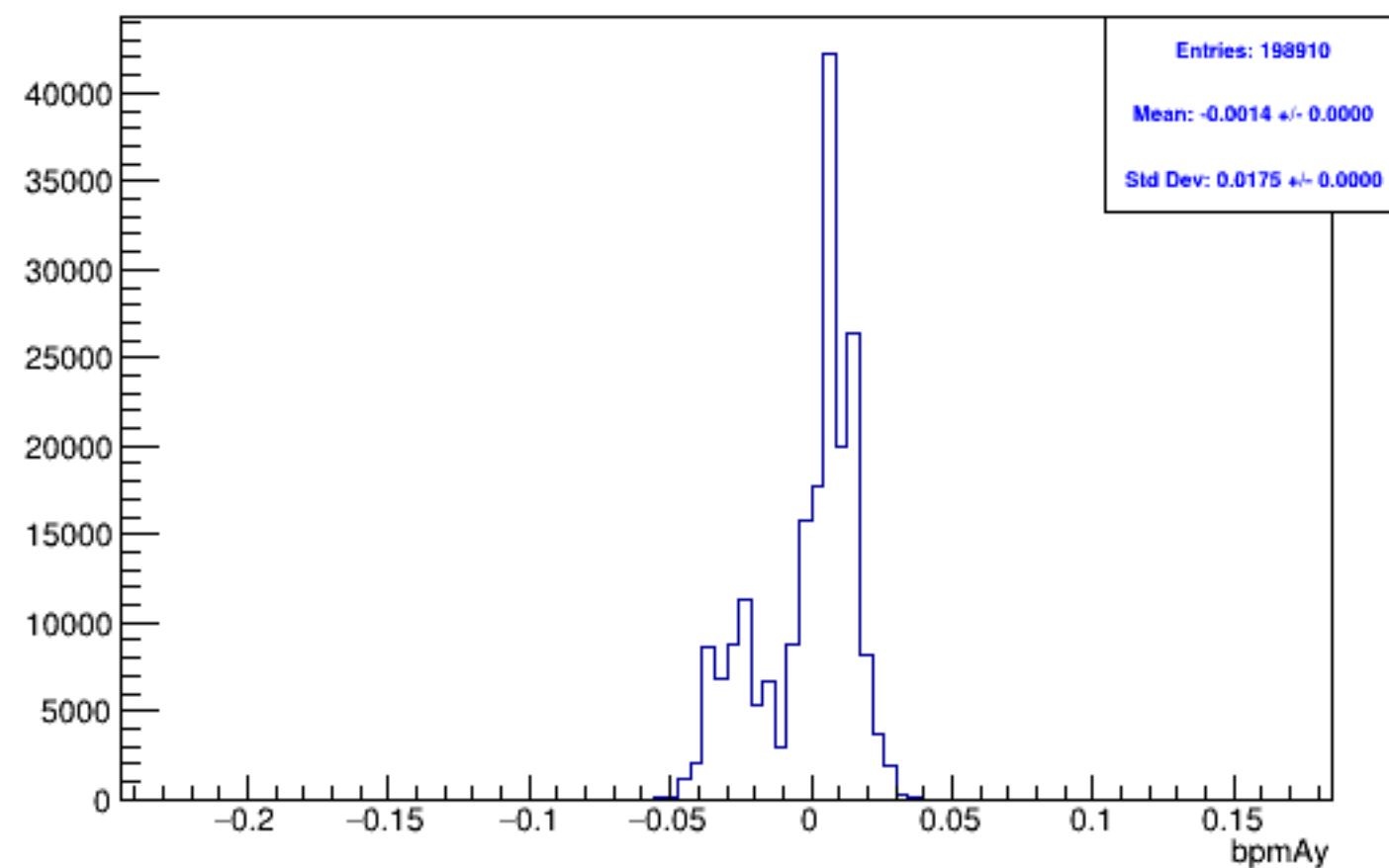
Run 5936, mpwise, bpmAy: Beam ON, Laser OFF
