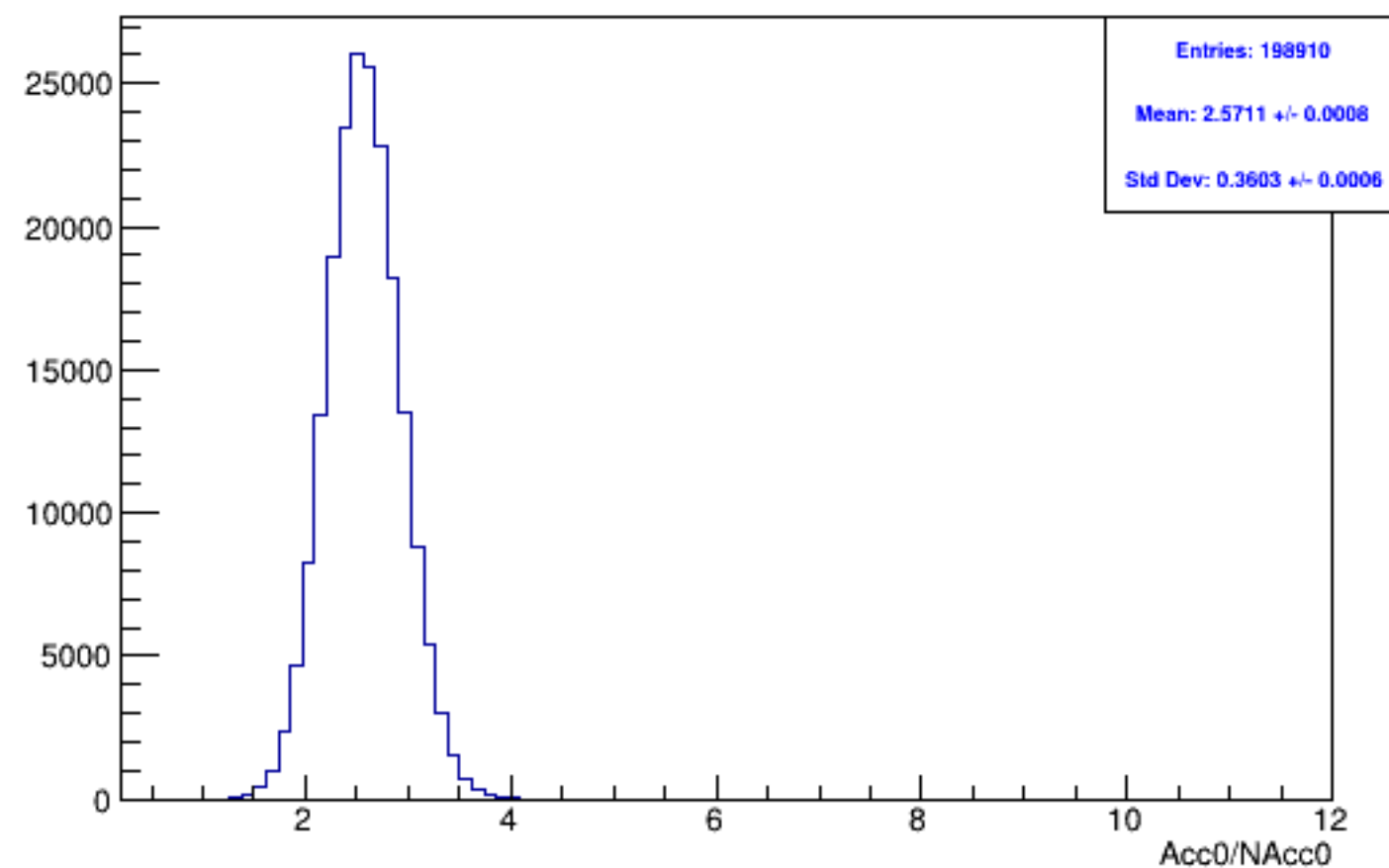
Run 5936, mpwise, acc0: Beam ON, Laser OFF
