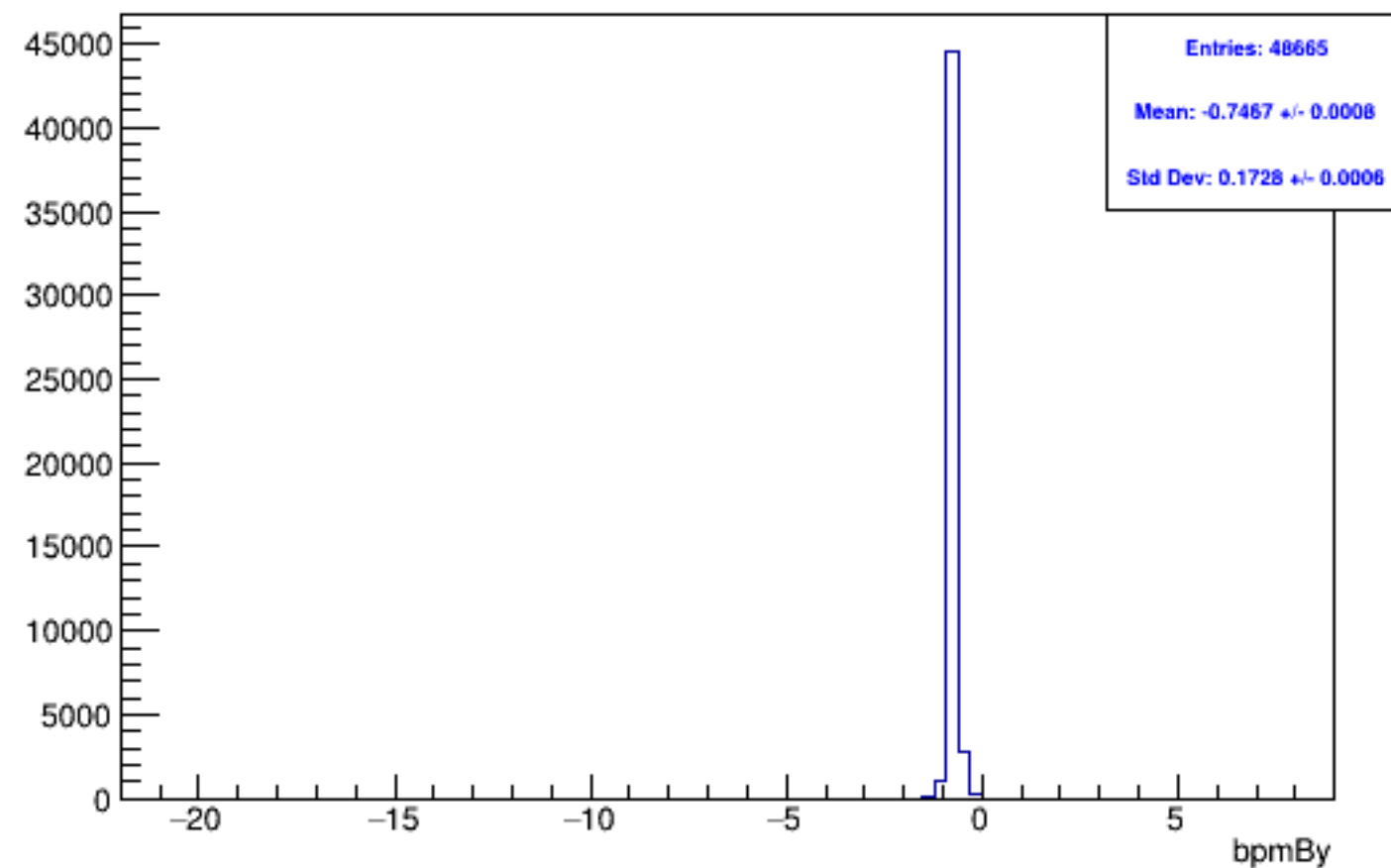
Run 5936 mpwise, bpmBy: Beam OFF
