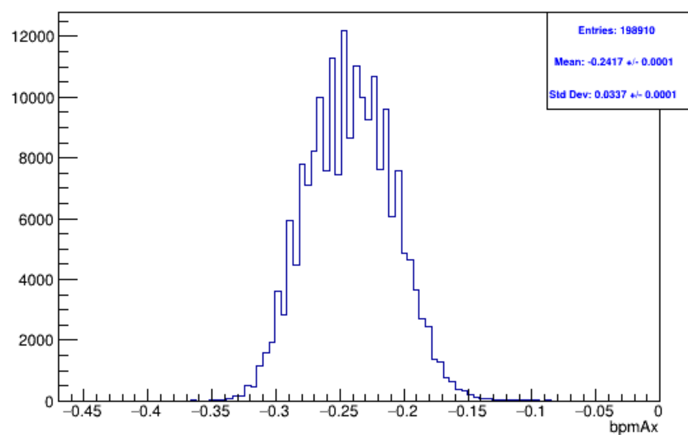
Run 5936, mpwise, bpmAx: Beam ON, Laser OFF
