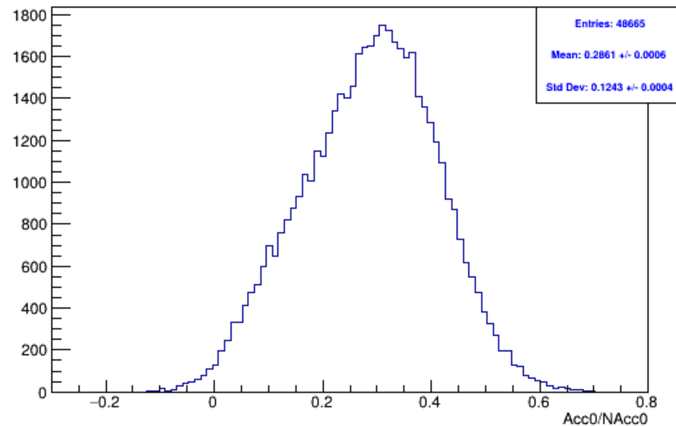
Run 5936 mpwise, acc0: Beam OFF
