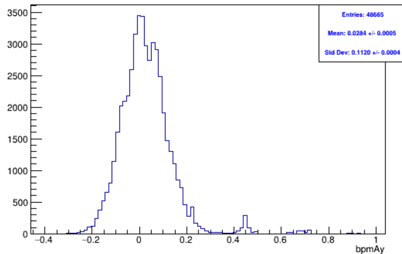
Run 5936 mpwise, bpmAy: Beam OFF
