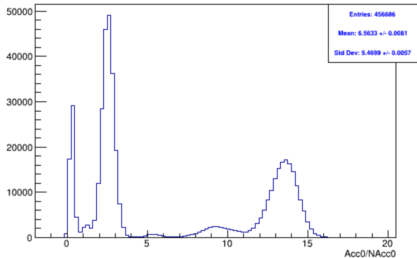
Run 5936 mpwise, acc0: All
