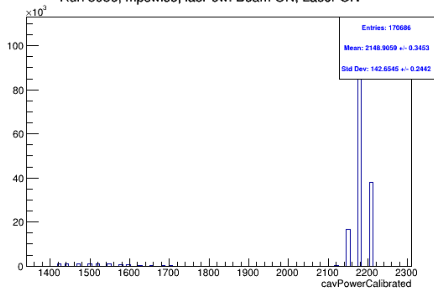
Run 5936, mpwise, lasPow: Beam ON, Laser ON
