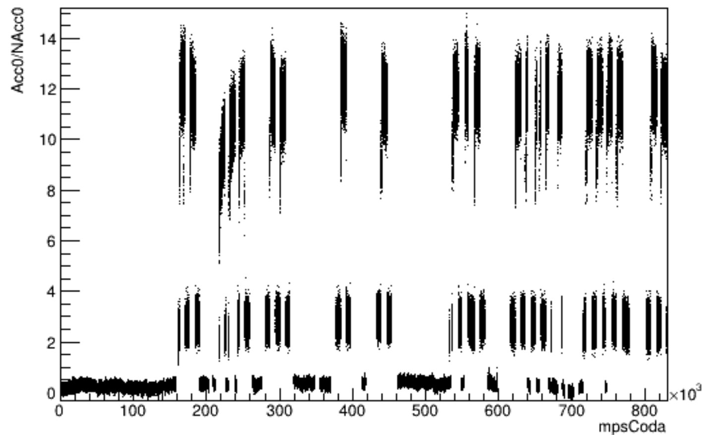
Run 5941 mpwise, Acc0 vs Time: All
