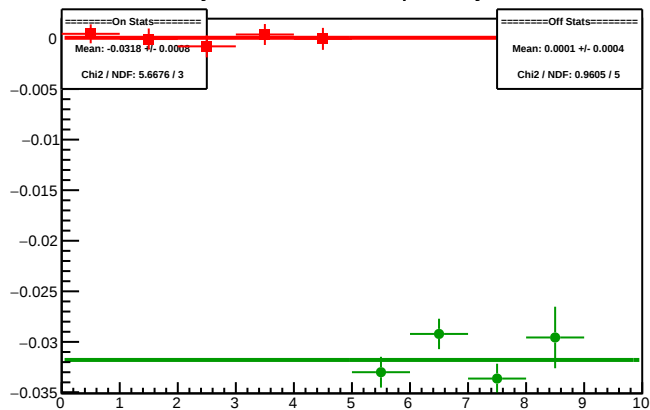
Cycle 5941.16: Multiplet Asyms
