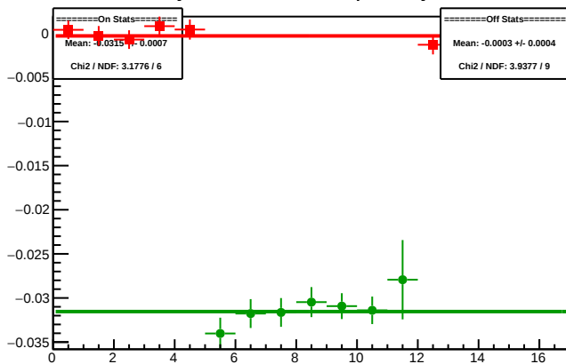
Cycle 5941.13: Multiplet Asyms
