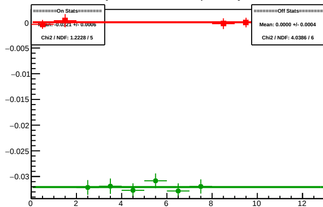
Cycle 5941.1: Multiplet Asyms
