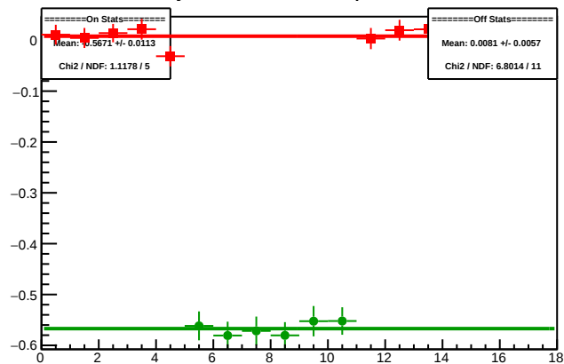
Cycle 5941.21: Multiplet Diffs
