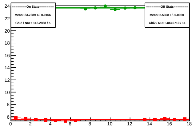
Cycle 5941.12: Multiplet Sums
