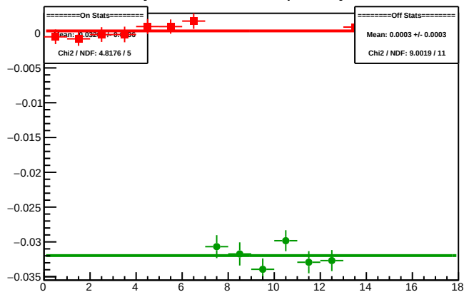
Cycle 5941.12: Multiplet Asyms
