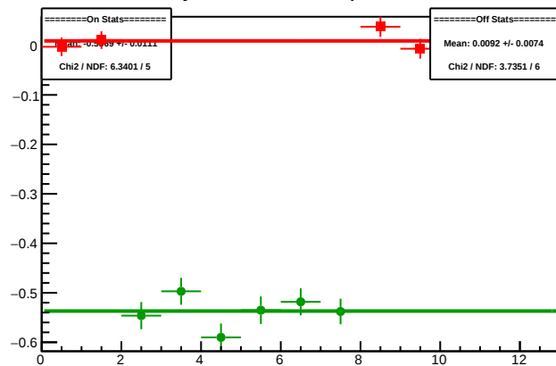
Cycle 5941.5: Multiplet Diffs
