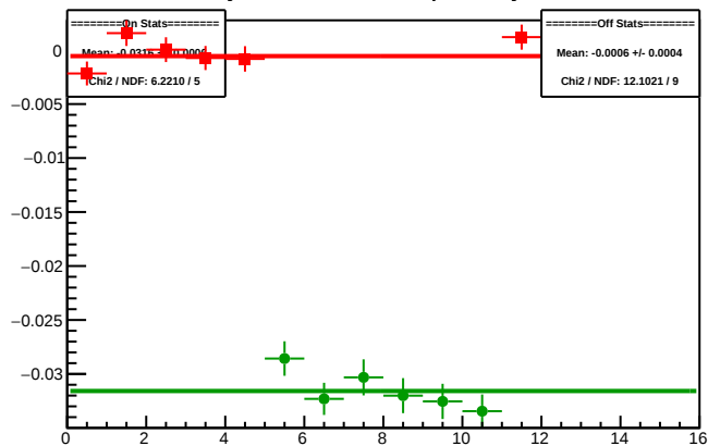
Cycle 5941.9: Multiplet Asyms
