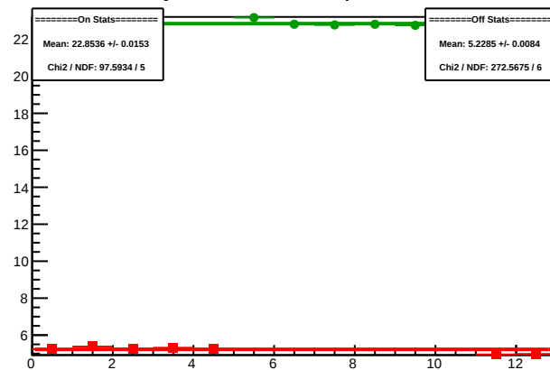
Cycle 5941.23: Multiplet Sums
