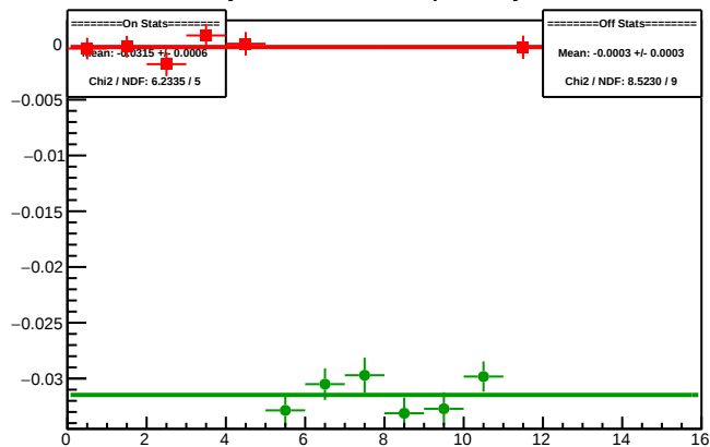
Cycle 5941.8: Multiplet Asyms
