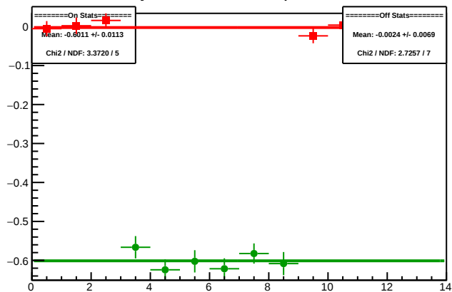
Cycle 5941.18: Multiplet Diffs
