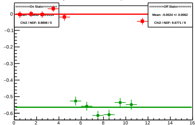
Cycle 5941.2: Multiplet Diffs
