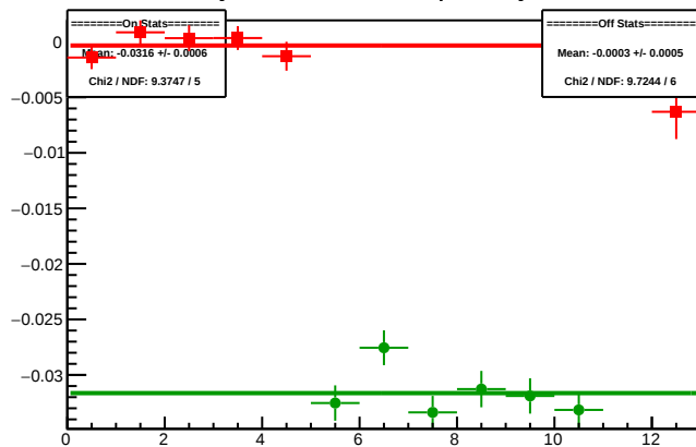
Cycle 5941.23: Multiplet Asyms
