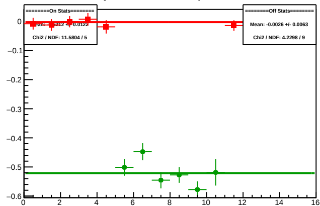
Cycle 5941.7: Multiplet Diffs
