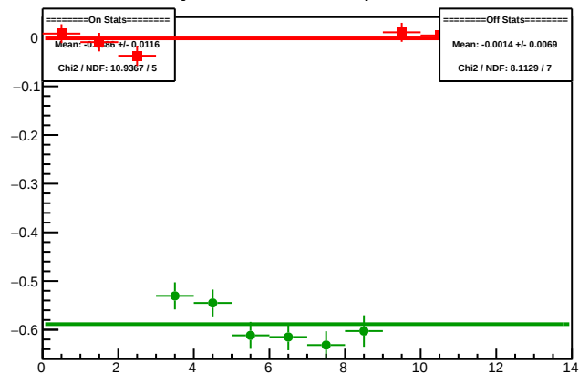
Cycle 5941.20: Multiplet Diffs
