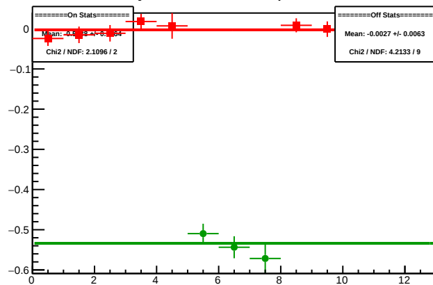
Cycle 5941.15: Multiplet Diffs
