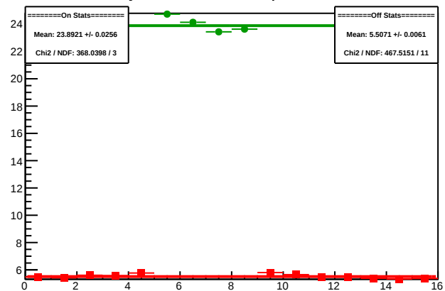
Cycle 5941.11: Multiplet Sums
