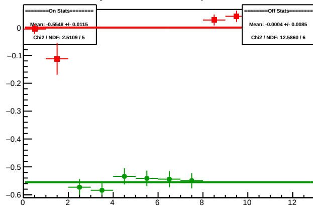
Cycle 5941.10: Multiplet Diffs
