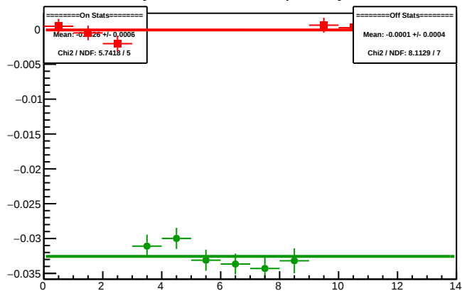
Cycle 5941.20: Multiplet Asyms
