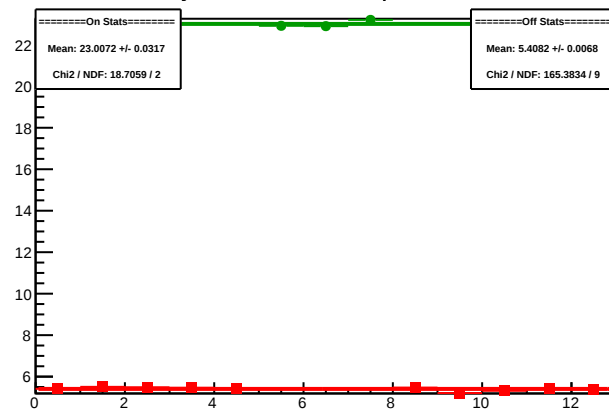
Cycle 5941.15: Multiplet Sums
