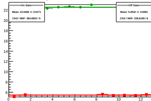
Cycle 5941.5: Multiplet Sums
