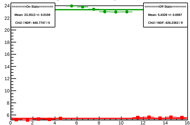
Cycle 5941.2: Multiplet Sums
