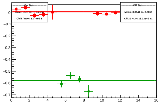
Cycle 5941.11: Multiplet Diffs
