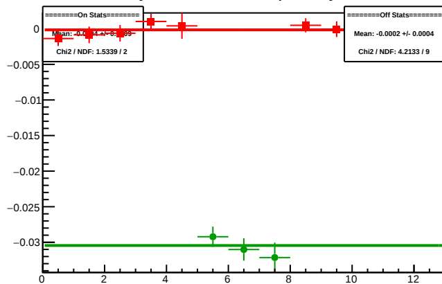
Cycle 5941.15: Multiplet Asyms
