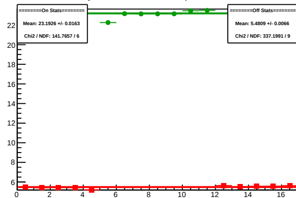
Cycle 5941.13: Multiplet Sums
