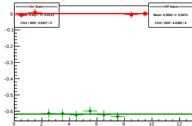
Cycle 5941.1: Multiplet Diffs
