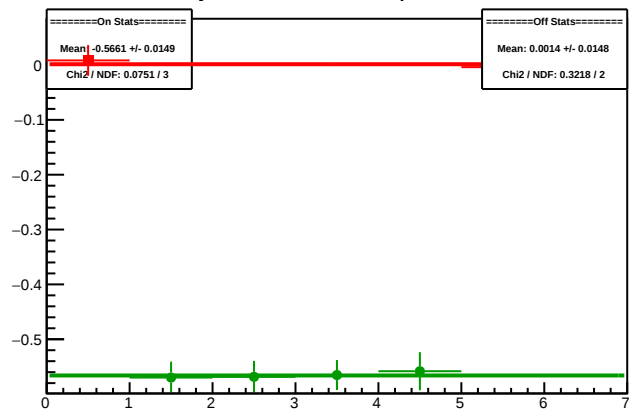
Cycle 5941.17: Multiplet Diffs
