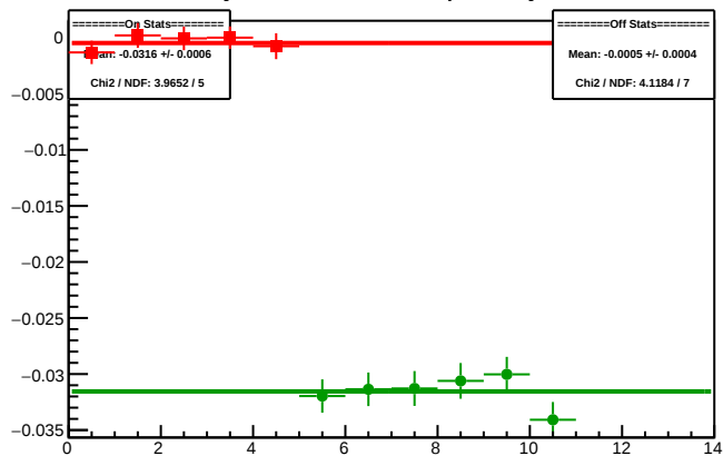
Cycle 5941.19: Multiplet Asyms
