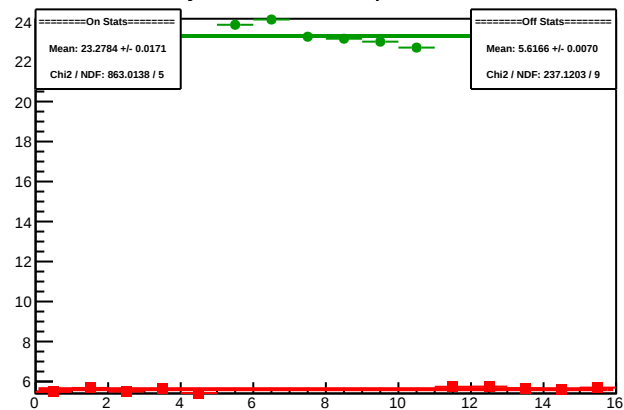
Cycle 5941.6: Multiplet Sums
