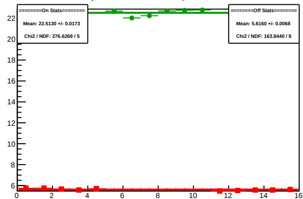
Cycle 5941.7: Multiplet Sums
