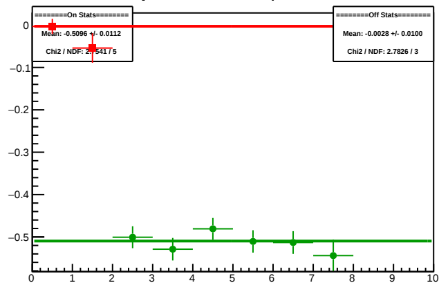
Cycle 5941.4: Multiplet Diffs
