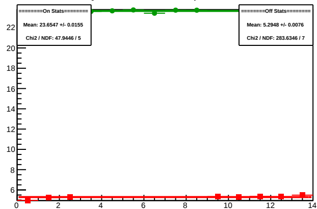
Cycle 5941.18: Multiplet Sums
