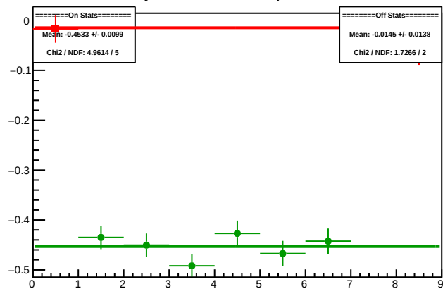
Cycle 5941.3: Multiplet Diffs
