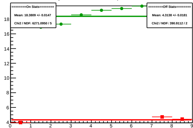
Cycle 5941.3: Multiplet Sums
