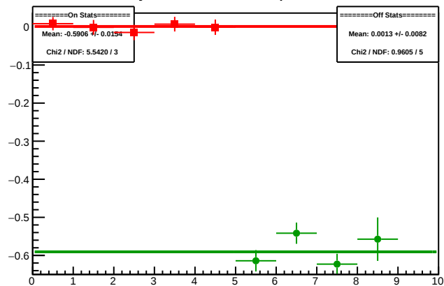
Cycle 5941.16: Multiplet Diffs
