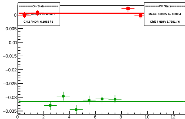
Cycle 5941.5: Multiplet Asyms
