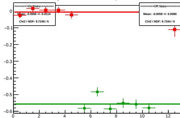
Cycle 5941.23: Multiplet Diffs
