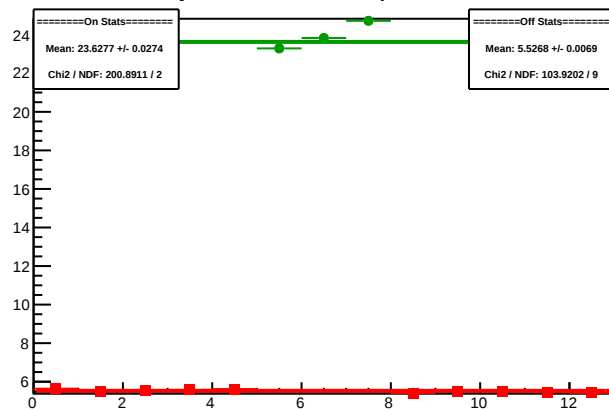
Cycle 5941.14: Multiplet Sums
