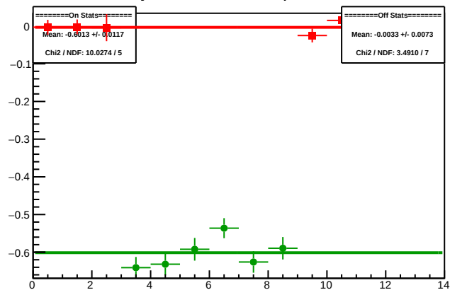
Cycle 5941.22: Multiplet Diffs
