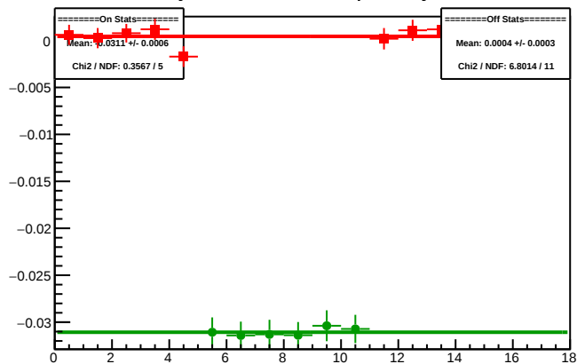
Cycle 5941.21: Multiplet Asyms
