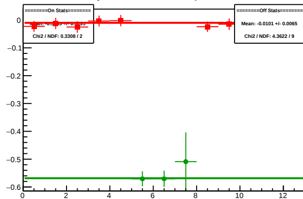
Cycle 5941.14: Multiplet Diffs
