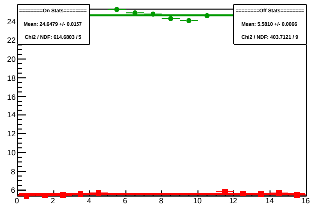
Cycle 5941.8: Multiplet Sums
