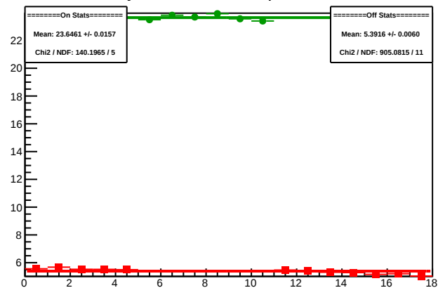
Cycle 5941.21: Multiplet Sums
