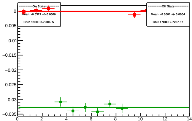
Cycle 5941.18: Multiplet Asyms
