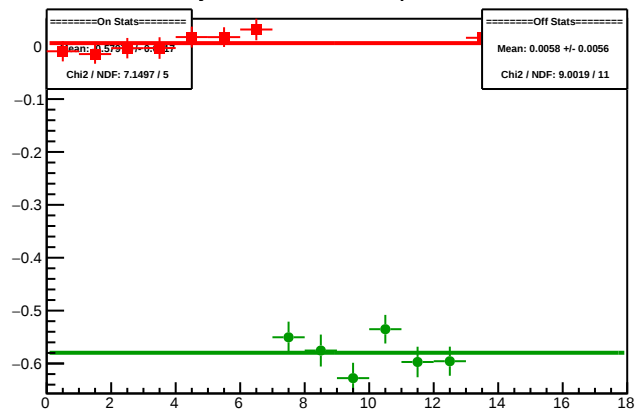
Cycle 5941.12: Multiplet Diffs
