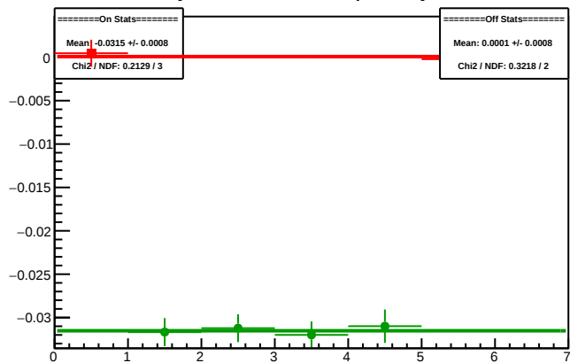
Cycle 5941.17: Multiplet Asyms
