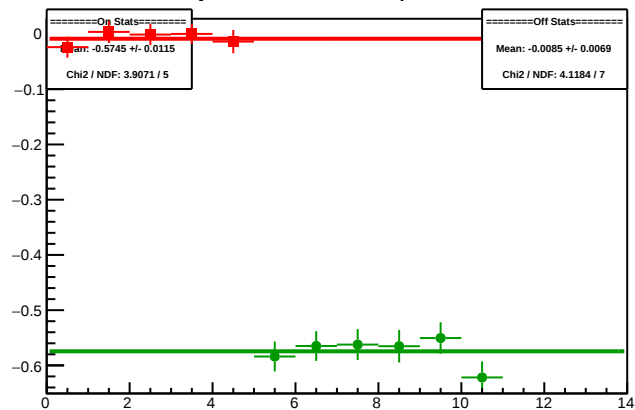
Cycle 5941.19: Multiplet Diffs
