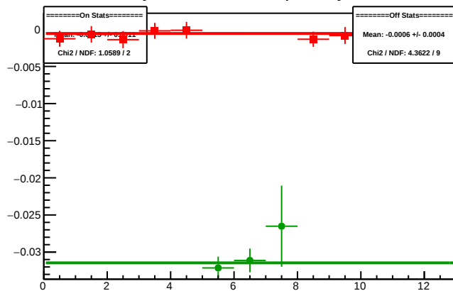
Cycle 5941.14: Multiplet Asyms
