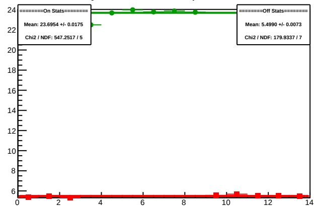
Cycle 5941.20: Multiplet Sums
