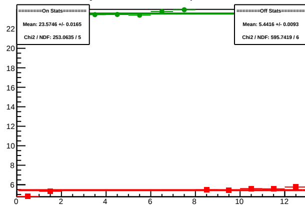
Cycle 5941.10: Multiplet Sums
