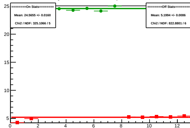
Cycle 5941.1: Multiplet Sums
