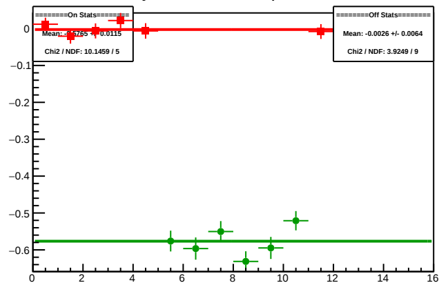
Cycle 5941.6: Multiplet Diffs
