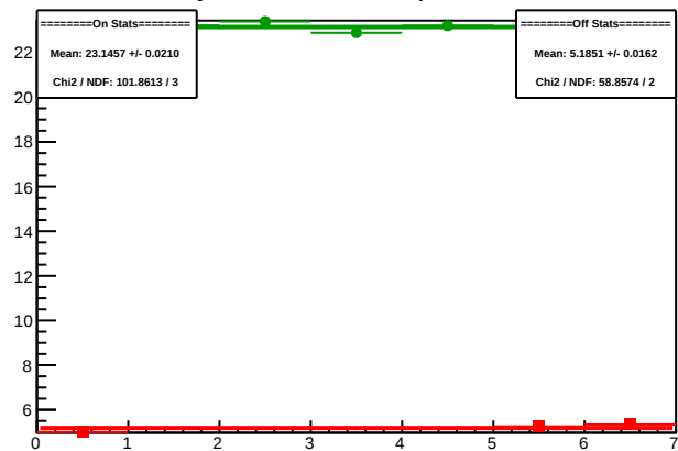
Cycle 5941.17: Multiplet Sums
