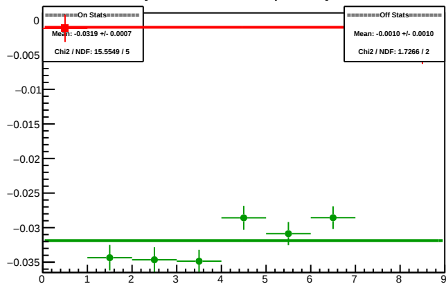
Cycle 5941.3: Multiplet Asyms
