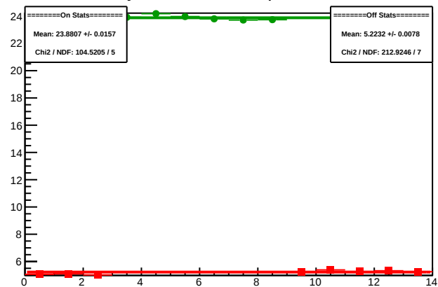
Cycle 5941.22: Multiplet Sums
