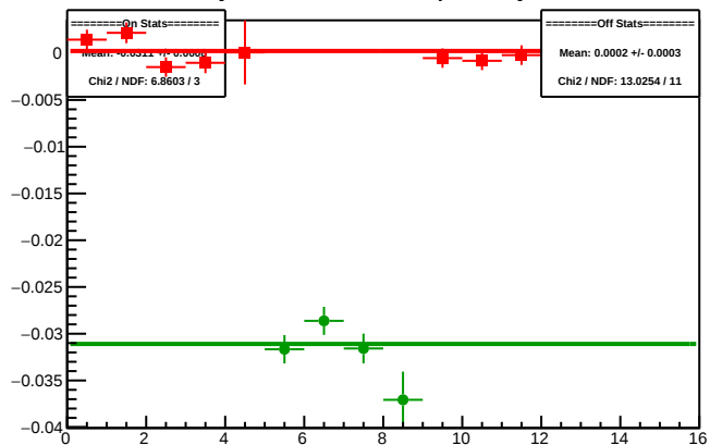
Cycle 5941.11: Multiplet Asyms
