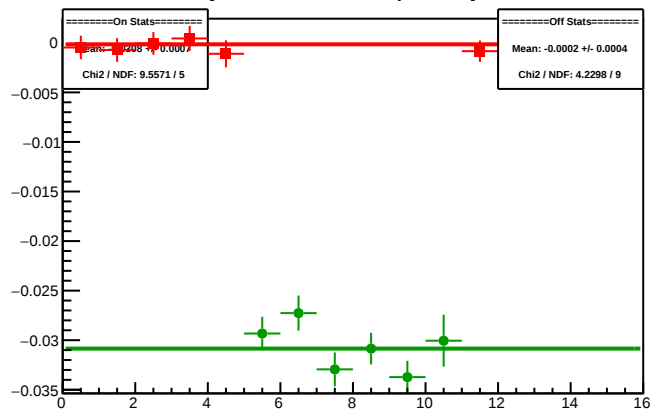
Cycle 5941.7: Multiplet Asyms
