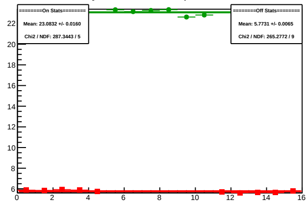
Cycle 5941.9: Multiplet Sums
