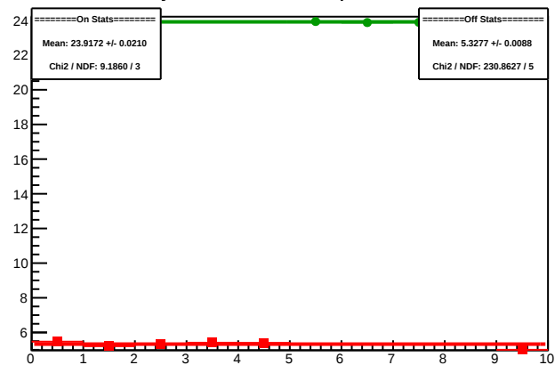
Cycle 5941.16: Multiplet Sums
