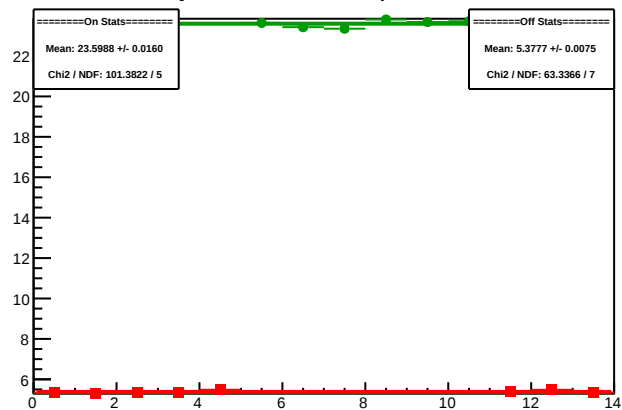
Cycle 5941.19: Multiplet Sums
