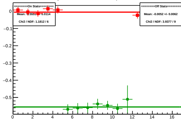
Cycle 5941.13: Multiplet Diffs
