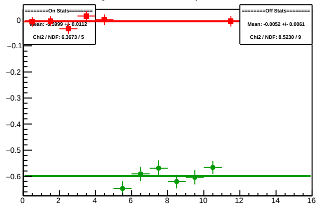
Cycle 5941.8: Multiplet Diffs
