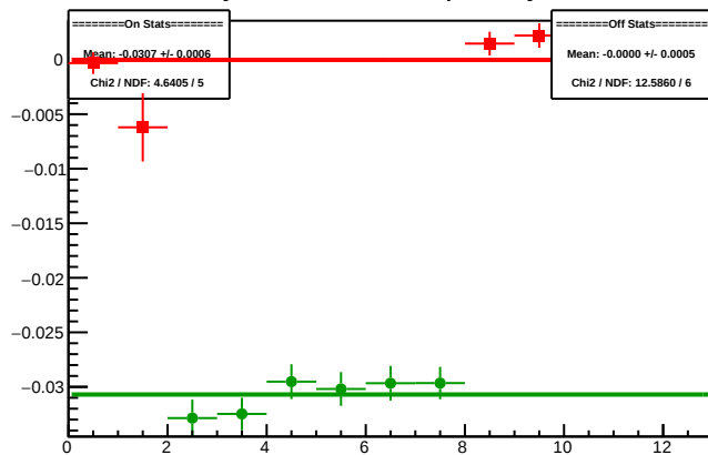
Cycle 5941.10: Multiplet Asyms
