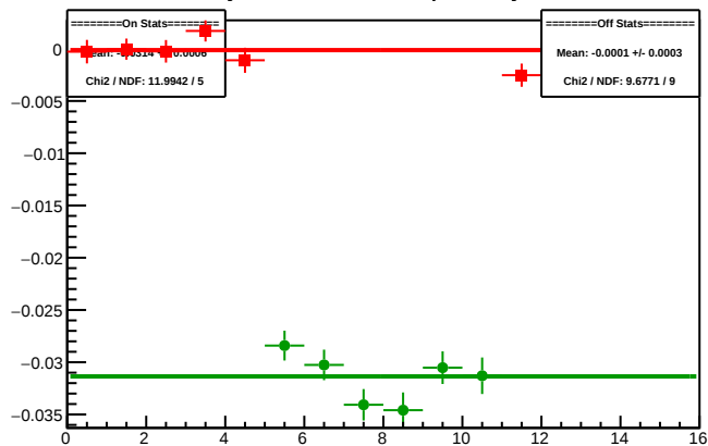
Cycle 5941.2: Multiplet Asyms
