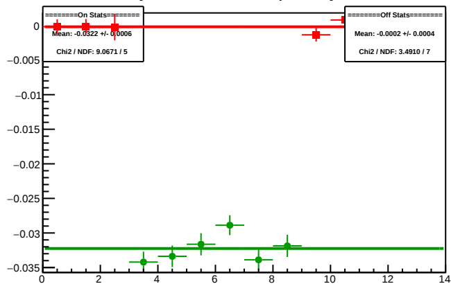
Cycle 5941.22: Multiplet Asyms
