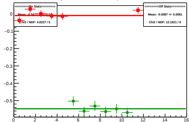
Cycle 5941.9: Multiplet Diffs
