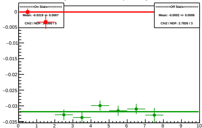
Cycle 5941.4: Multiplet Asyms
