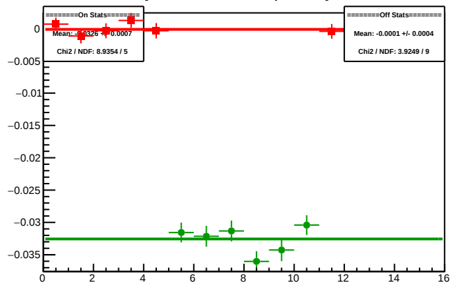
Cycle 5941.6: Multiplet Asyms
