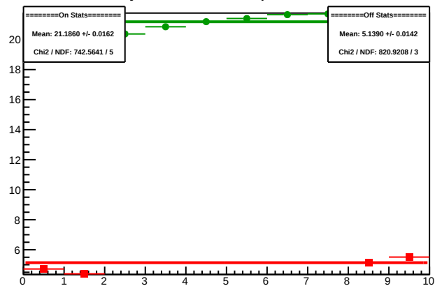
Cycle 5941.4: Multiplet Sums
