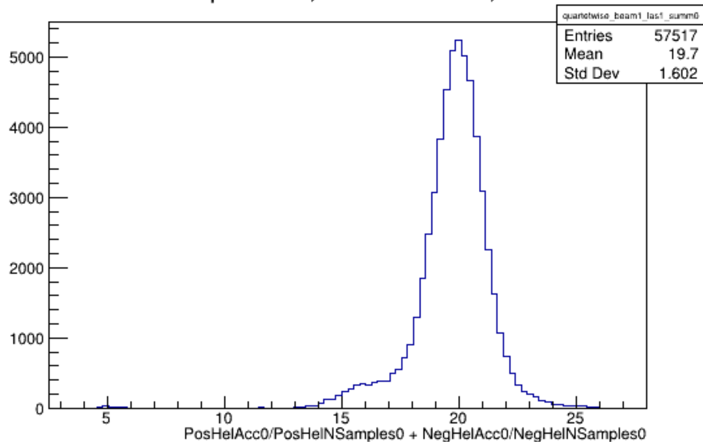
Run 5944 quartetwise, Sums0: Beam ON, Laser ON
