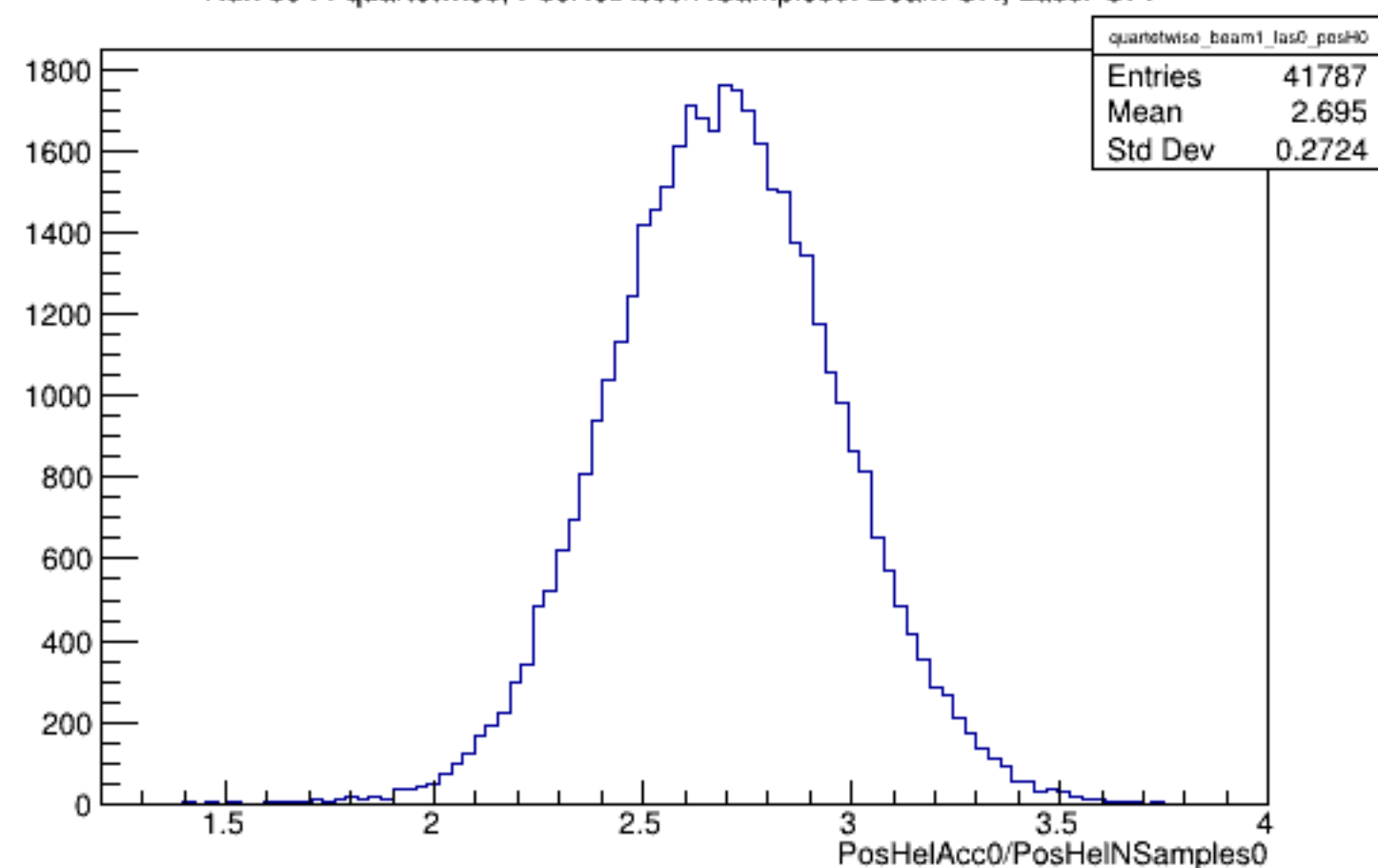
Run 5944 quartetwise, PosHelAcc0/NSamples0: Beam ON, Laser OFF
