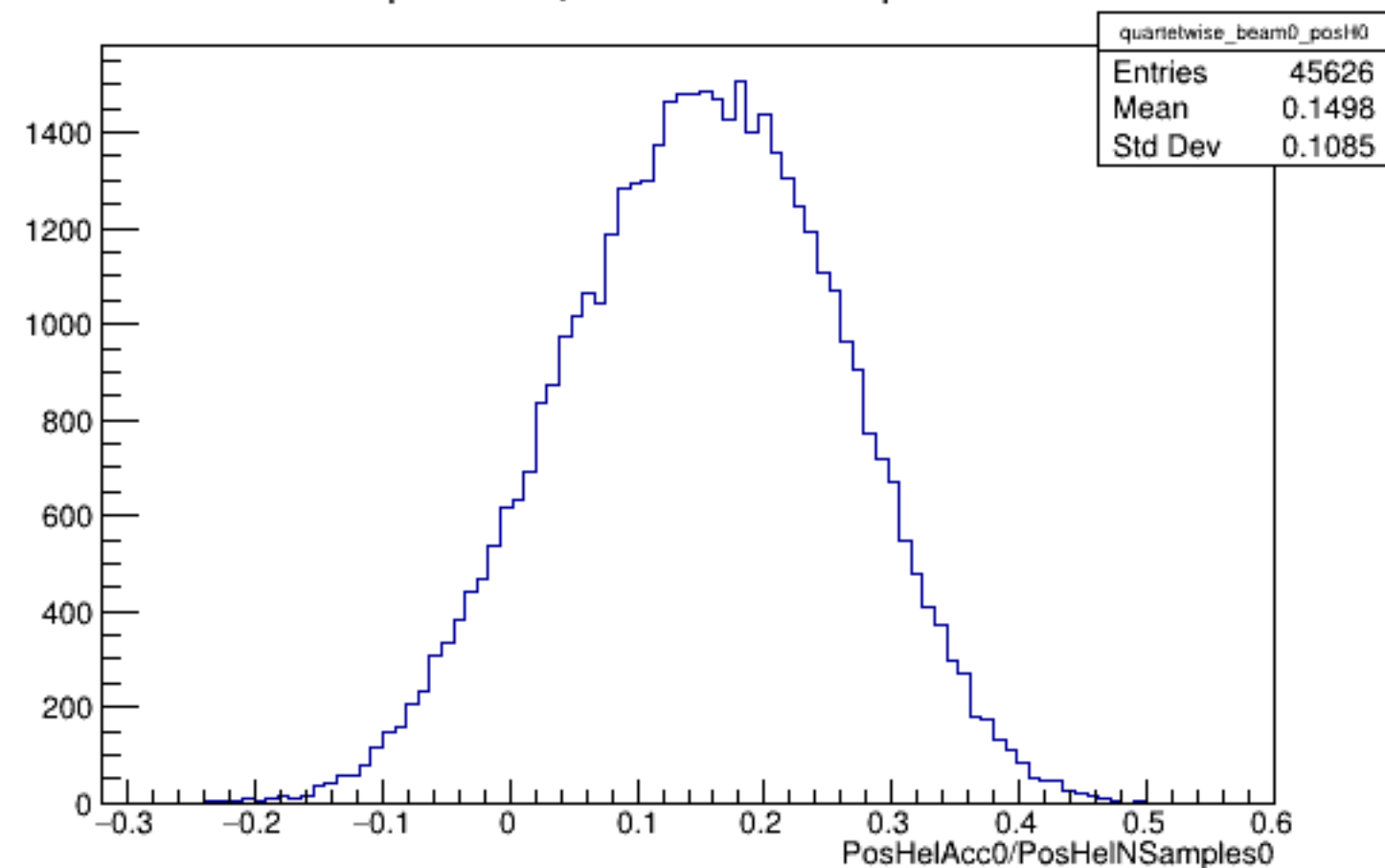
Run 5944 quartetwise, PosHelAcc0/NSamples0: Beam OFF
