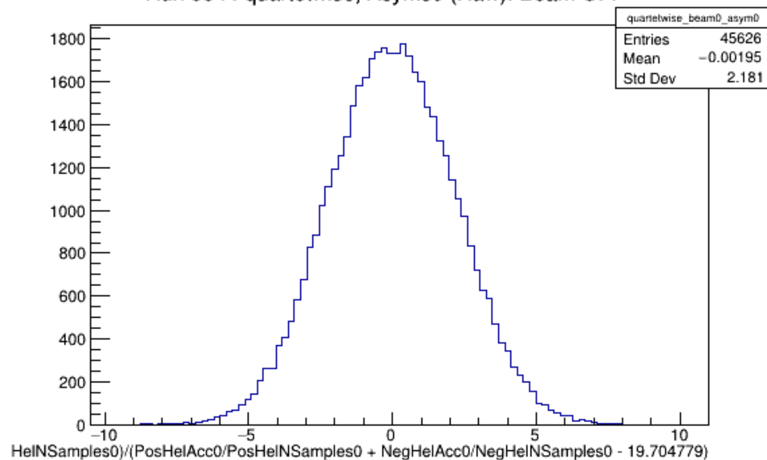
Run 5944 quartetwise, Asyms0 (Raw): Beam OFF
