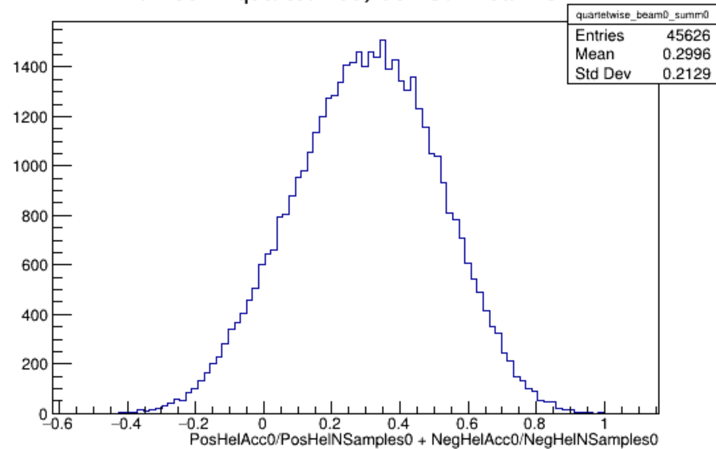
Run 5944 quartetwise, Sums0: Beam OFF
