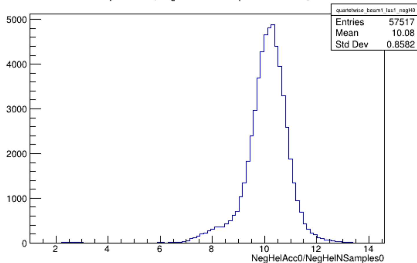
Run 5944 quartetwise, NegHelAcc0/NSamples0: Beam ON, Laser ON
