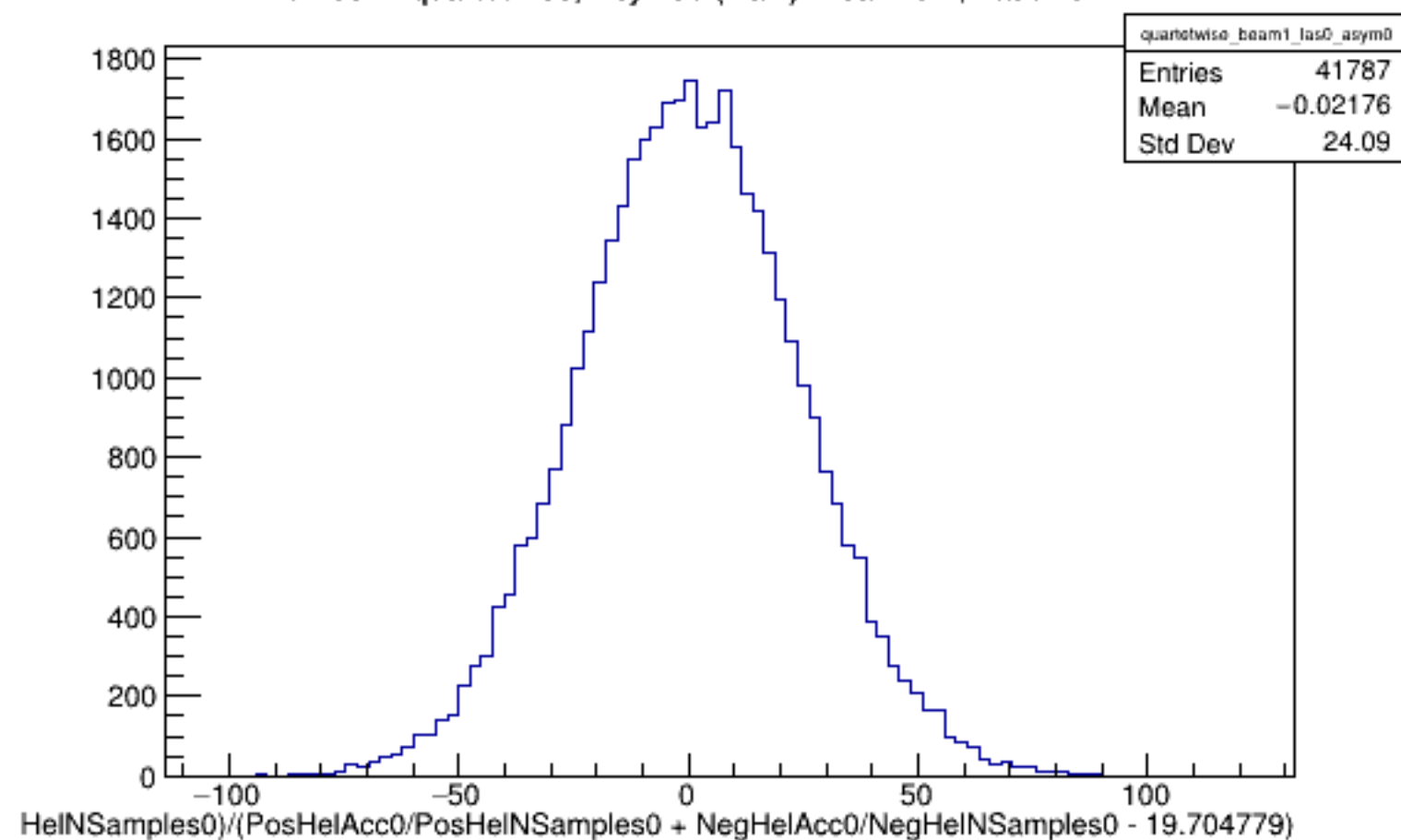
Run 5944 quartetwise, Asyms0 (Raw): Beam ON, Laser OFF
