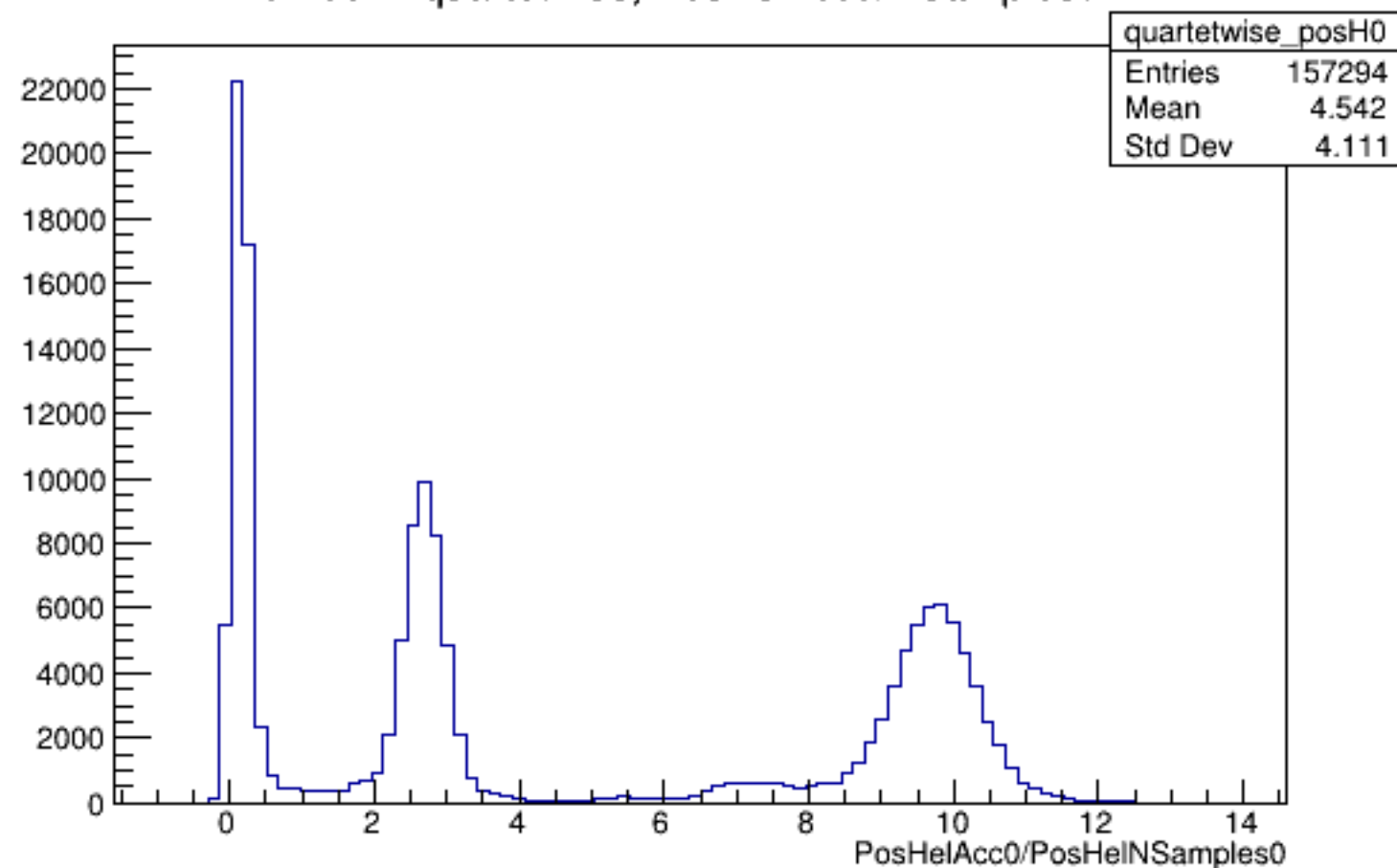
Run 5944 quartetwise, PosHelAcc0/NSamples0: All
