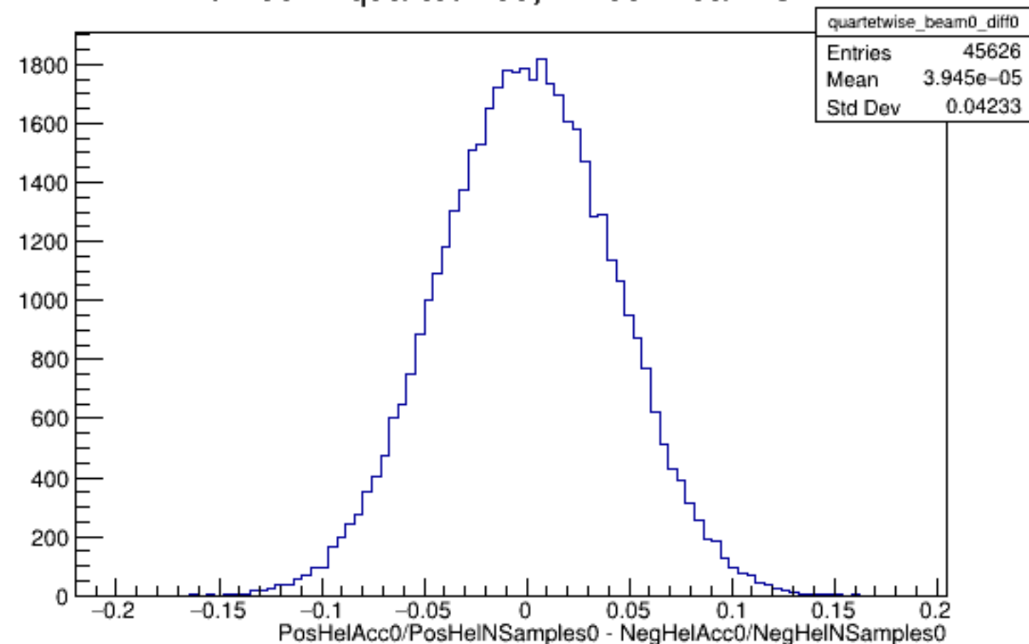
Run 5944 quartetwise, Diffs0: Beam OFF
