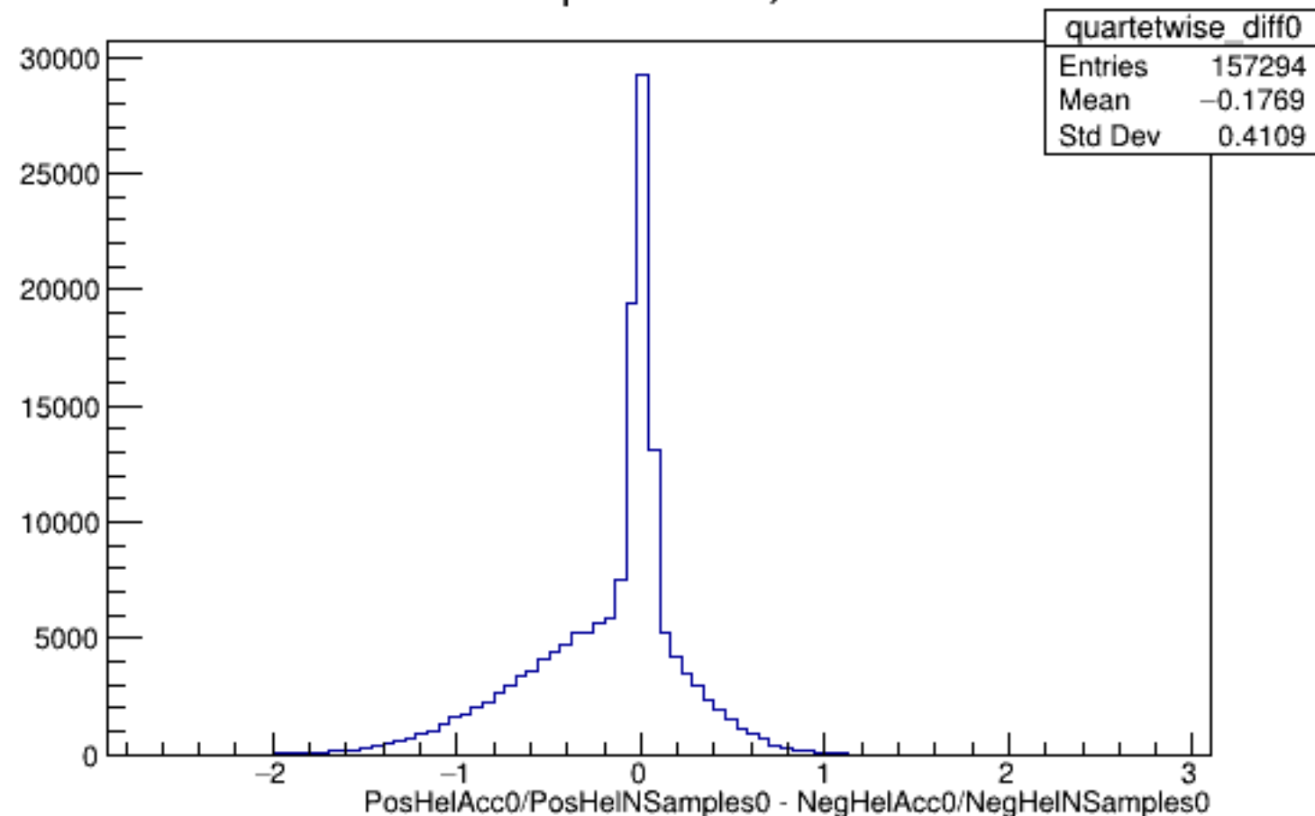
Run 5944 quartetwise, Diffs0: All
