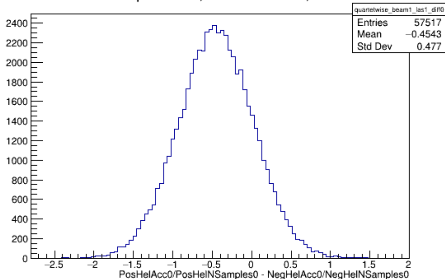
Run 5944 quartetwise, Diffs0: Beam ON, Laser ON
