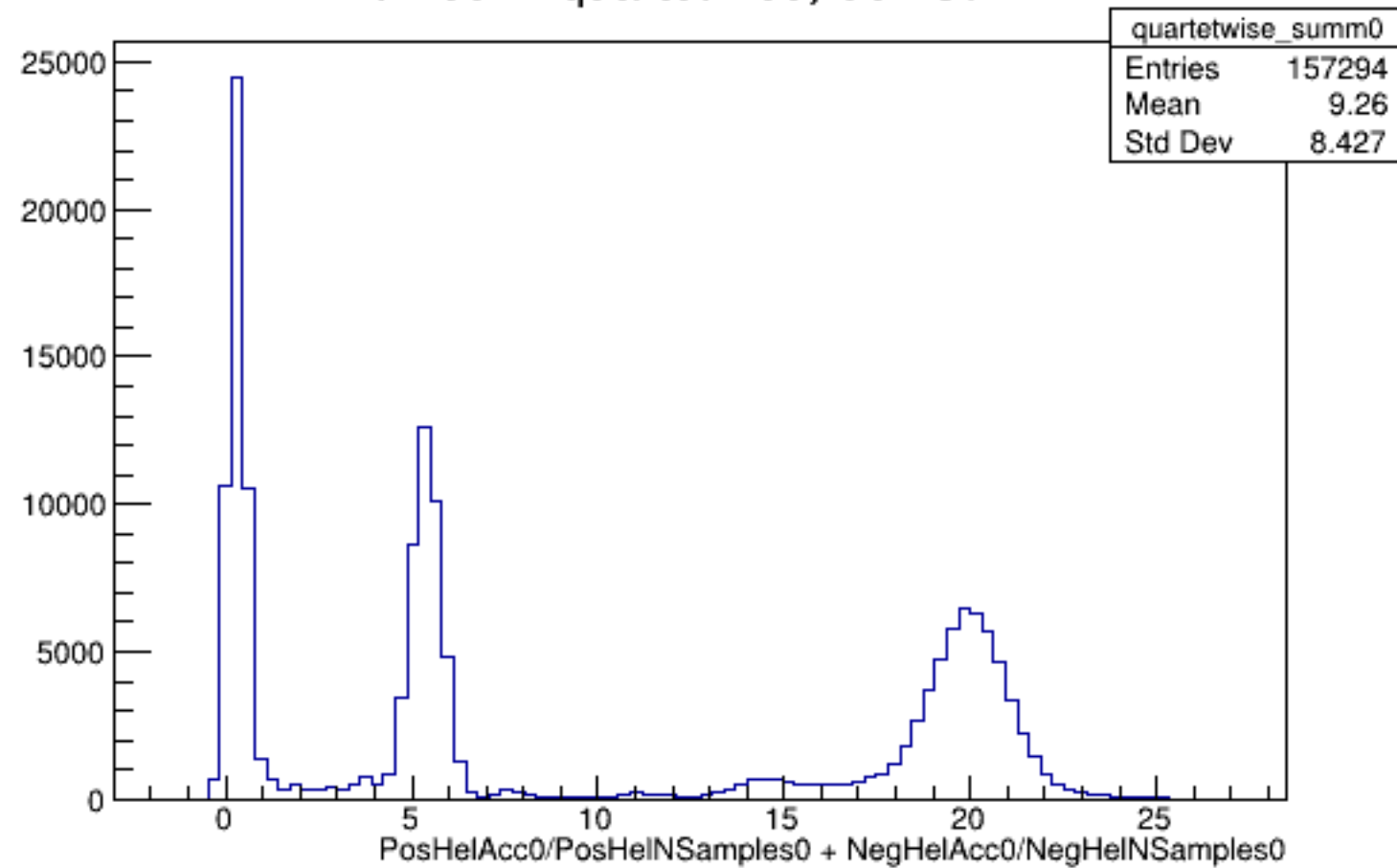
Run 5944 quartetwise, Sums0: All
