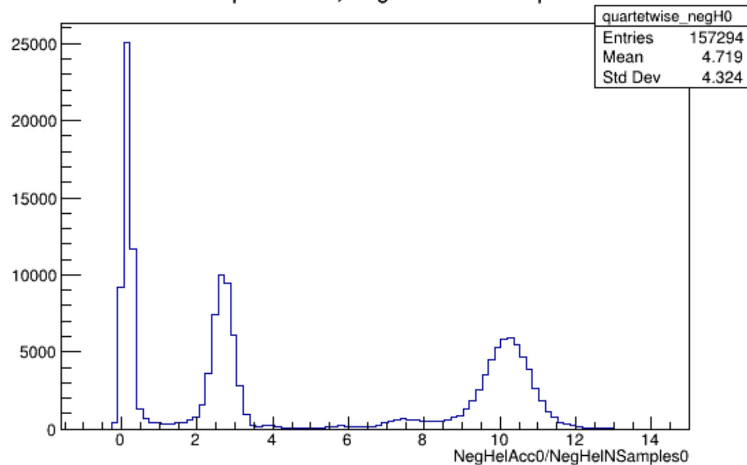
Run 5944 quartetwise, NegHelAcc0/NSamples0: All
