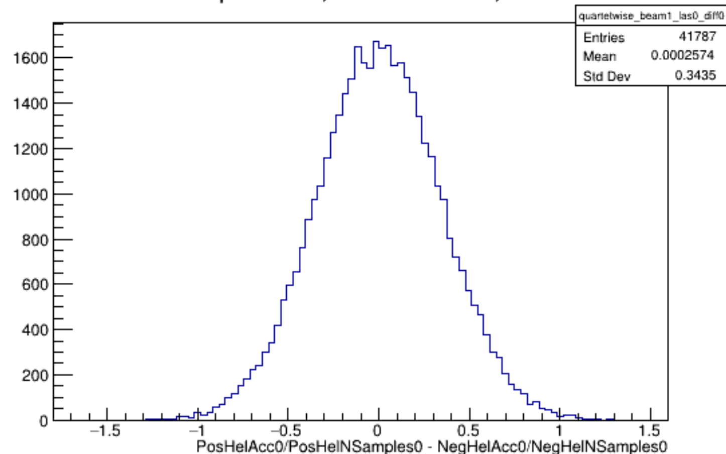
Run 5944 quartetwise, Diffs0: Beam ON, Laser OFF
