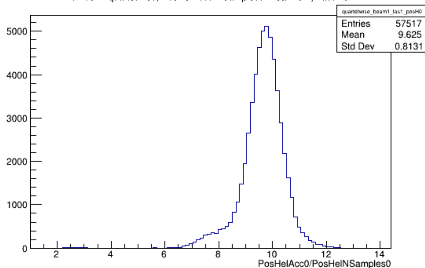
Run 5944 quartetwise, PosHelAcc0/NSamples0: Beam ON, Laser ON
