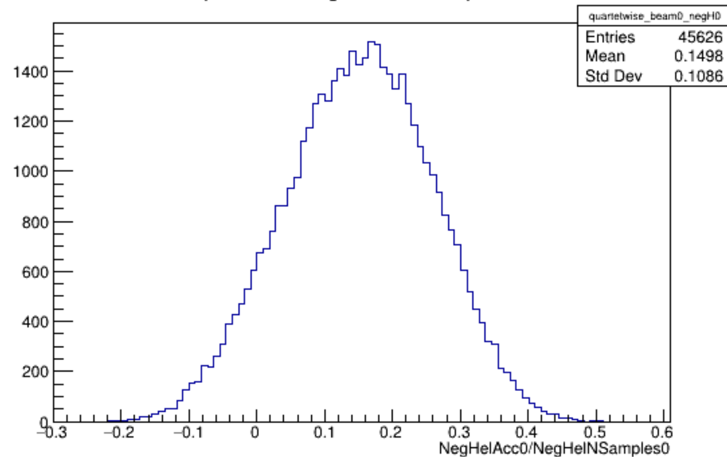
Run 5944 quartetwise, NegHelAcc0/NSamples0: Beam OFF
