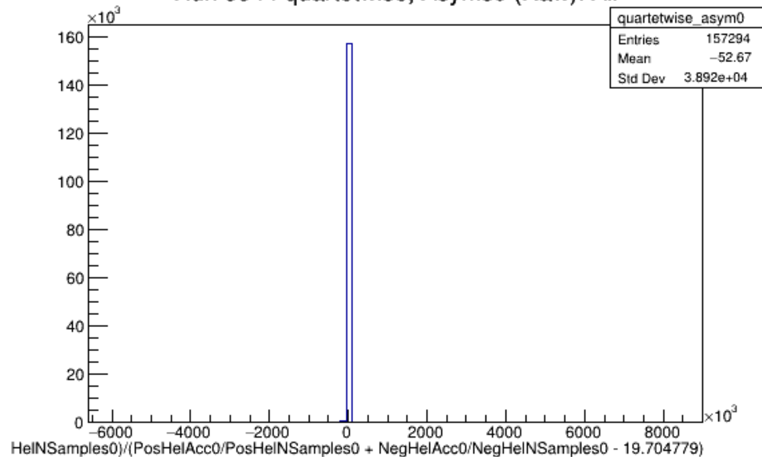
Run 5944 quartetwise, Asyms0 (Raw): All
