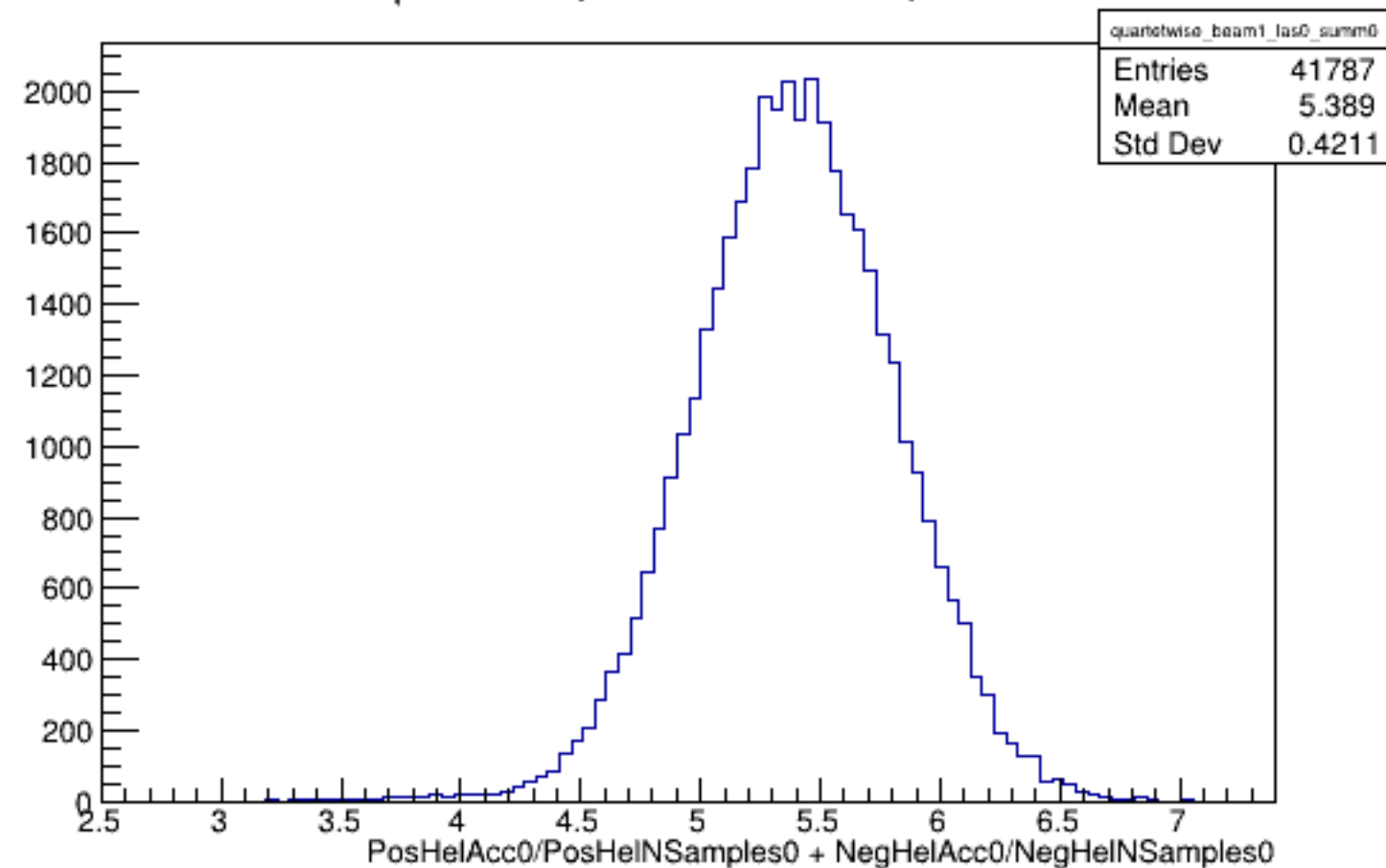
Run 5944 quartetwise, Sums0: Beam ON, Laser OFF
