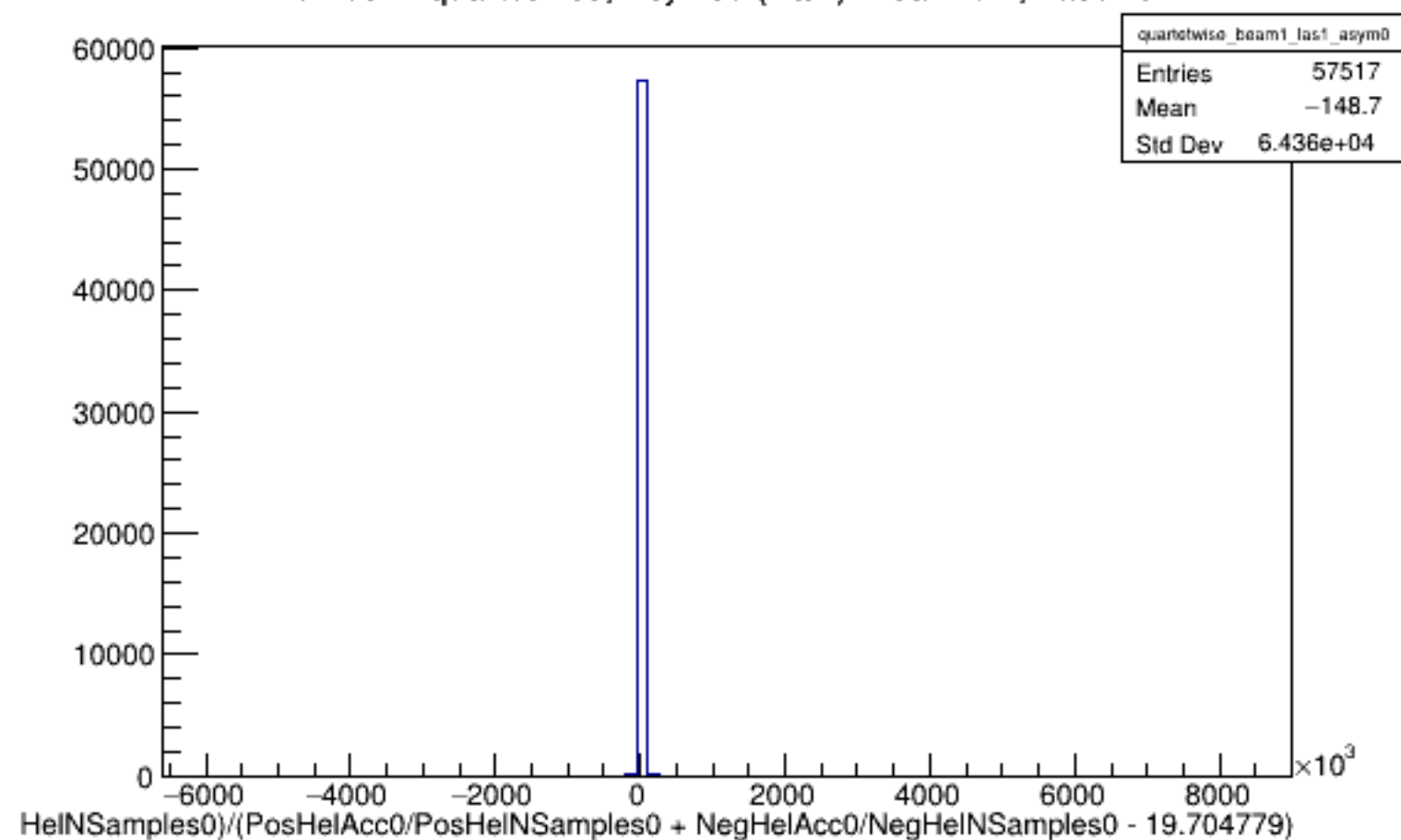
Run 5944 quartetwise, Asyms0 (Raw): Beam ON, Laser ON
