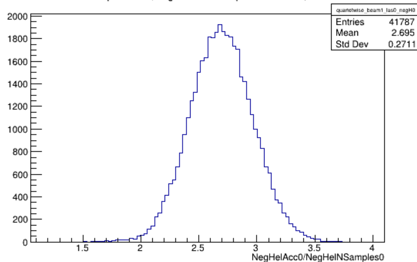
Run 5944 quartetwise, NegHelAcc0/NSamples0: Beam ON, Laser OFF
