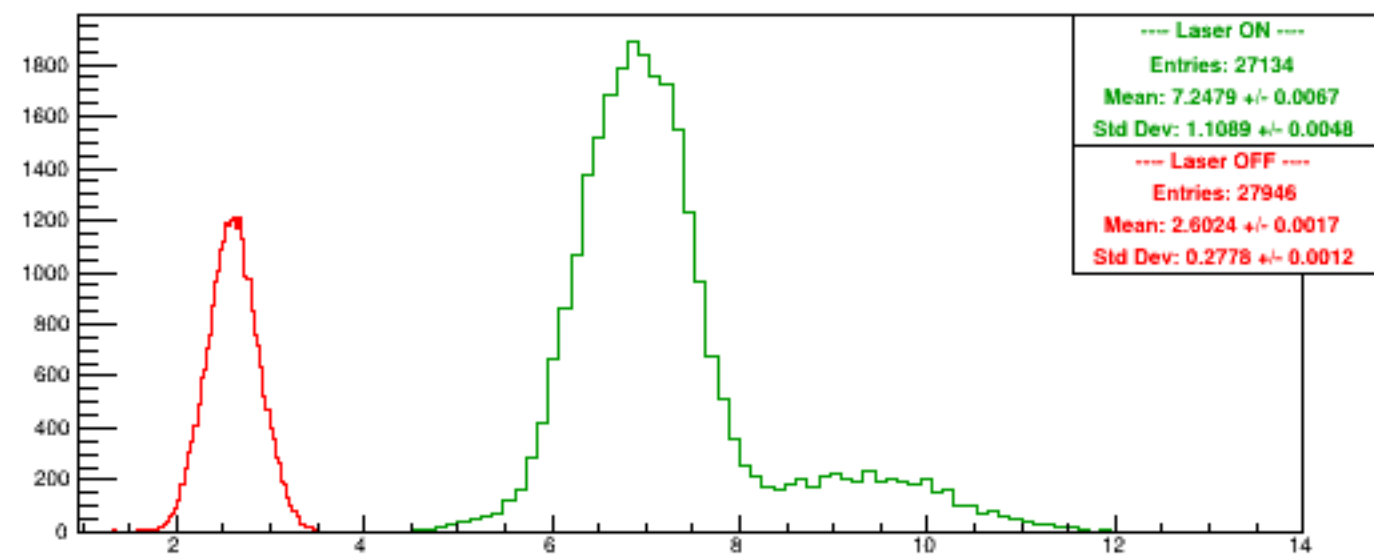
Run 5945 quartetwise, PosHelAcc0/NSamples0
