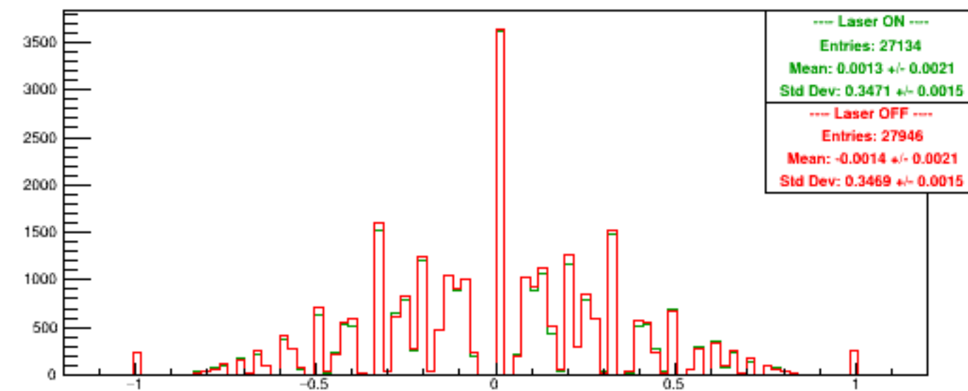
Run 5945 quartetwise, Asyms USbg2
