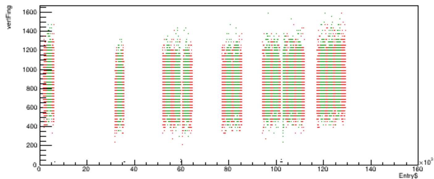
Run 5945 quartetwise, vertFing vs time
