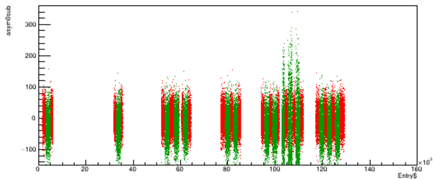
Run 5945 quartetwise, asym0sub vs time
