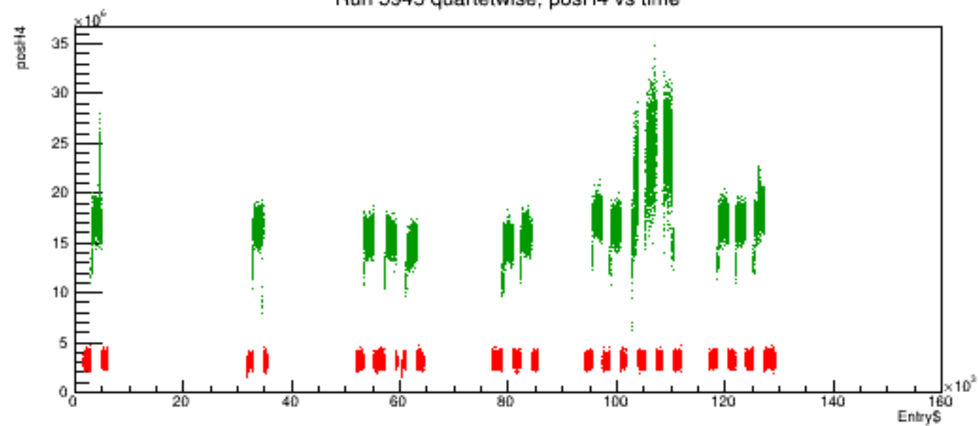
Run 5945 quartetwise, posH4 vs time
