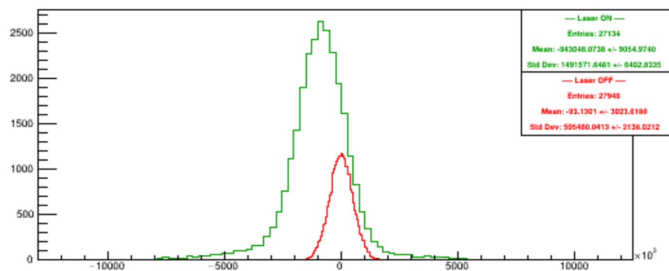
Run 5945 quartetwise, Diffs4
