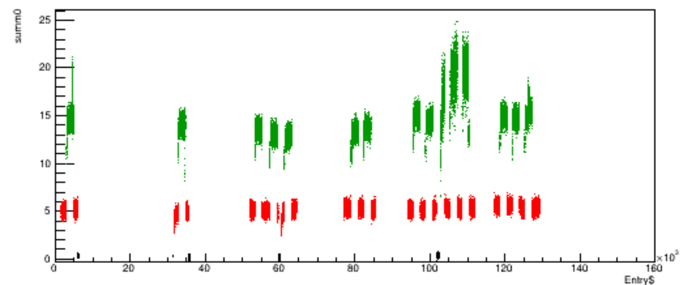
Run 5945 quartetwise, summ0 vs time
