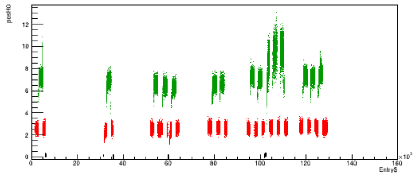
Run 5945 quartetwise, posH0 vs time
