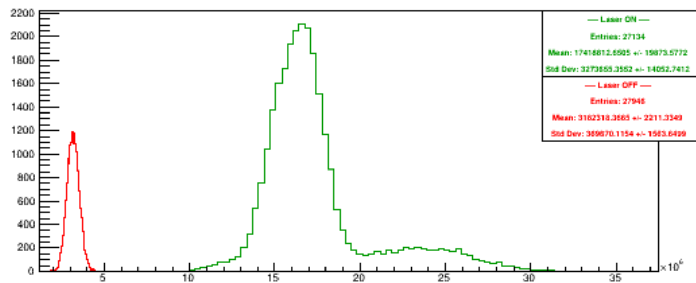
Run 5945 quartetwise, PosHelAcc4
