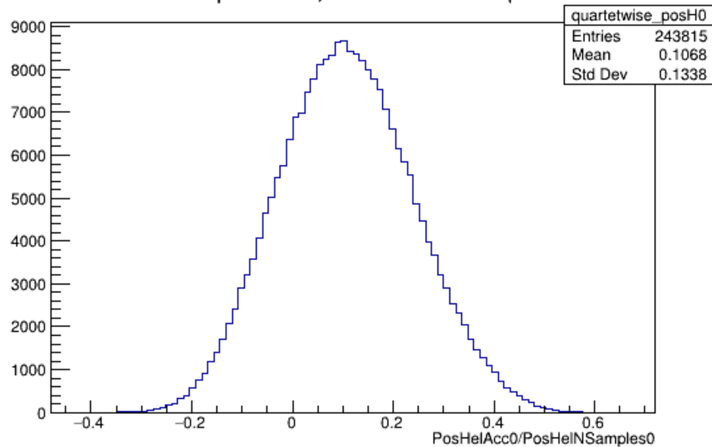
Run 5947 quartetwise, PosHelAcc0/NSamples0: All
