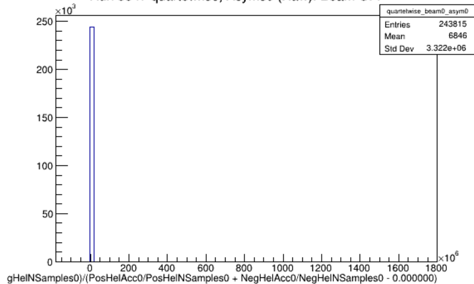
Run 5947 quartetwise, Asyms0 (Raw): Beam OFF
