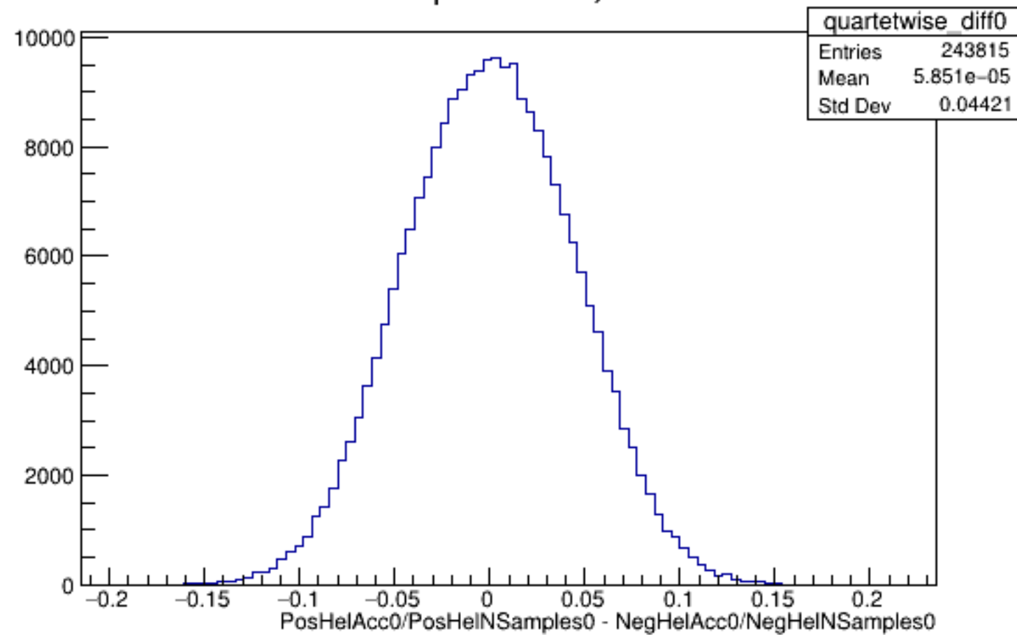
Run 5947 quartetwise, Diffs0: All
