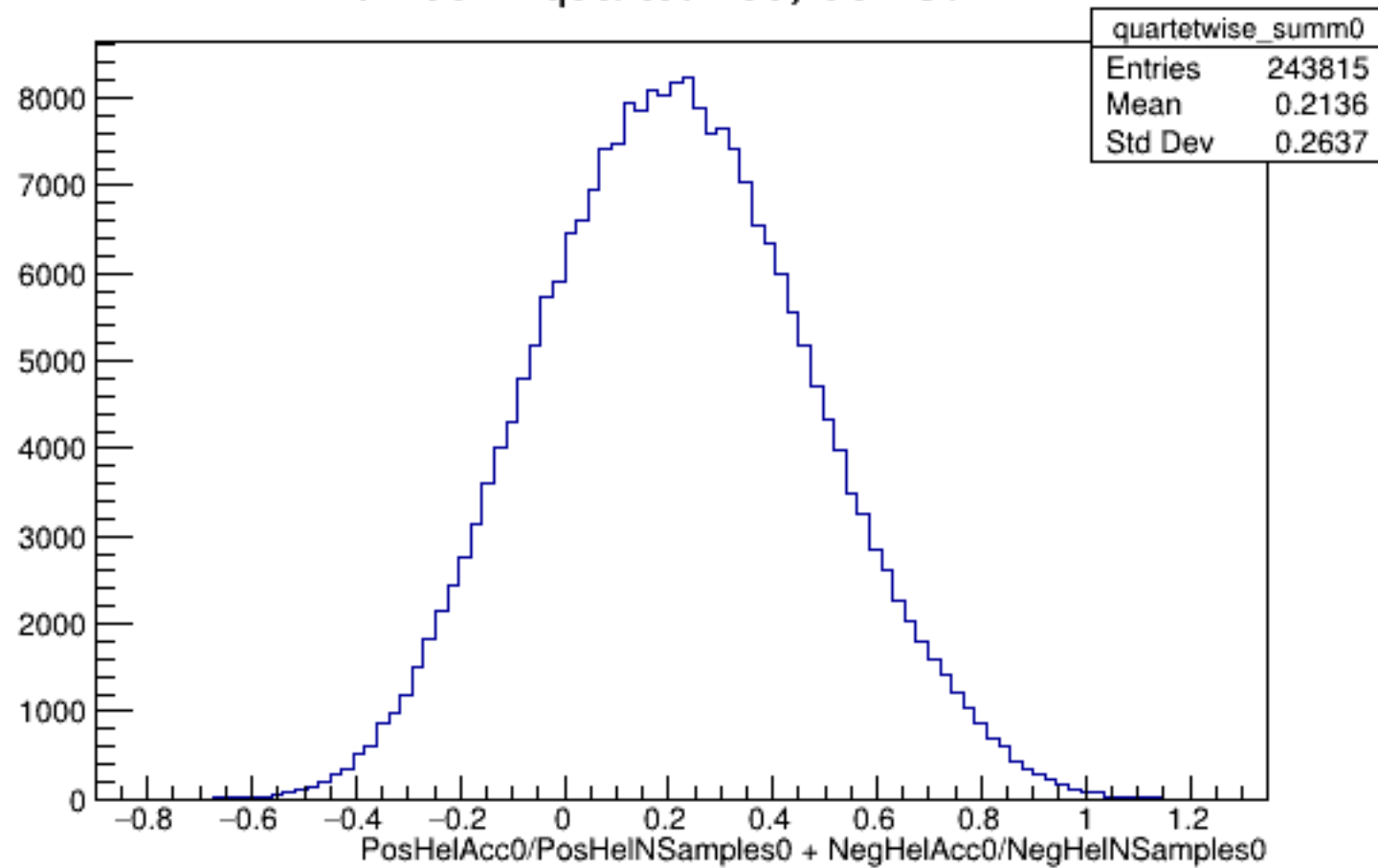
Run 5947 quartetwise, Sums0: All
