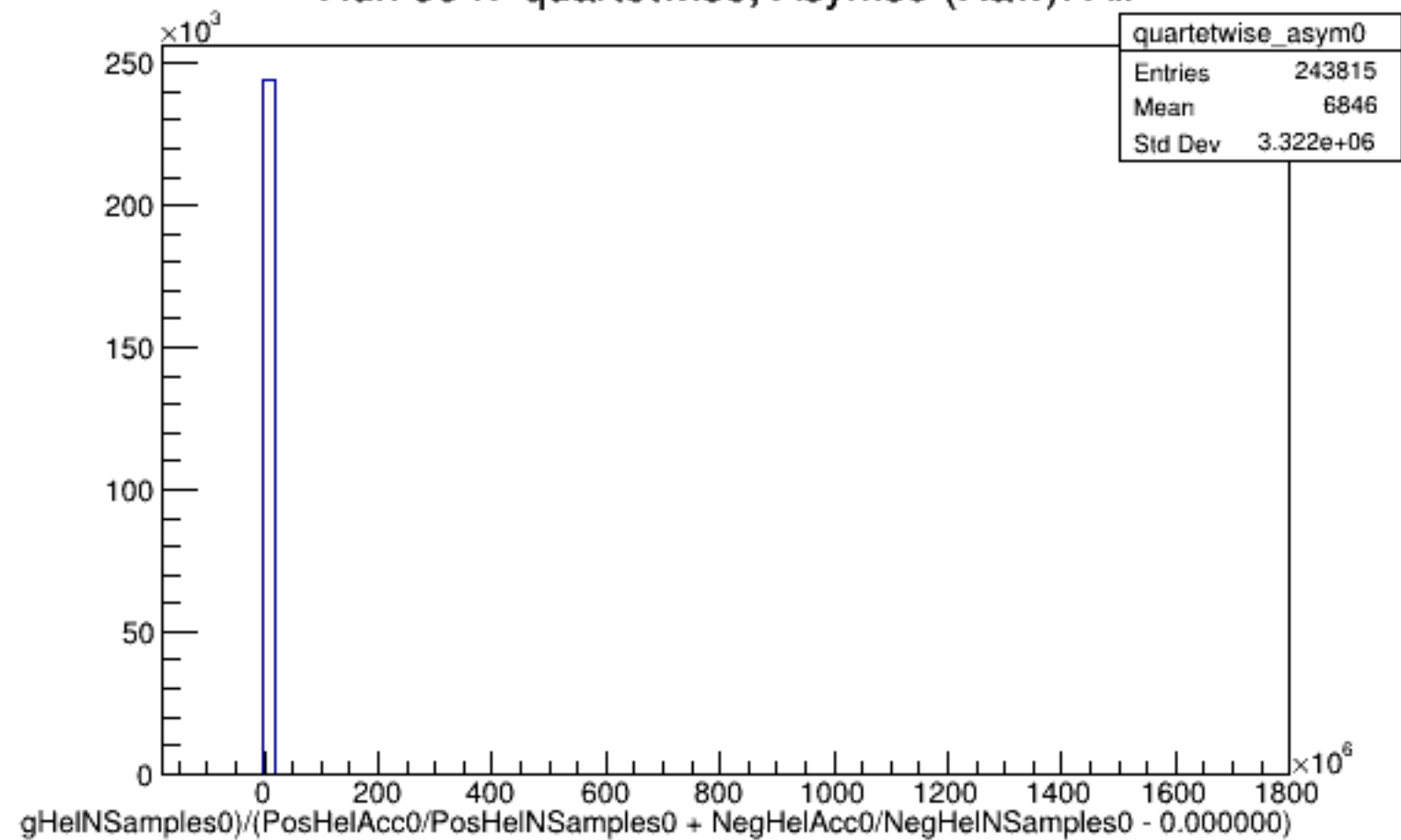
Run 5947 quartetwise, Asyms0 (Raw): All
