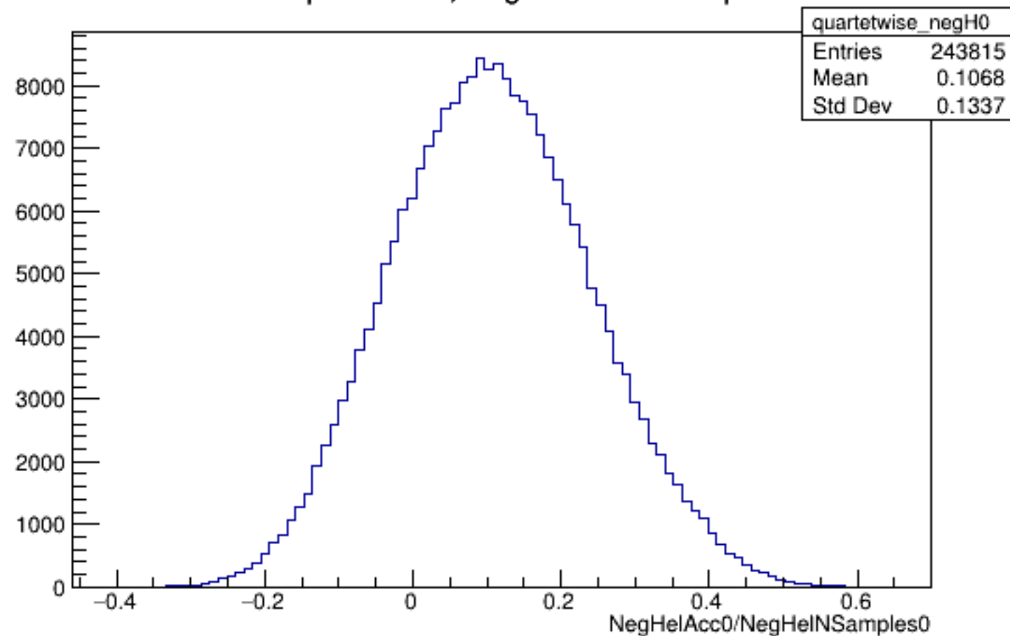
Run 5947 quartetwise, NegHelAcc0/NSamples0: All
