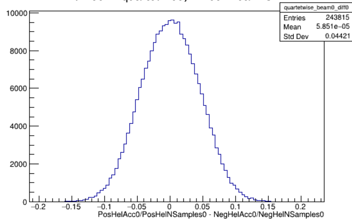
Run 5947 quartetwise, Diffs0: Beam OFF
