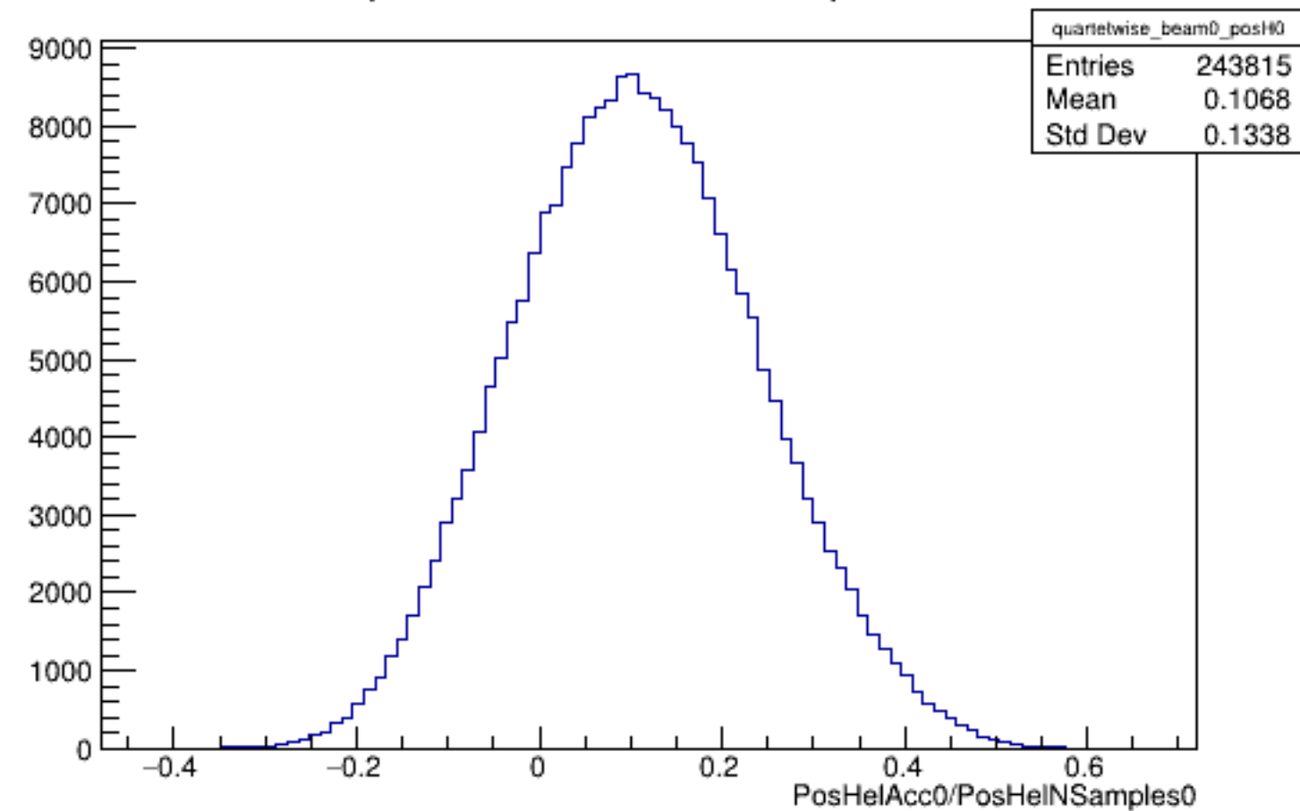
Run 5947 quartetwise, PosHelAcc0/NSamples0: Beam OFF
