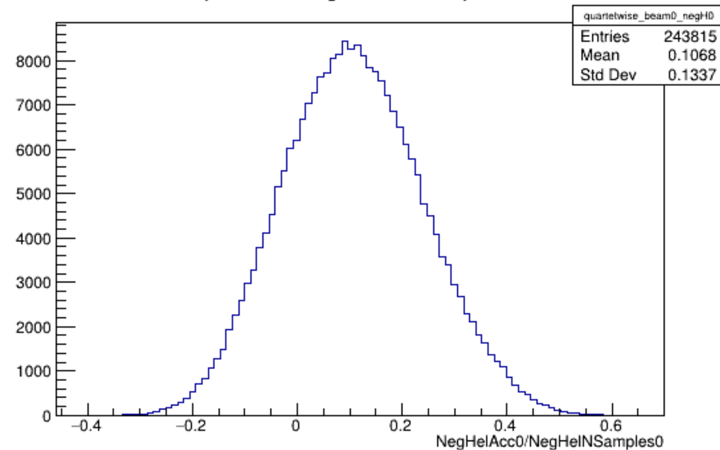
Run 5947 quartetwise, NegHelAcc0/NSamples0: Beam OFF
