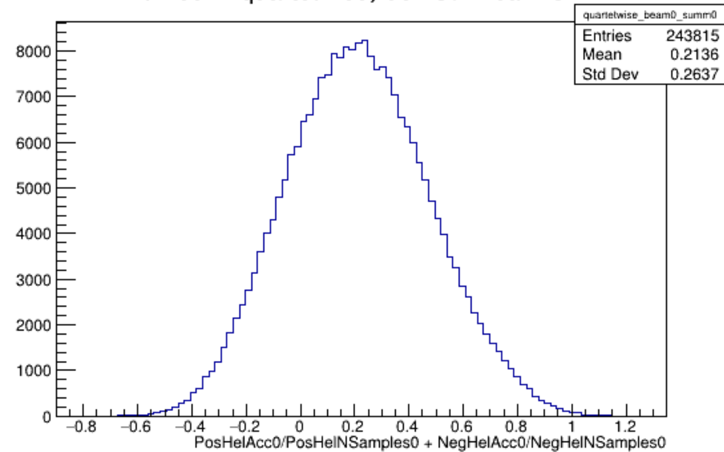
Run 5947 quartetwise, Sums0: Beam OFF
