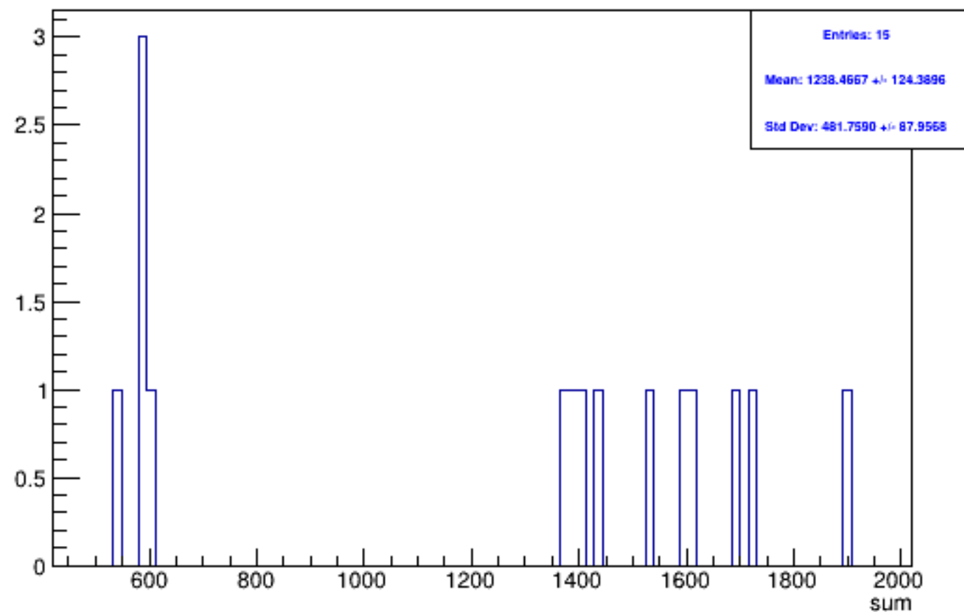
Run 5947 triggerwise, sums: All
