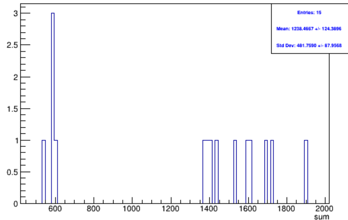
Run 5947 triggerwise, sums: Beam OFF
