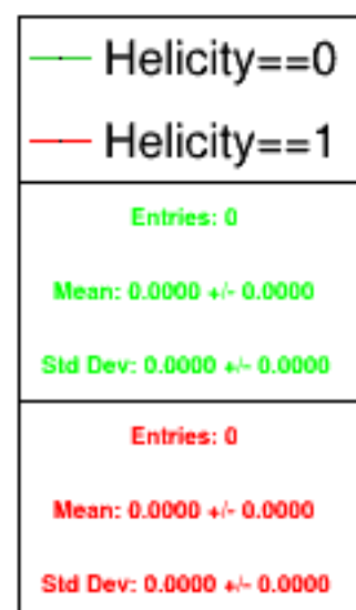
Run 5947 triggerwise, sums: Beam ON, Laser OFF
