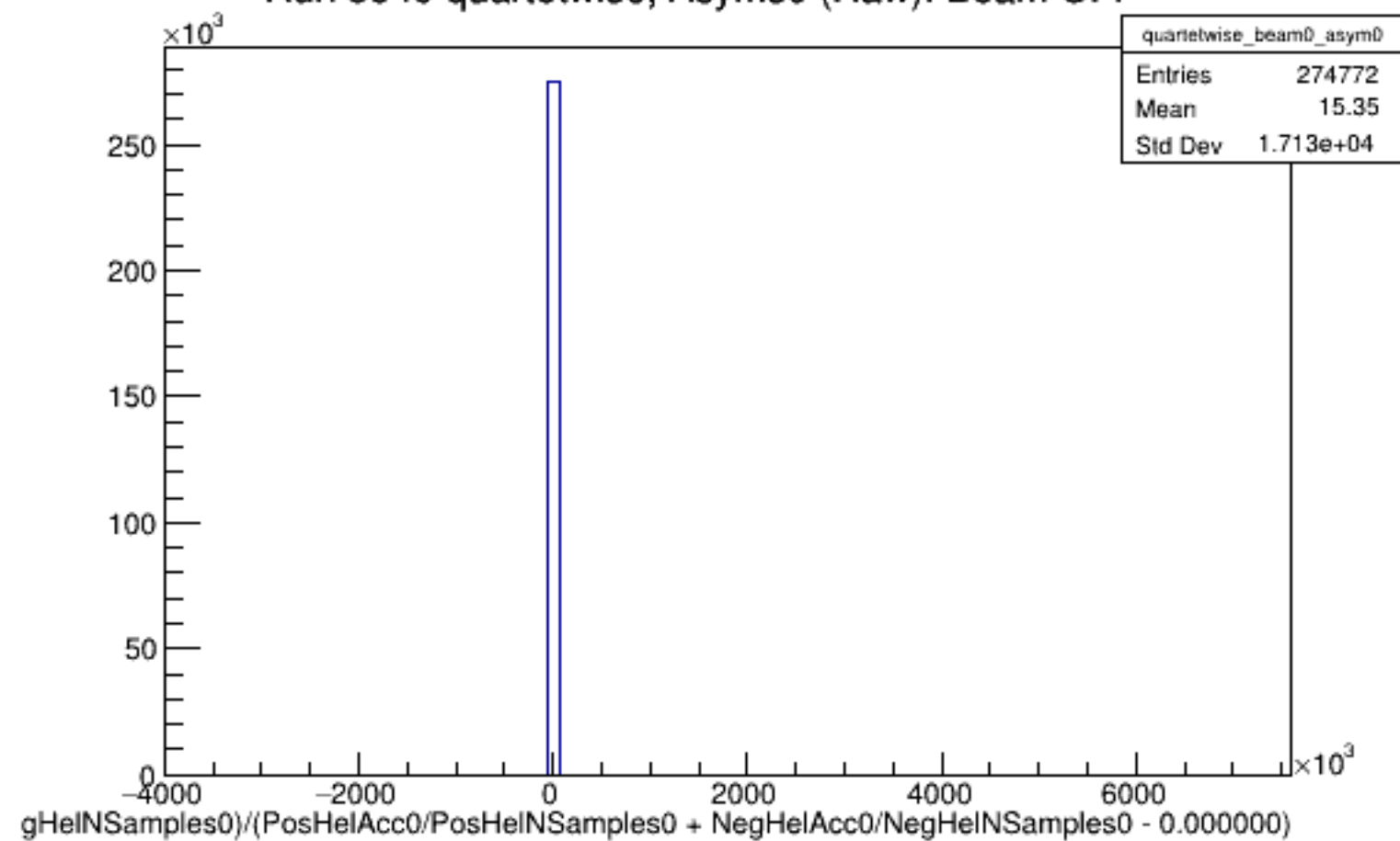
Run 5949 quartetwise, Asyms0 (Raw): Beam OFF
