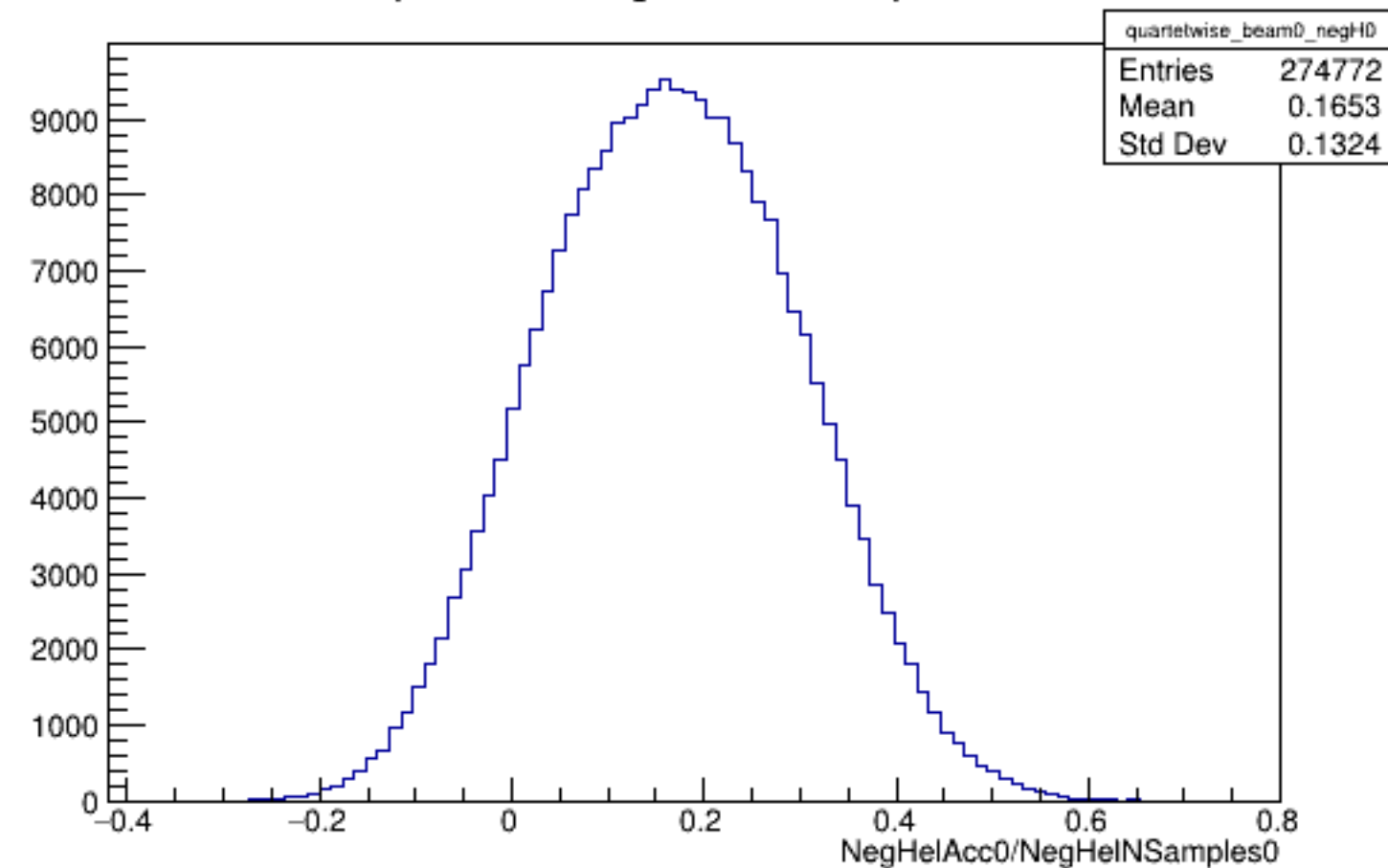
Run 5949 quartetwise, NegHelAcc0/NSamples0: Beam OFF
