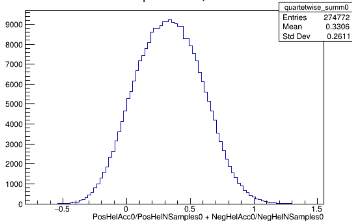
Run 5949 quartetwise, Sums0: All
