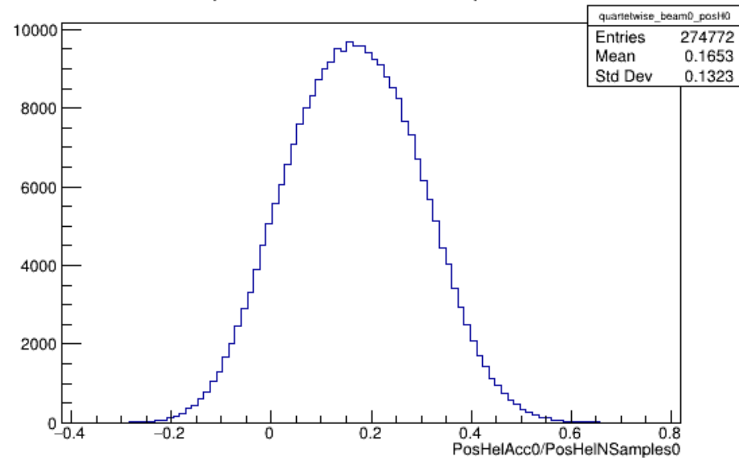
Run 5949 quartetwise, PosHelAcc0/NSamples0: Beam OFF
