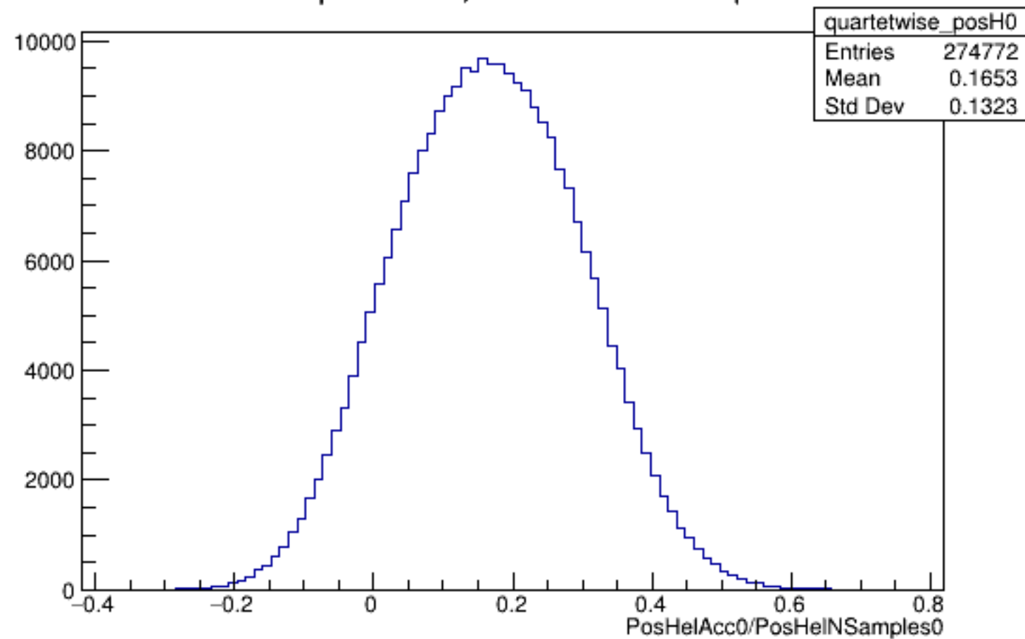
Run 5949 quartetwise, PosHelAcc0/NSamples0: All
