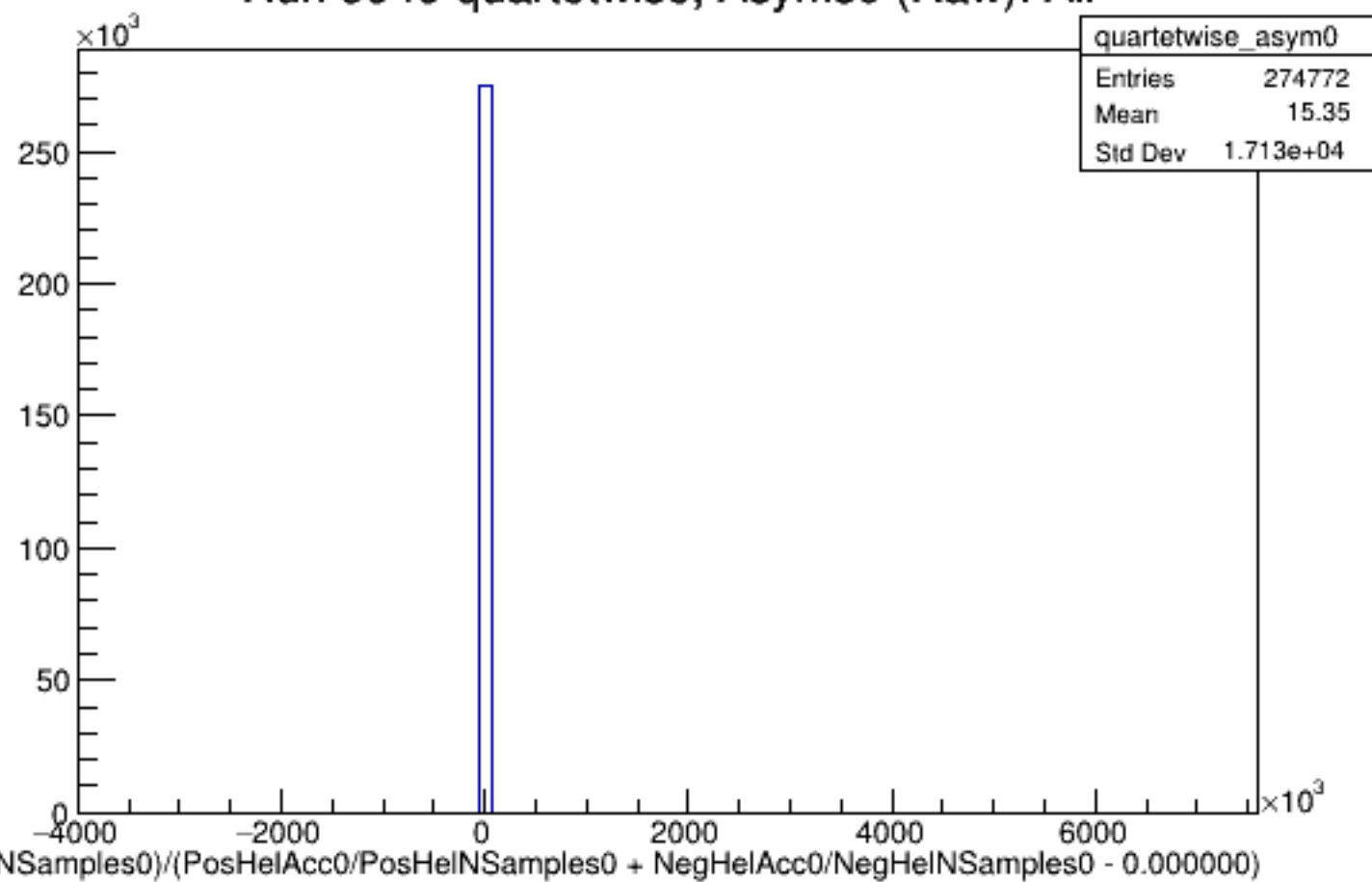
Run 5949 quartetwise, Asyms0 (Raw): All
