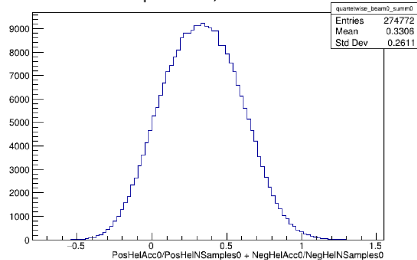
Run 5949 quartetwise, Sums0: Beam OFF
