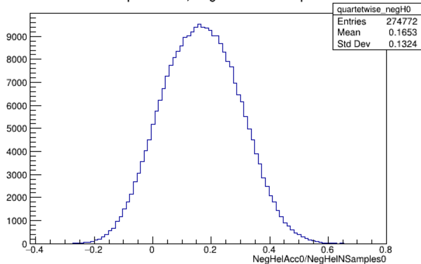
Run 5949 quartetwise, NegHelAcc0/NSamples0: All
