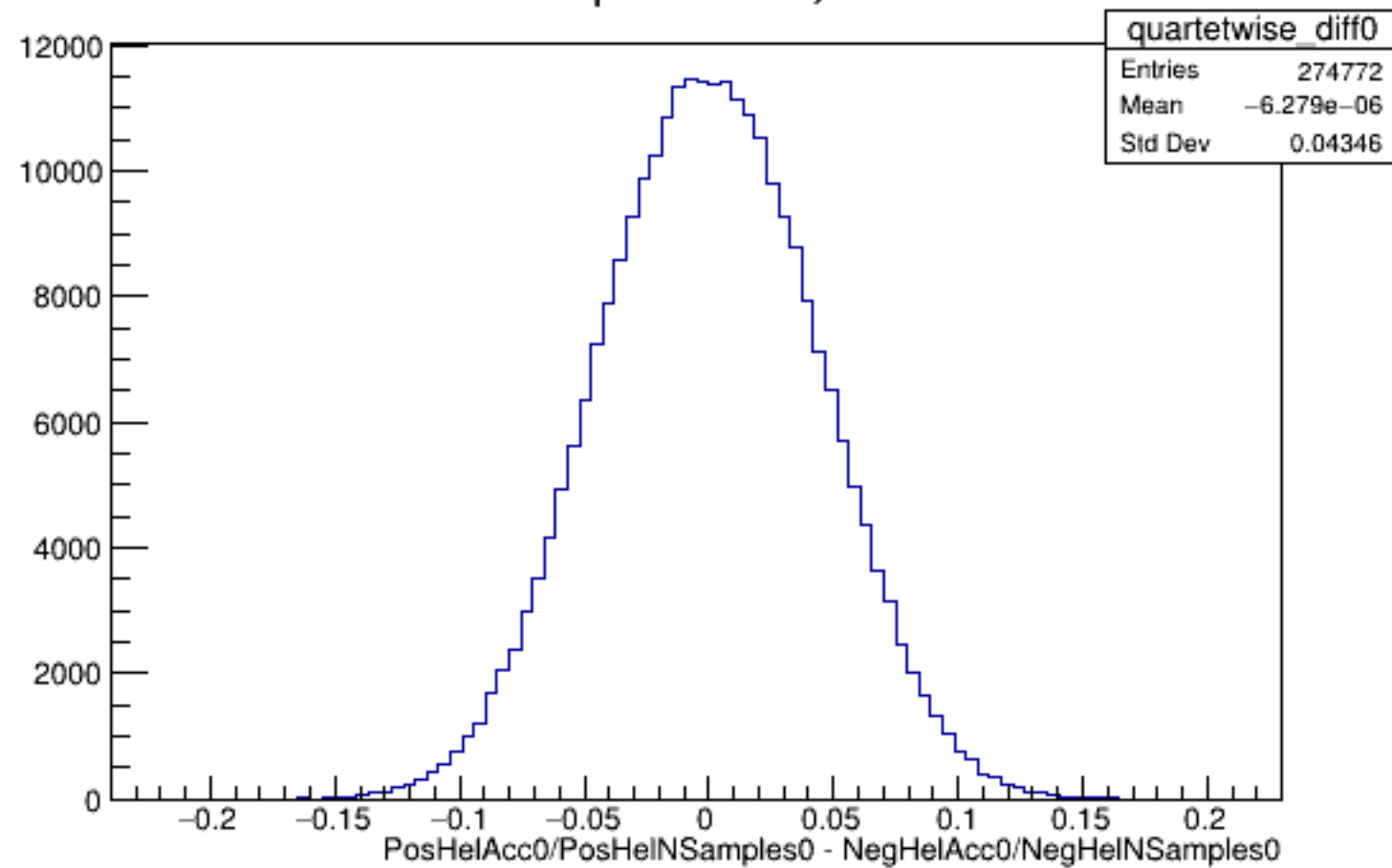
Run 5949 quartetwise, Diffs0: All
