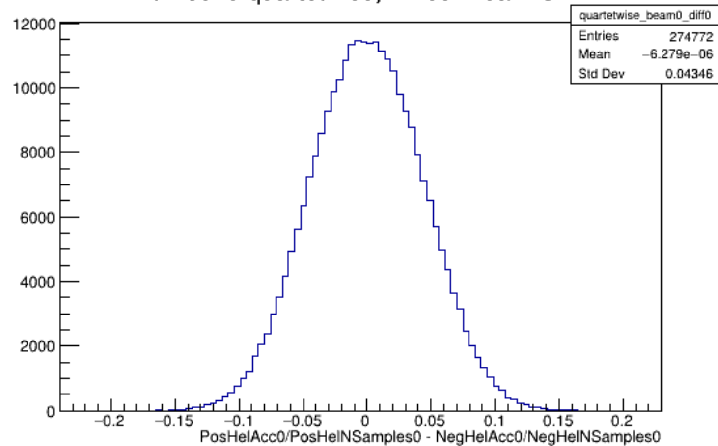
Run 5949 quartetwise, Diffs0: Beam OFF
