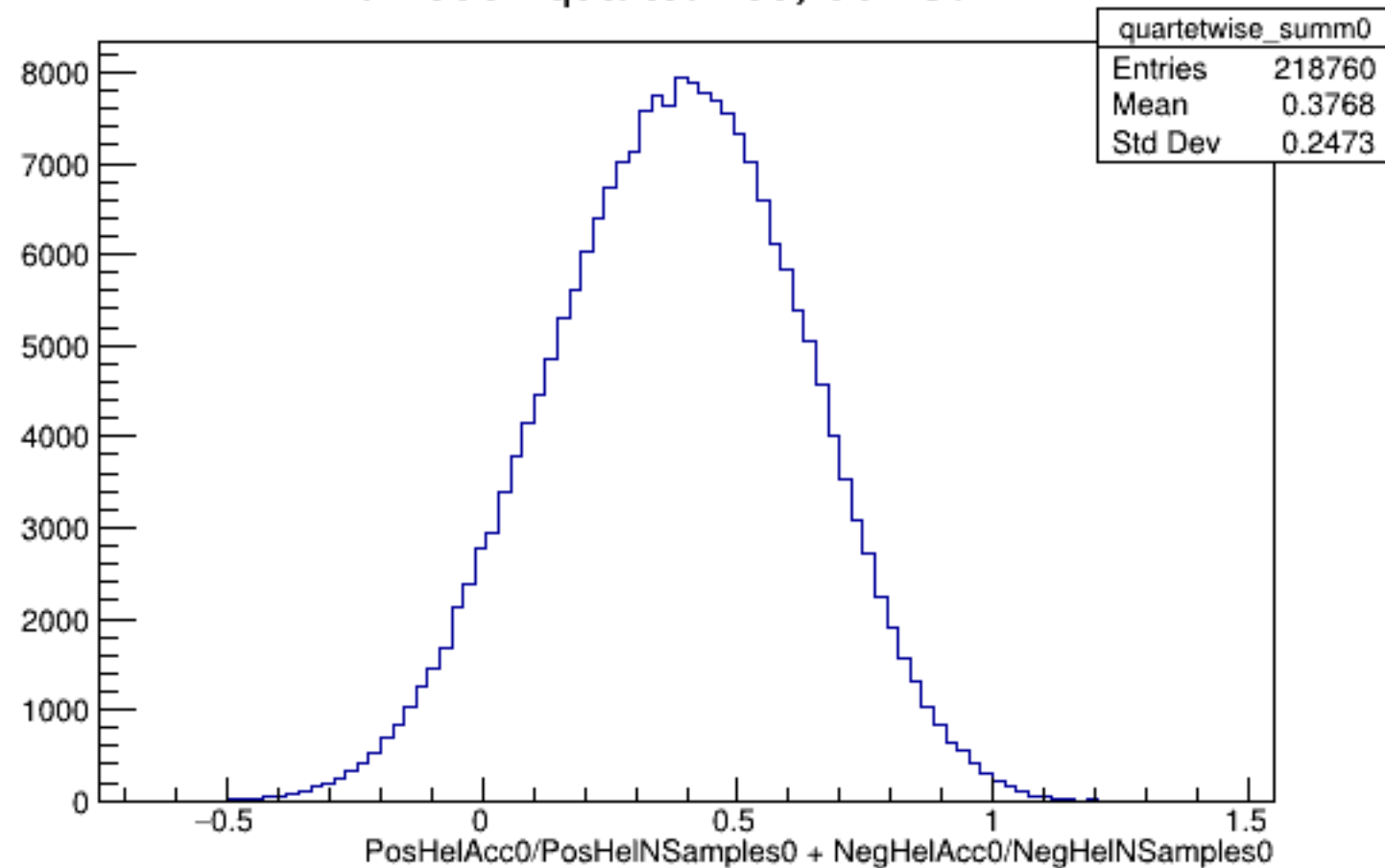
Run 5951 quartetwise, Sums0: All
