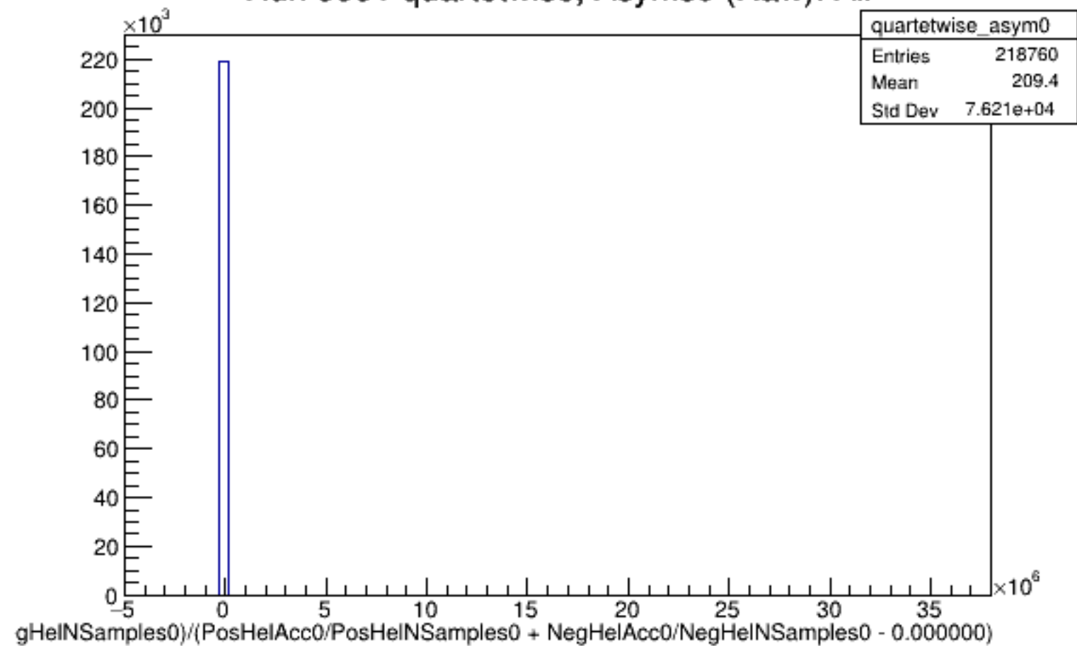
Run 5951 quartetwise, Asyms0 (Raw): All
