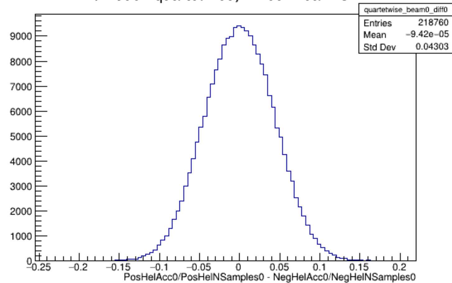
Run 5951 quartetwise, Diffs0: Beam OFF
