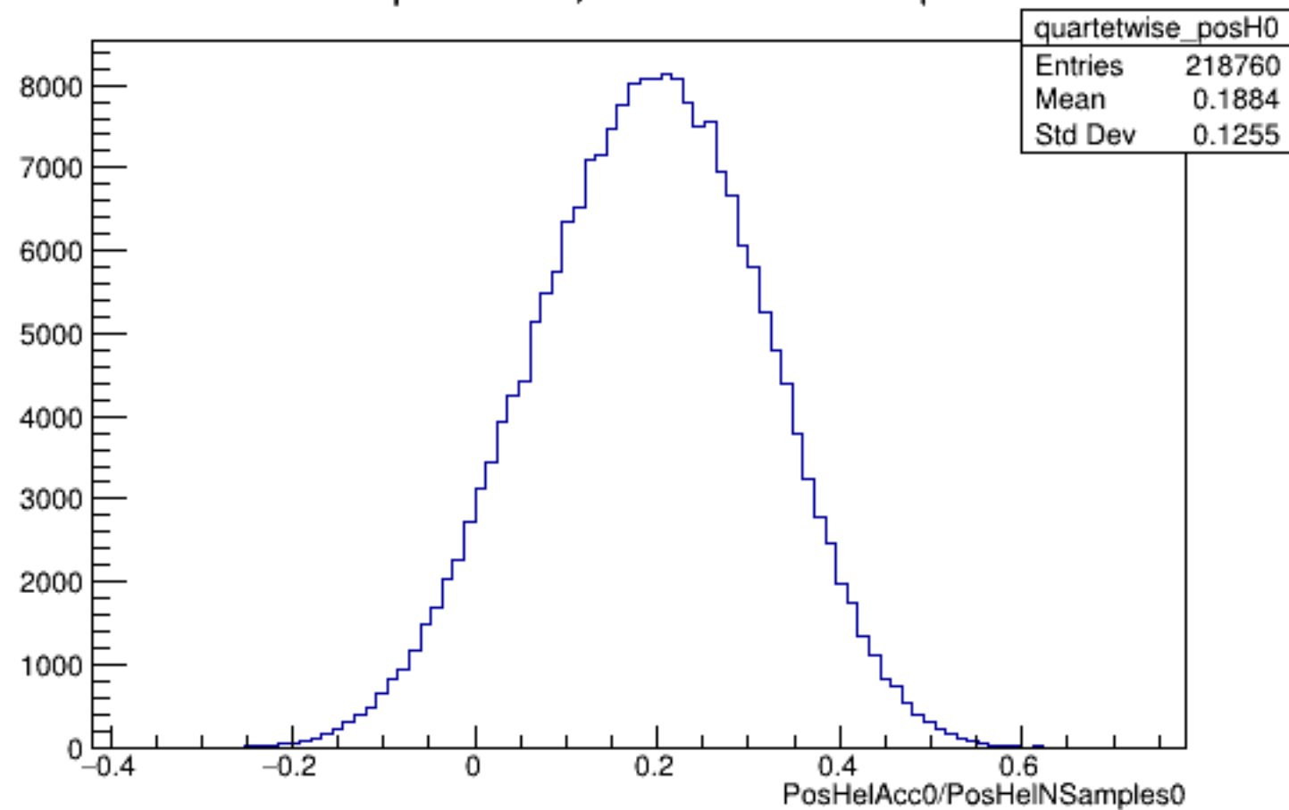
Run 5951 quartetwise, PosHelAcc0/NSamples0: All
