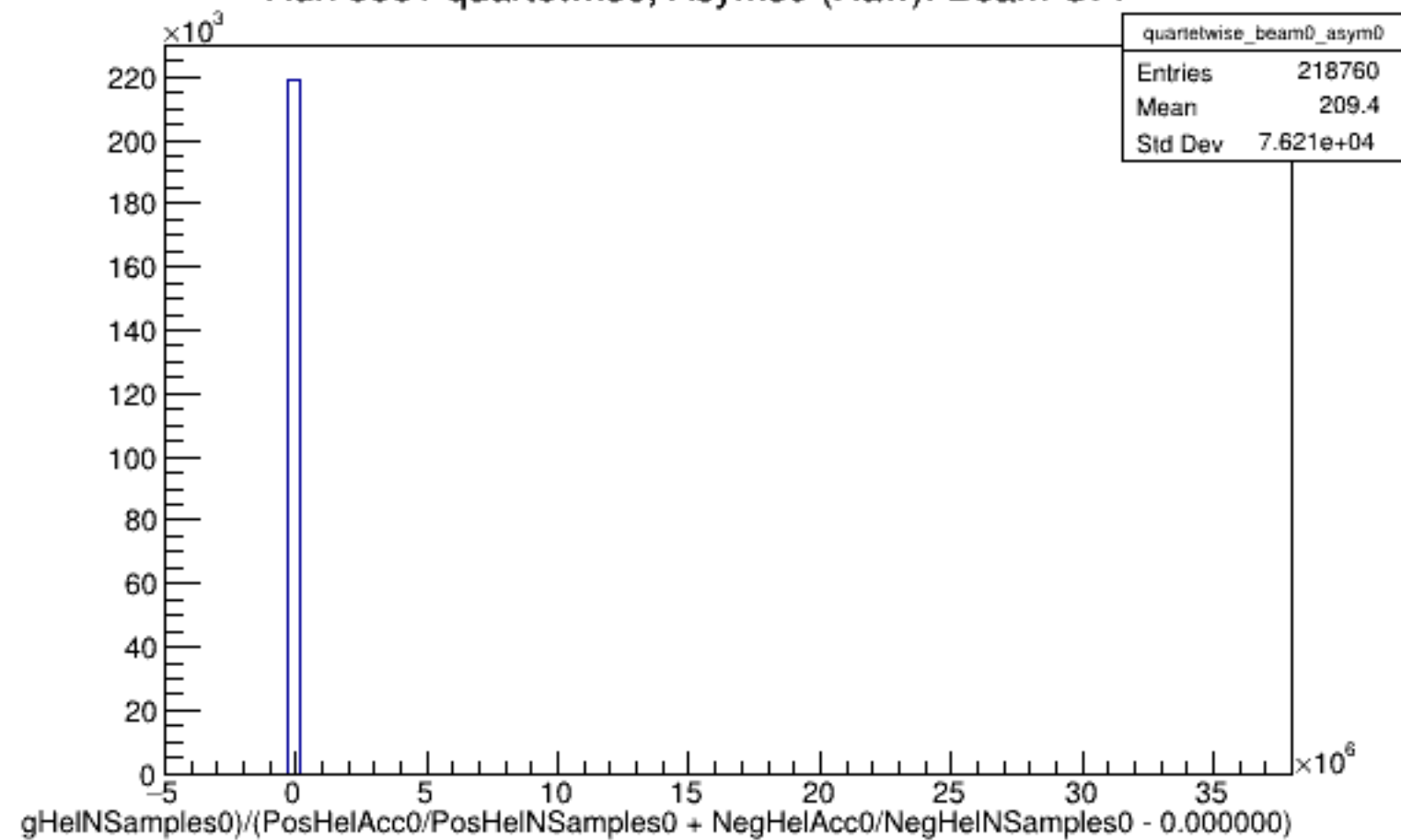
Run 5951 quartetwise, Asyms0 (Raw): Beam OFF
