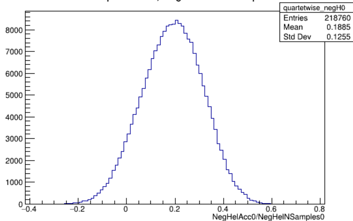
Run 5951 quartetwise, NegHelAcc0/NSamples0: All
