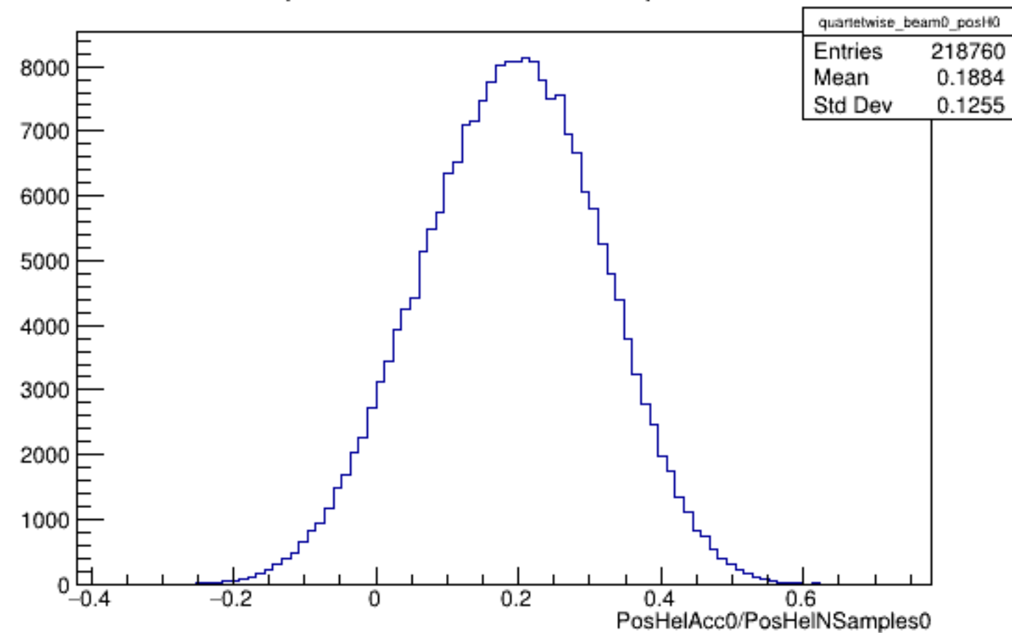
Run 5951 quartetwise, PosHelAcc0/NSamples0: Beam OFF
