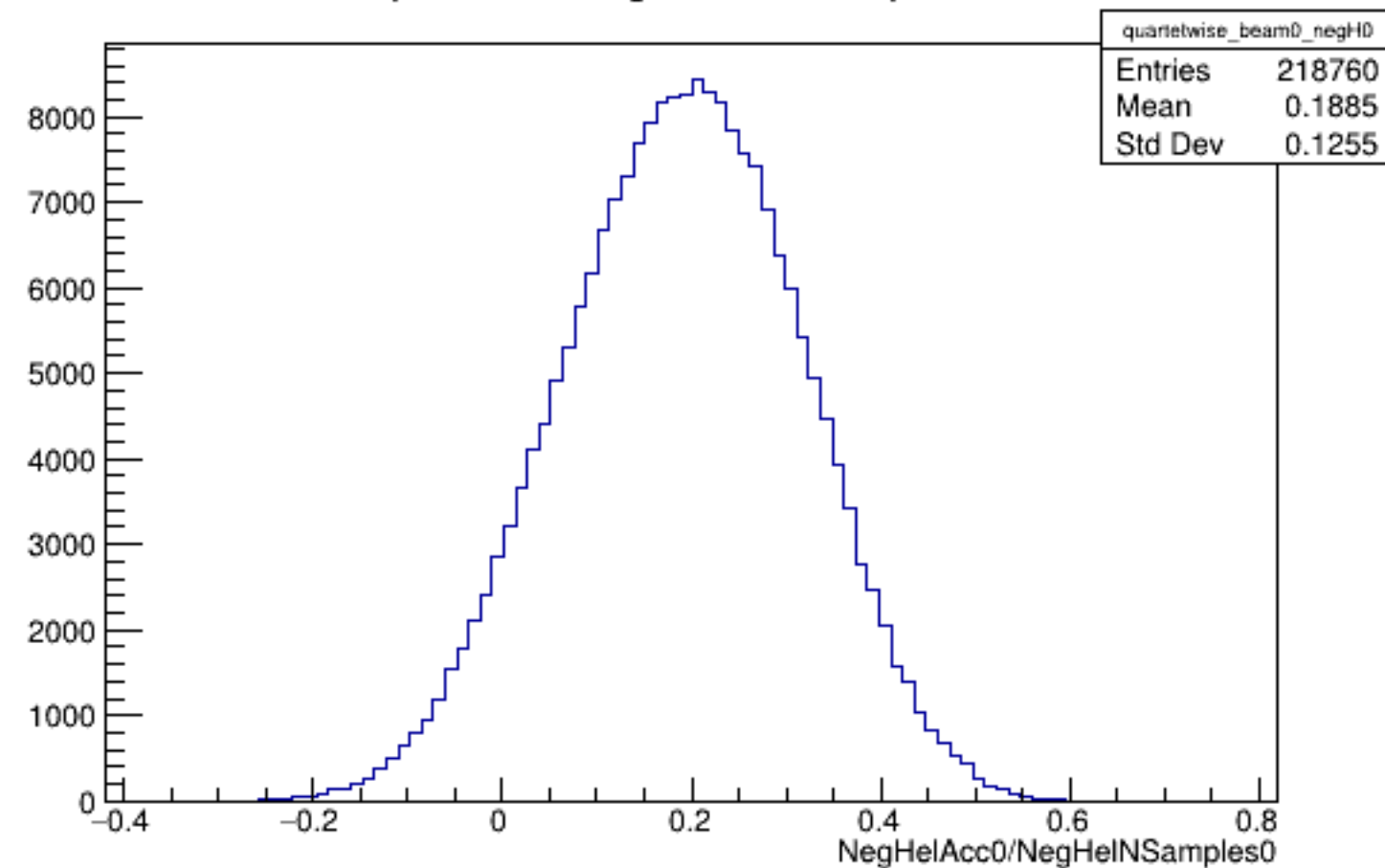
Run 5951 quartetwise, NegHelAcc0/NSamples0: Beam OFF
