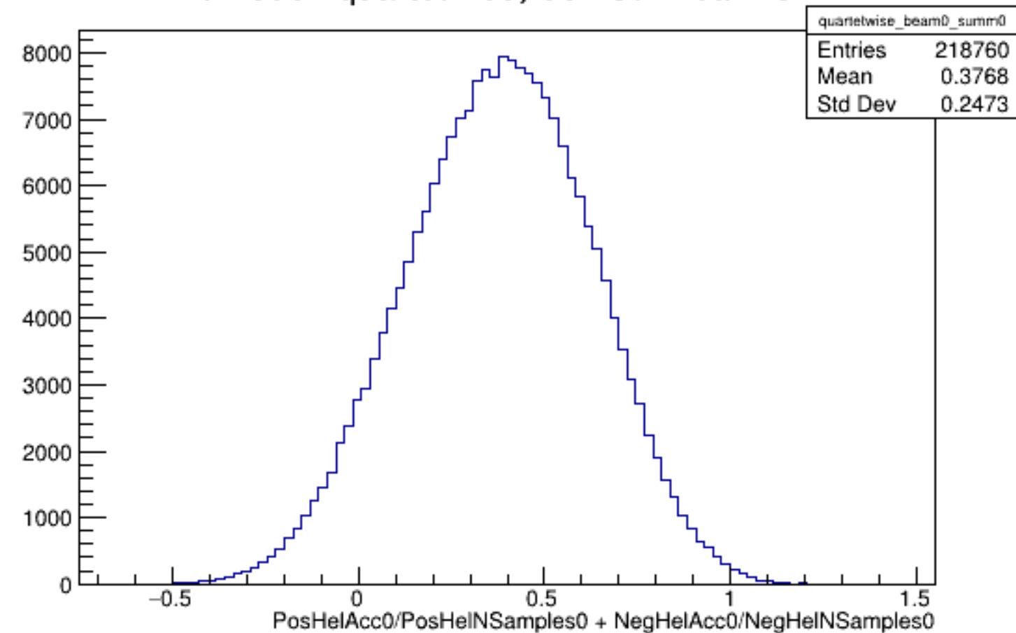
Run 5951 quartetwise, Sums0: Beam OFF
