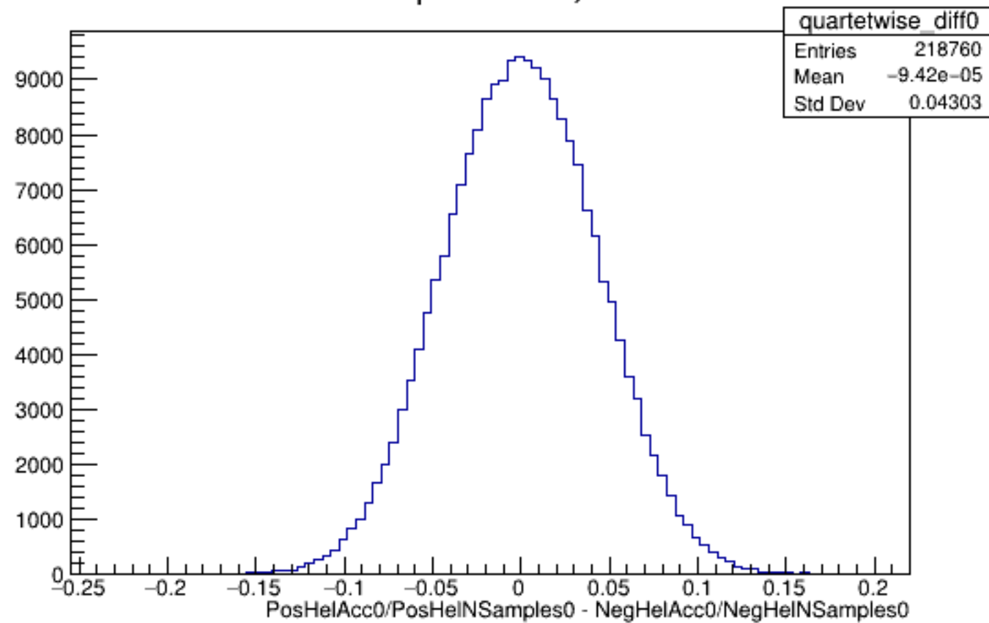
Run 5951 quartetwise, Diffs0: All
