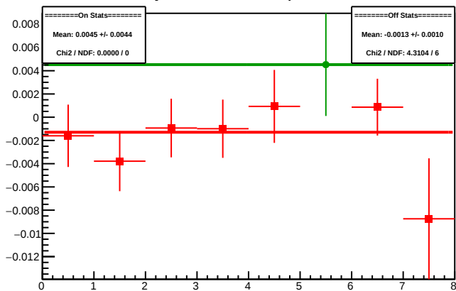
Cycle 5954.2: Multiplet Diffs
