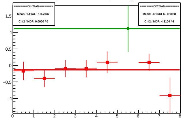
Cycle 5954.2: Multiplet Asyms
