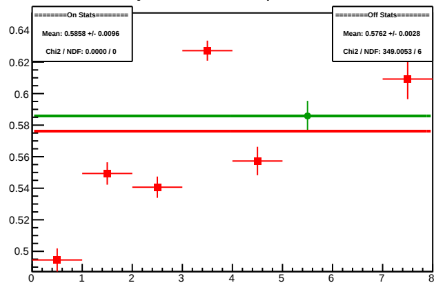
Cycle 5954.2: Multiplet Sums
