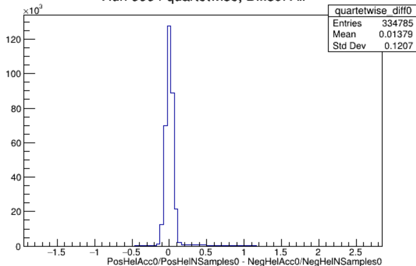
Run 5954 quartetwise, Diffs0: All
