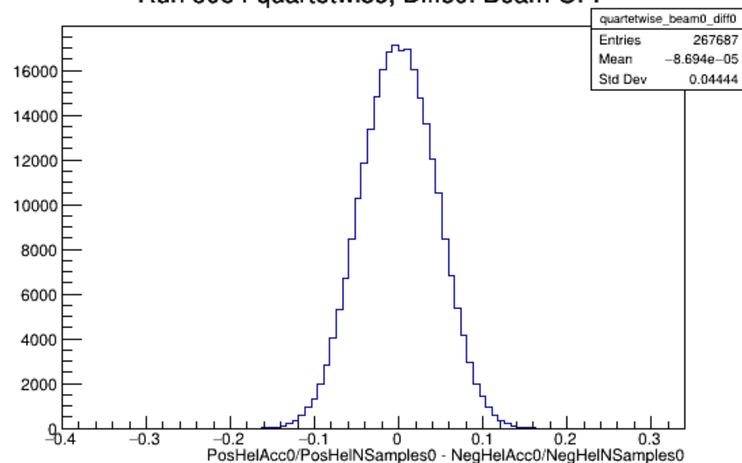
Run 5954 quartetwise, Diffs0: Beam OFF
