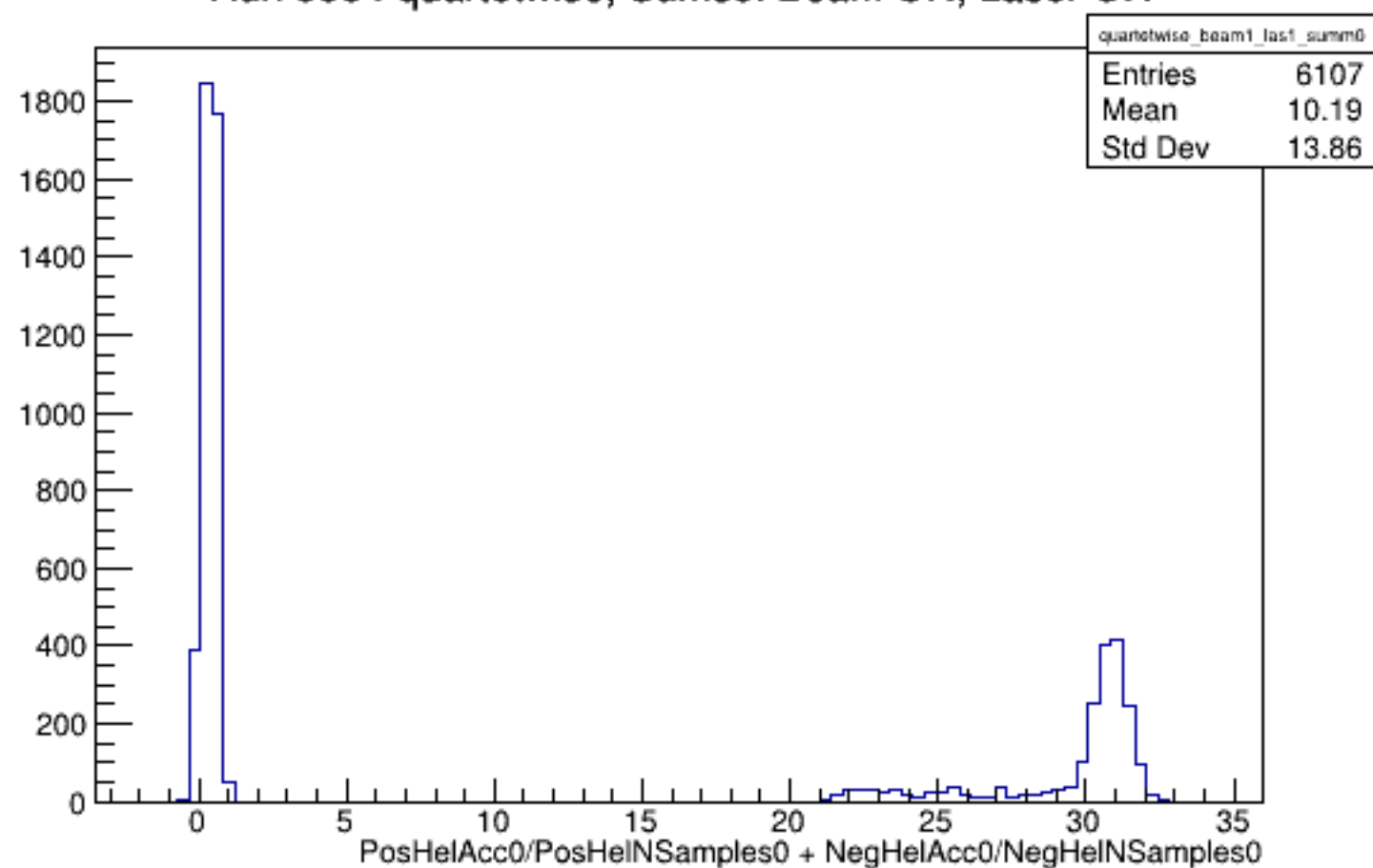
Run 5954 quartetwise, Sums0: Beam ON, Laser ON
