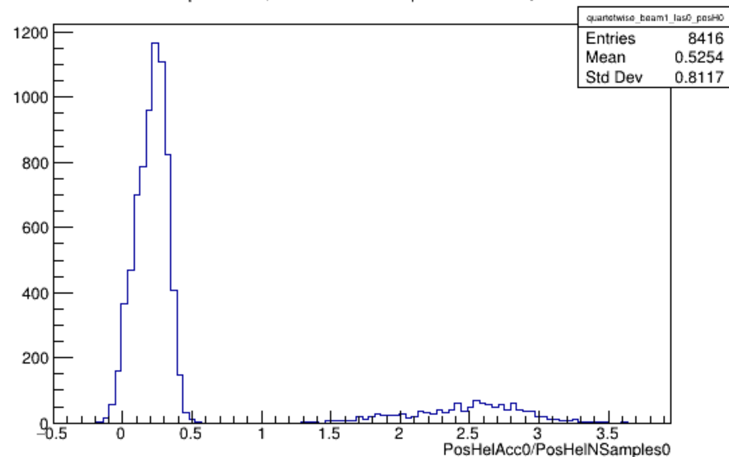
Run 5954 quartetwise, PosHelAcc0/NSamples0: Beam ON, Laser OFF
