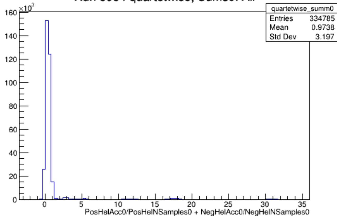
Run 5954 quartetwise, Sums0: All
