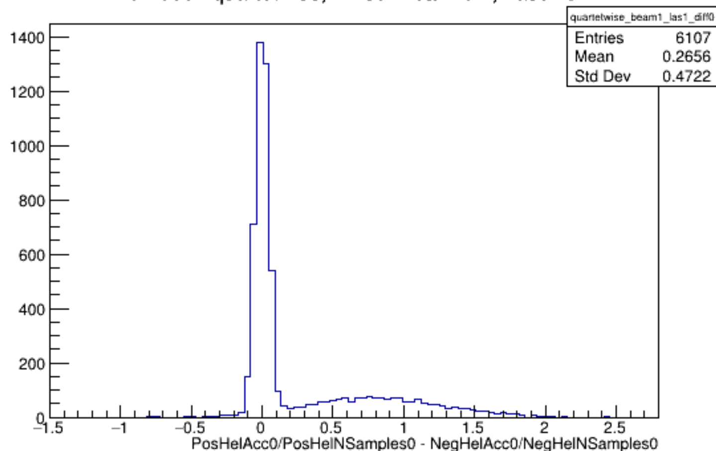
Run 5954 quartetwise, Diffs0: Beam ON, Laser ON
