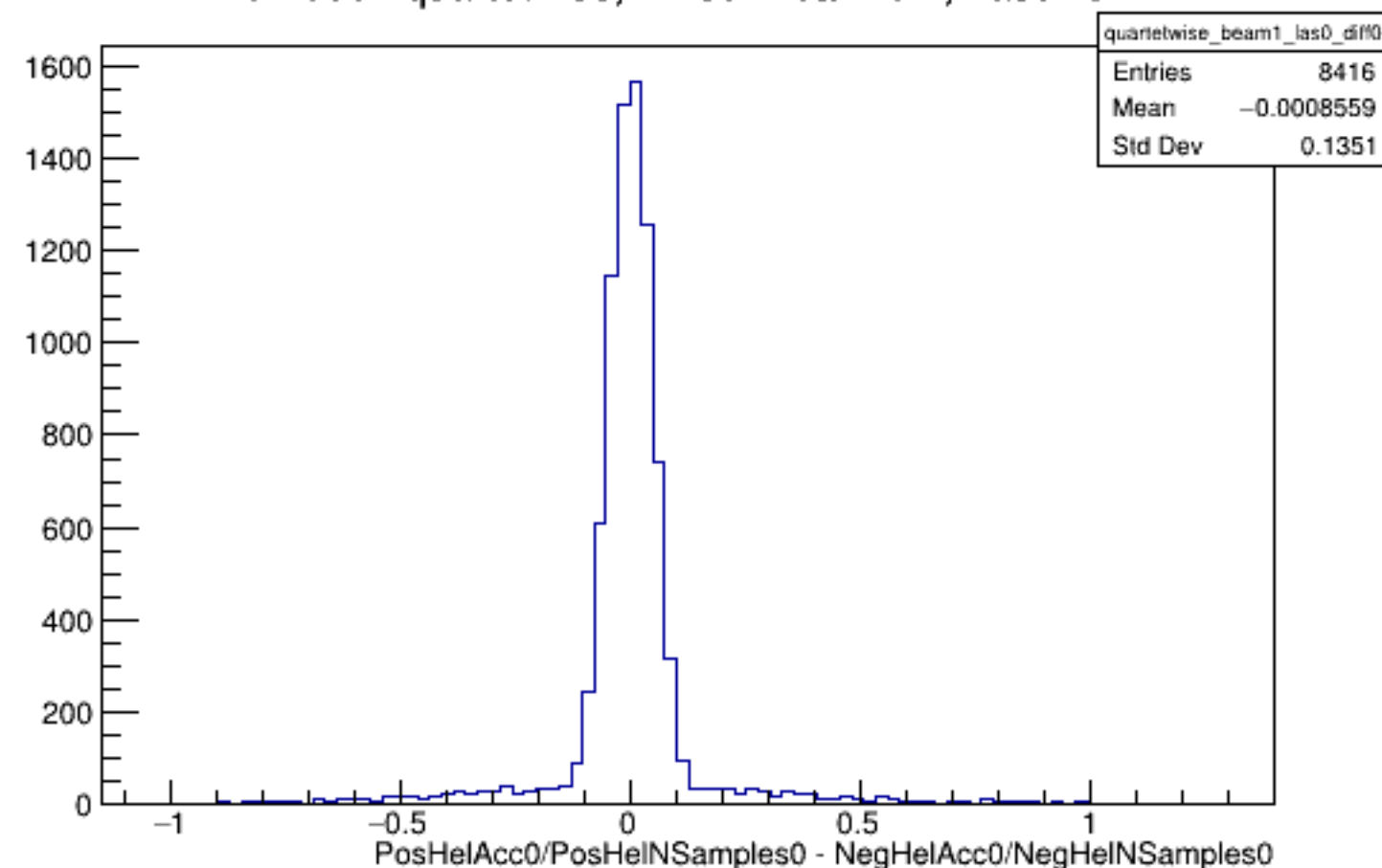
Run 5954 quartetwise, Diffs0: Beam ON, Laser OFF
