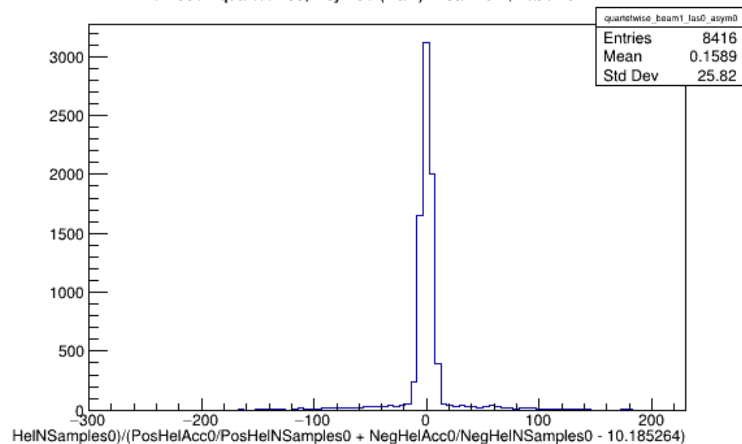
Run 5954 quartetwise, Asyms0 (Raw): Beam ON, Laser OFF
