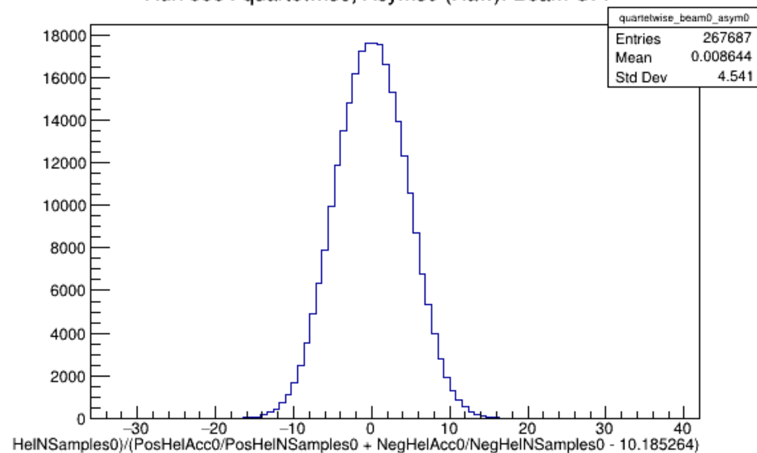
Run 5954 quartetwise, Asyms0 (Raw): Beam OFF
