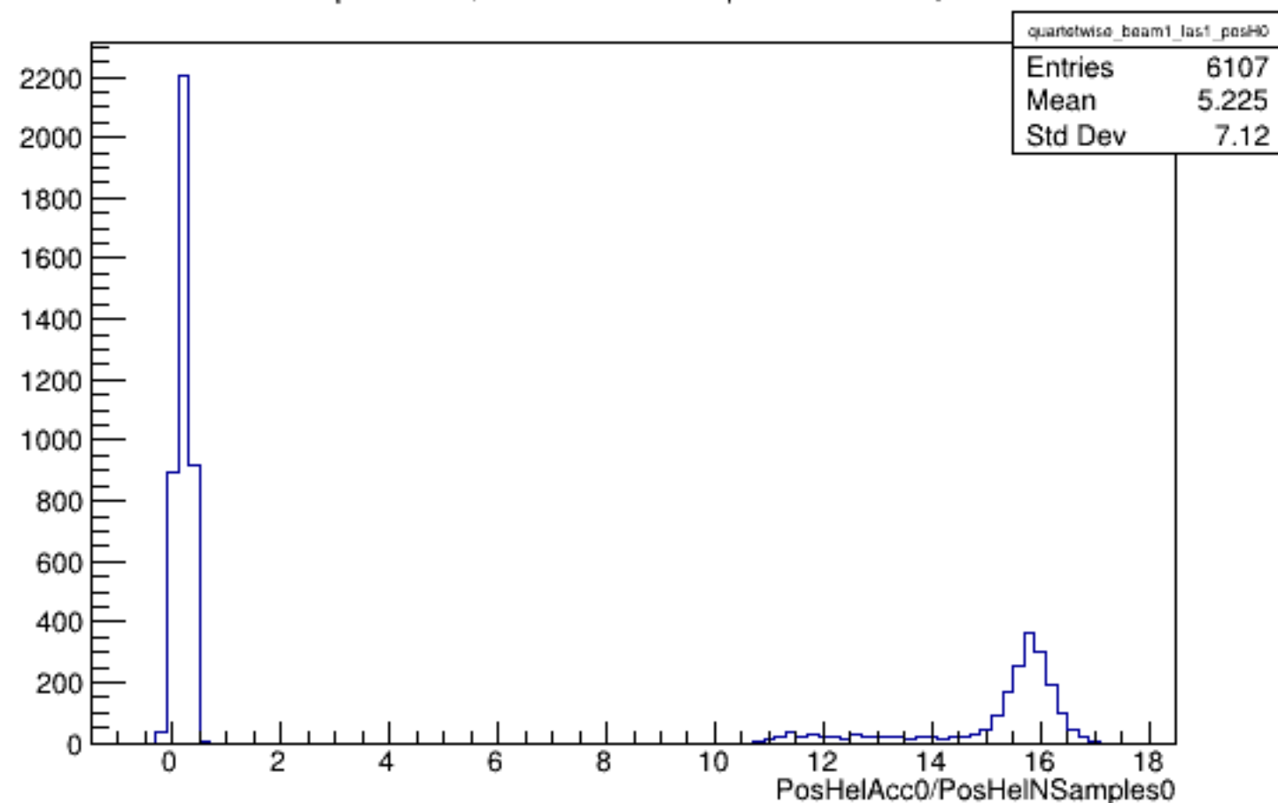
Run 5954 quartetwise, PosHelAcc0/NSamples0: Beam ON, Laser ON
