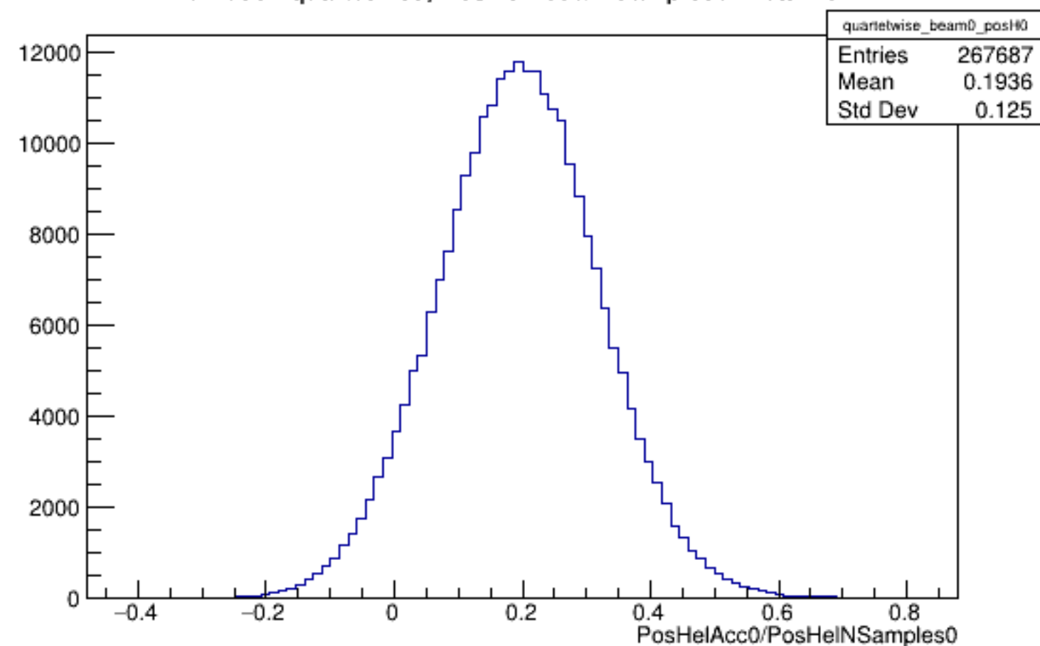
Run 5954 quartetwise, PosHelAcc0/NSamples0: Beam OFF
