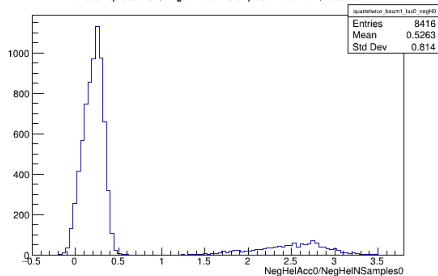
Run 5954 quartetwise, NegHelAcc0/NSamples0: Beam ON, Laser OFF
