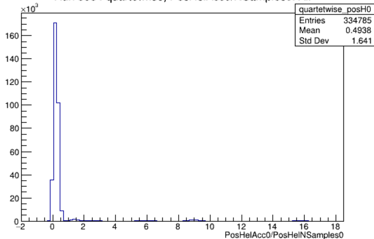
Run 5954 quartetwise, PosHelAcc0/NSamples0: All
