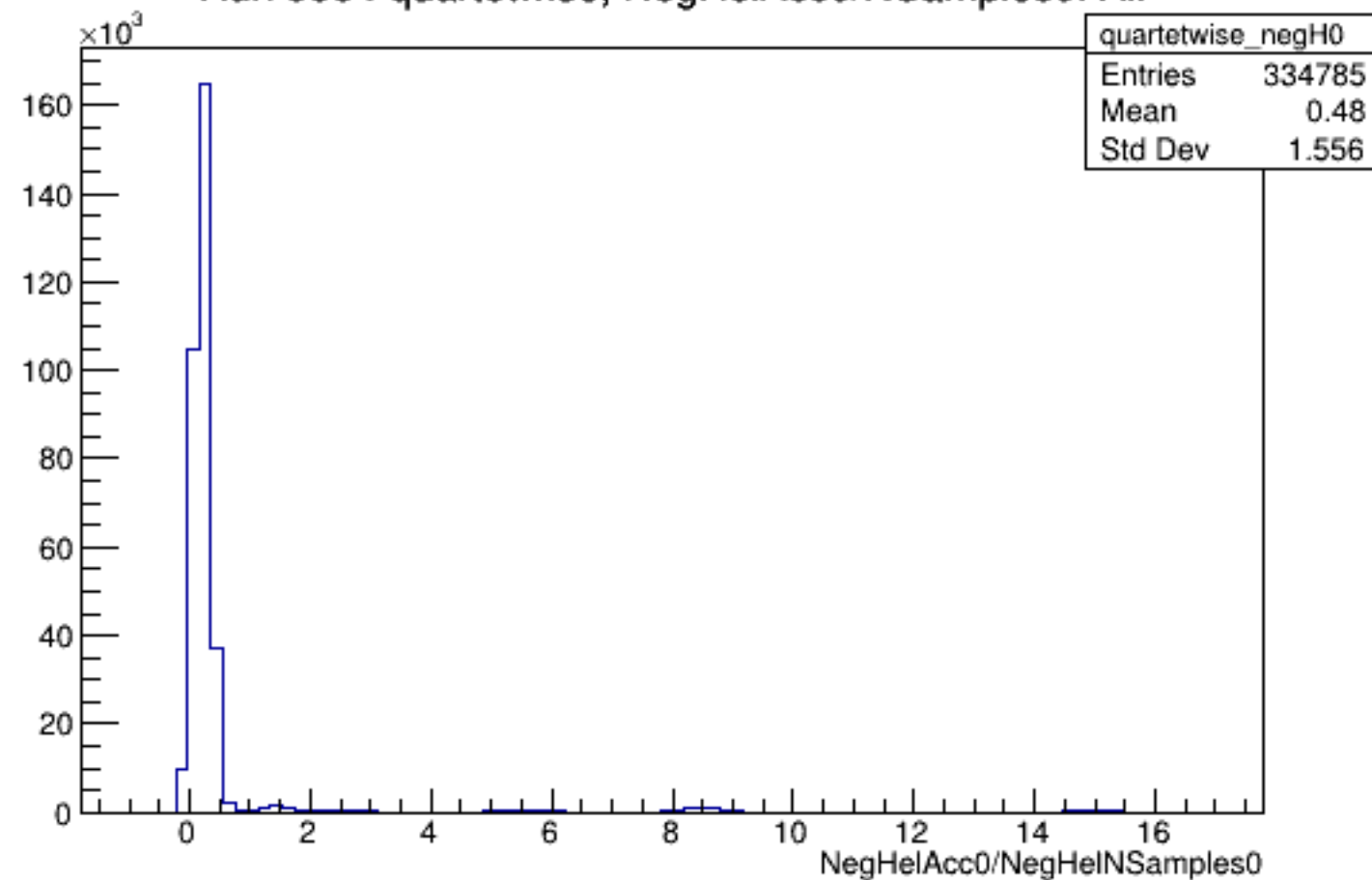
Run 5954 quartetwise, NegHelAcc0/NSamples0: All
