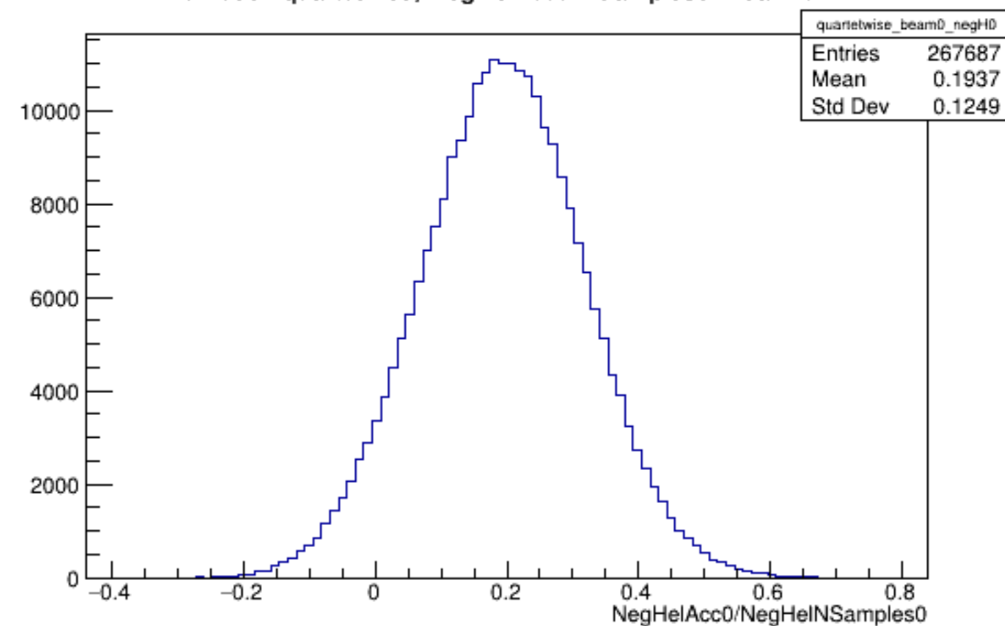
Run 5954 quartetwise, NegHelAcc0/NSamples0: Beam OFF
