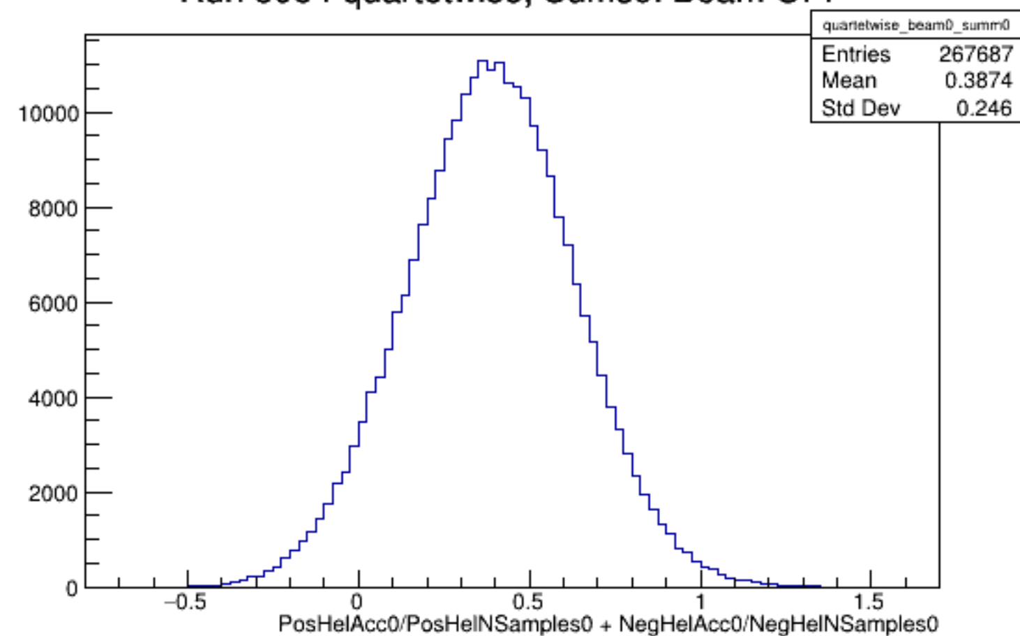
Run 5954 quartetwise, Sums0: Beam OFF
