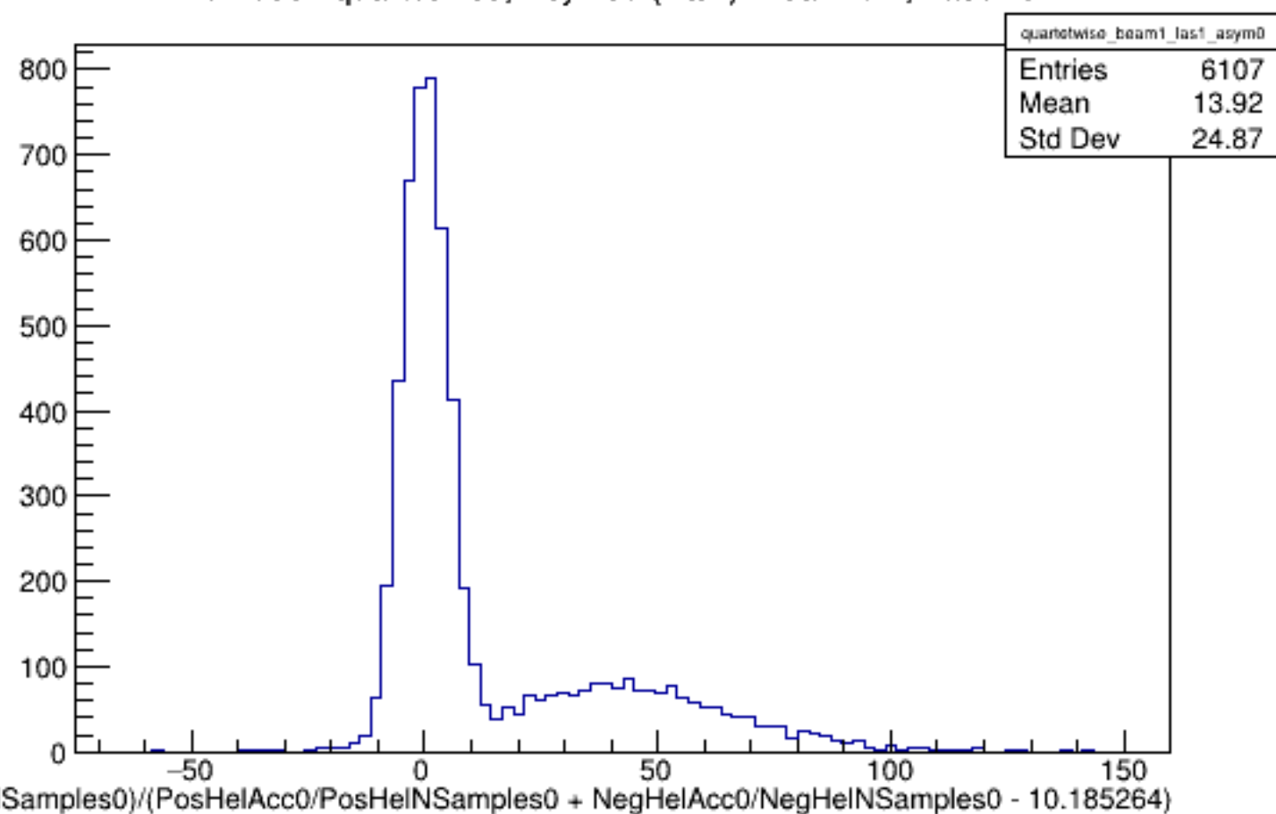
Run 5954 quartetwise, Asyms0 (Raw): Beam ON, Laser ON
