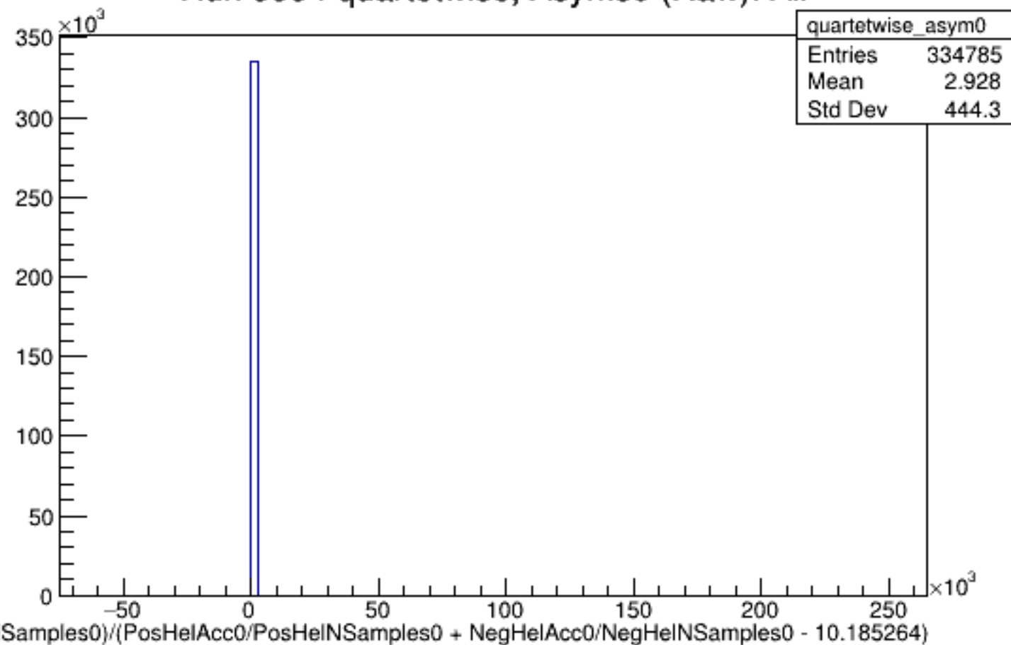
Run 5954 quartetwise, Asyms0 (Raw): All
