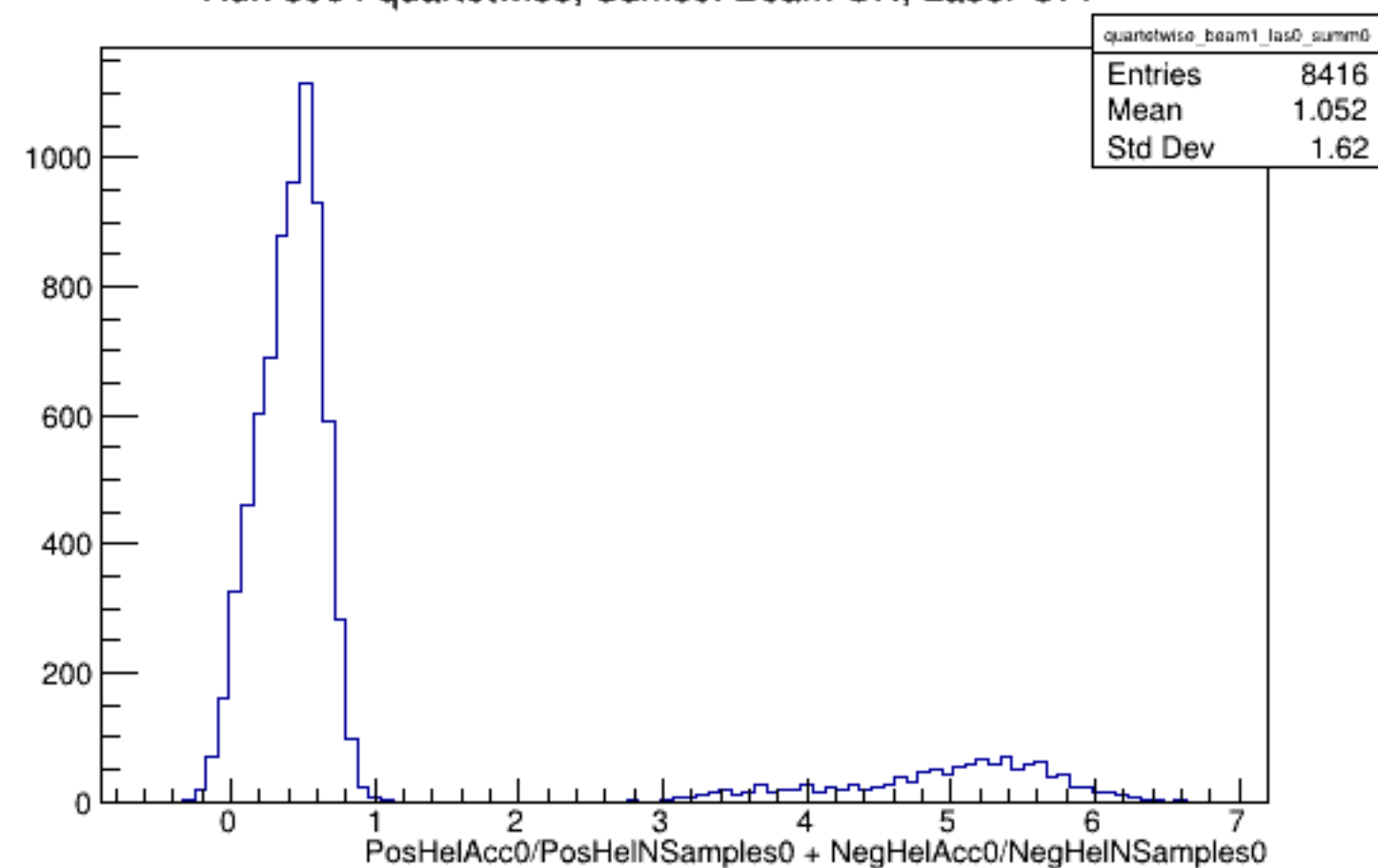
Run 5954 quartetwise, Sums0: Beam ON, Laser OFF
