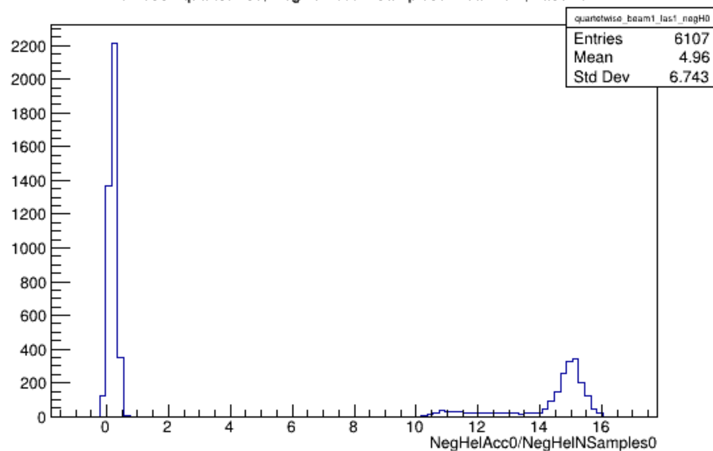
Run 5954 quartetwise, NegHelAcc0/NSamples0: Beam ON, Laser ON
