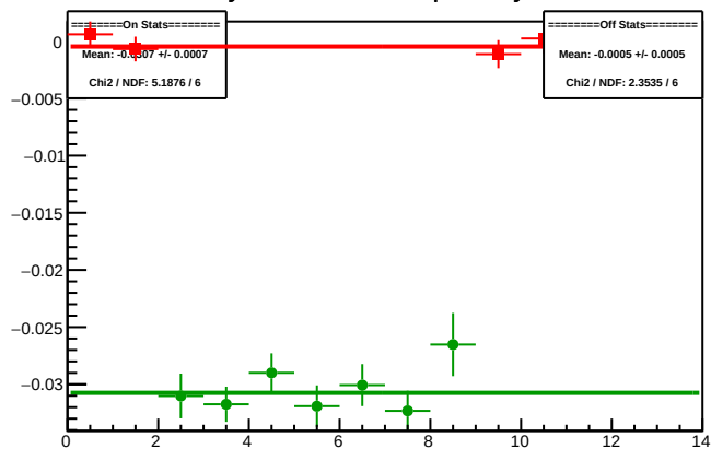
Cycle 5959.2: Multiplet Asyms
