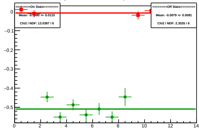
Cycle 5959.2: Multiplet Diffs
