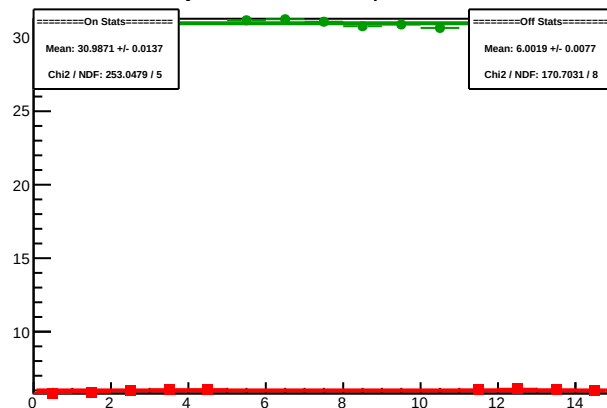
Cycle 5959.5: Multiplet Sums
