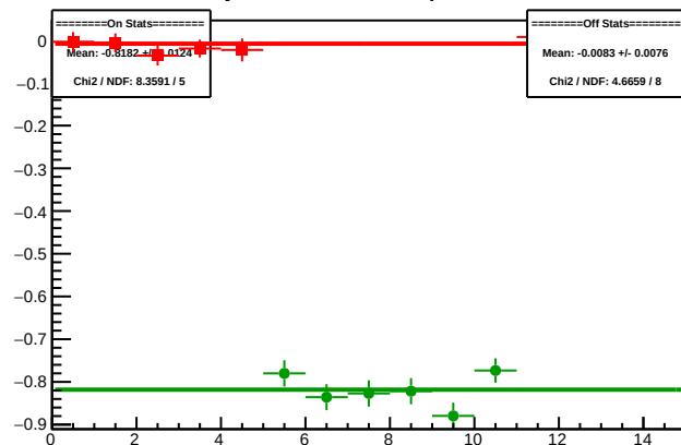
Cycle 5959.5: Multiplet Diffs
