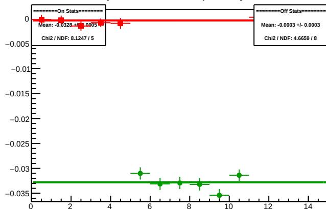
Cycle 5959.5: Multiplet Asyms
