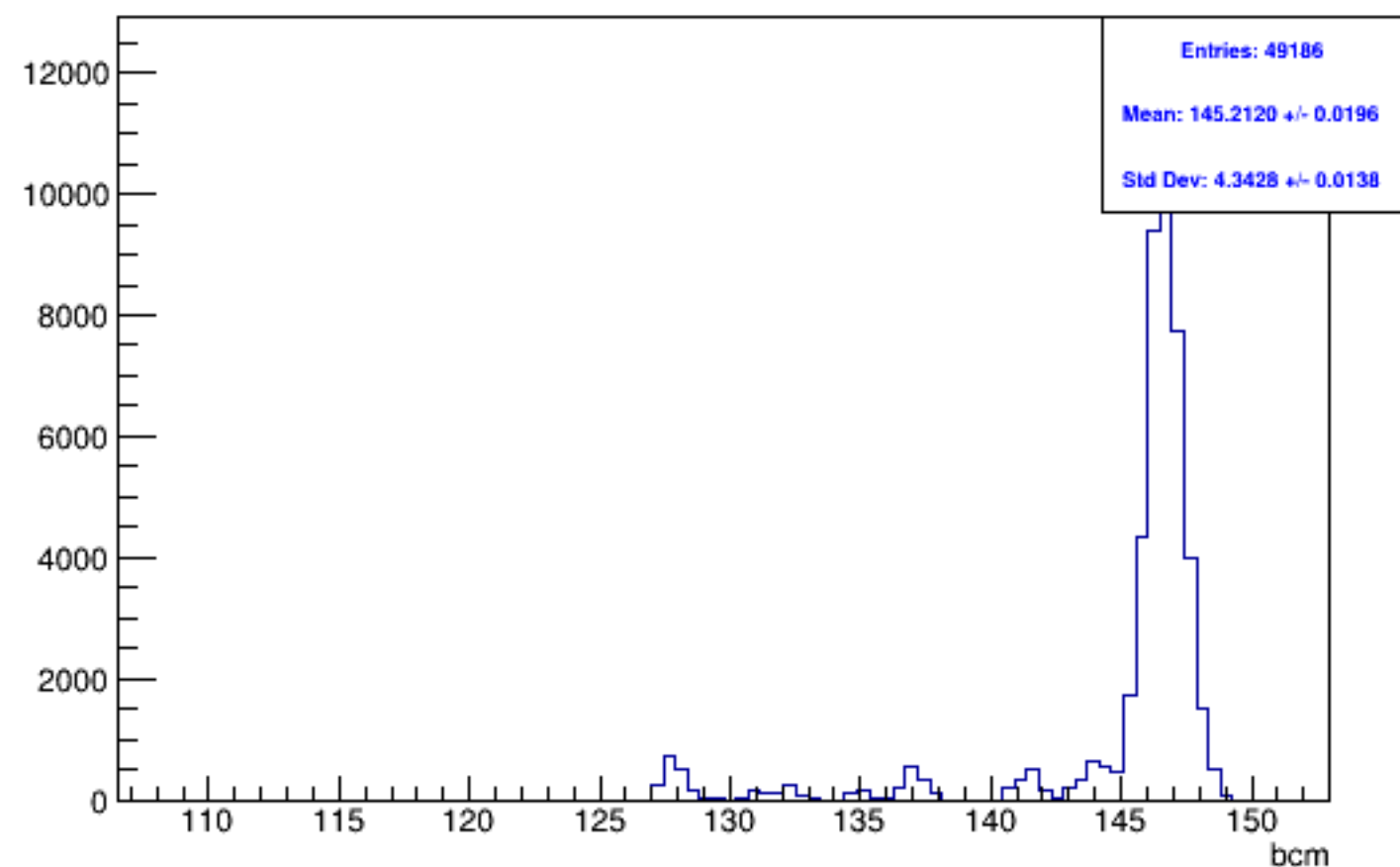
Run 5959, mpwise, BCM: Beam ON, Laser ON
