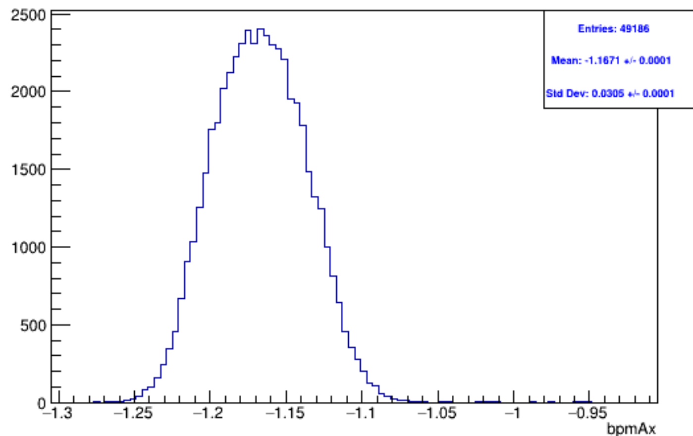
Run 5959, mpwise, bpmAx: Beam ON, Laser ON
