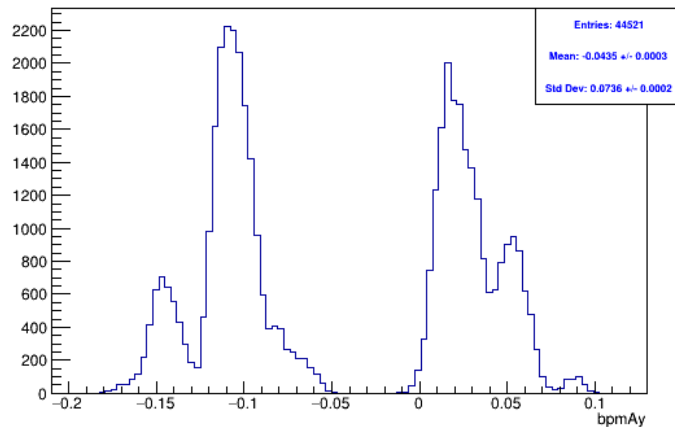
Run 5959, mpwise, bpmAy: Beam ON, Laser OFF
