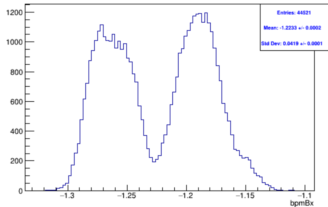
Run 5959, mpwise, bpmBx: Beam ON, Laser OFF
