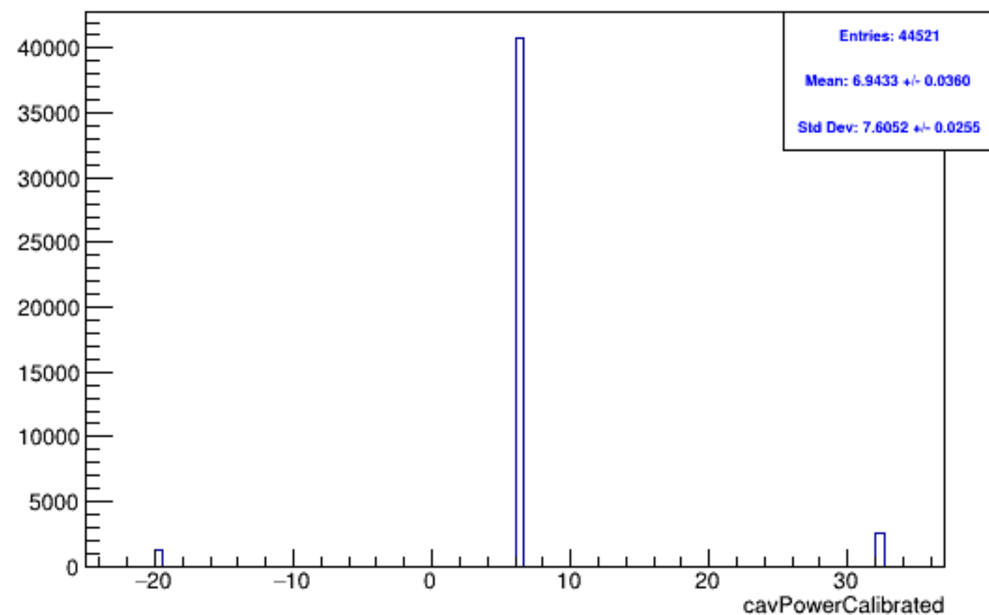
Run 5959, mpwise, lasPow: Beam ON, Laser OFF
