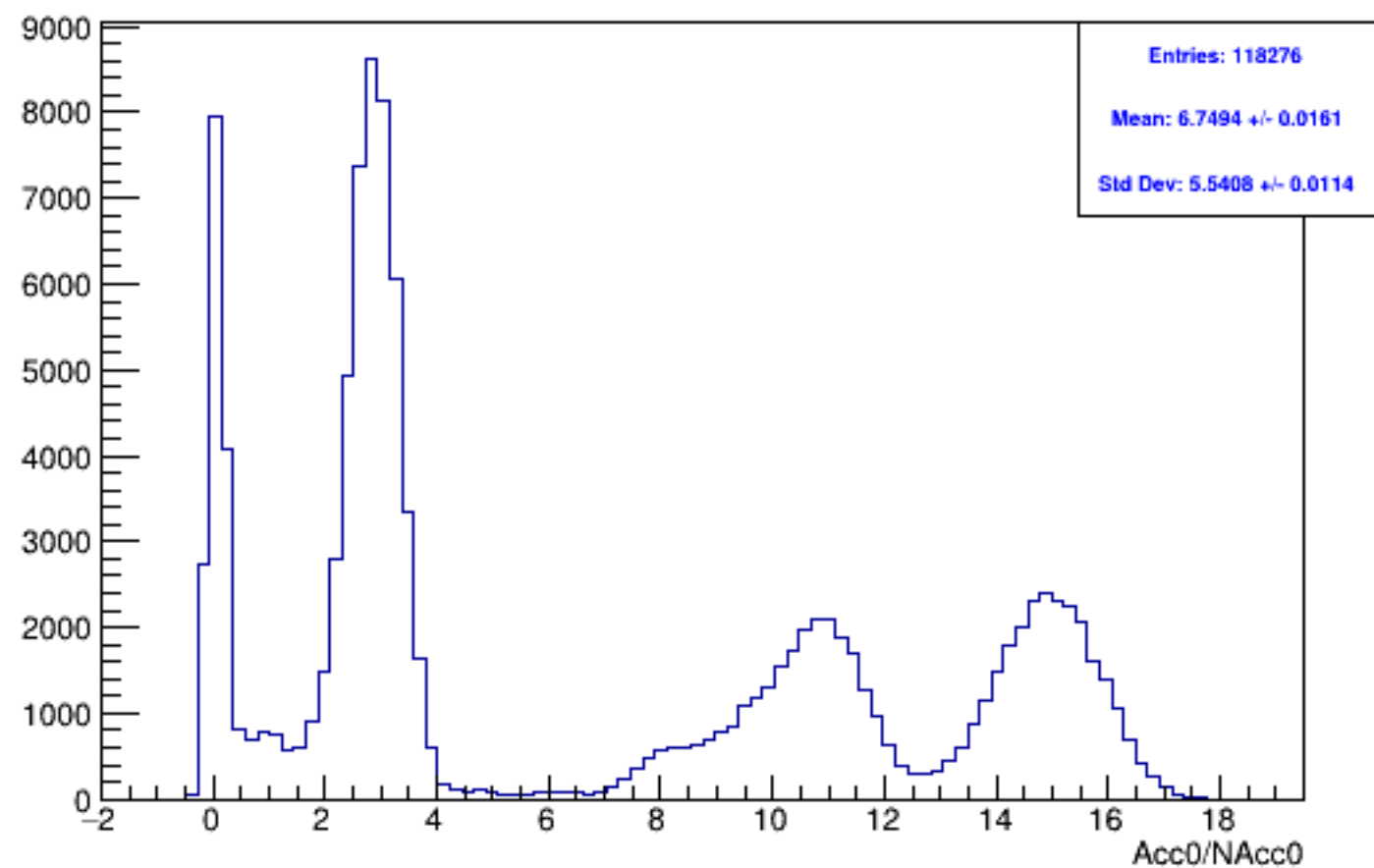
Run 5959 mpwise, acc0: All
