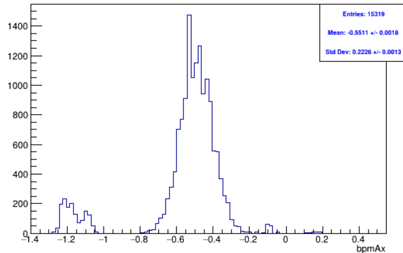
Run 5959 mpwise, bpmAx: Beam OFF
