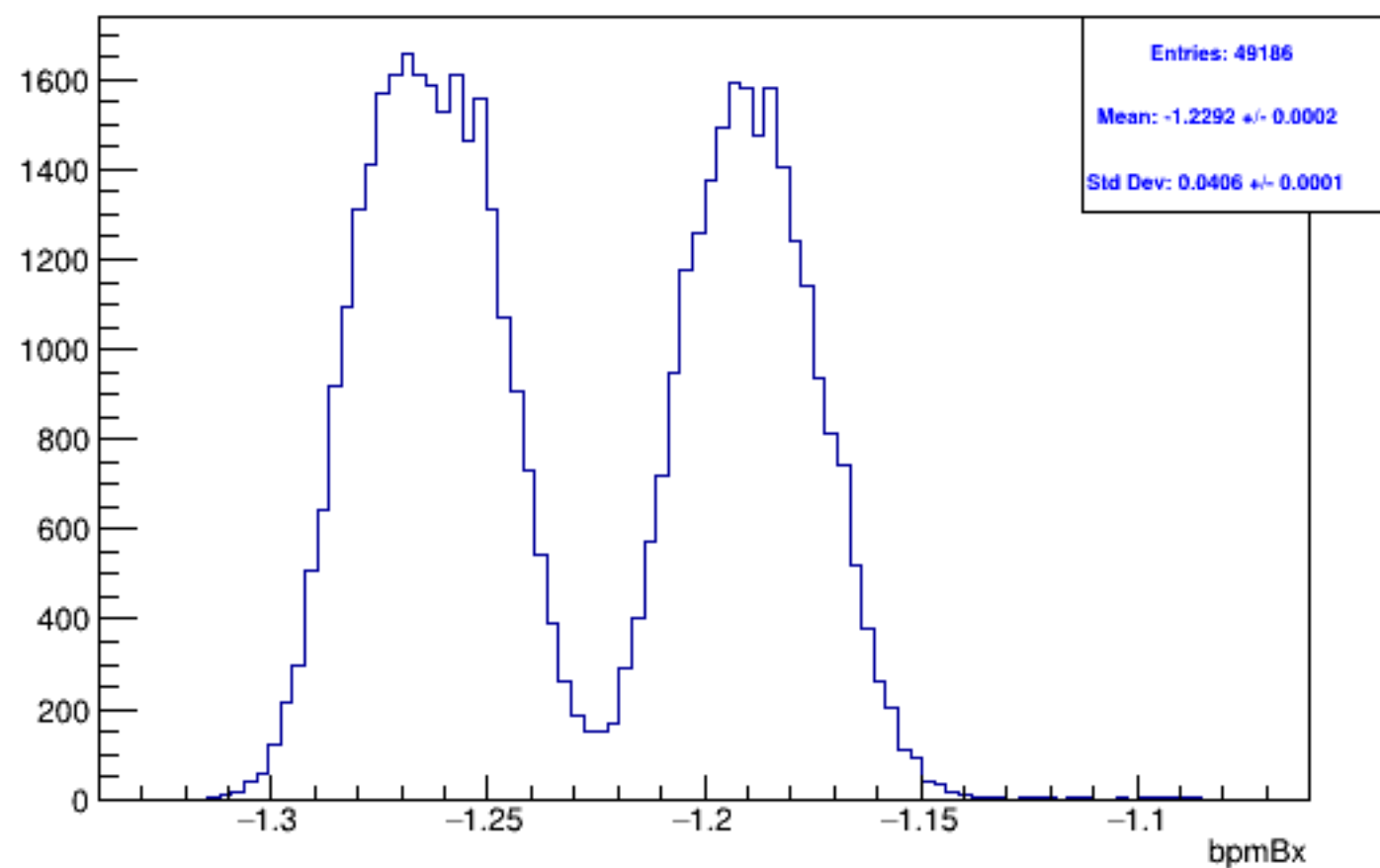
Run 5959, mpwise, bpmBx: Beam ON, Laser ON
