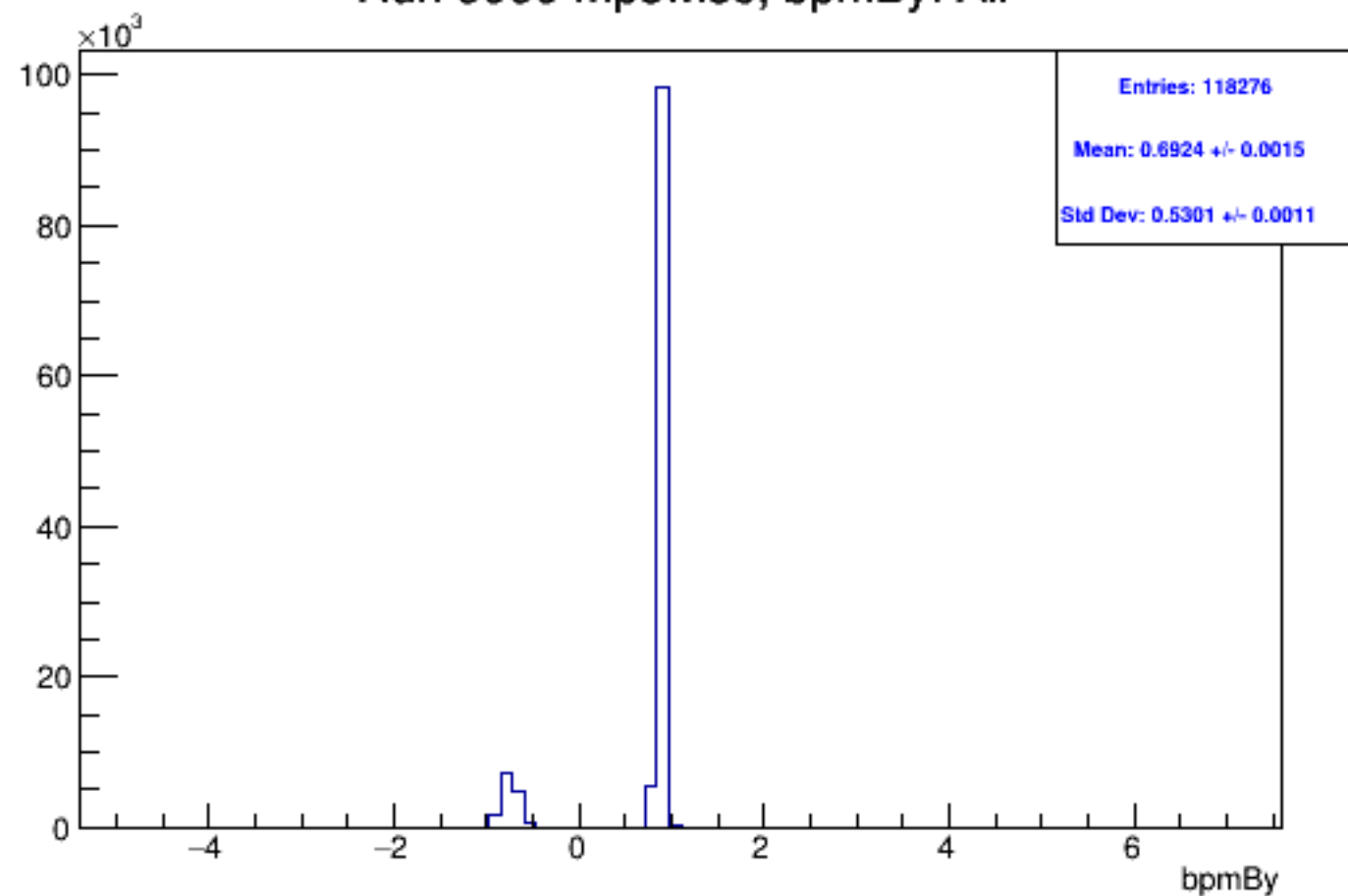
Run 5959 mpwise, bpmBy: All
