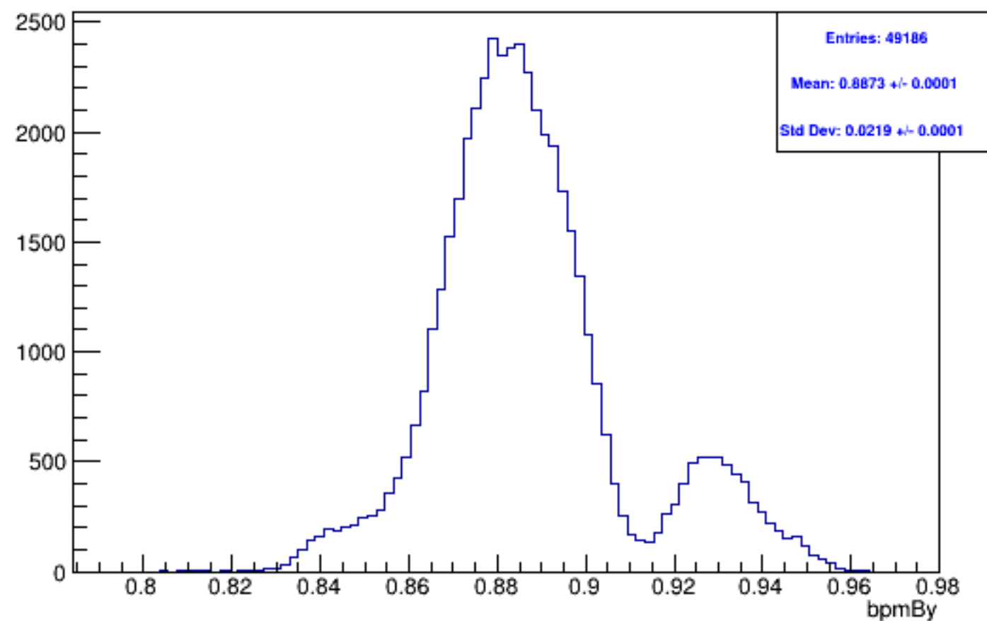
Run 5959, mpwise, bpmBy: Beam ON, Laser ON
