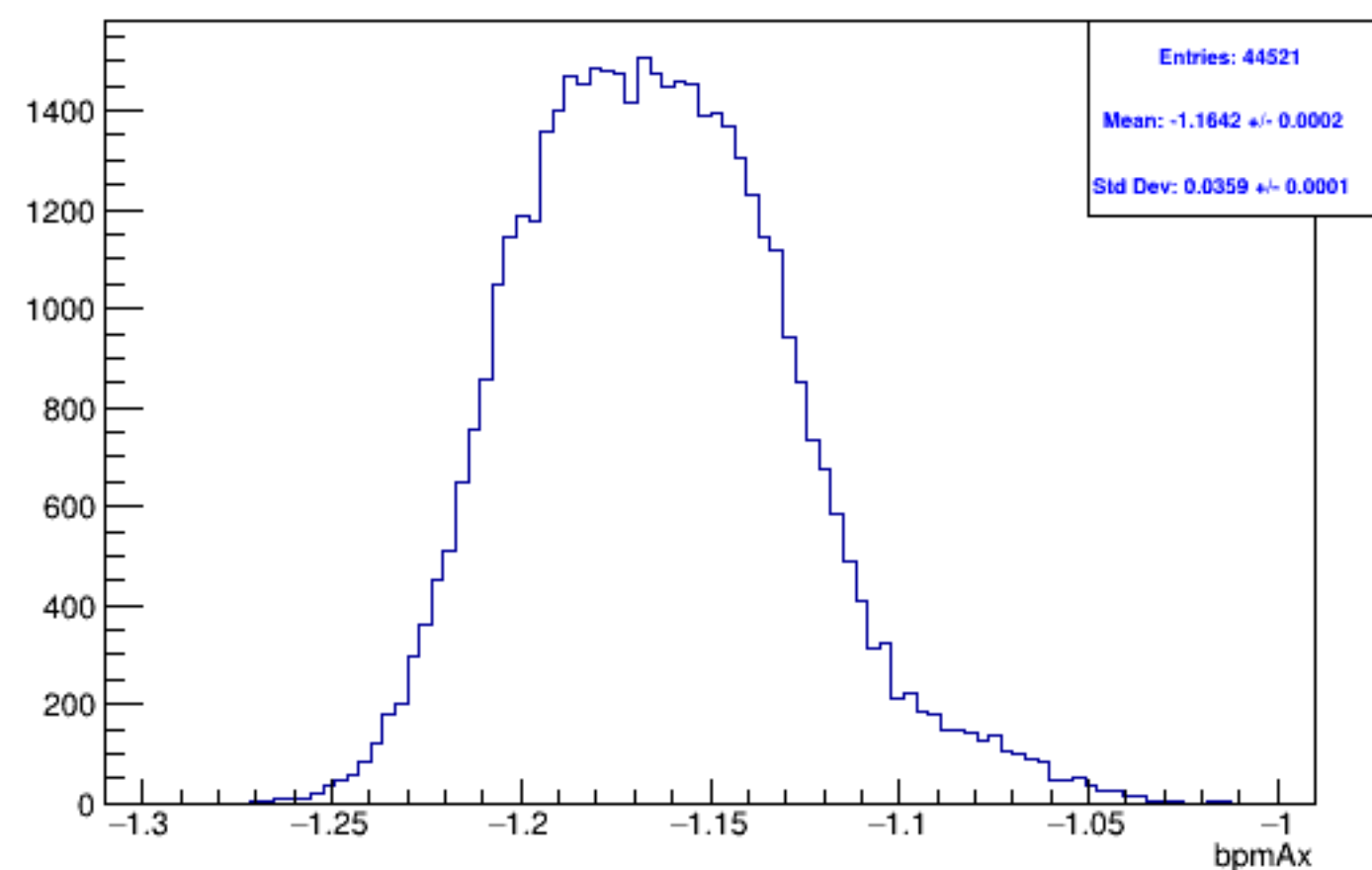
Run 5959, mpwise, bpmAx: Beam ON, Laser OFF
