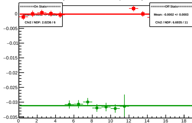
Cycle 5960.7: Multiplet Asyms
