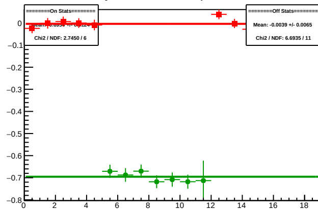
Cycle 5960.7: Multiplet Diffs
