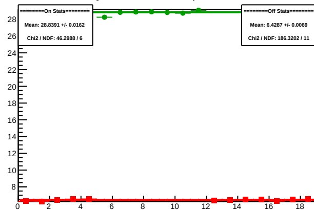
Cycle 5960.7: Multiplet Sums
