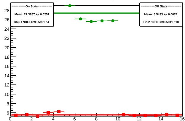
Cycle 5962.3: Multiplet Sums
