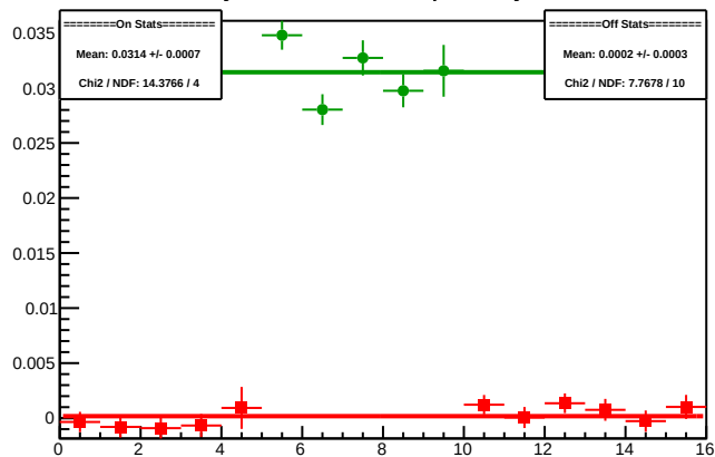
Cycle 5962.3: Multiplet Asyms
