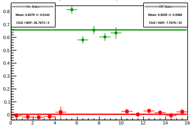
Cycle 5962.3: Multiplet Diffs
