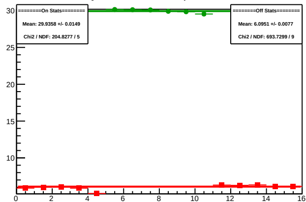
Cycle 5962.8: Multiplet Sums
