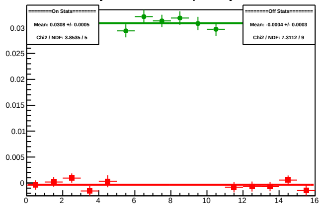
Cycle 5962.8: Multiplet Asyms
