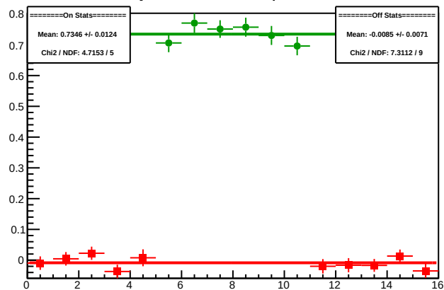
Cycle 5962.8: Multiplet Diffs
