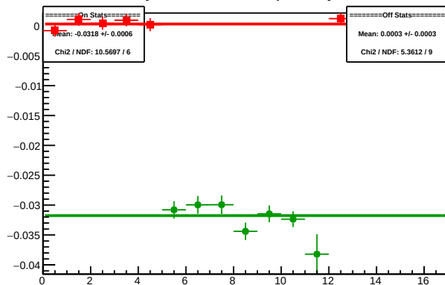
Cycle 5967.1: Multiplet Asyms
