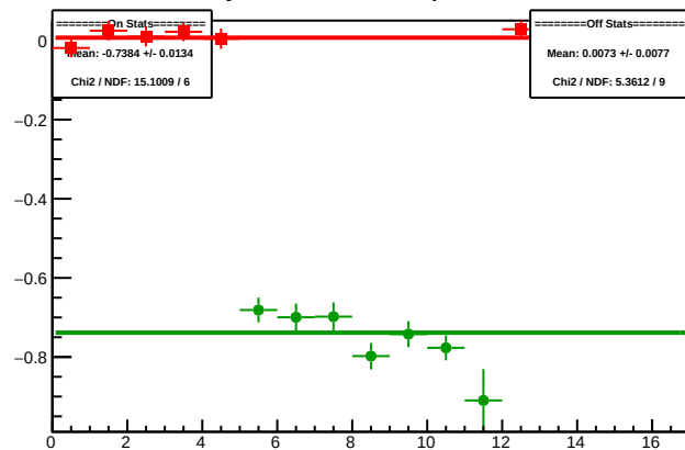
Cycle 5967.1: Multiplet Diffs
