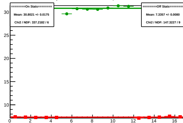
Cycle 5967.1: Multiplet Sums
