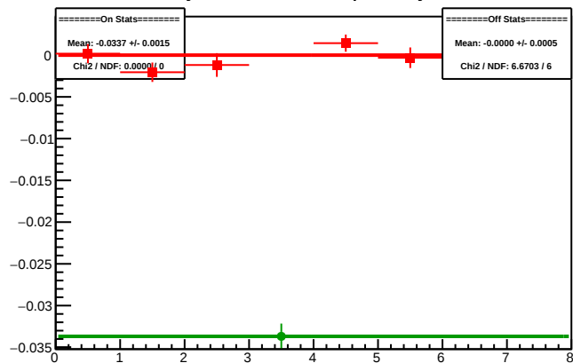
Cycle 5967.9: Multiplet Asyms
