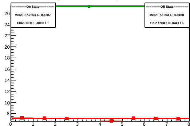
Cycle 5967.9: Multiplet Sums
