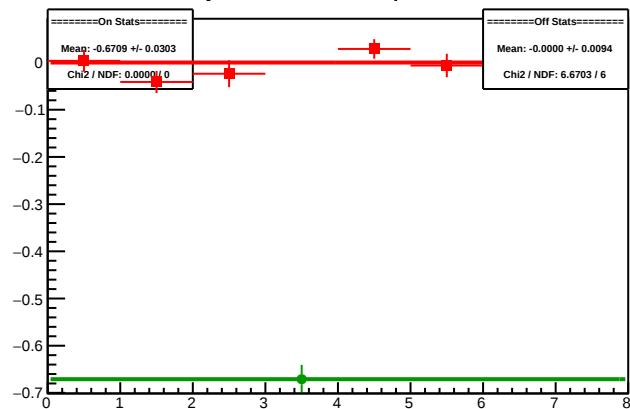
Cycle 5967.9: Multiplet Diffs
