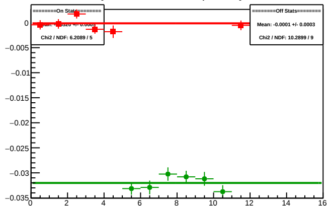
Cycle 5967.13: Multiplet Asyms
