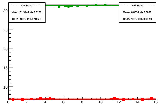
Cycle 5967.13: Multiplet Sums
