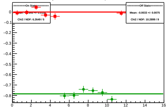
Cycle 5967.13: Multiplet Diffs
