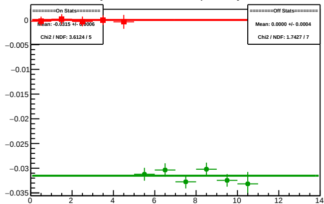
Cycle 5967.14: Multiplet Asyms
