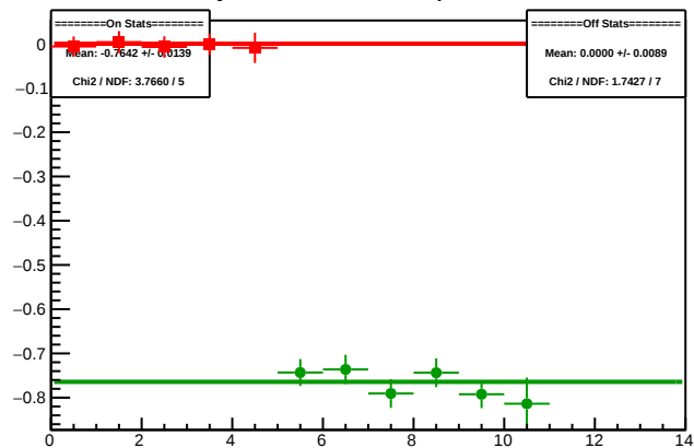
Cycle 5967.14: Multiplet Diffs
