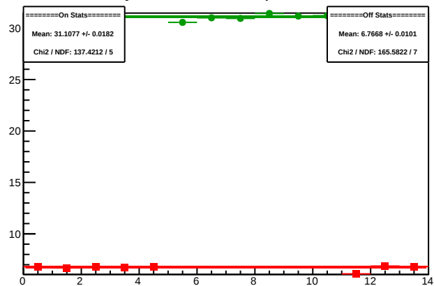
Cycle 5967.14: Multiplet Sums
